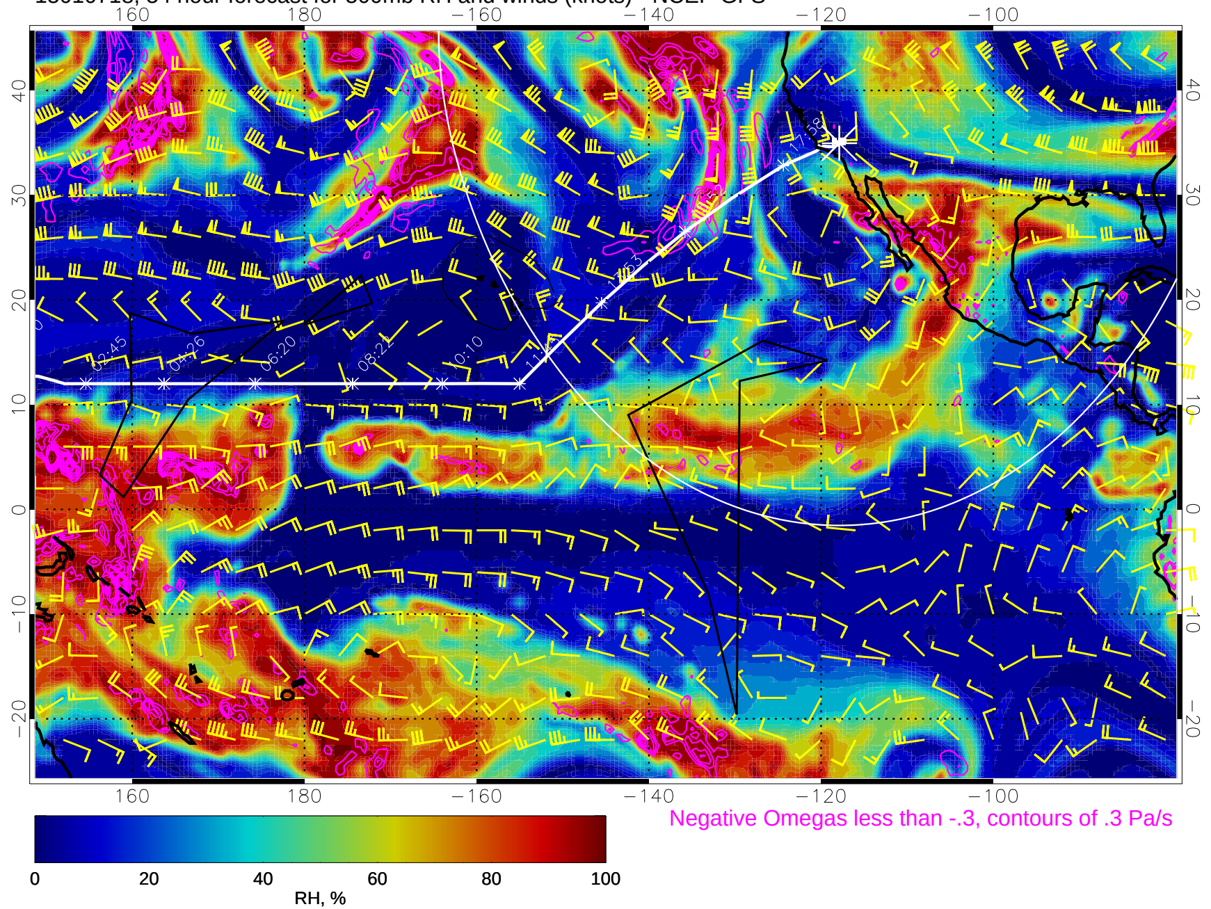
15010718, 54 hour forecast for 500mb RH and winds (knots) - NCEP GFS
