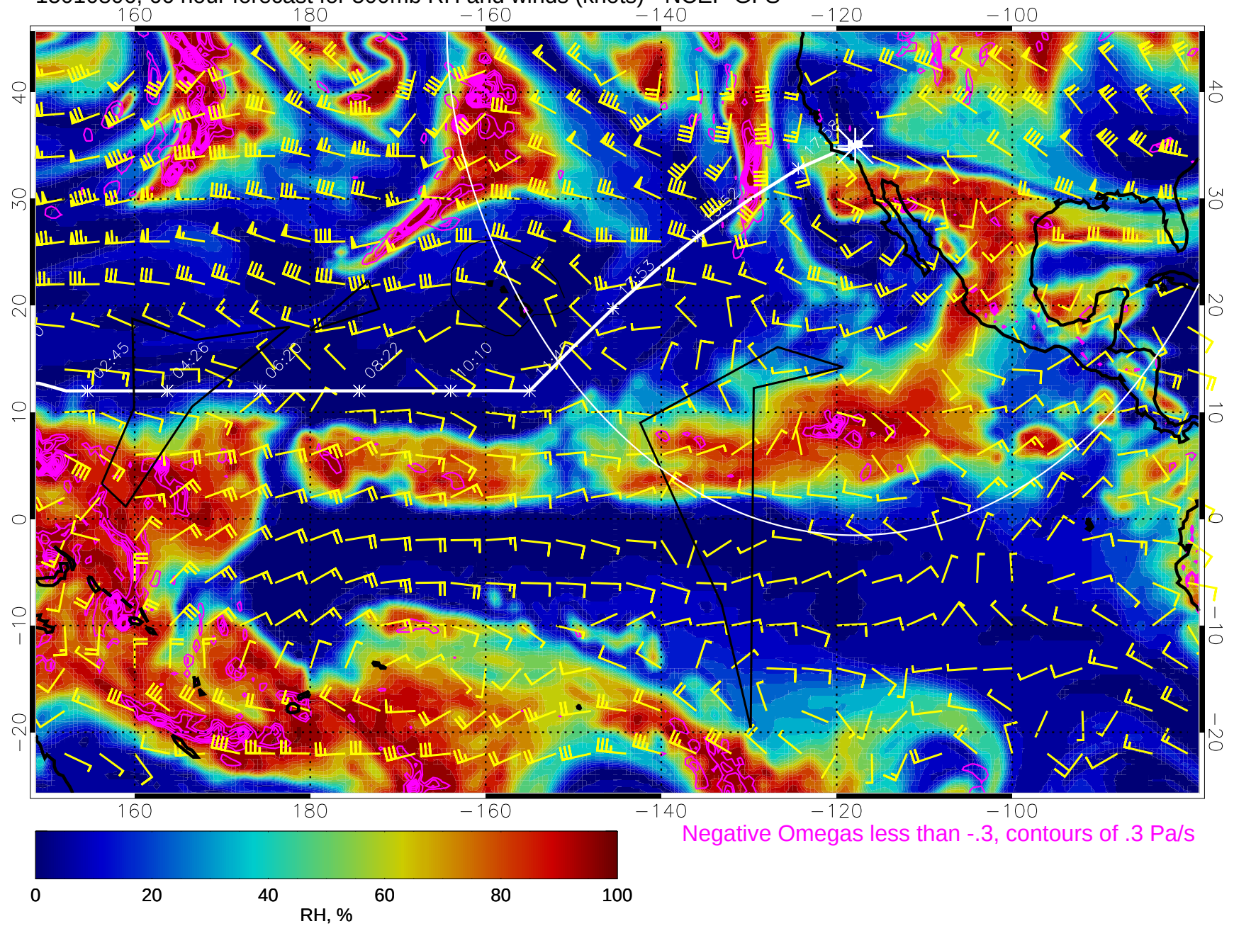
15010806, 66 hour forecast for 500mb RH and winds (knots) - NCEP GFS
