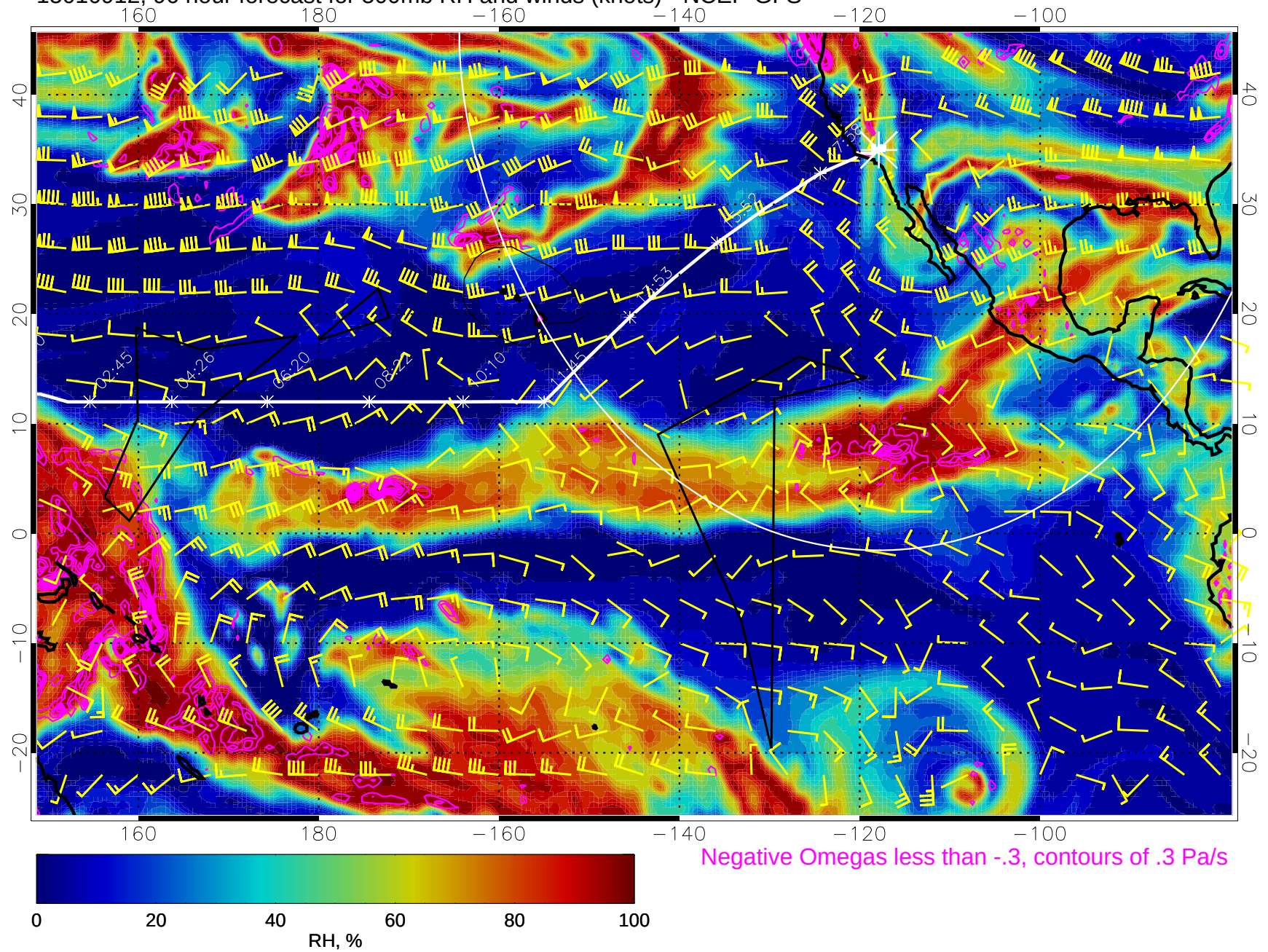
15010912, 96 hour forecast for 500mb RH and winds (knots) - NCEP GFS
