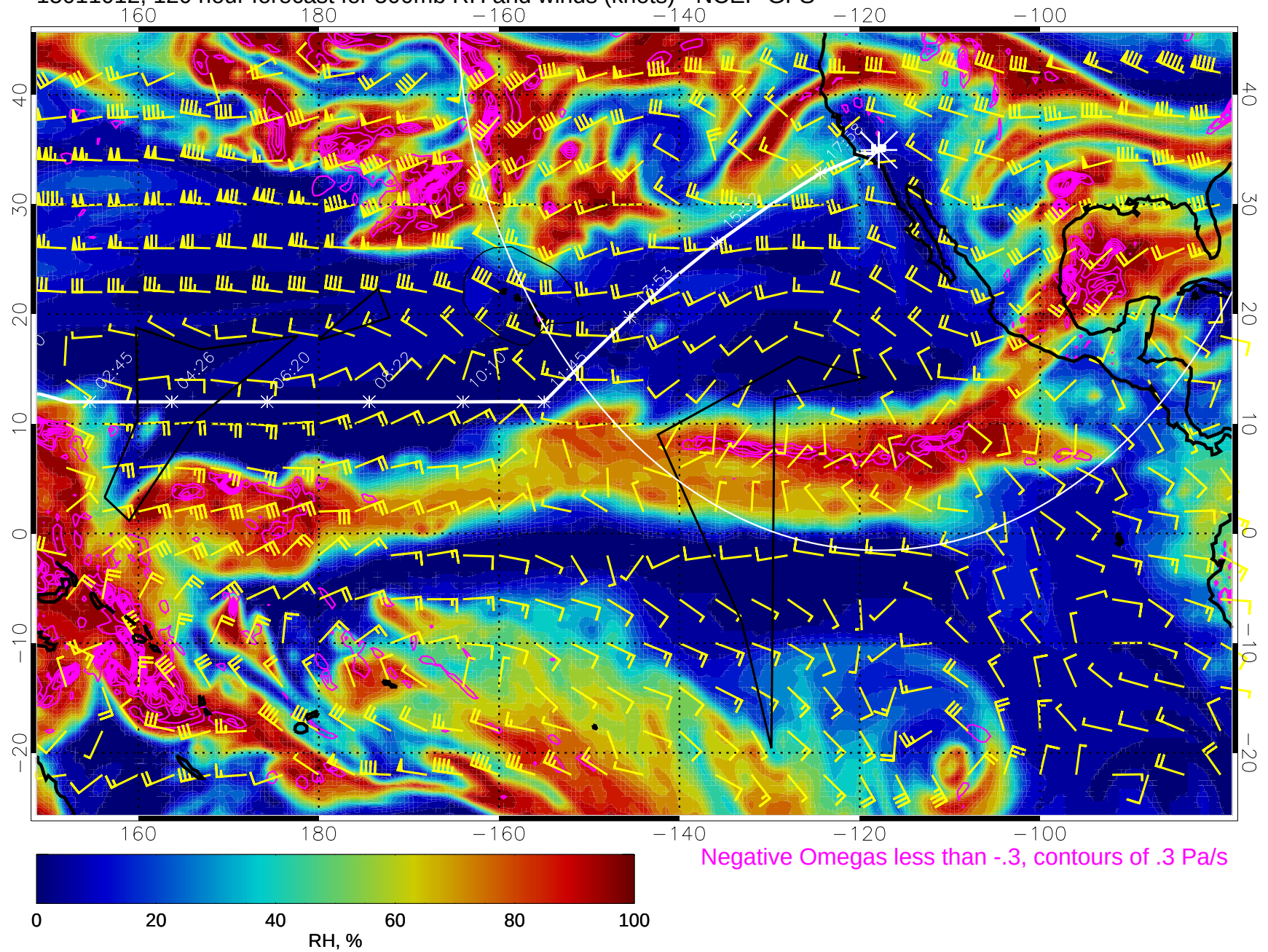
15011012, 120 hour forecast for 500mb RH and winds (knots) - NCEP GFS
