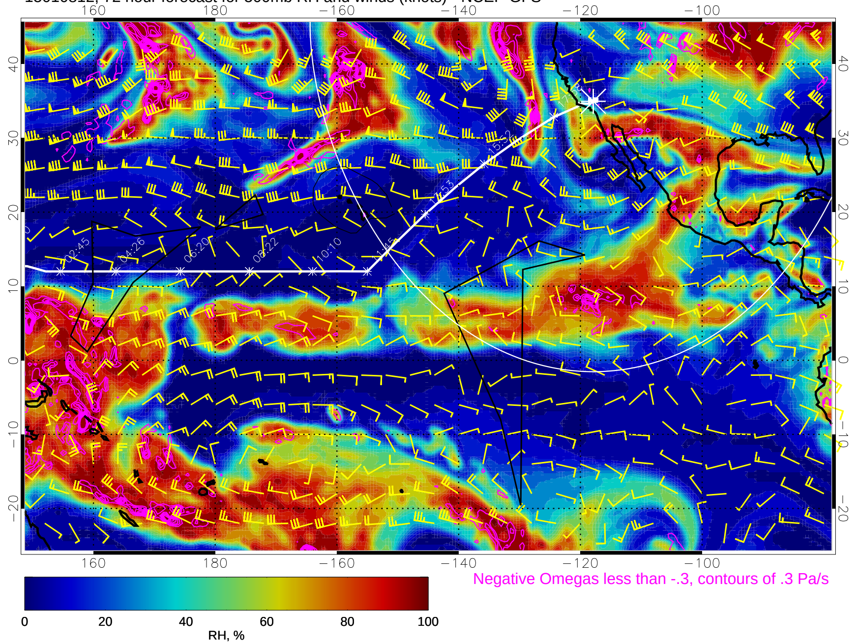
15010812, 72 hour forecast for 500mb RH and winds (knots) - NCEP GFS
