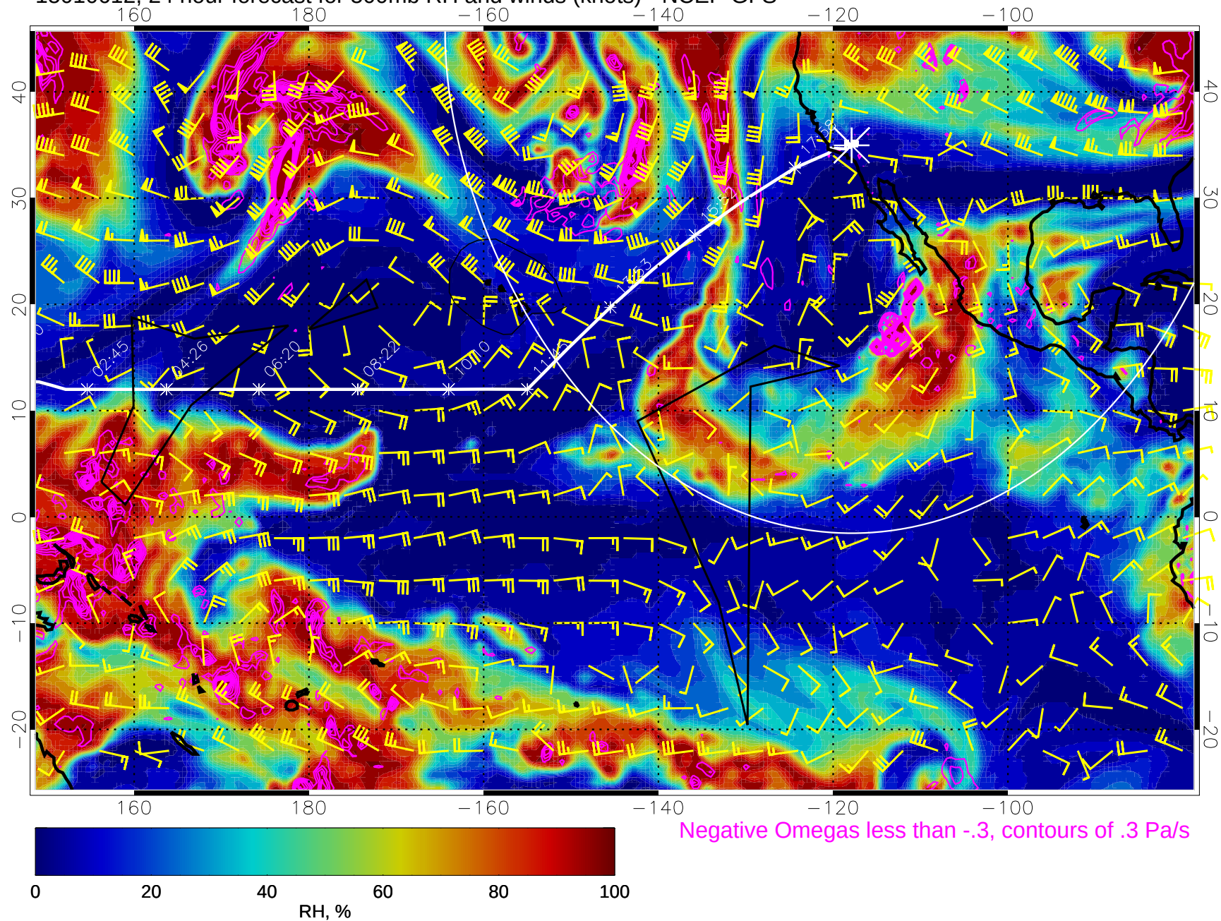
15010612, 24 hour forecast for 500mb RH and winds (knots) - NCEP GFS
