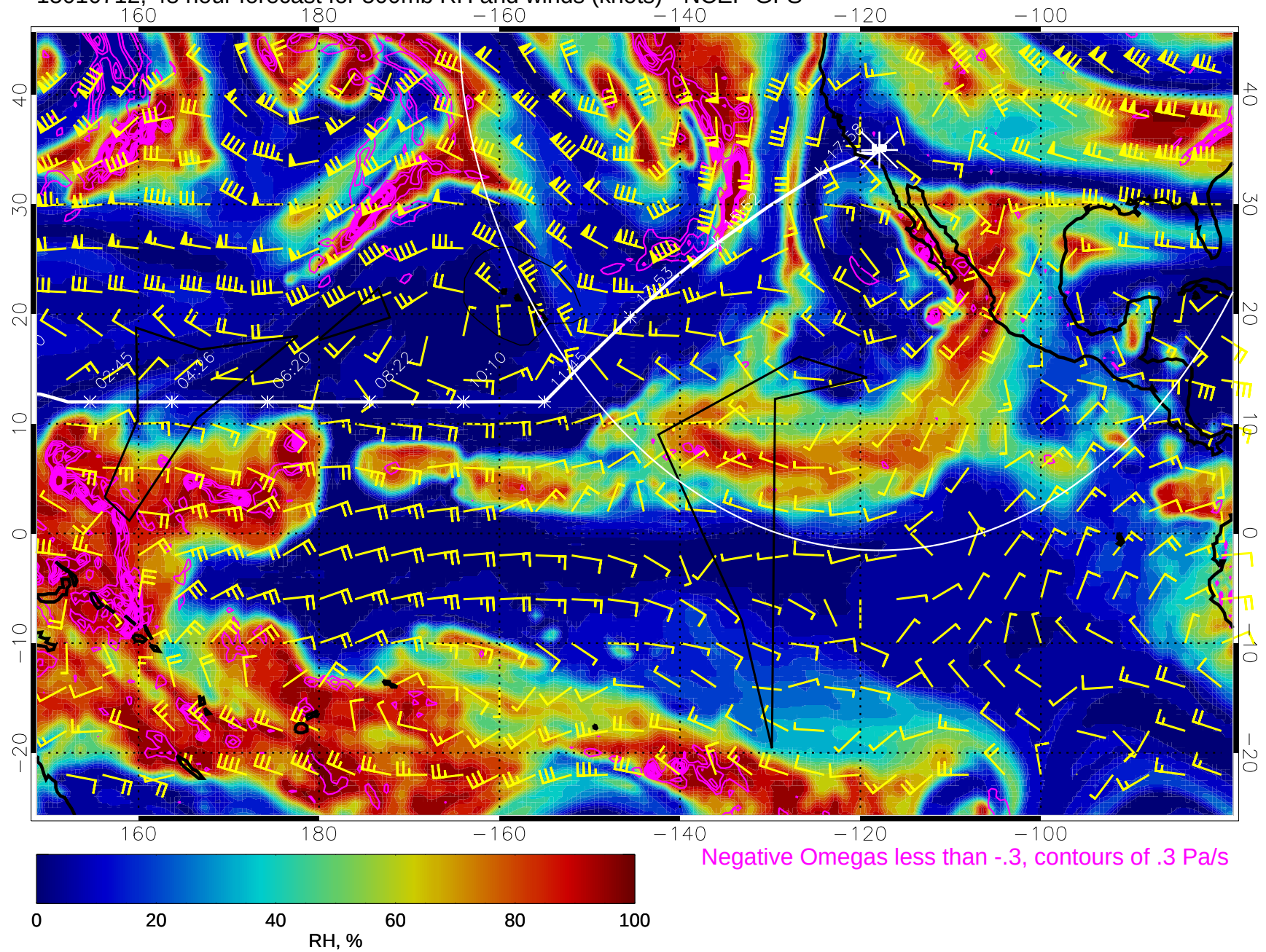
15010712, 48 hour forecast for 500mb RH and winds (knots) - NCEP GFS
