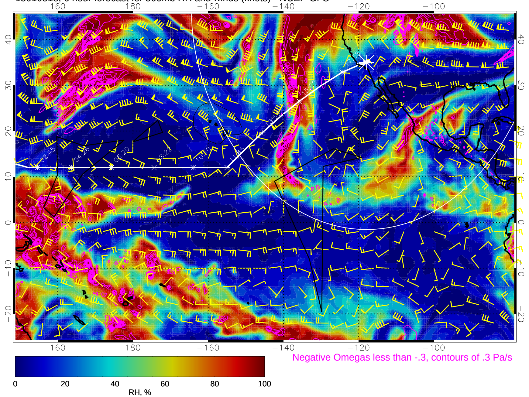
15010518, 6 hour forecast for 500mb RH and winds (knots) - NCEP GFS
