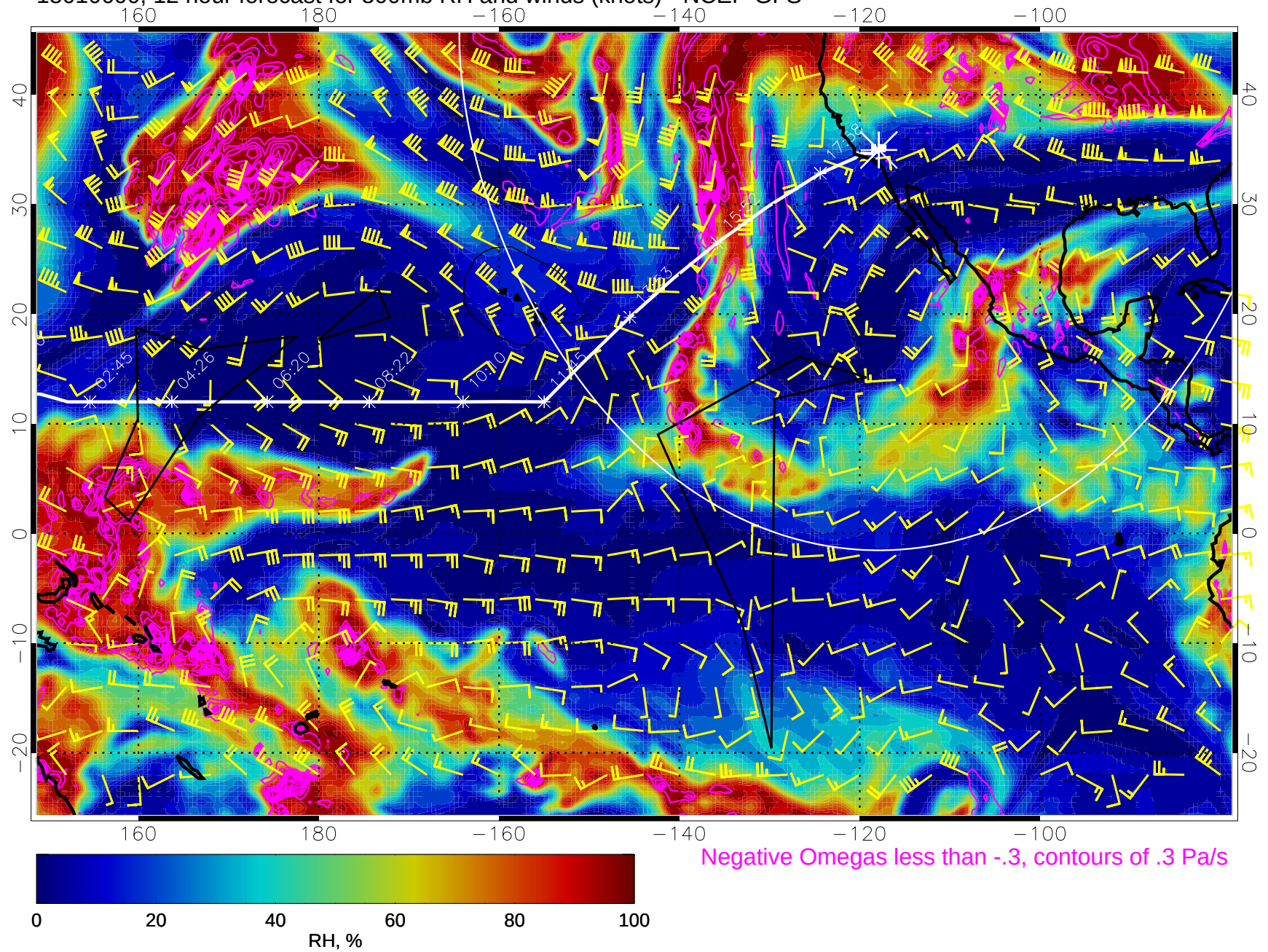
15010600, 12 hour forecast for 500mb RH and winds (knots) - NCEP GFS
