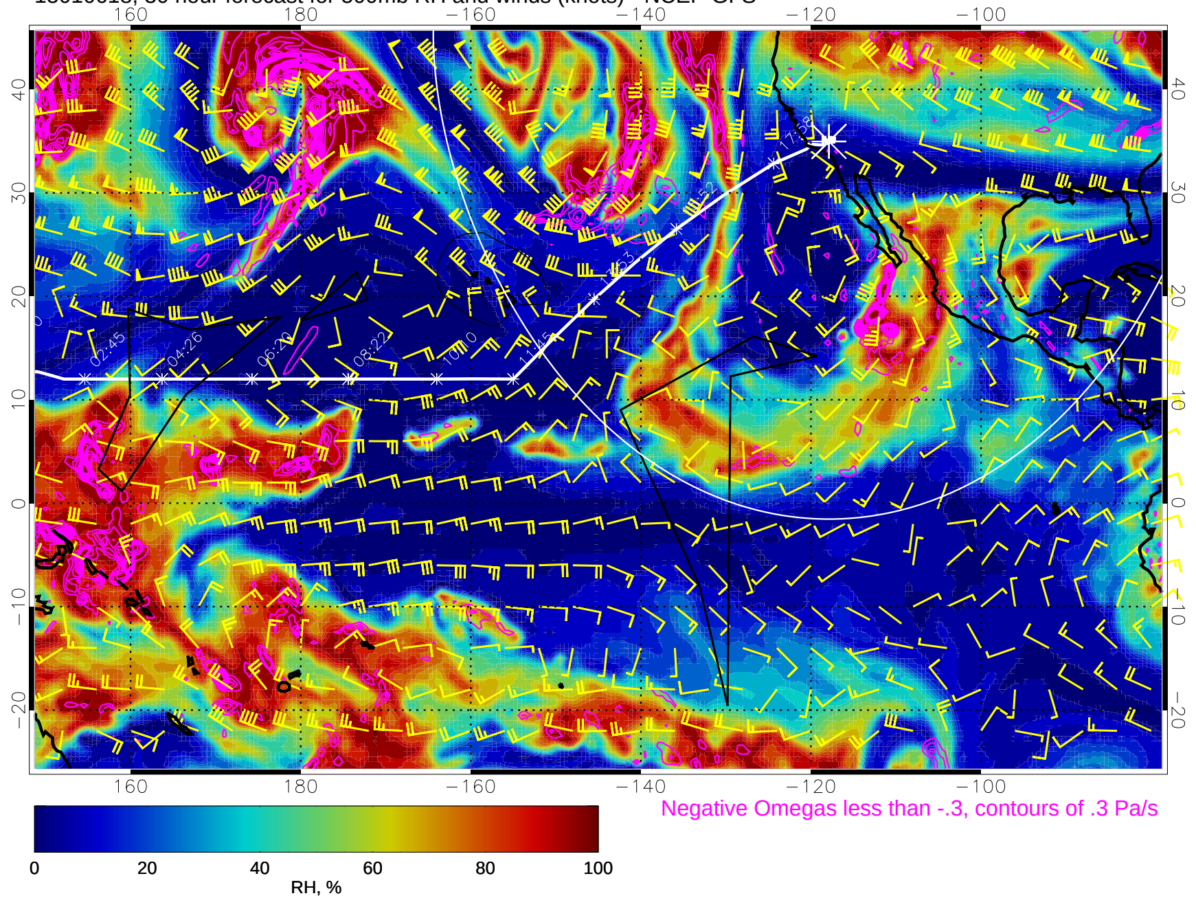
15010618, 30 hour forecast for 500mb RH and winds (knots) - NCEP GFS
