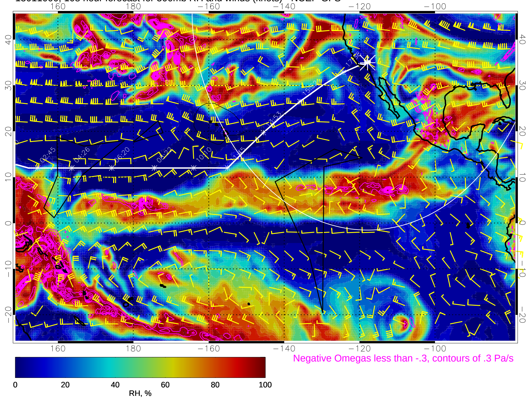
15011000, 108 hour forecast for 500mb RH and winds (knots) - NCEP GFS
