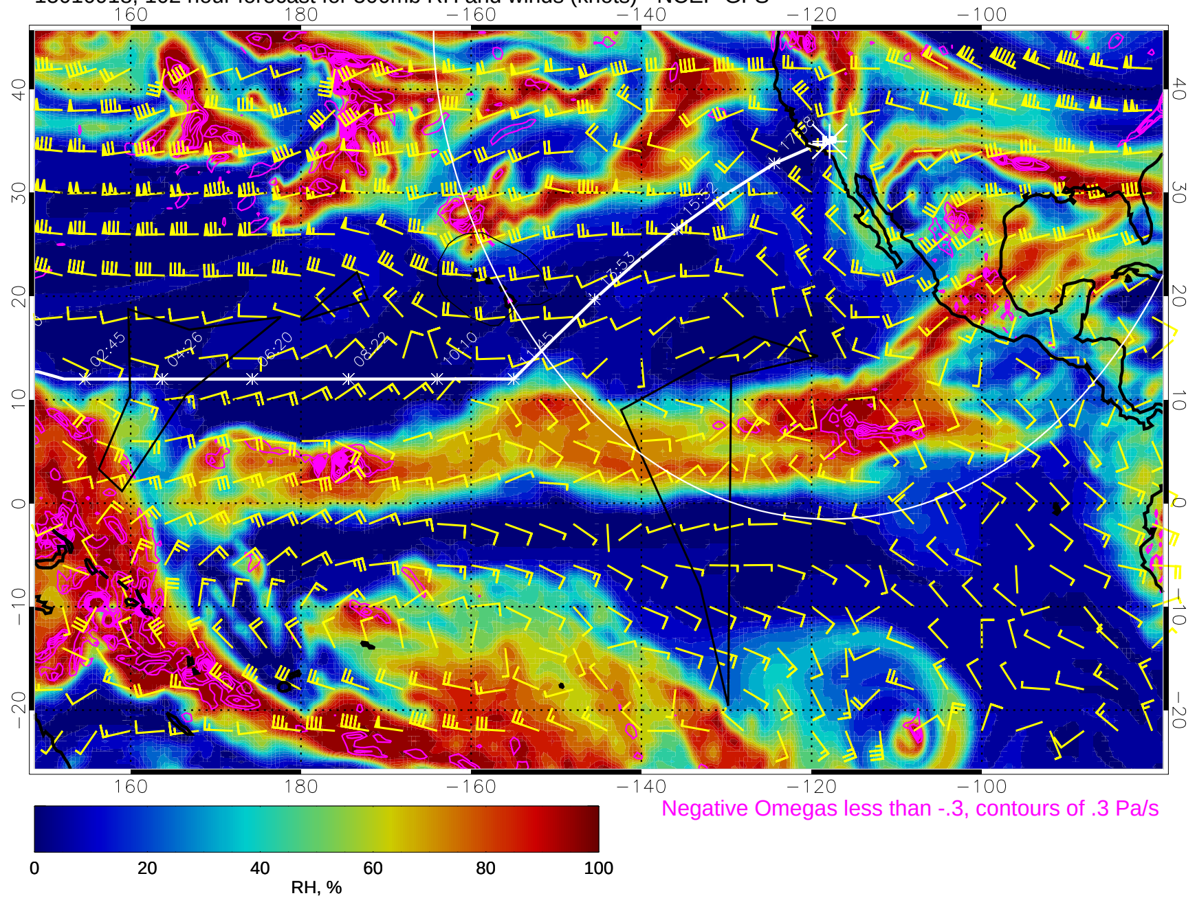
15010918, 102 hour forecast for 500mb RH and winds (knots) - NCEP GFS
