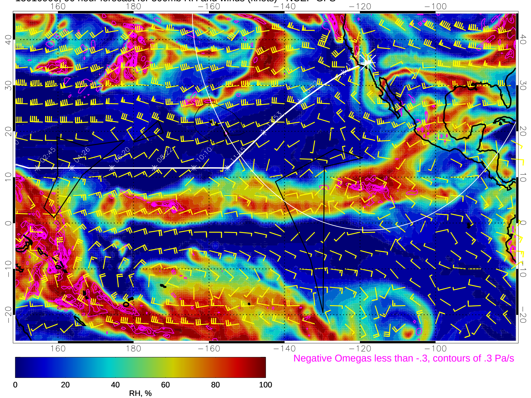
15010906, 90 hour forecast for 500mb RH and winds (knots) - NCEP GFS
