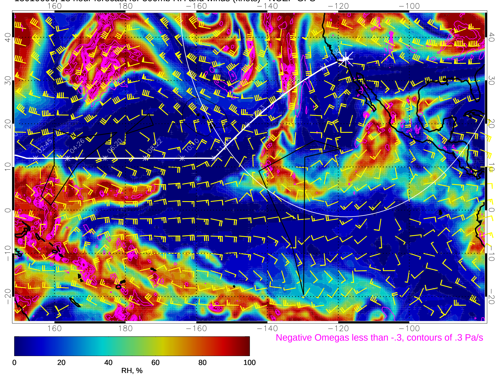
15010606, 18 hour forecast for 500mb RH and winds (knots) - NCEP GFS
