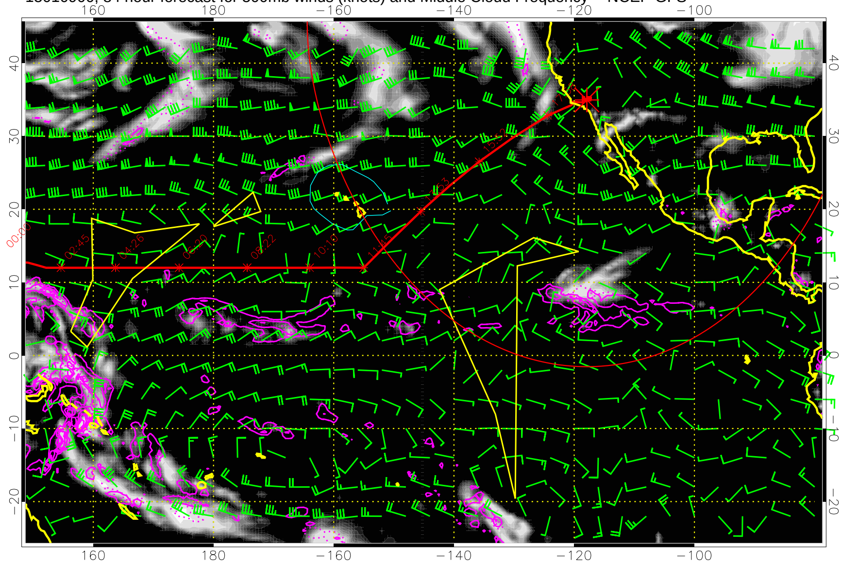
15010900, 84 hour forecast for 500mb winds (knots) and Middle Cloud Frequency -- NCEP GFS
