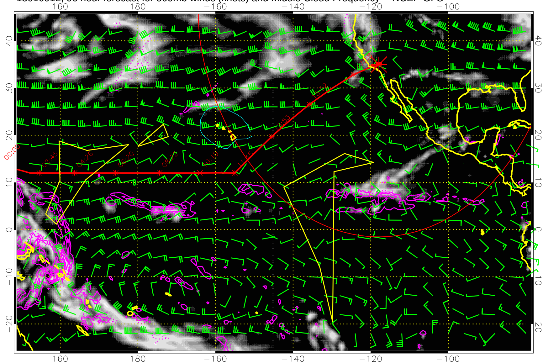
15010912, 96 hour forecast for 500mb winds (knots) and Middle Cloud Frequency -- NCEP GFS
