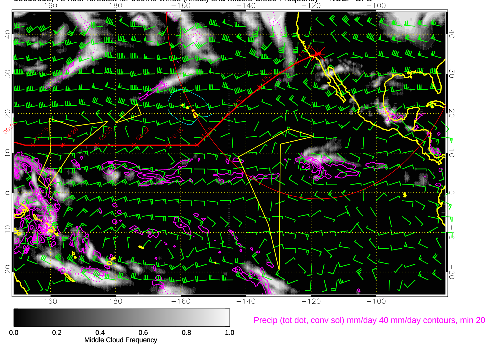
15010818, 78 hour forecast for 500mb winds (knots) and Middle Cloud Frequency -- NCEP GFS
