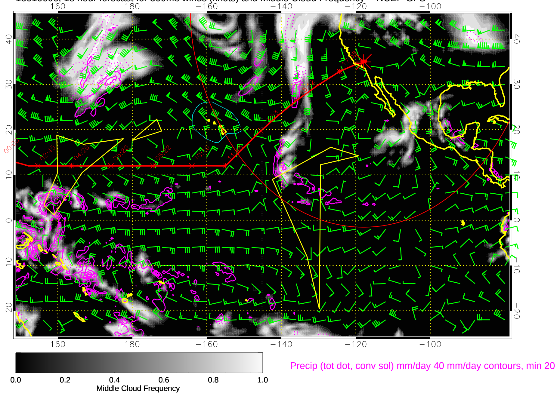
15010606, 18 hour forecast for 500mb winds (knots) and Middle Cloud Frequency -- NCEP GFS
