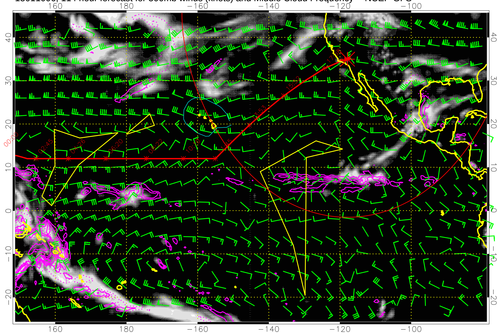
15011006, 114 hour forecast for 500mb winds (knots) and Middle Cloud Frequency -- NCEP GFS
