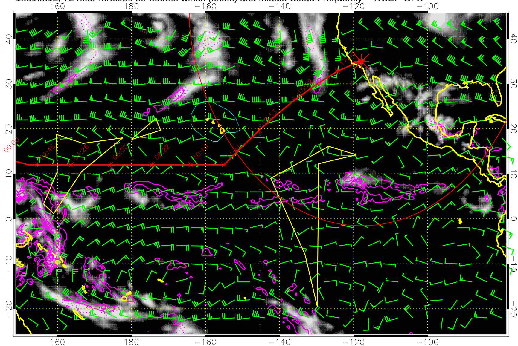
15010812, 72 hour forecast for 500mb winds (knots) and Middle Cloud Frequency -- NCEP GFS
