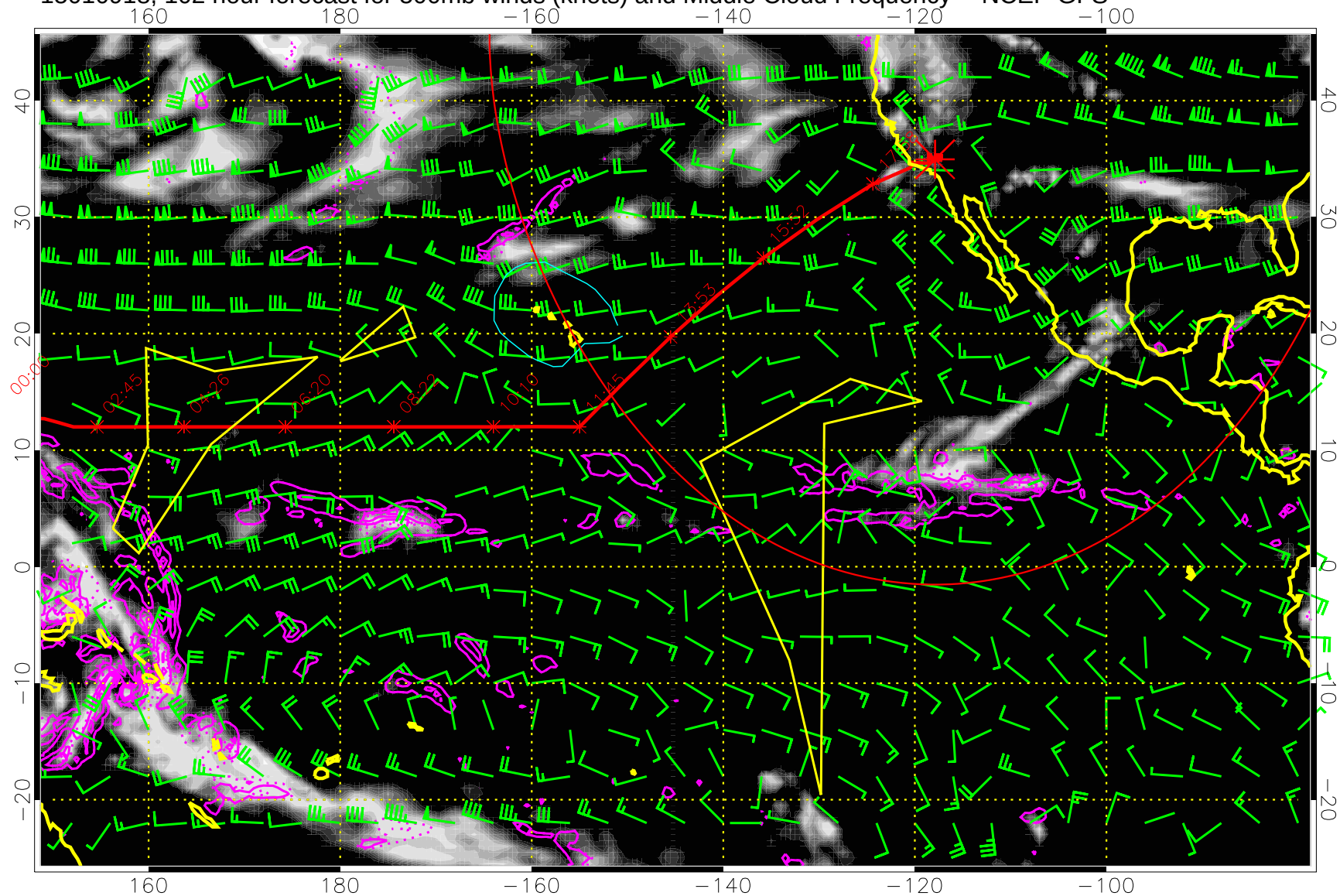
15010918, 102 hour forecast for 500mb winds (knots) and Middle Cloud Frequency -- NCEP GFS
