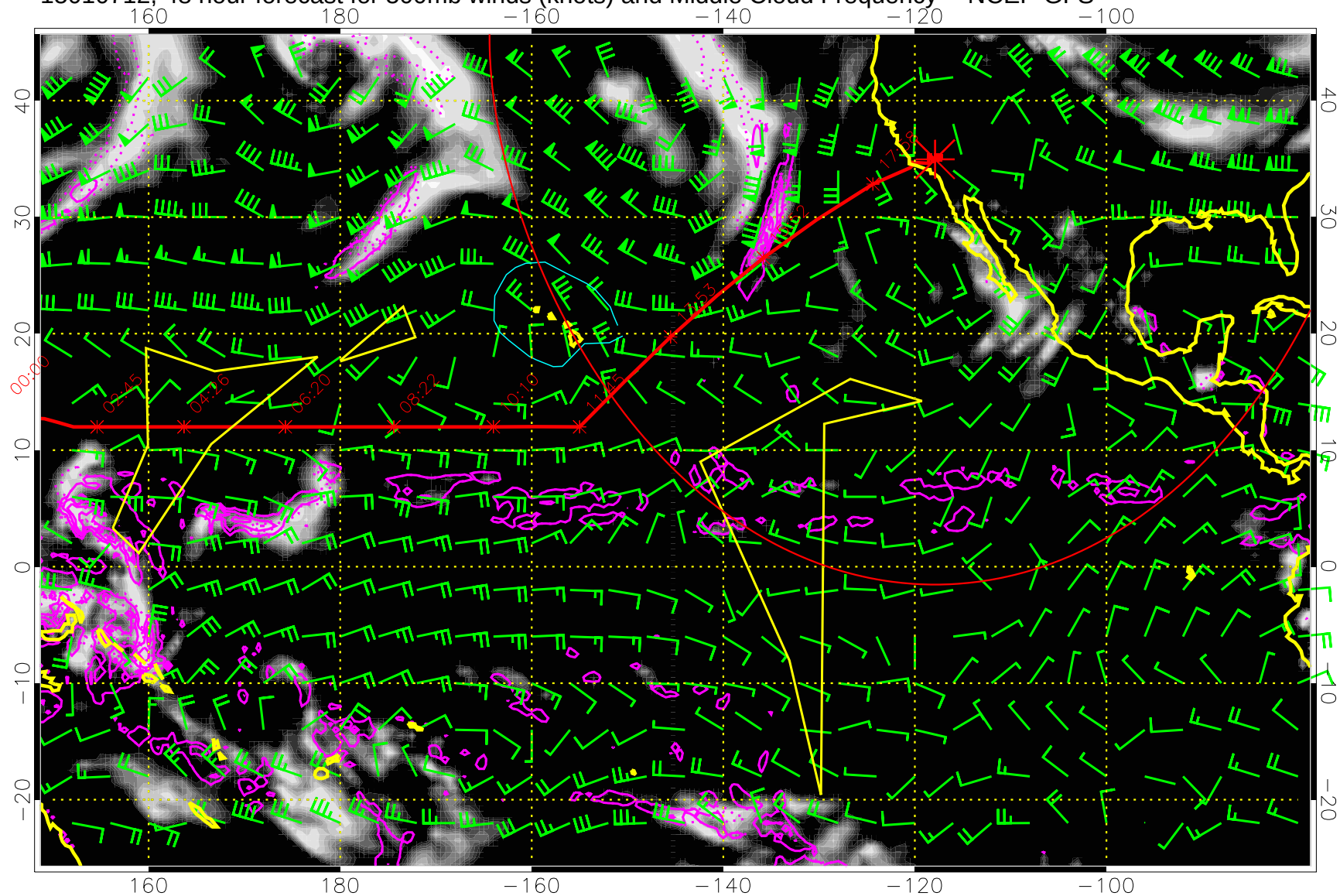
15010712, 48 hour forecast for 500mb winds (knots) and Middle Cloud Frequency -- NCEP GFS
