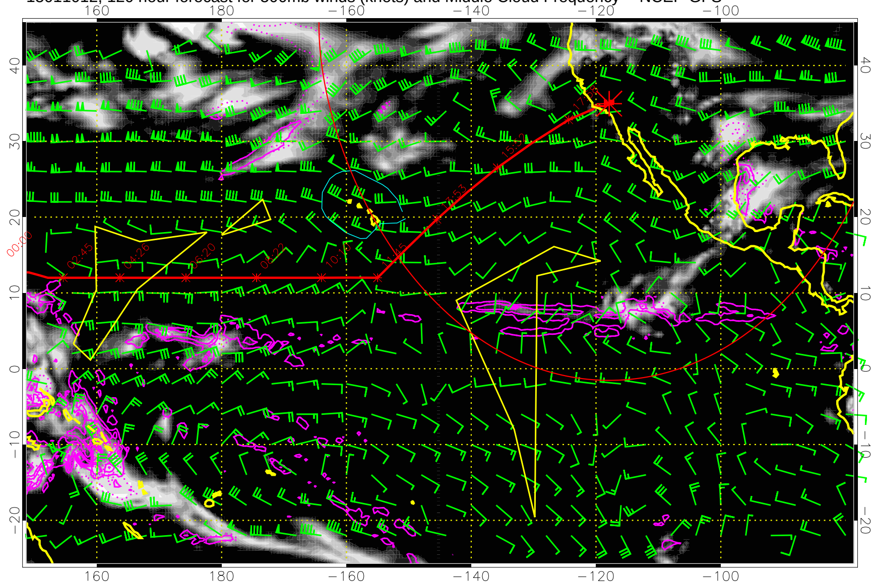
15011012, 120 hour forecast for 500mb winds (knots) and Middle Cloud Frequency -- NCEP GFS
