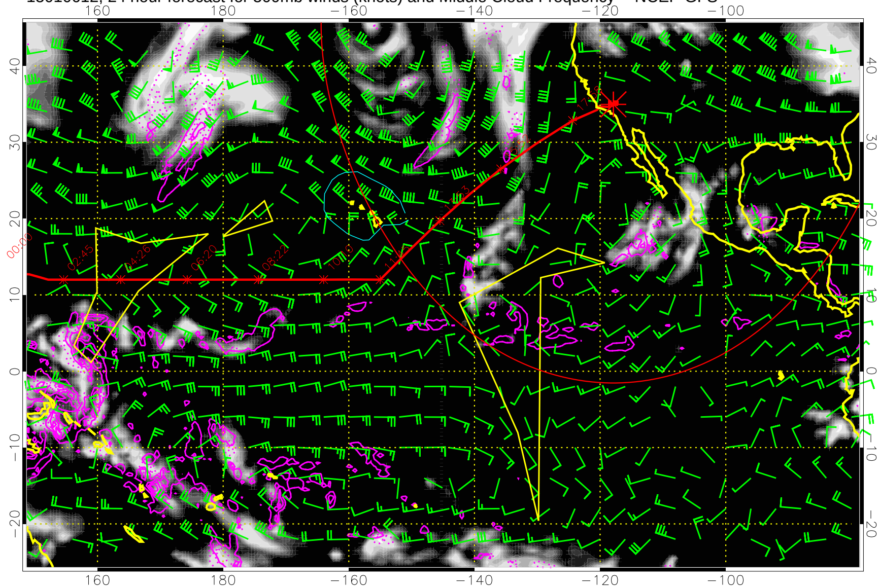
15010612, 24 hour forecast for 500mb winds (knots) and Middle Cloud Frequency -- NCEP GFS
