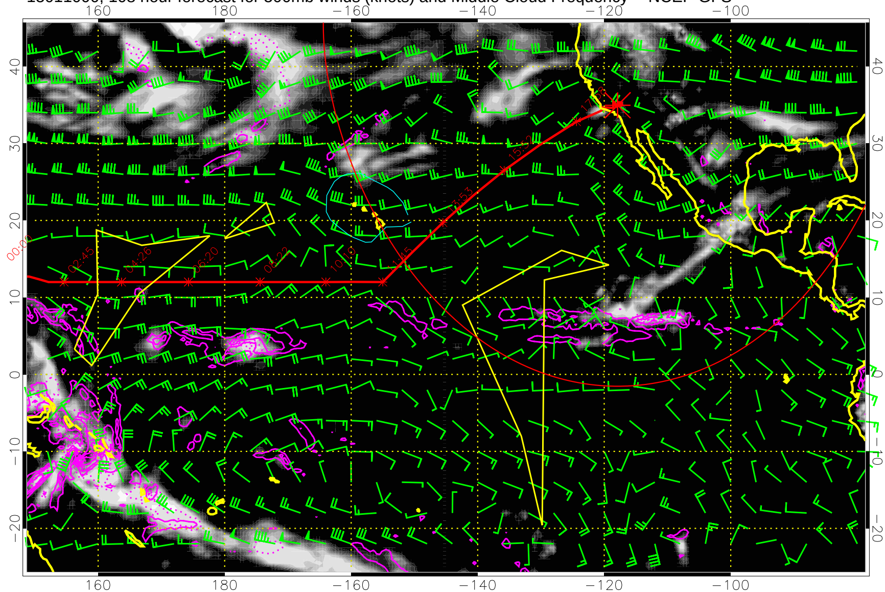
15011000, 108 hour forecast for 500mb winds (knots) and Middle Cloud Frequency -- NCEP GFS
