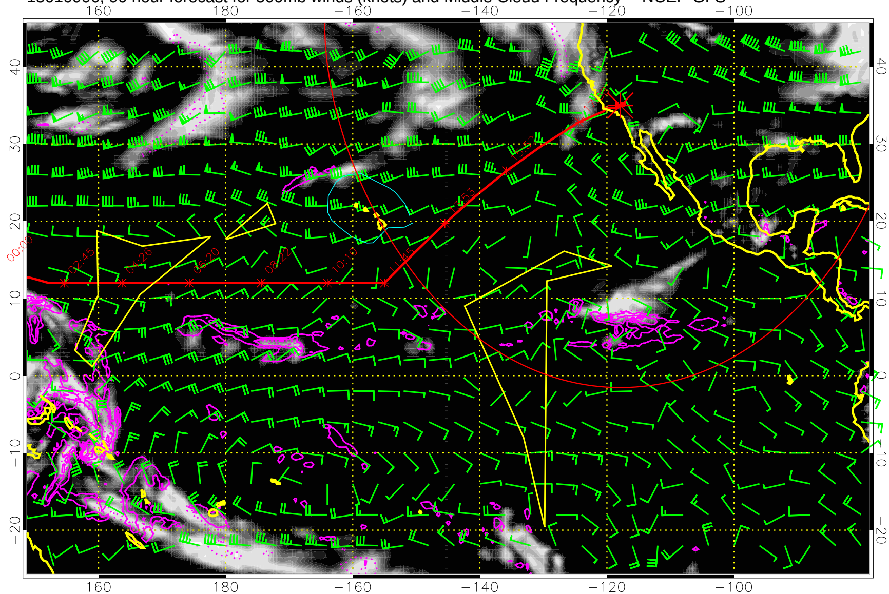
15010906, 90 hour forecast for 500mb winds (knots) and Middle Cloud Frequency -- NCEP GFS
