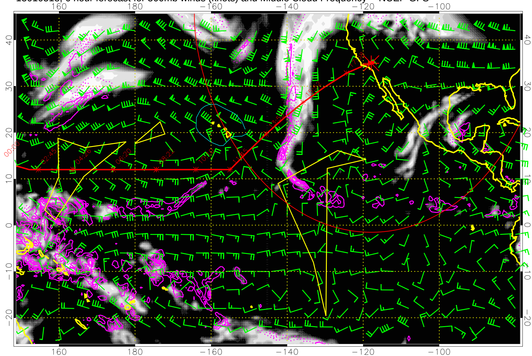
15010518, 6 hour forecast for 500mb winds (knots) and Middle Cloud Frequency -- NCEP GFS
