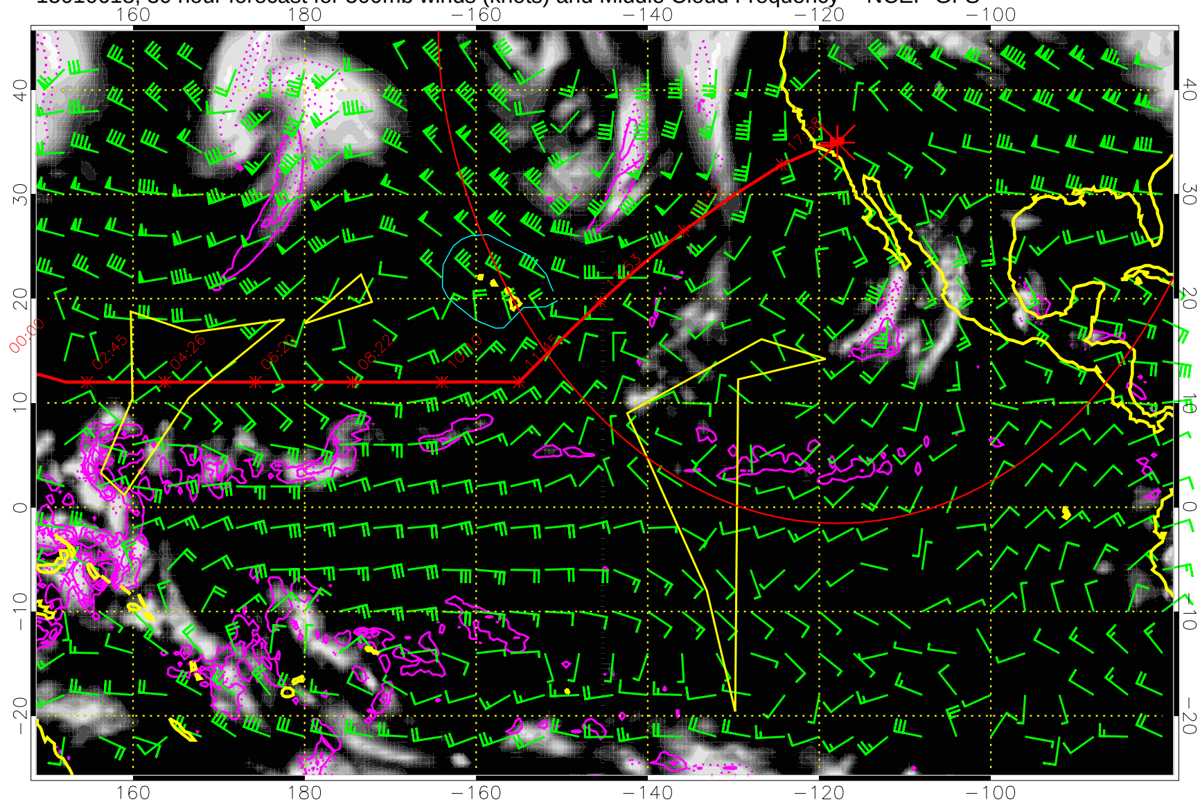
15010618, 30 hour forecast for 500mb winds (knots) and Middle Cloud Frequency -- NCEP GFS
