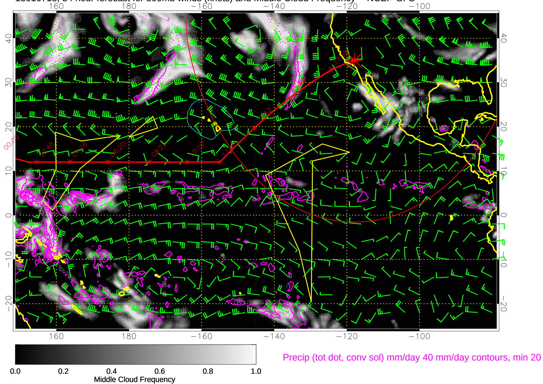
15010718, 54 hour forecast for 500mb winds (knots) and Middle Cloud Frequency -- NCEP GFS
