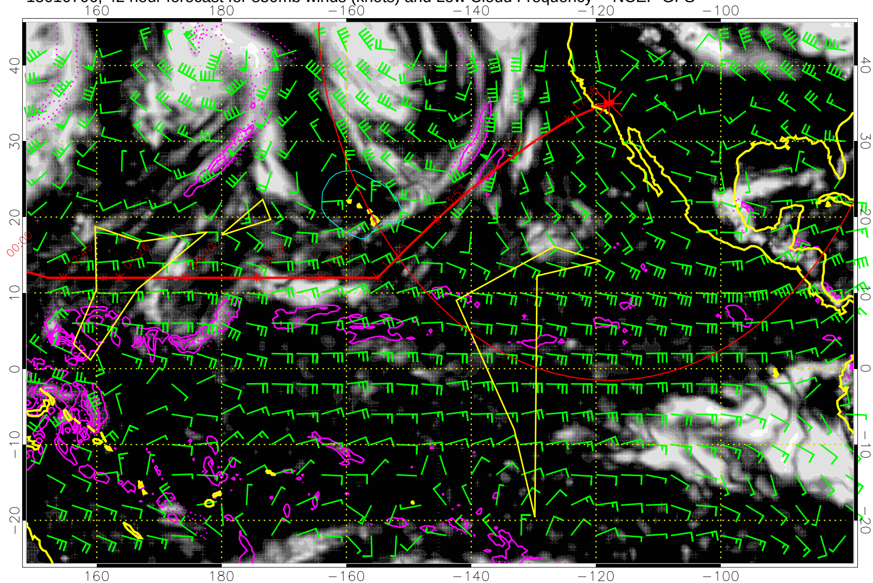
15010706, 42 hour forecast for 850mb winds (knots) and Low Cloud Frequency -- NCEP GFS
