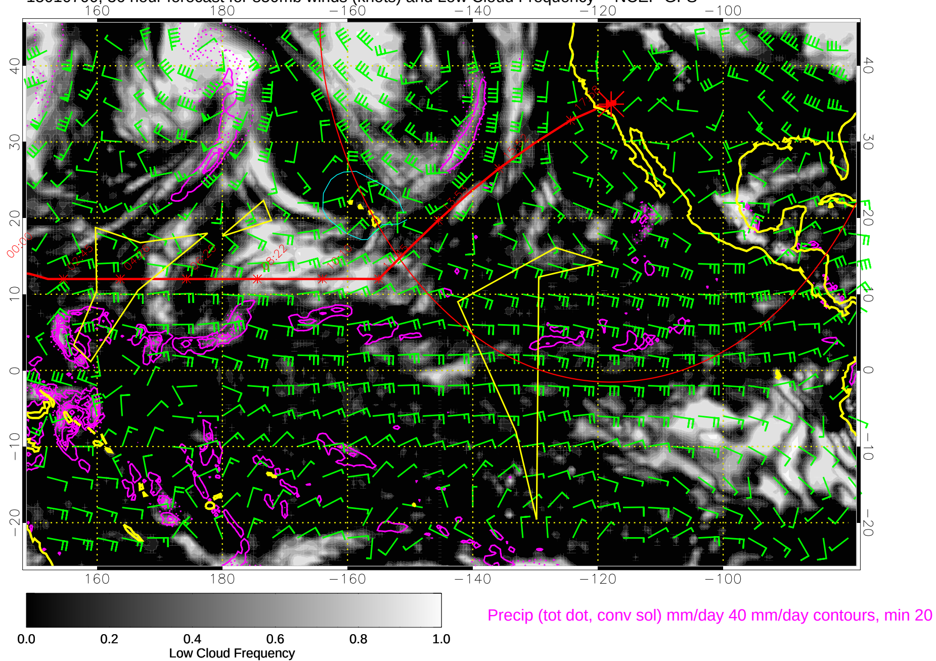
15010700, 36 hour forecast for 850mb winds (knots) and Low Cloud Frequency -- NCEP GFS
