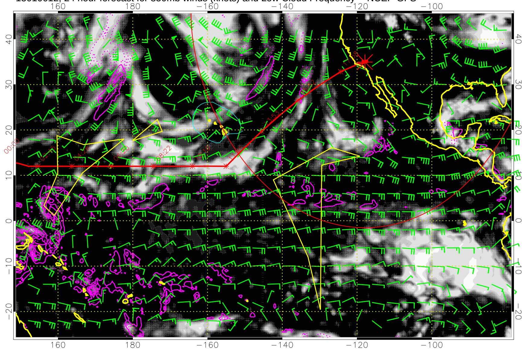
15010612, 24 hour forecast for 850mb winds (knots) and Low Cloud Frequency -- NCEP GFS
