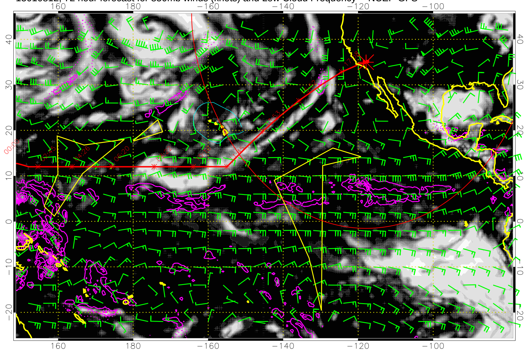
15010812, 72 hour forecast for 850mb winds (knots) and Low Cloud Frequency -- NCEP GFS
