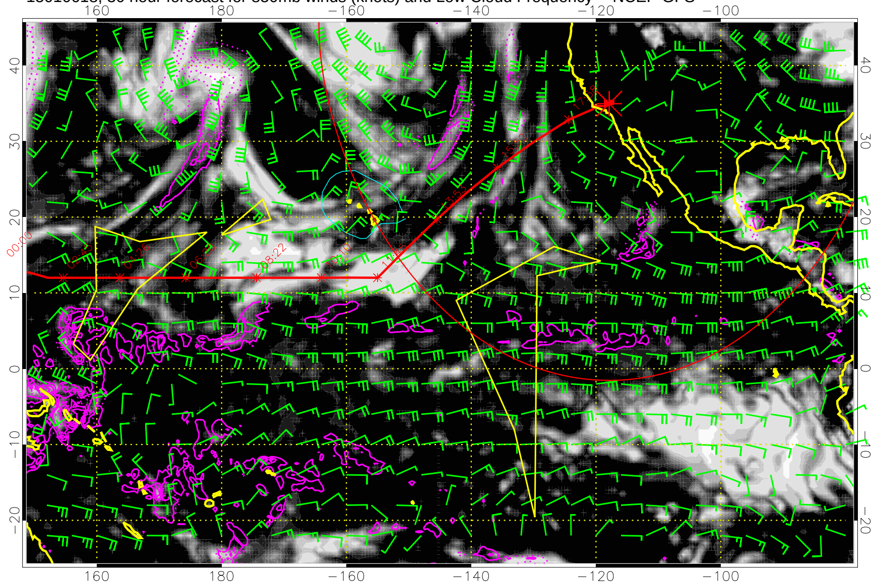
15010618, 30 hour forecast for 850mb winds (knots) and Low Cloud Frequency -- NCEP GFS
