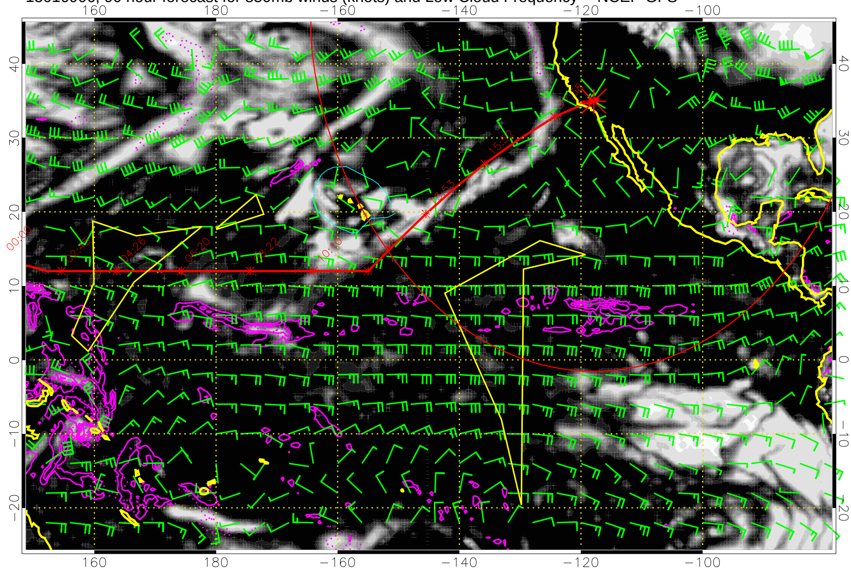
15010906, 90 hour forecast for 850mb winds (knots) and Low Cloud Frequency -- NCEP GFS
