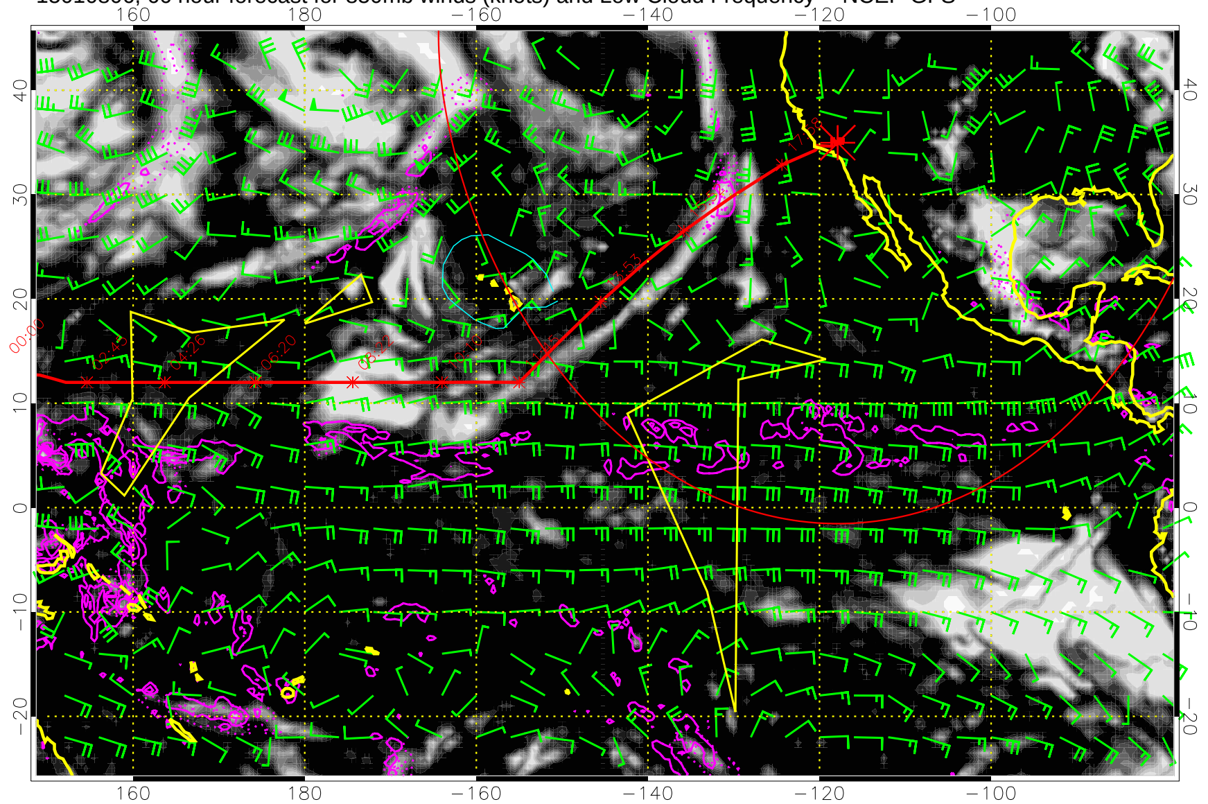
15010806, 66 hour forecast for 850mb winds (knots) and Low Cloud Frequency -- NCEP GFS
