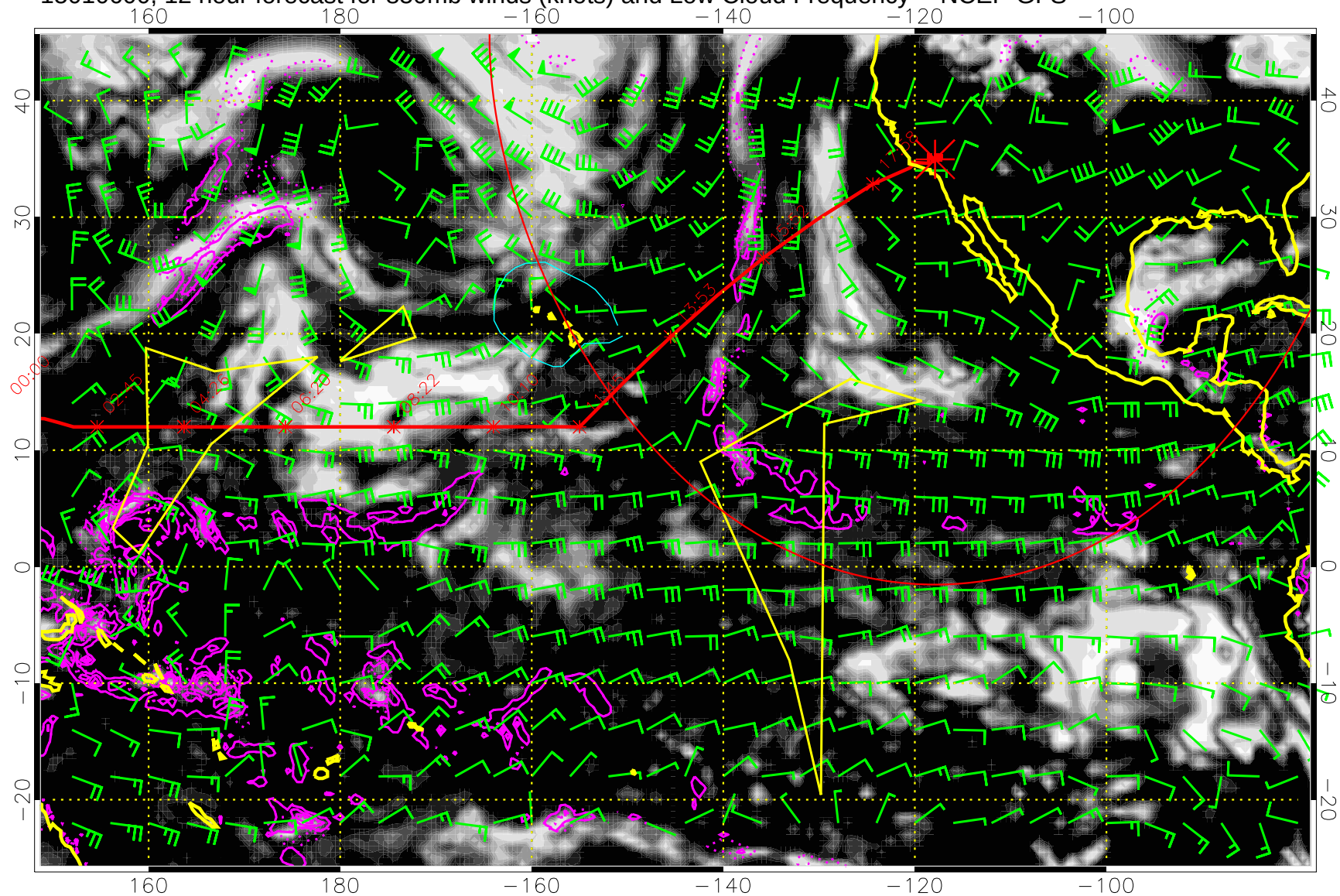
15010600, 12 hour forecast for 850mb winds (knots) and Low Cloud Frequency -- NCEP GFS
