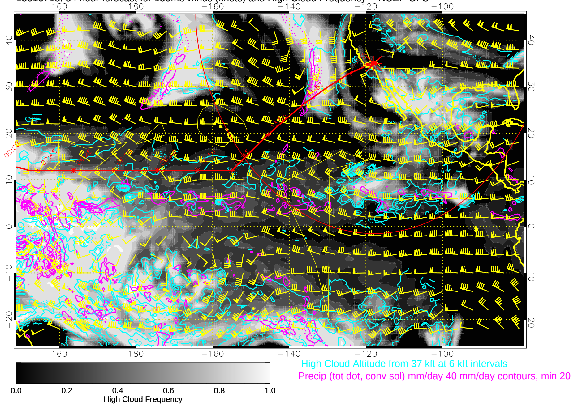
15010718, 54 hour forecast for 150mb winds (knots) and High Cloud Frequency -- NCEP GFS
