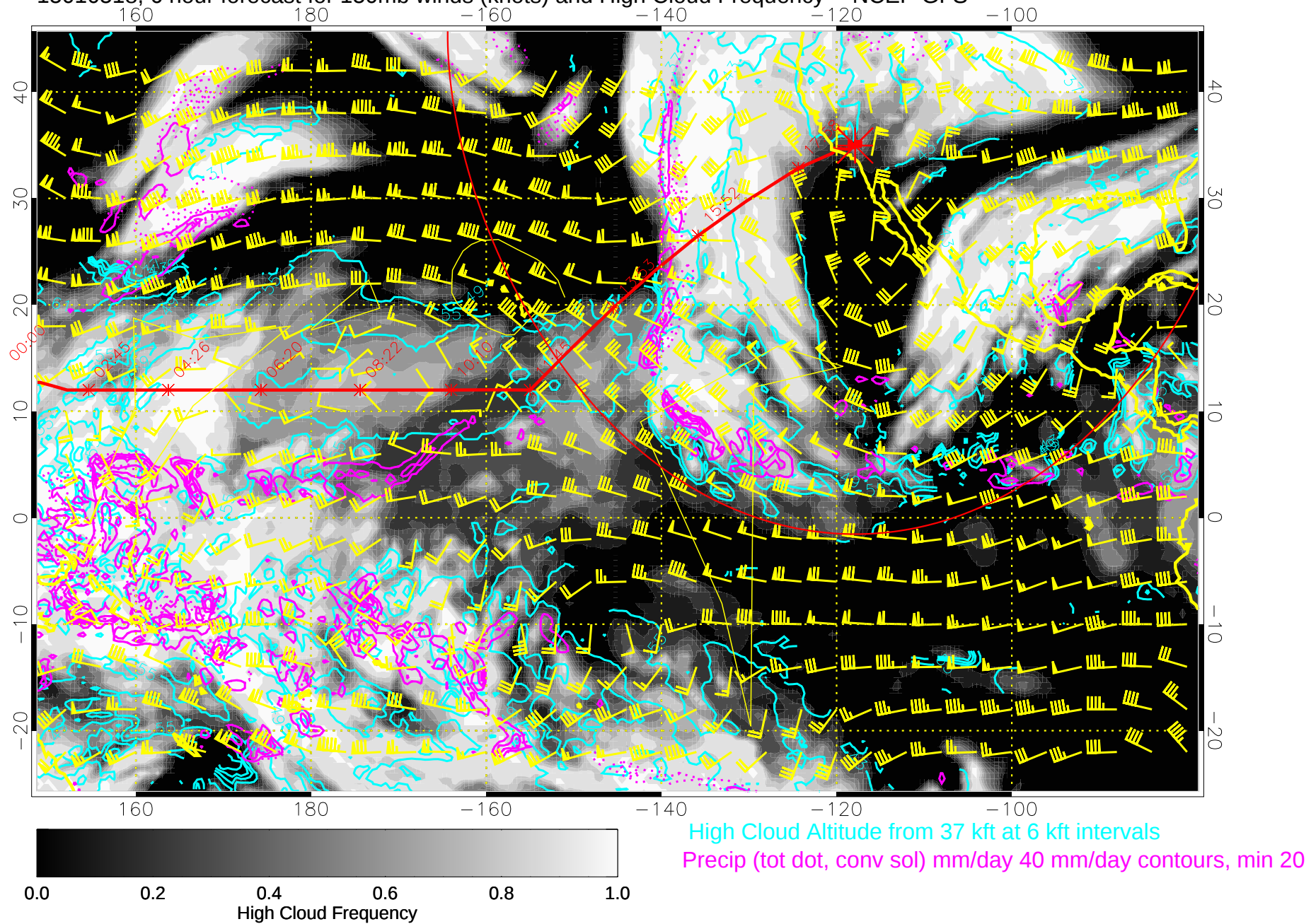
15010518, 6 hour forecast for 150mb winds (knots) and High Cloud Frequency -- NCEP GFS
