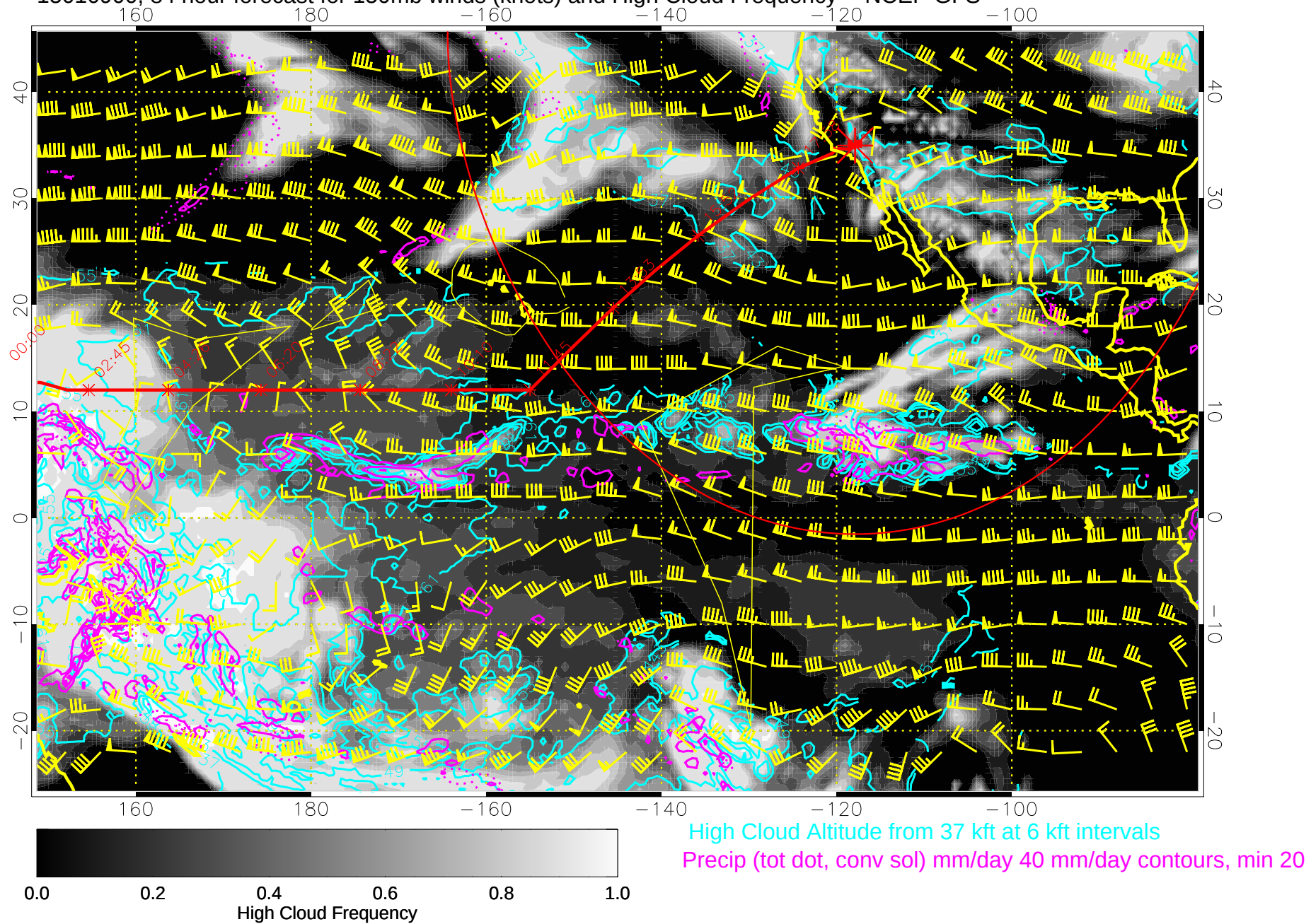
15010900, 84 hour forecast for 150mb winds (knots) and High Cloud Frequency -- NCEP GFS
