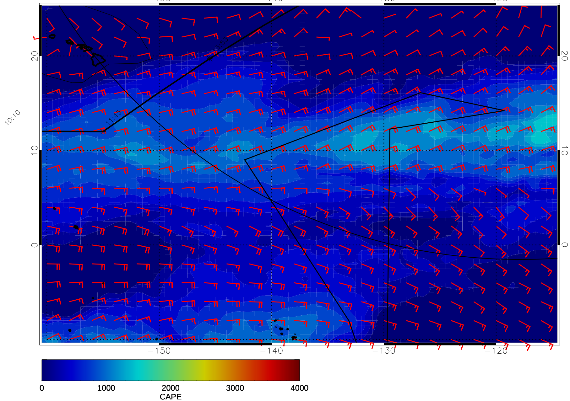
15011000, 108 hour forecast for CAPE and surface winds (knots) -- NCEP GFS
