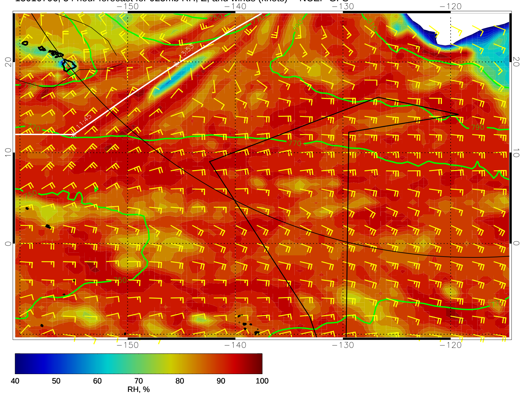
15010706, 54 hour forecast for 925mb RH, Z, and winds (knots) -- NCEP GFS
