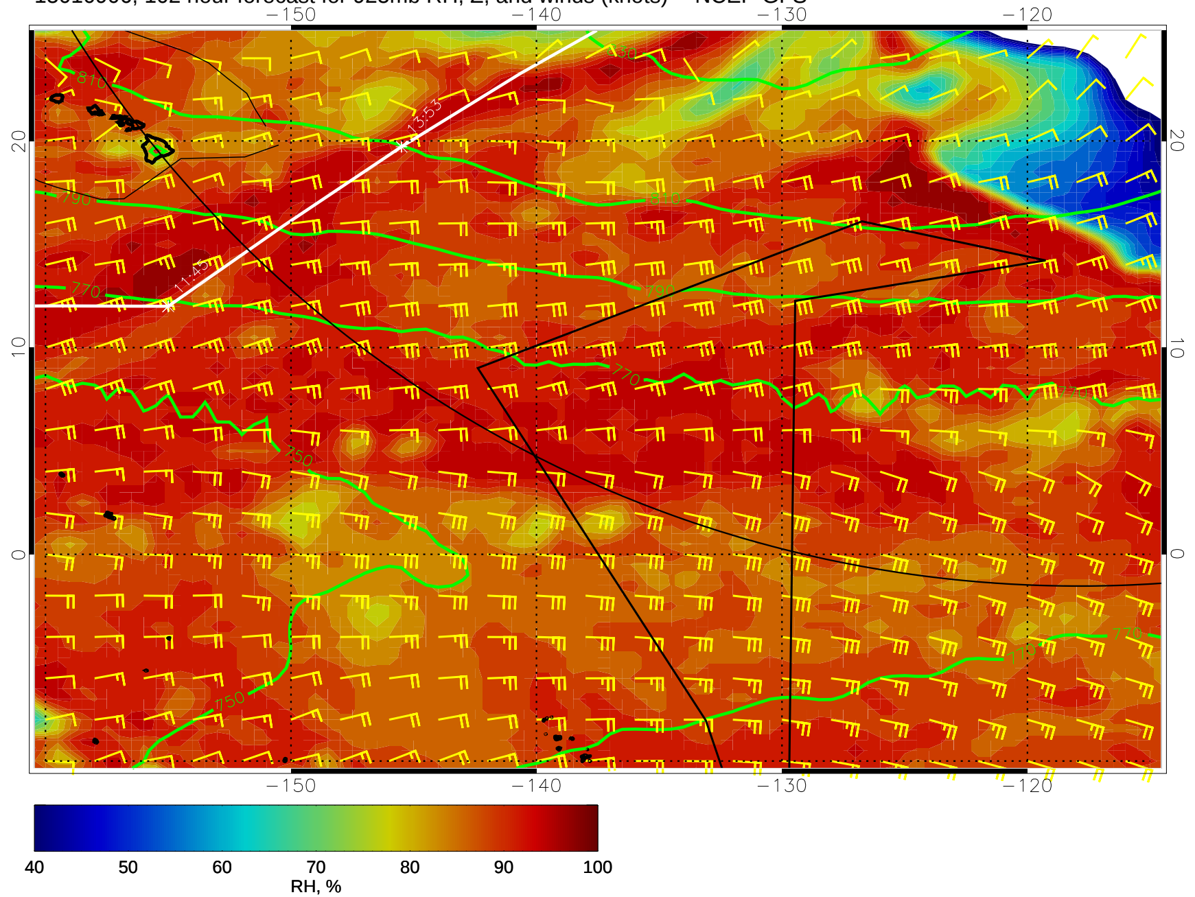
15010906, 102 hour forecast for 925mb RH, Z, and winds (knots) -- NCEP GFS
