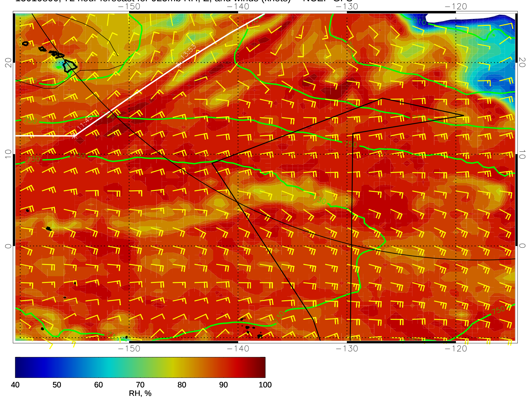
15010800, 72 hour forecast for 925mb RH, Z, and winds (knots) -- NCEP GFS
