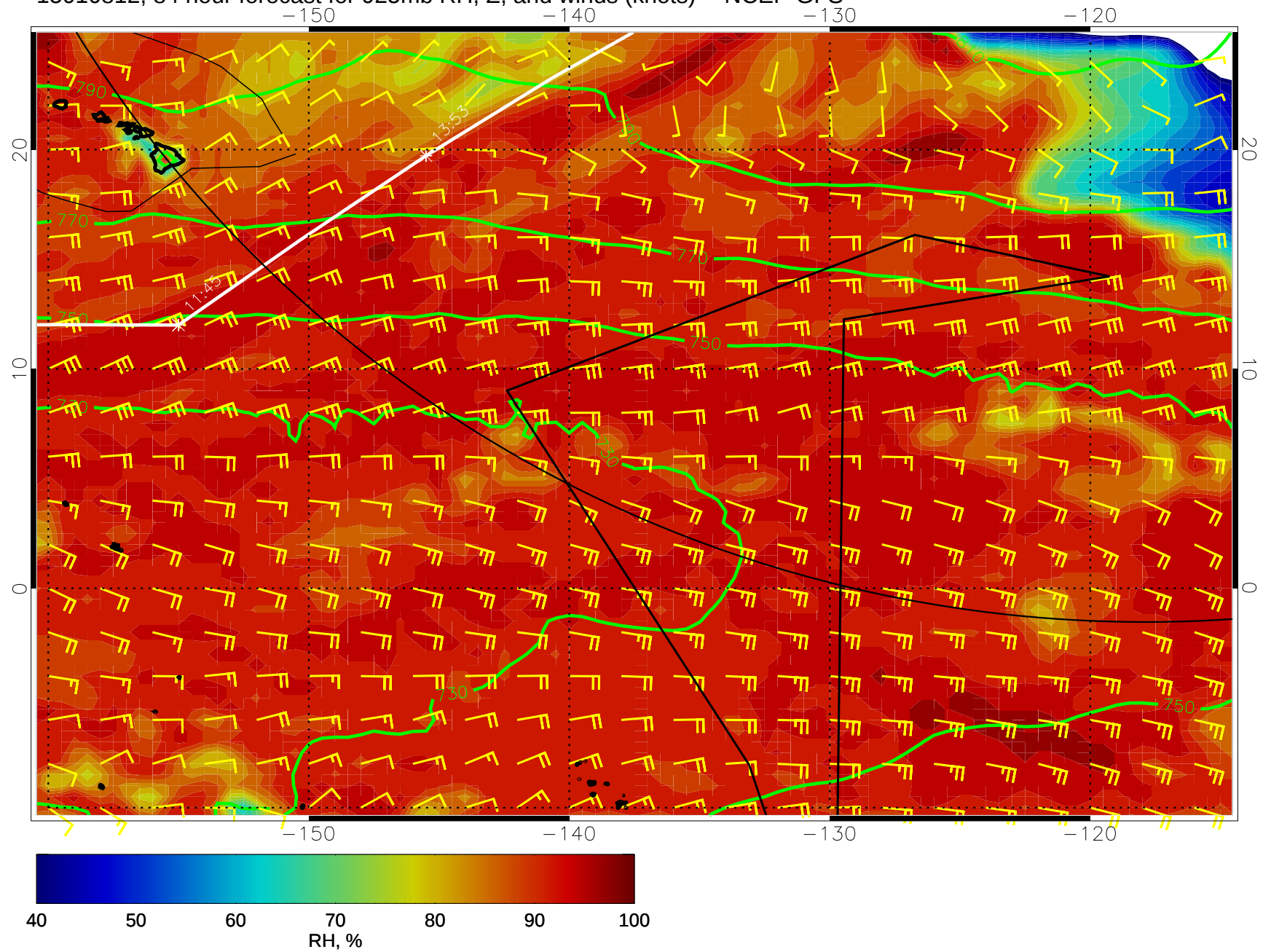
15010812, 84 hour forecast for 925mb RH, Z, and winds (knots) -- NCEP GFS
