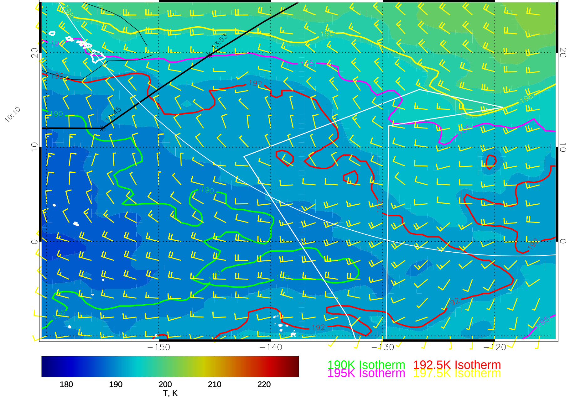
15011000, 120 hour forecast for 70mb T and winds (knots) -- NCEP GFS
