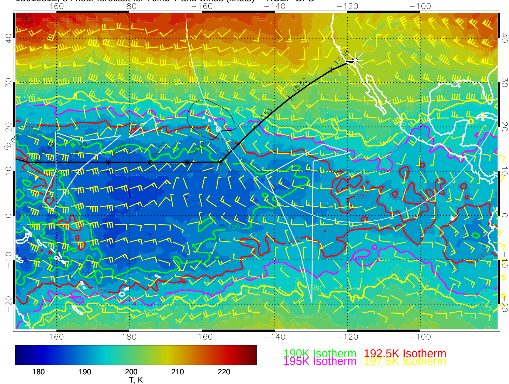
15010812, 84 hour forecast for 70mb T and winds (knots) -- NCEP GFS
