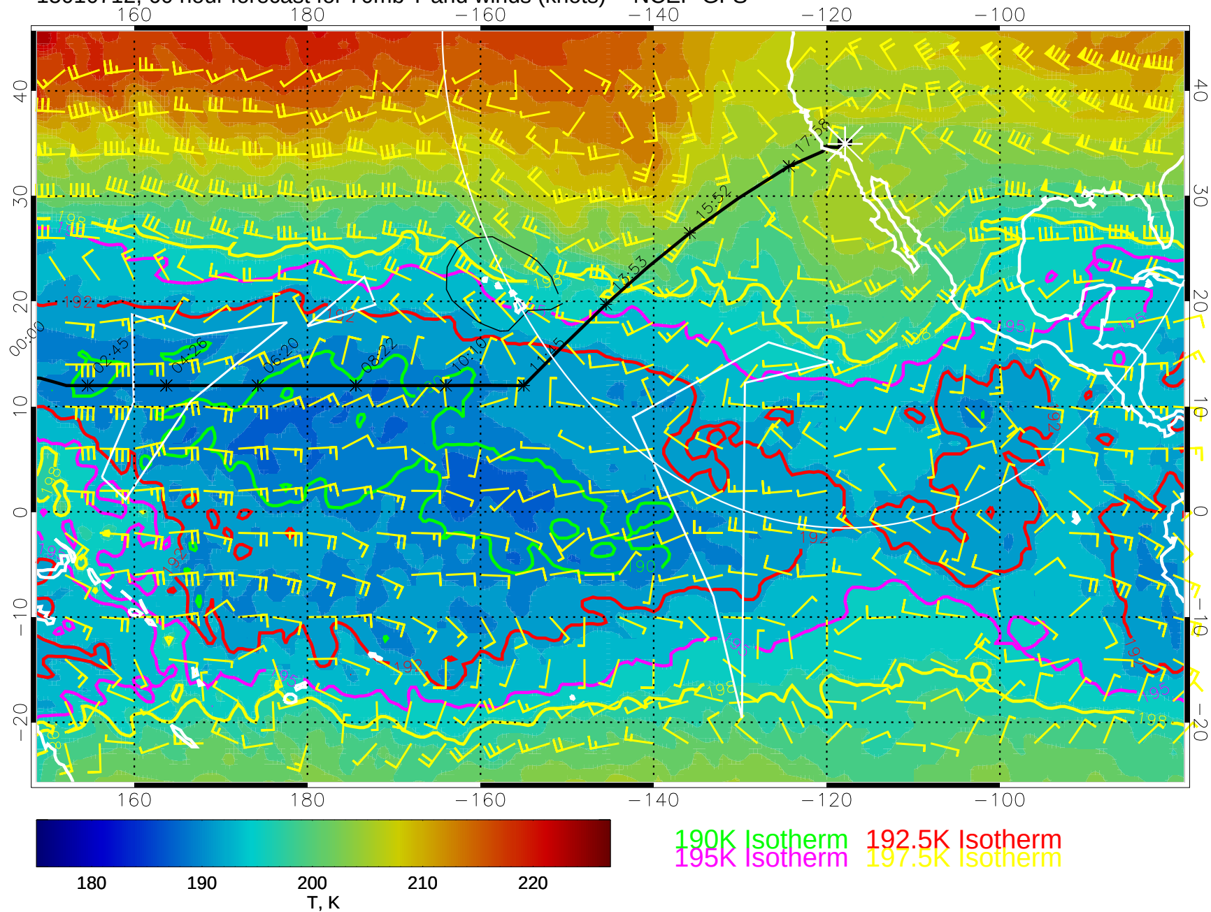
15010712, 60 hour forecast for 70mb T and winds (knots) -- NCEP GFS
