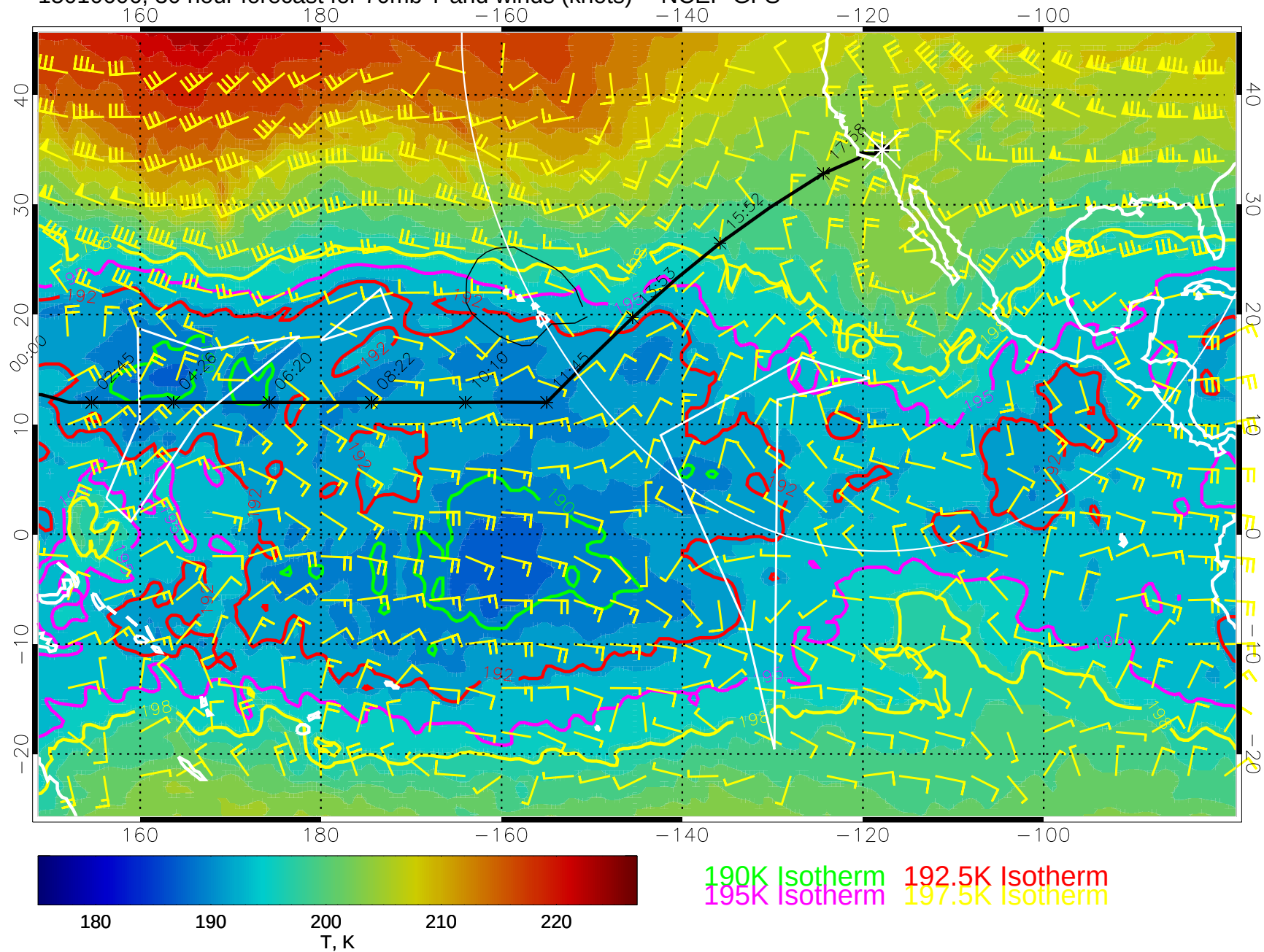
15010606, 30 hour forecast for 70mb T and winds (knots) -- NCEP GFS
