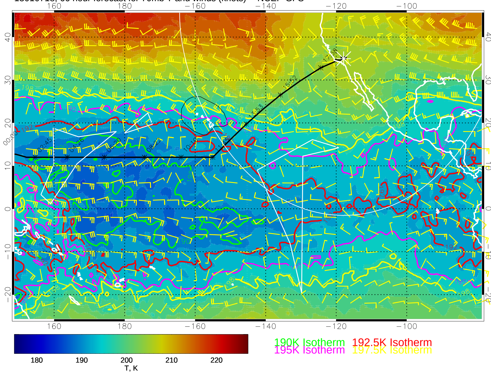
15010718, 66 hour forecast for 70mb T and winds (knots) -- NCEP GFS
