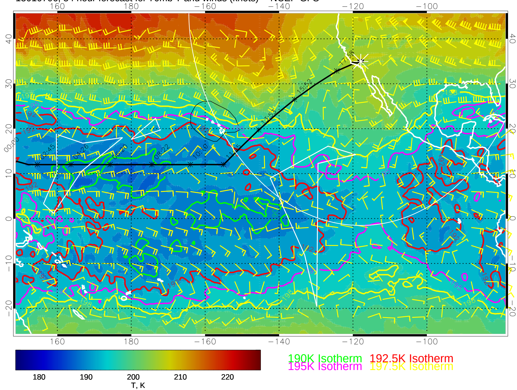
15010706, 54 hour forecast for 70mb T and winds (knots) -- NCEP GFS
