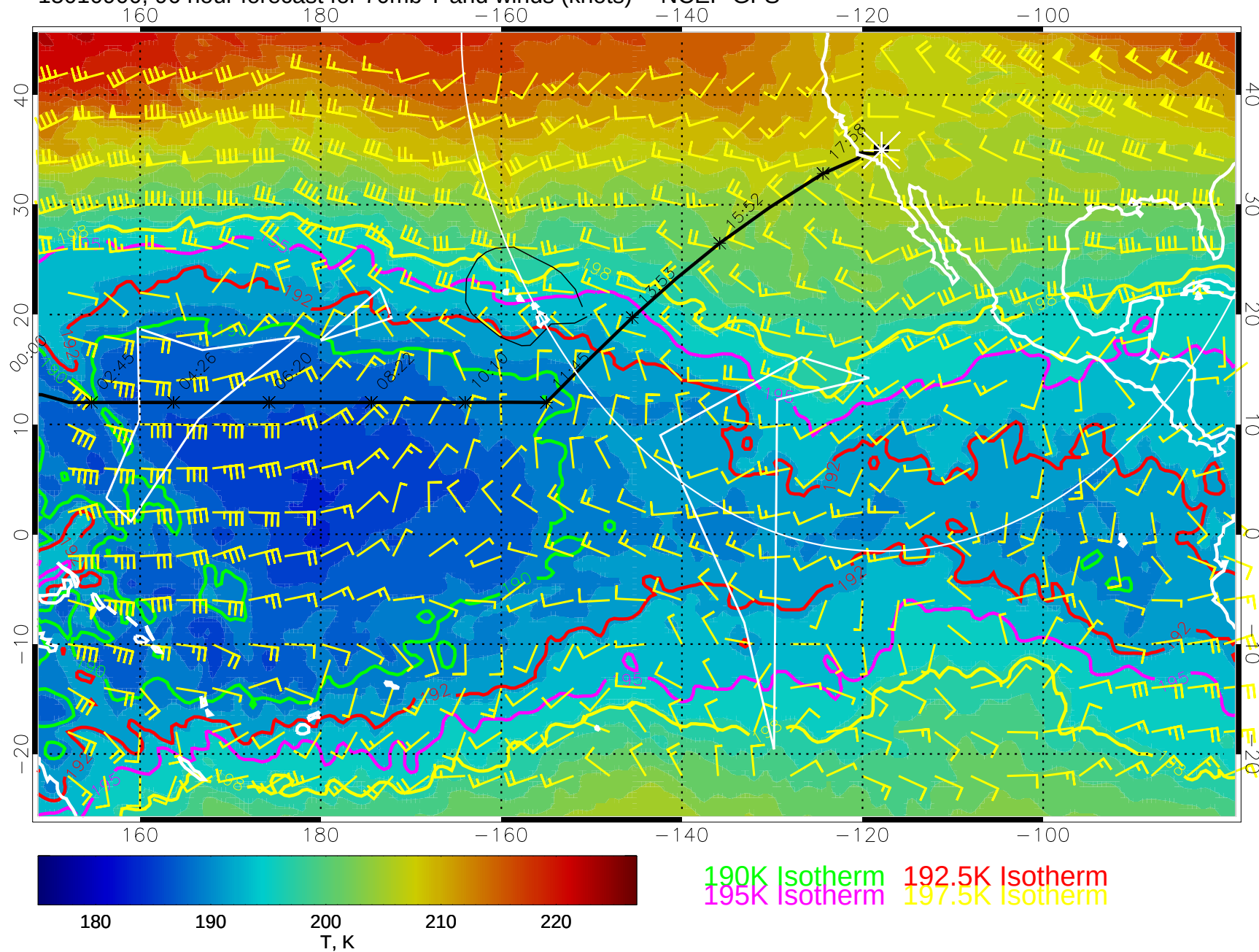
15010900, 96 hour forecast for 70mb T and winds (knots) -- NCEP GFS
