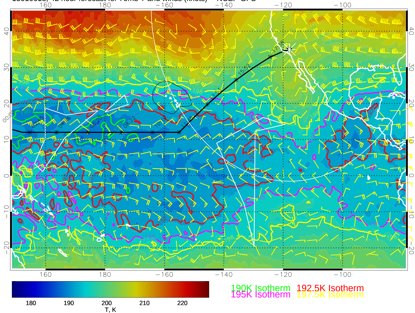
15010618, 42 hour forecast for 70mb T and winds (knots) -- NCEP GFS
