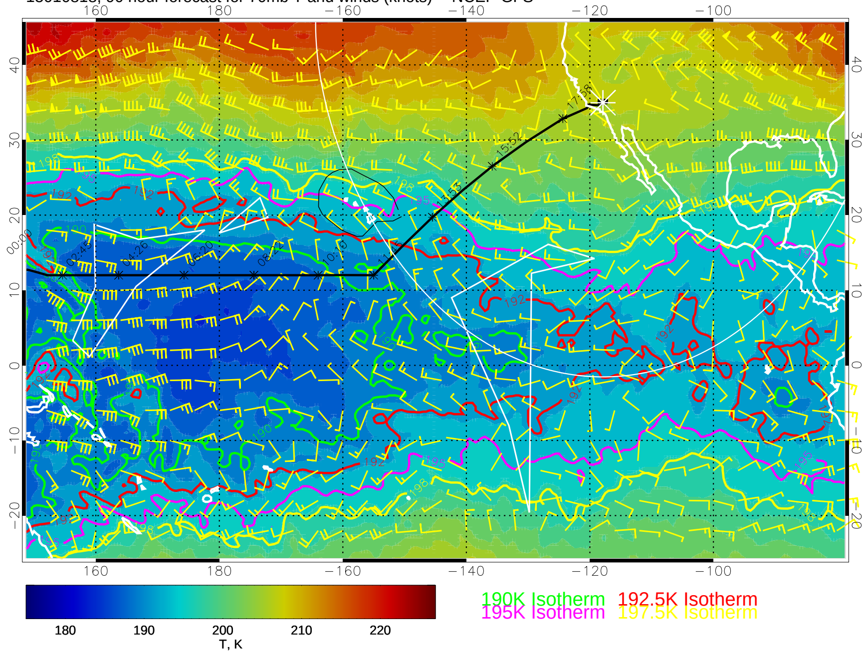
15010818, 90 hour forecast for 70mb T and winds (knots) -- NCEP GFS
