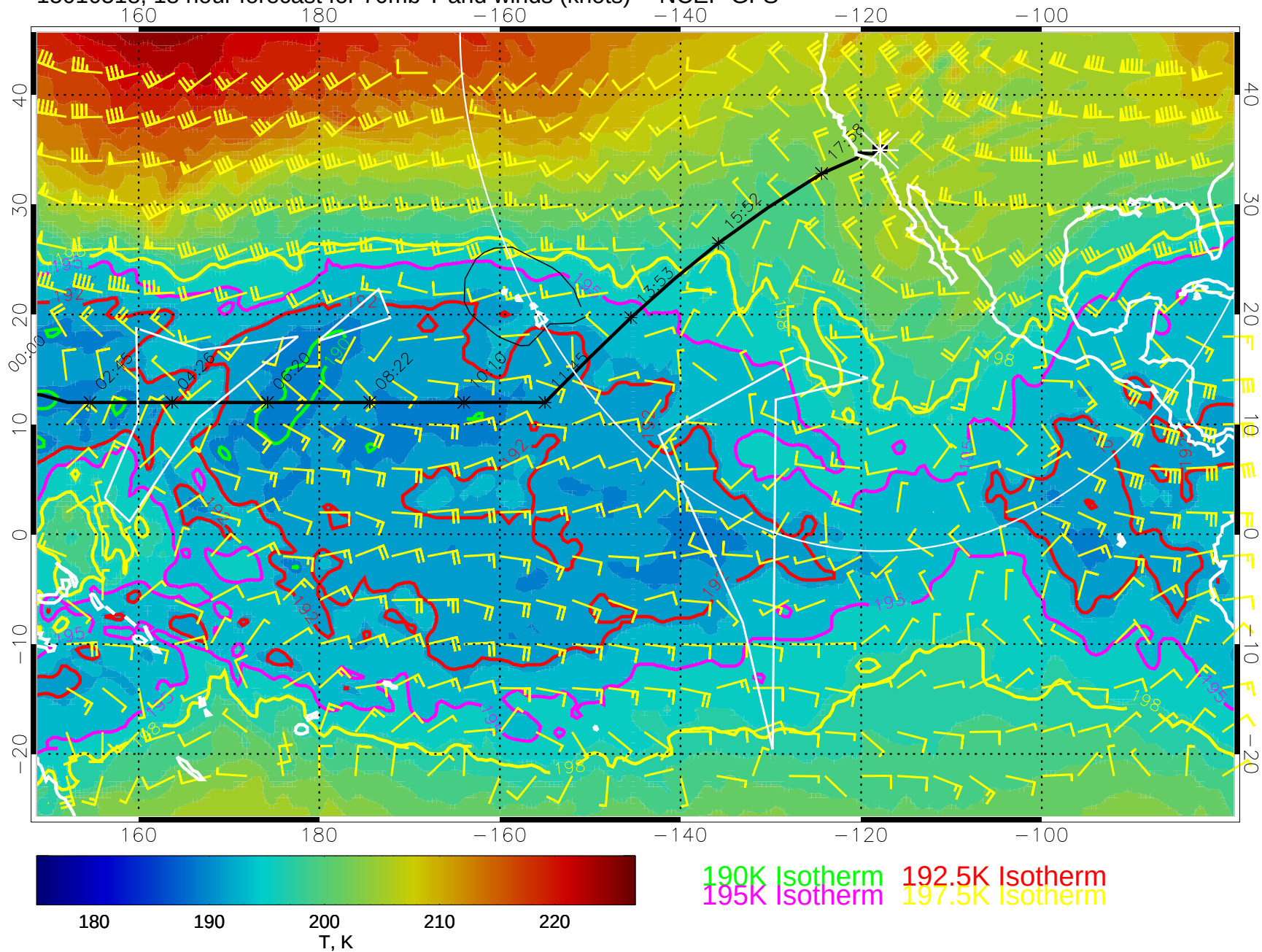
15010518, 18 hour forecast for 70mb T and winds (knots) -- NCEP GFS
