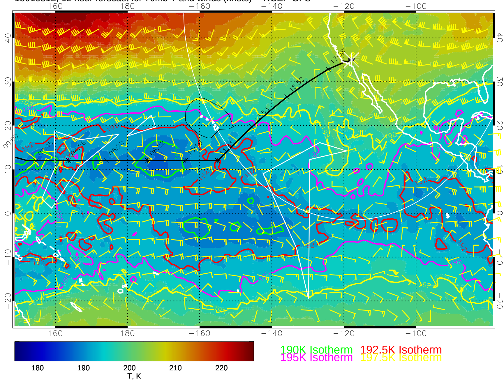
15010512, 12 hour forecast for 70mb T and winds (knots) -- NCEP GFS
