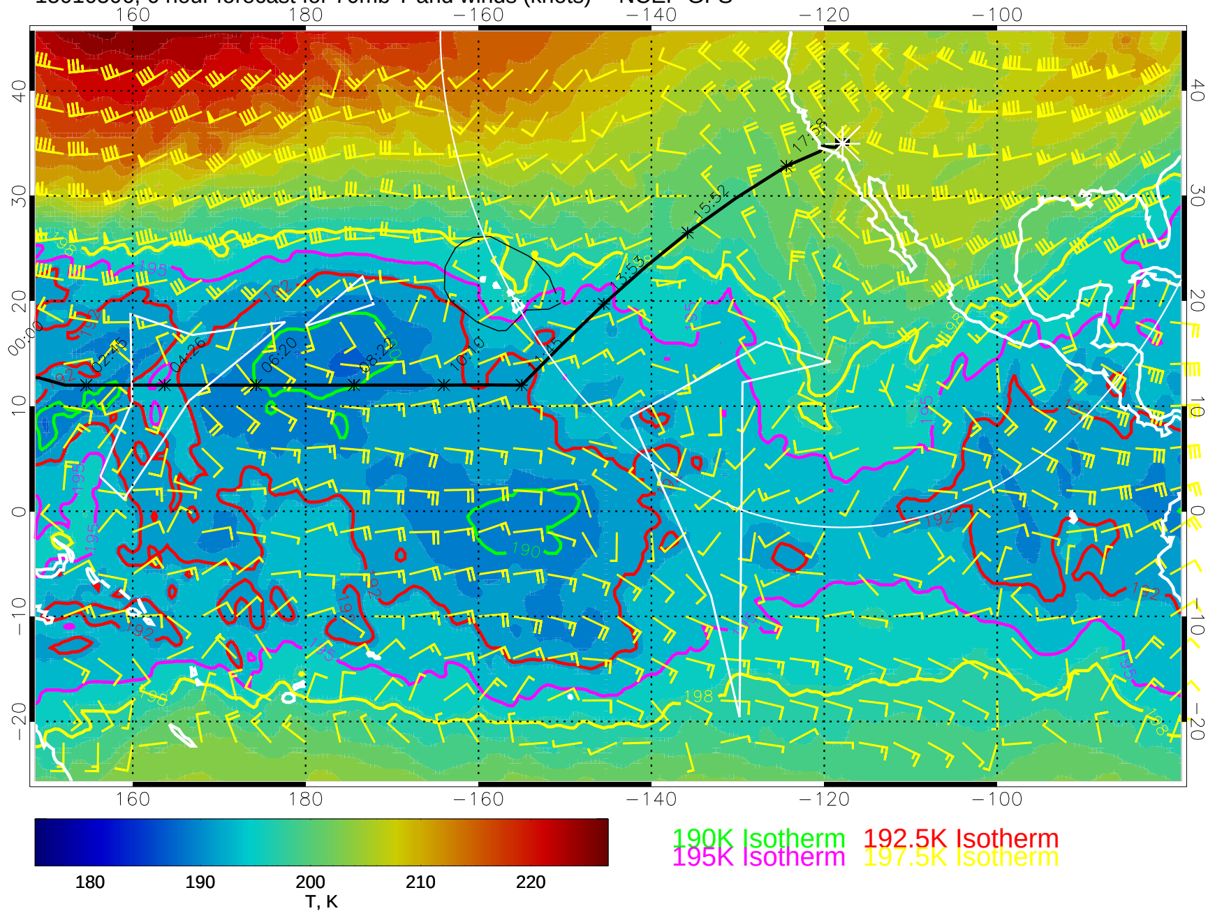
15010506, 6 hour forecast for 70mb T and winds (knots) -- NCEP GFS
