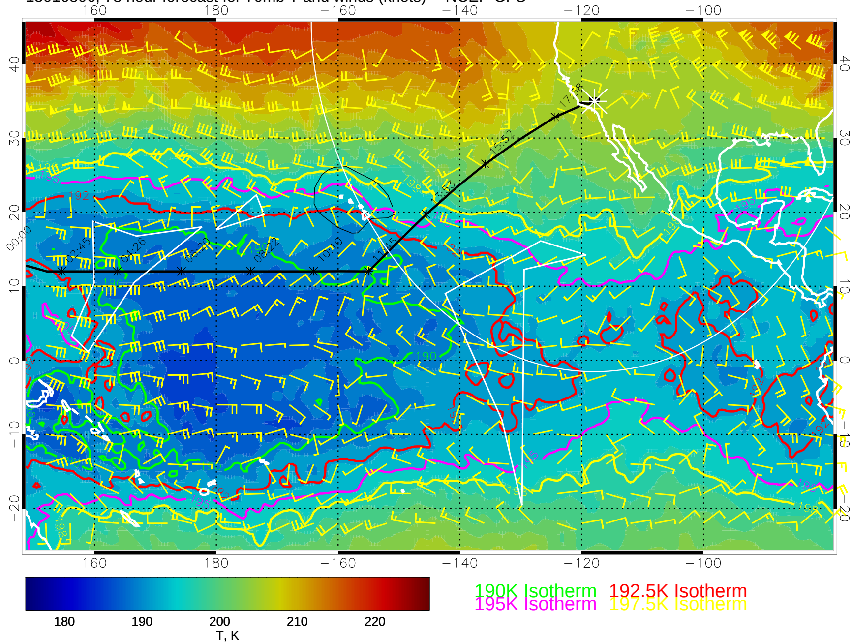
15010806, 78 hour forecast for 70mb T and winds (knots) -- NCEP GFS
