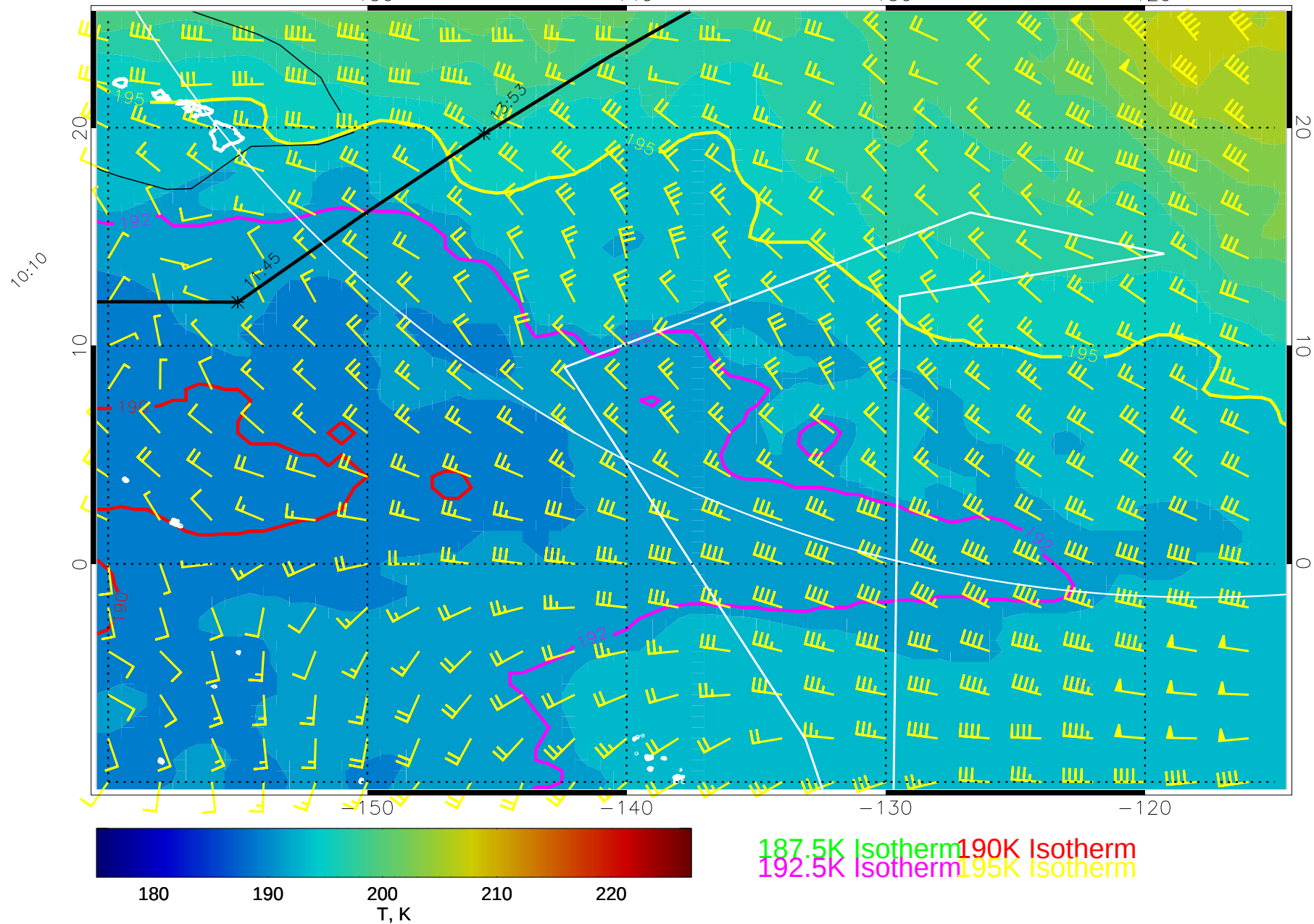
15010506, 6 hour forecast for 100mb T and winds (knots) -- NCEP GFS
