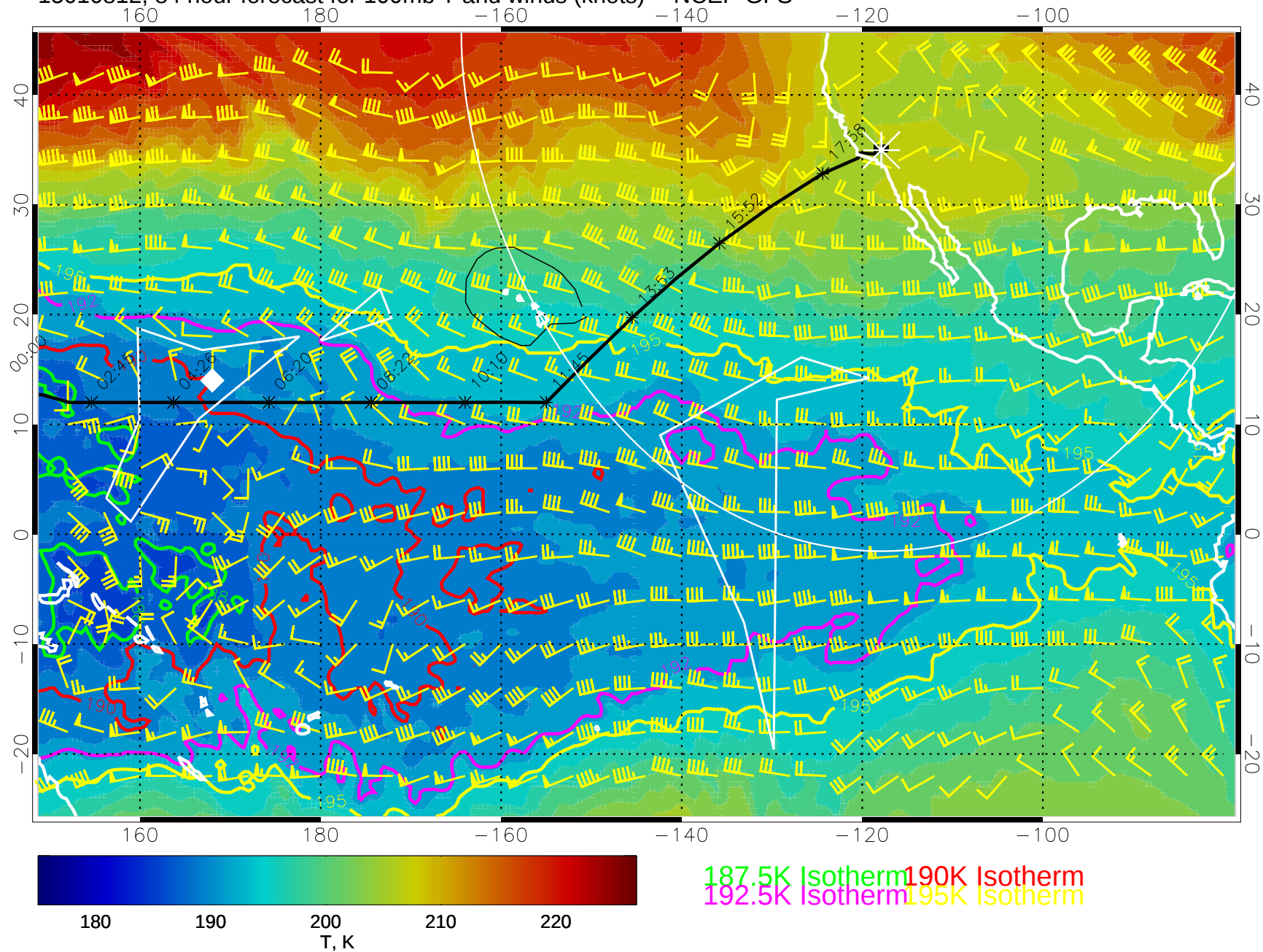
15010812, 84 hour forecast for 100mb T and winds (knots) -- NCEP GFS
