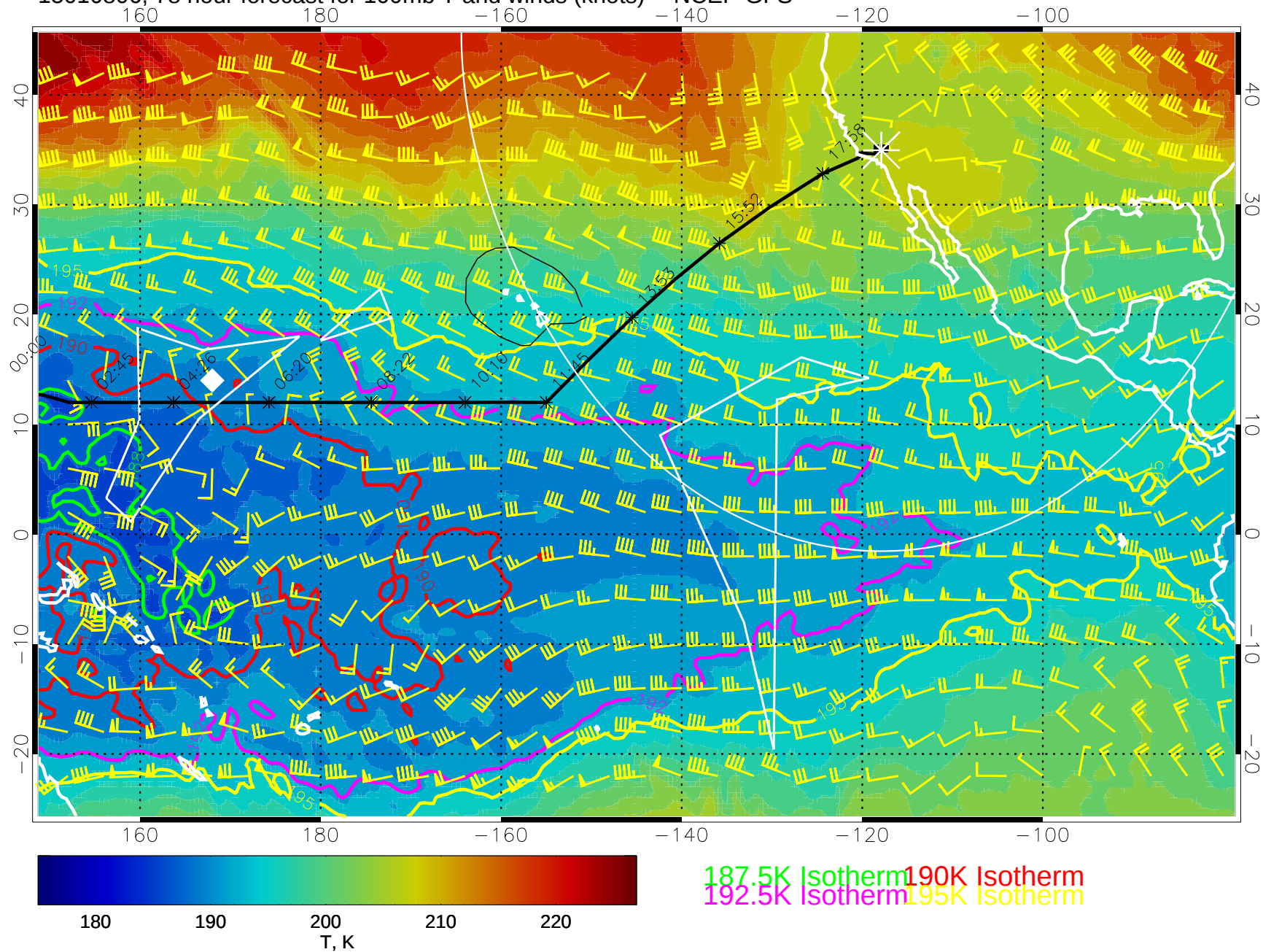
15010806, 78 hour forecast for 100mb T and winds (knots) -- NCEP GFS
