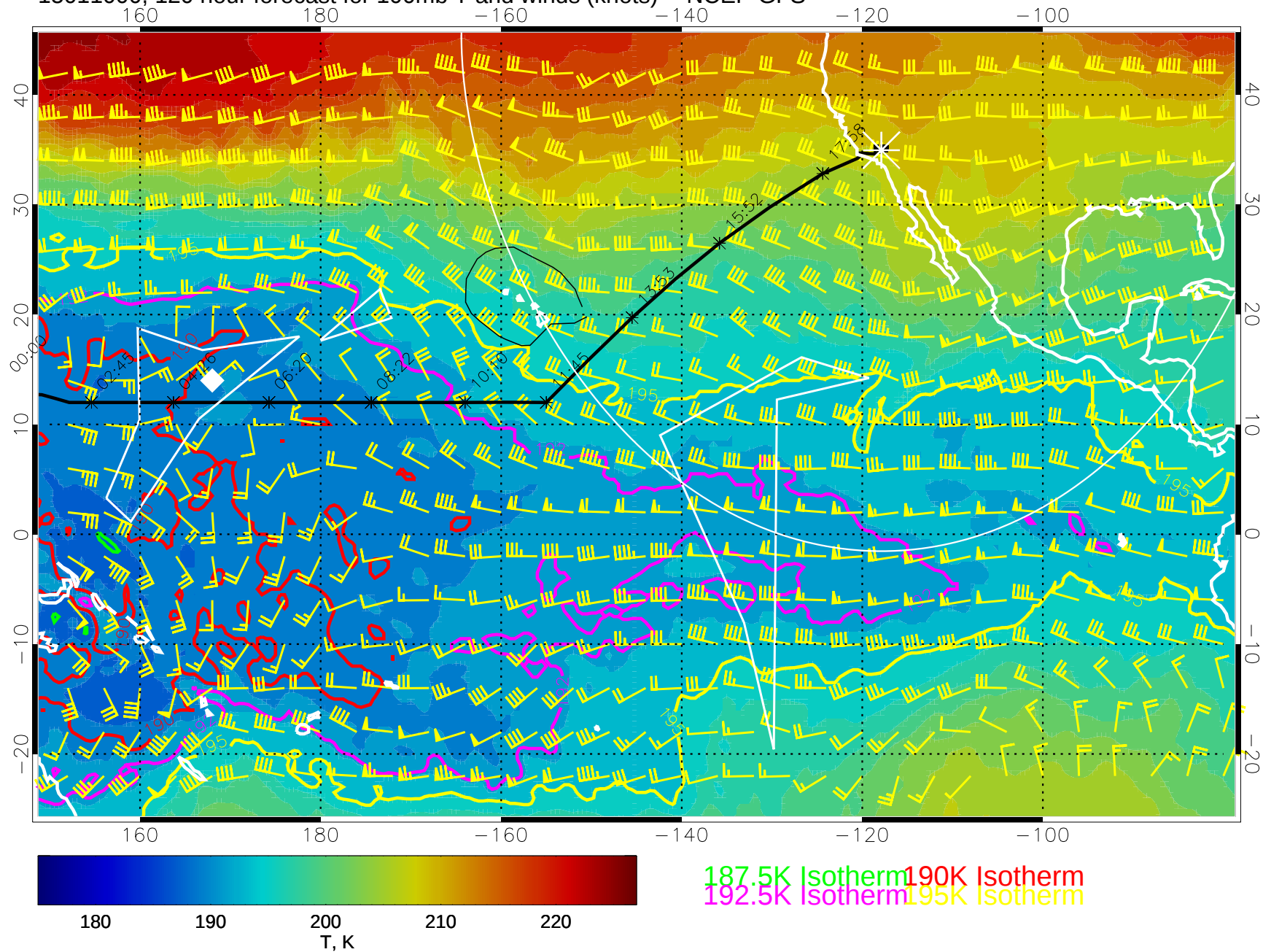
15011000, 120 hour forecast for 100mb T and winds (knots) -- NCEP GFS
