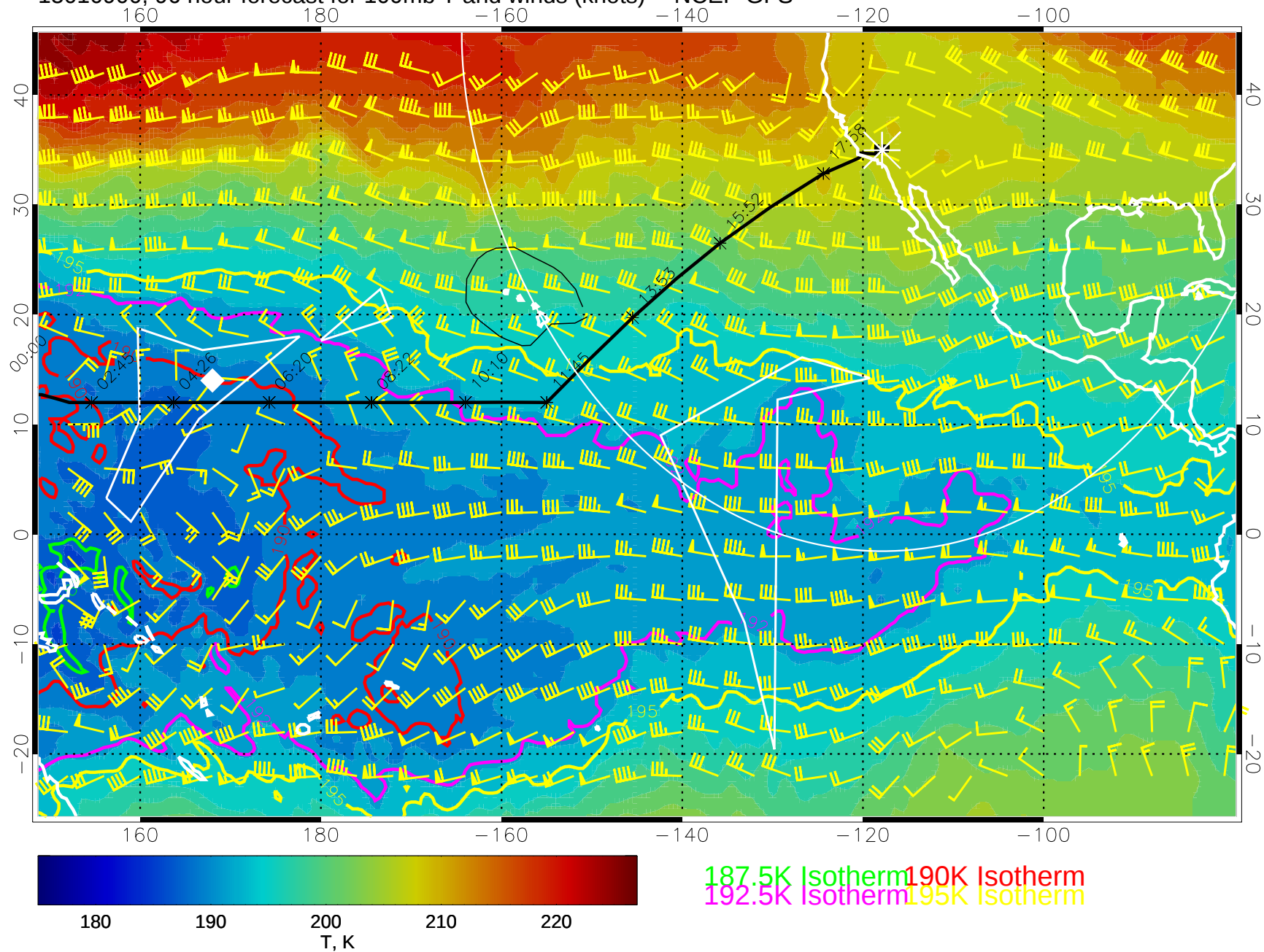
15010900, 96 hour forecast for 100mb T and winds (knots) -- NCEP GFS
