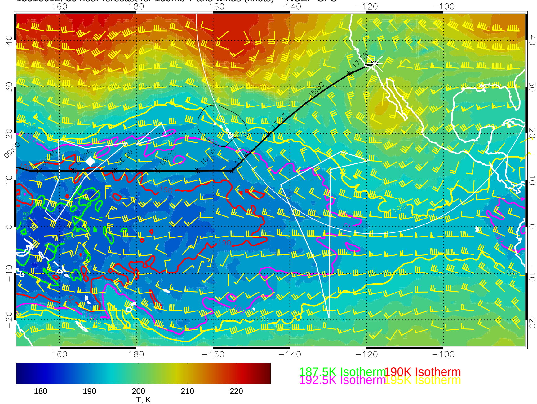
15010612, 36 hour forecast for 100mb T and winds (knots) -- NCEP GFS
