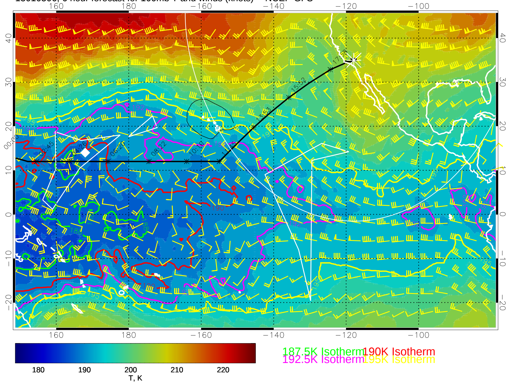
15010506, 6 hour forecast for 100mb T and winds (knots) -- NCEP GFS
