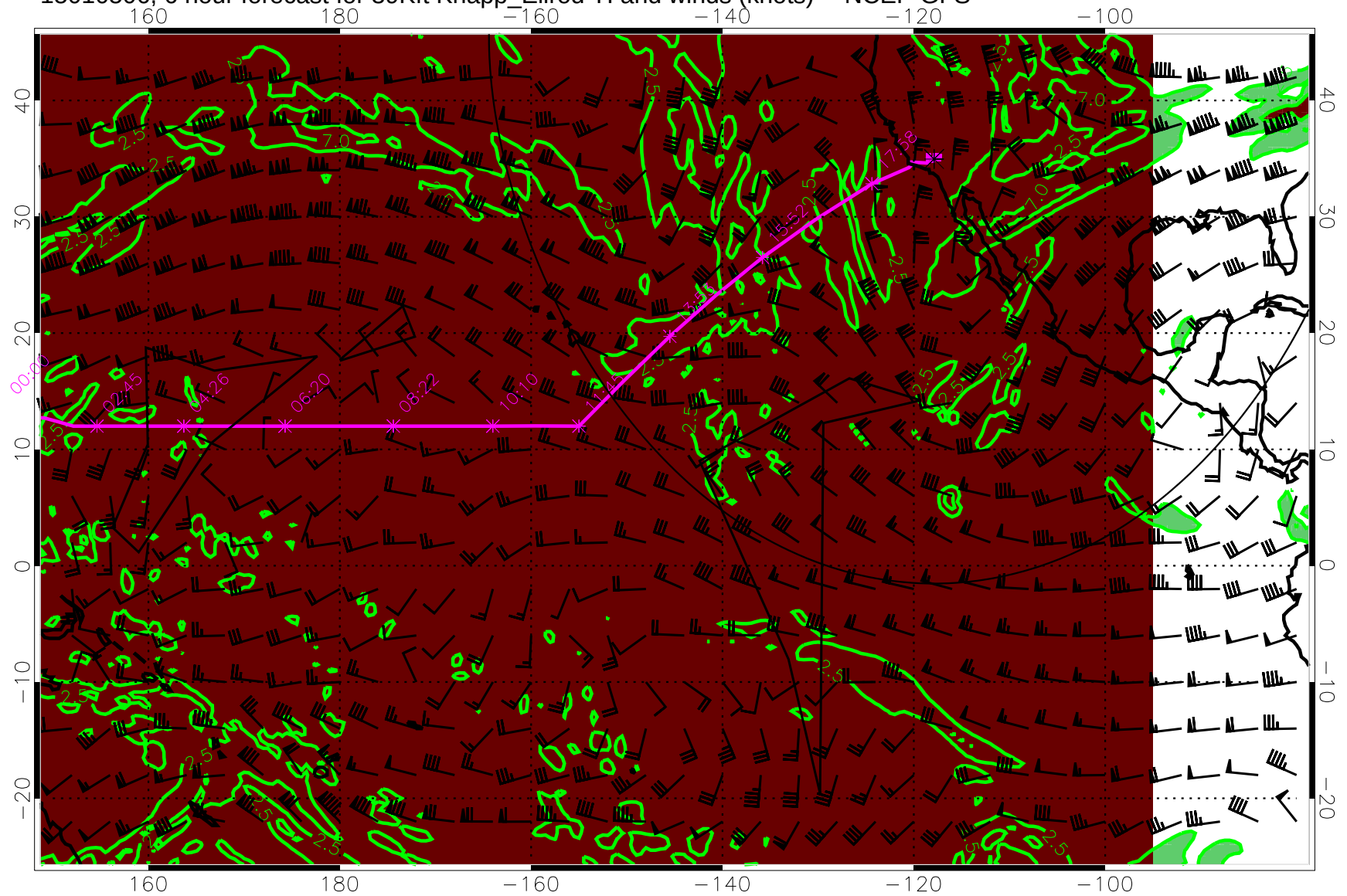
15010506, 6 hour forecast for 39Kft Knapp_Ellrod TI and winds (knots) -- NCEP GFS
