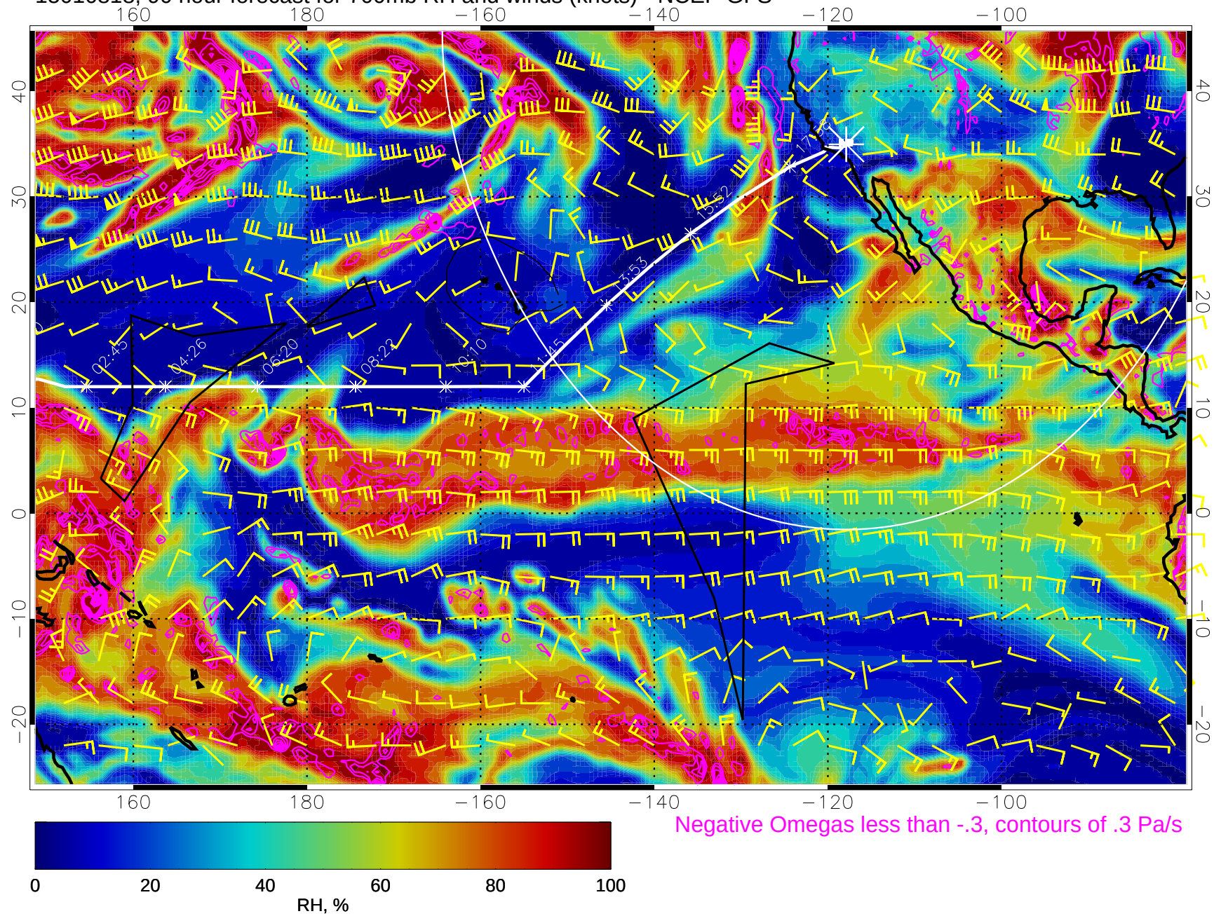
15010818, 90 hour forecast for 700mb RH and winds (knots) - NCEP GFS
