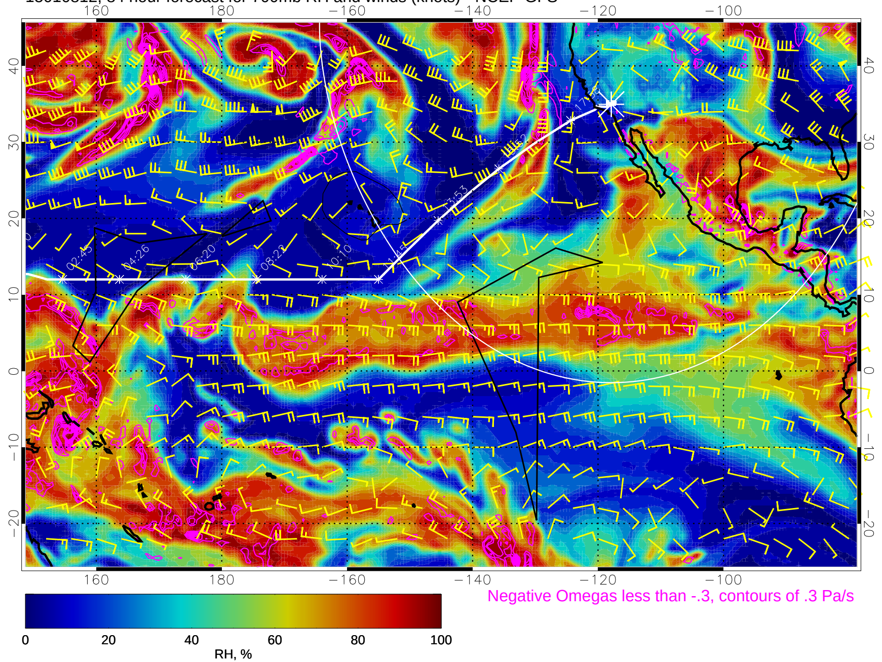
15010812, 84 hour forecast for 700mb RH and winds (knots) - NCEP GFS
