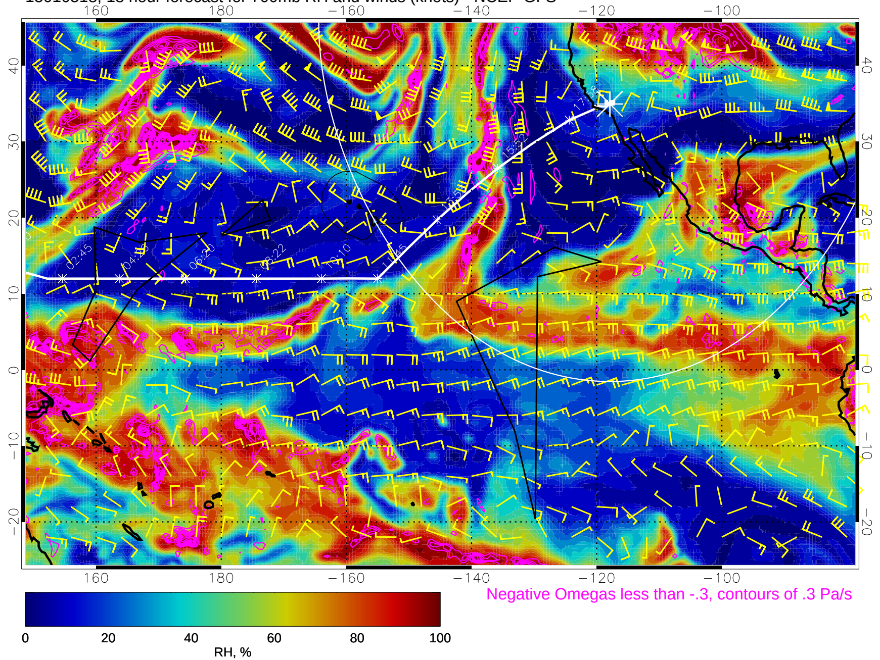
15010518, 18 hour forecast for 700mb RH and winds (knots) - NCEP GFS
