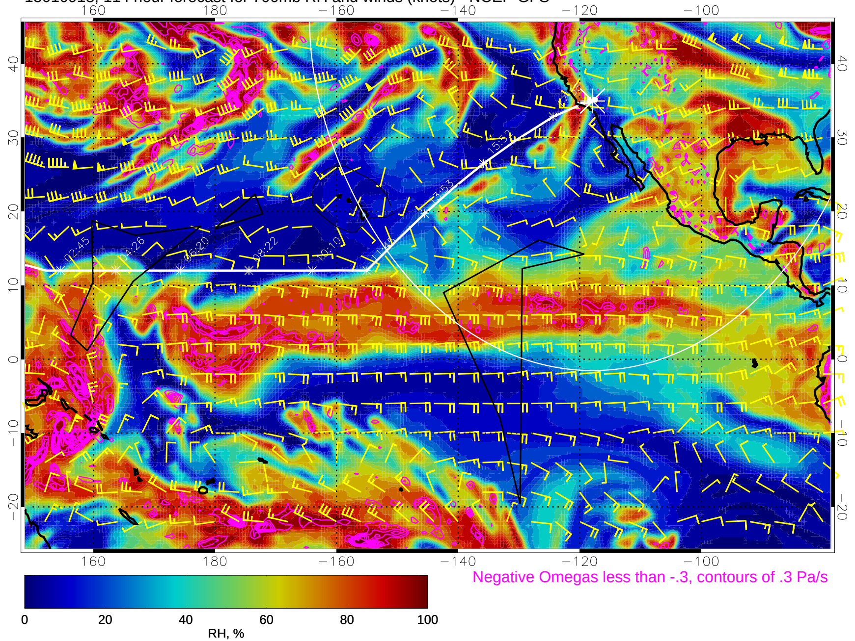
15010918, 114 hour forecast for 700mb RH and winds (knots) - NCEP GFS
