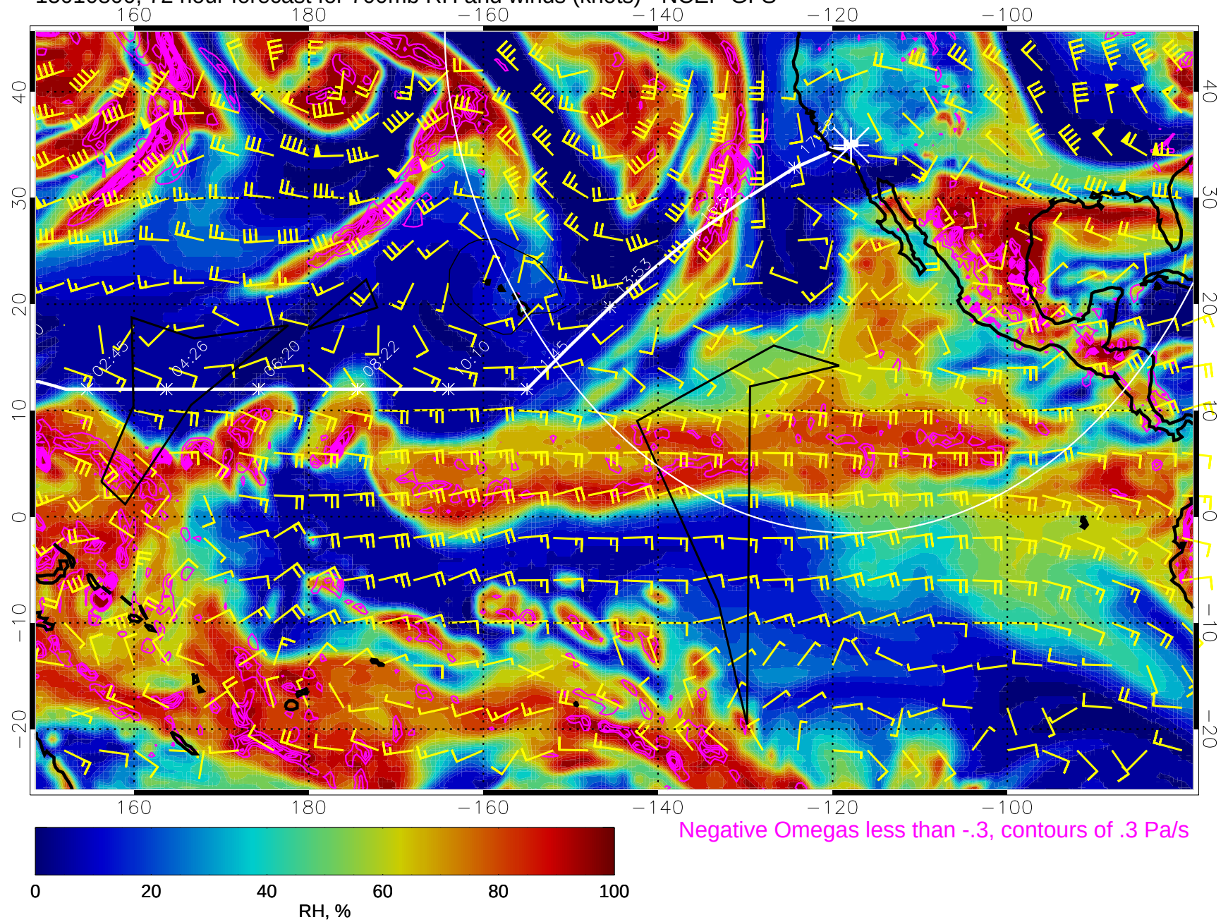
15010800, 72 hour forecast for 700mb RH and winds (knots) - NCEP GFS
