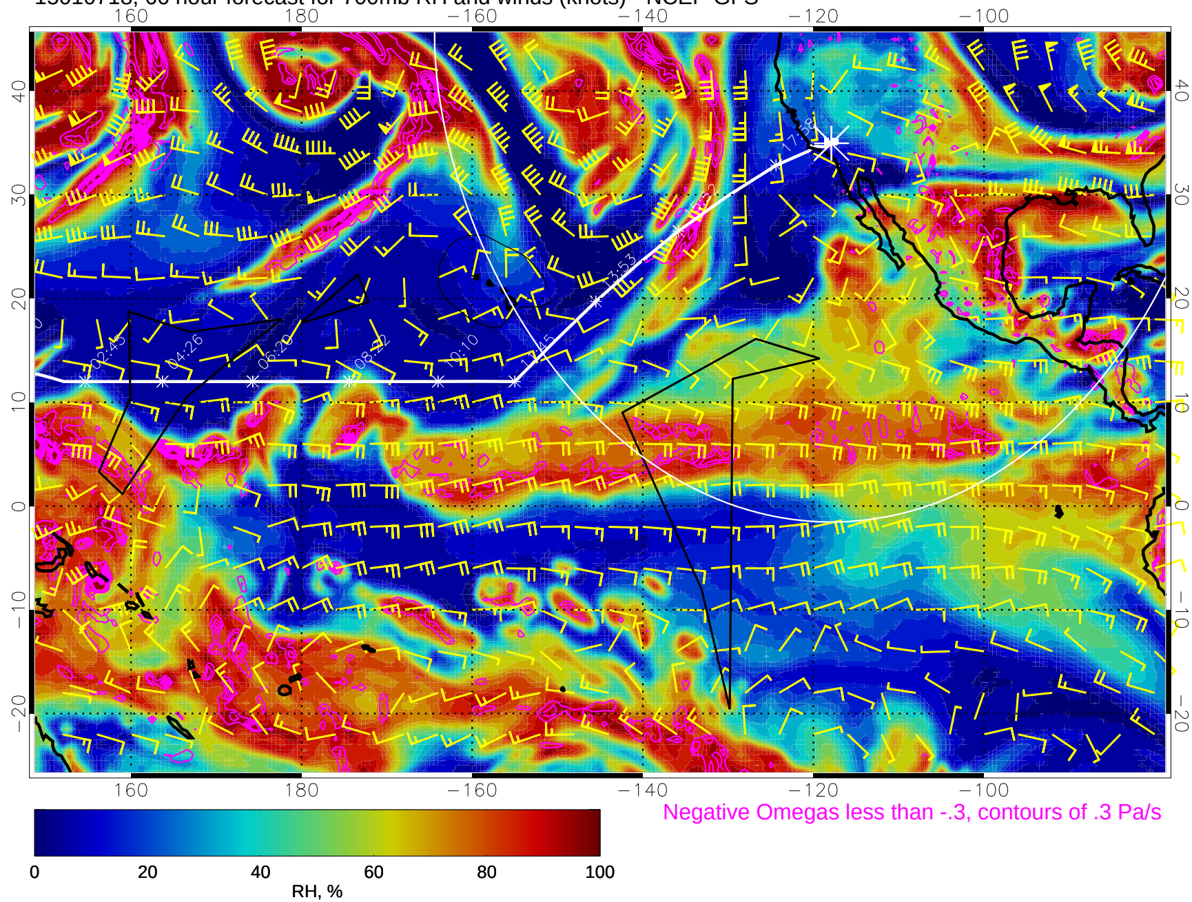
15010718, 66 hour forecast for 700mb RH and winds (knots) - NCEP GFS
