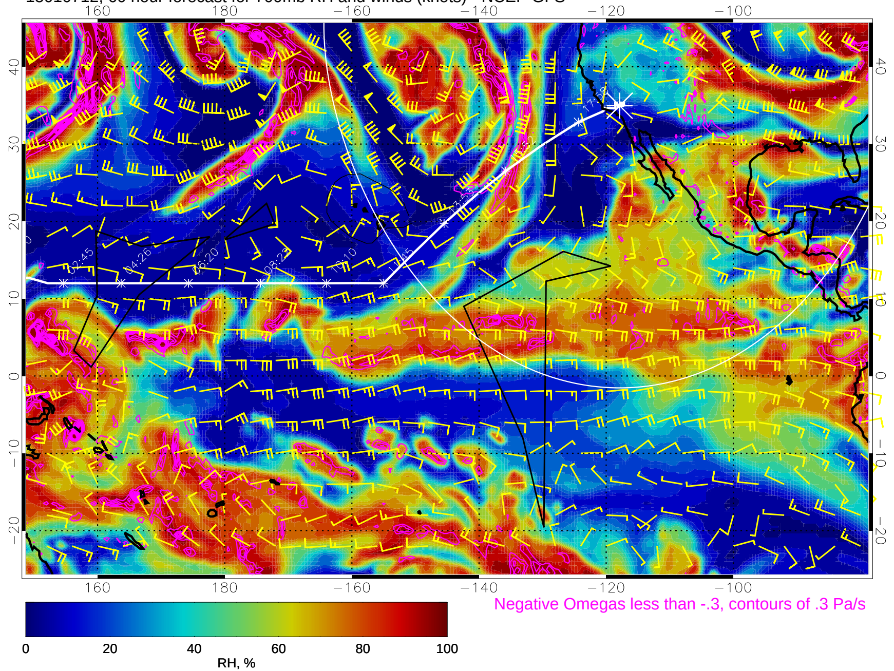
15010712, 60 hour forecast for 700mb RH and winds (knots) - NCEP GFS
