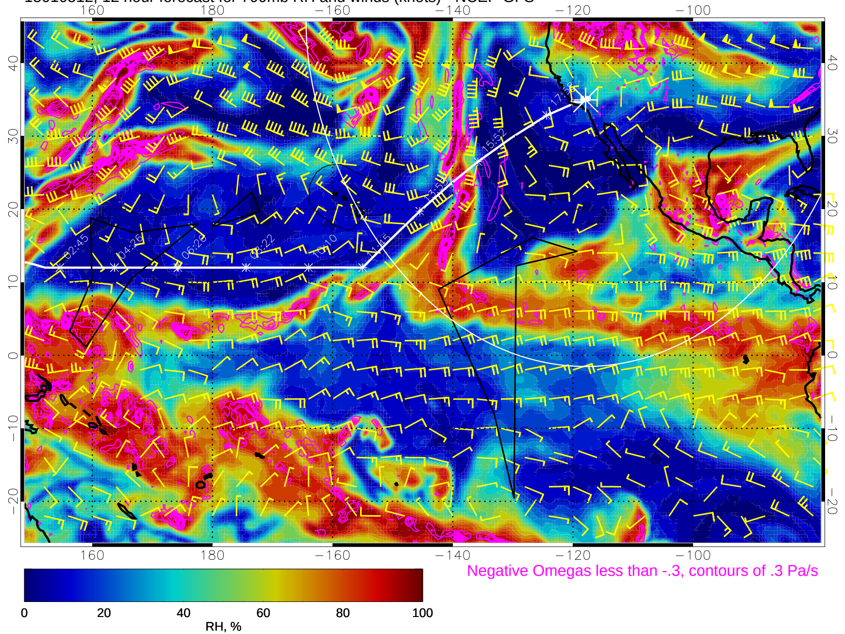
15010512, 12 hour forecast for 700mb RH and winds (knots) - NCEP GFS
