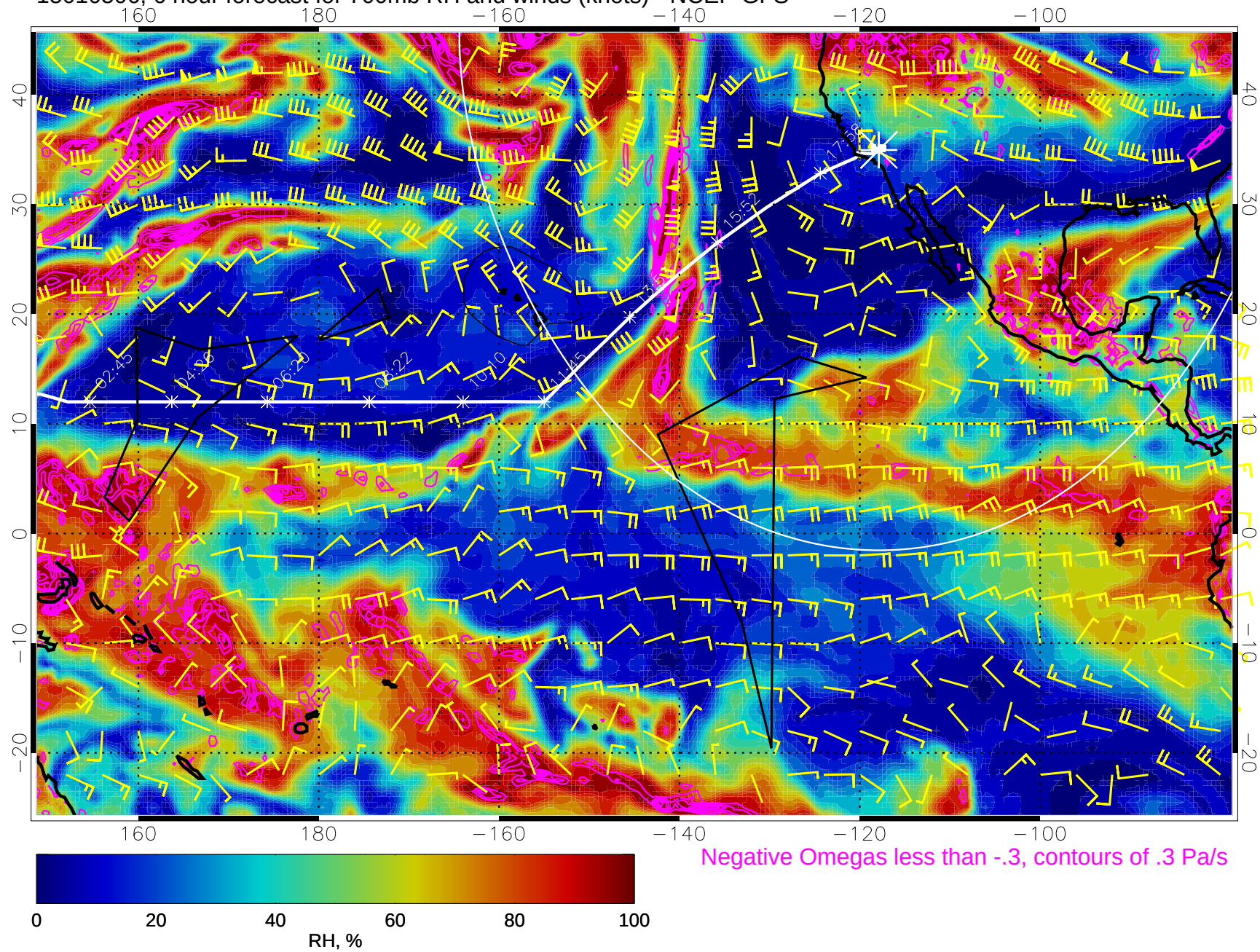
15010506, 6 hour forecast for 700mb RH and winds (knots) - NCEP GFS
