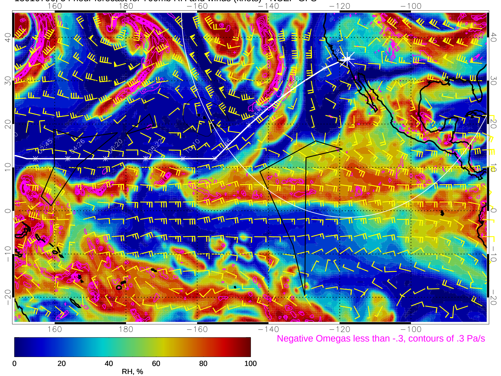
15010706, 54 hour forecast for 700mb RH and winds (knots) - NCEP GFS
