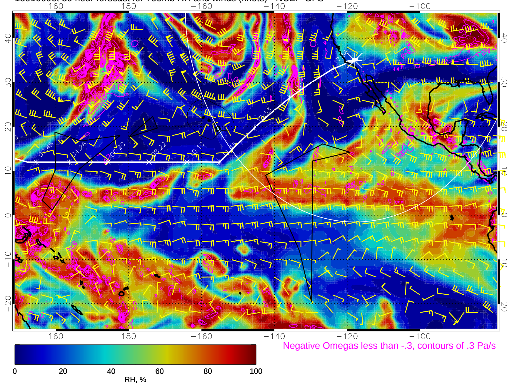
15010606, 30 hour forecast for 700mb RH and winds (knots) - NCEP GFS
