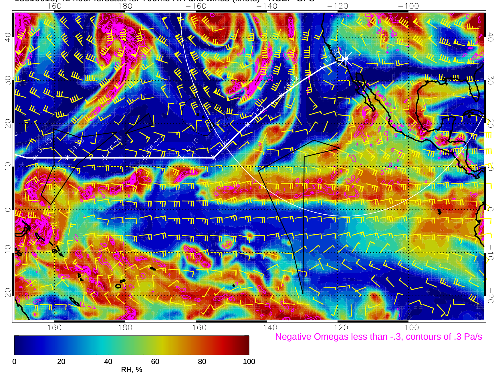
15010618, 42 hour forecast for 700mb RH and winds (knots) - NCEP GFS
