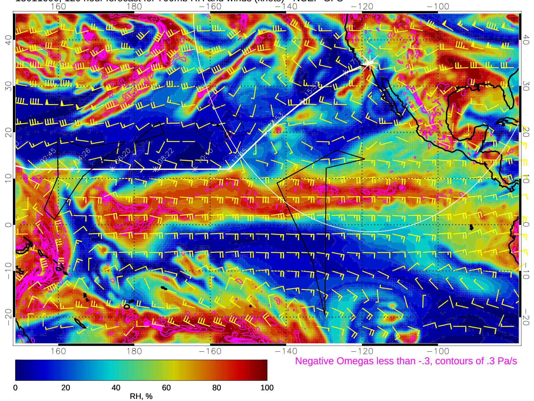
15011000, 120 hour forecast for 700mb RH and winds (knots) - NCEP GFS
