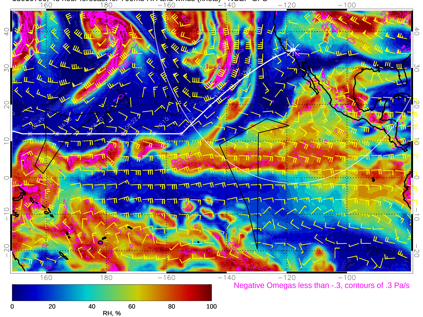
15010700, 48 hour forecast for 700mb RH and winds (knots) - NCEP GFS
