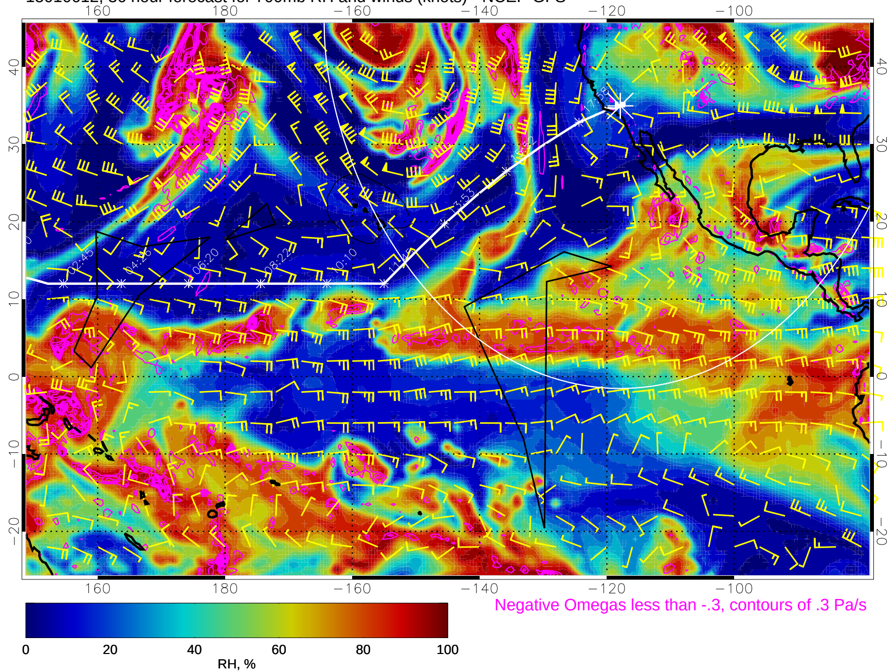
15010612, 36 hour forecast for 700mb RH and winds (knots) - NCEP GFS
