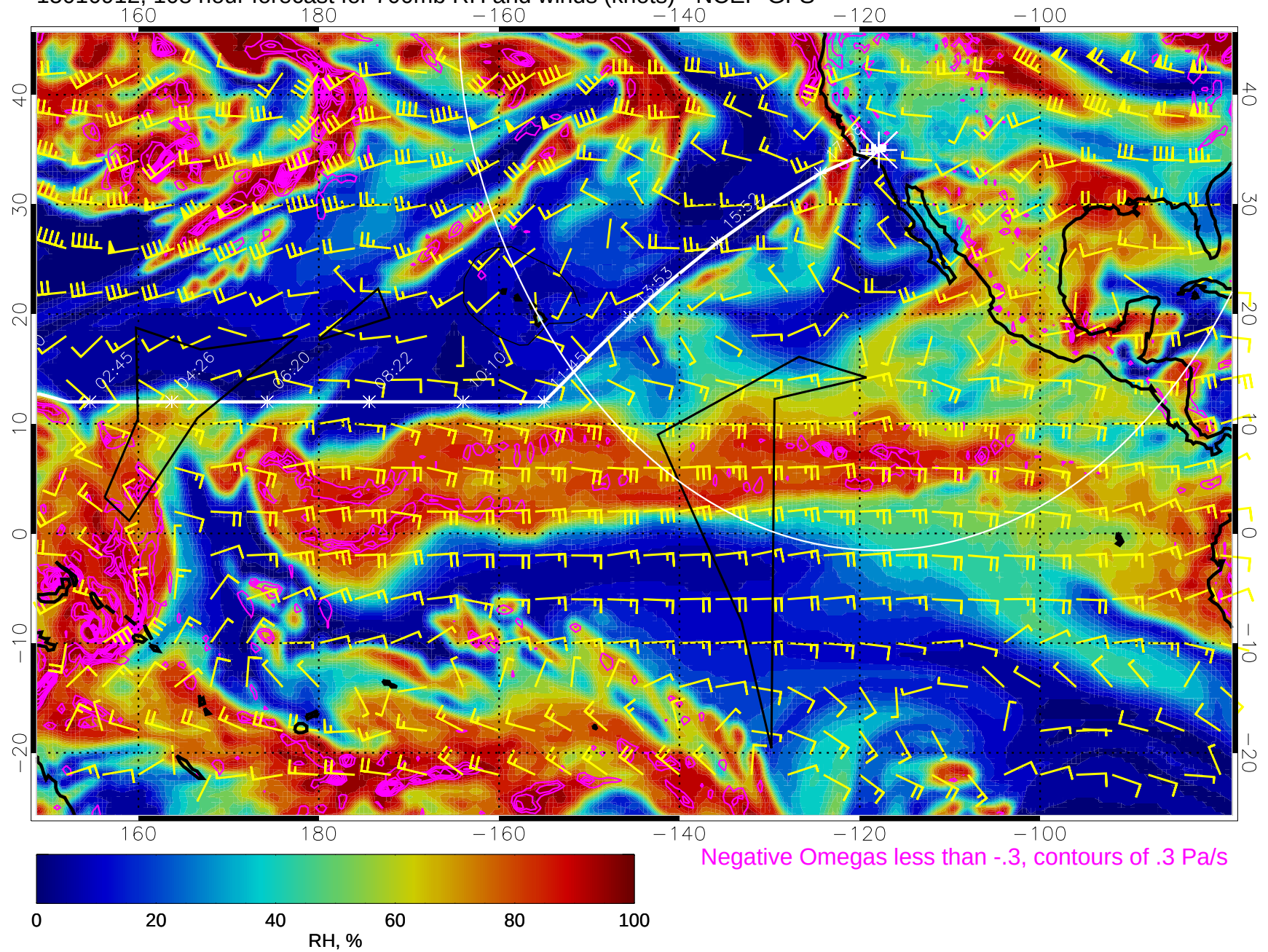
15010912, 108 hour forecast for 700mb RH and winds (knots) - NCEP GFS
