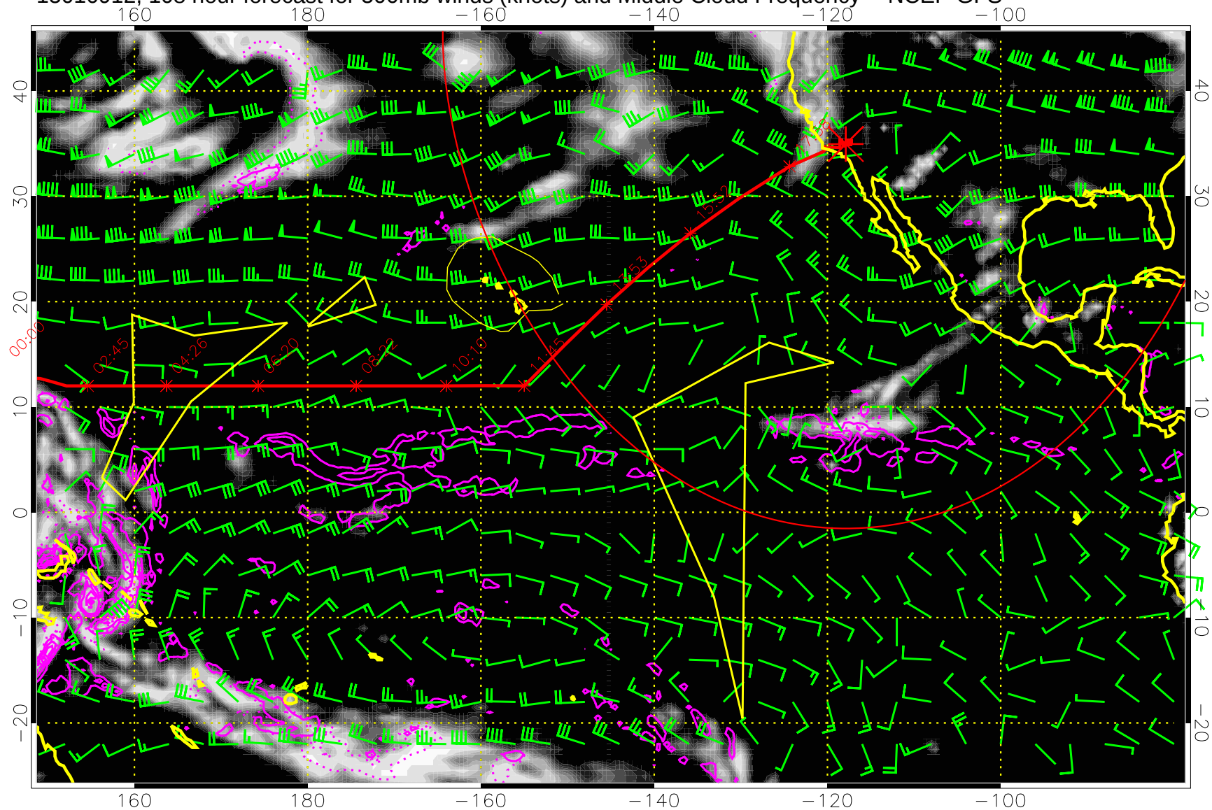
15010912, 108 hour forecast for 500mb winds (knots) and Middle Cloud Frequency -- NCEP GFS
