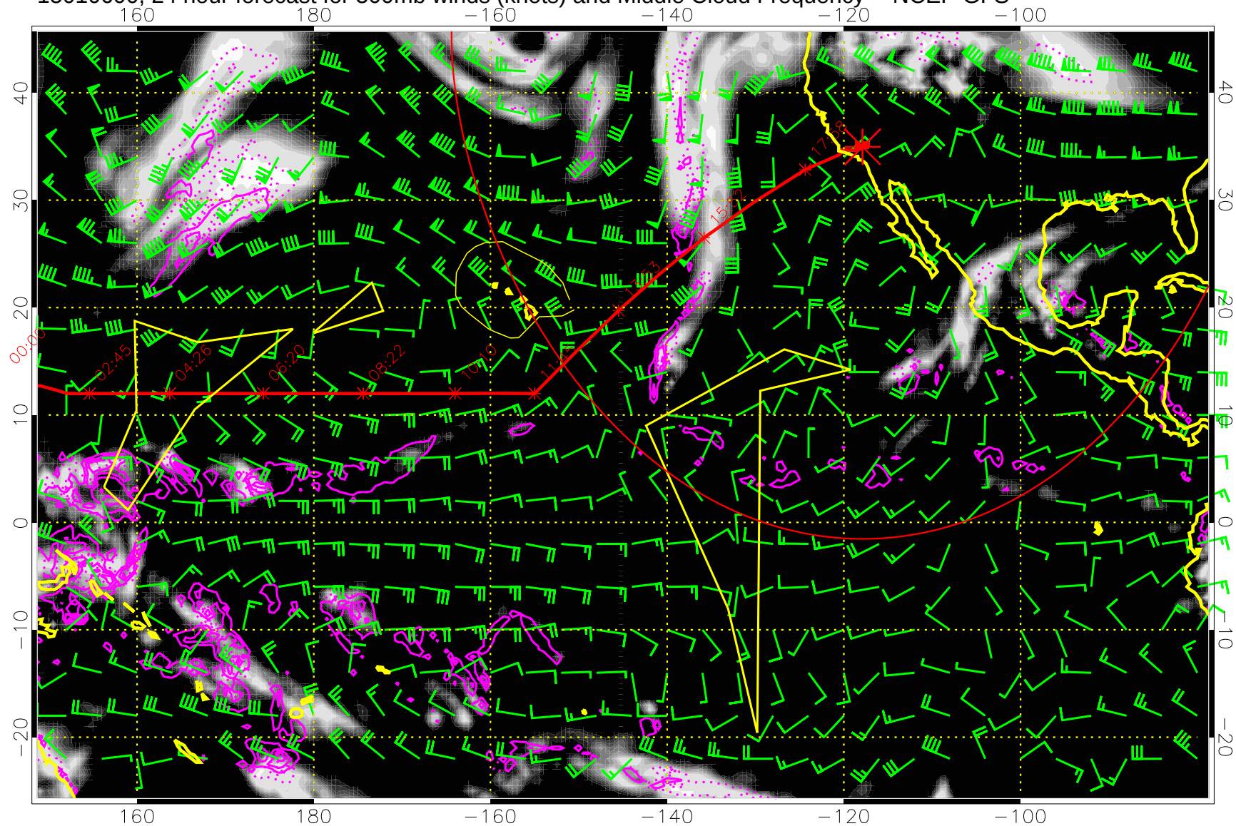
15010600, 24 hour forecast for 500mb winds (knots) and Middle Cloud Frequency -- NCEP GFS
