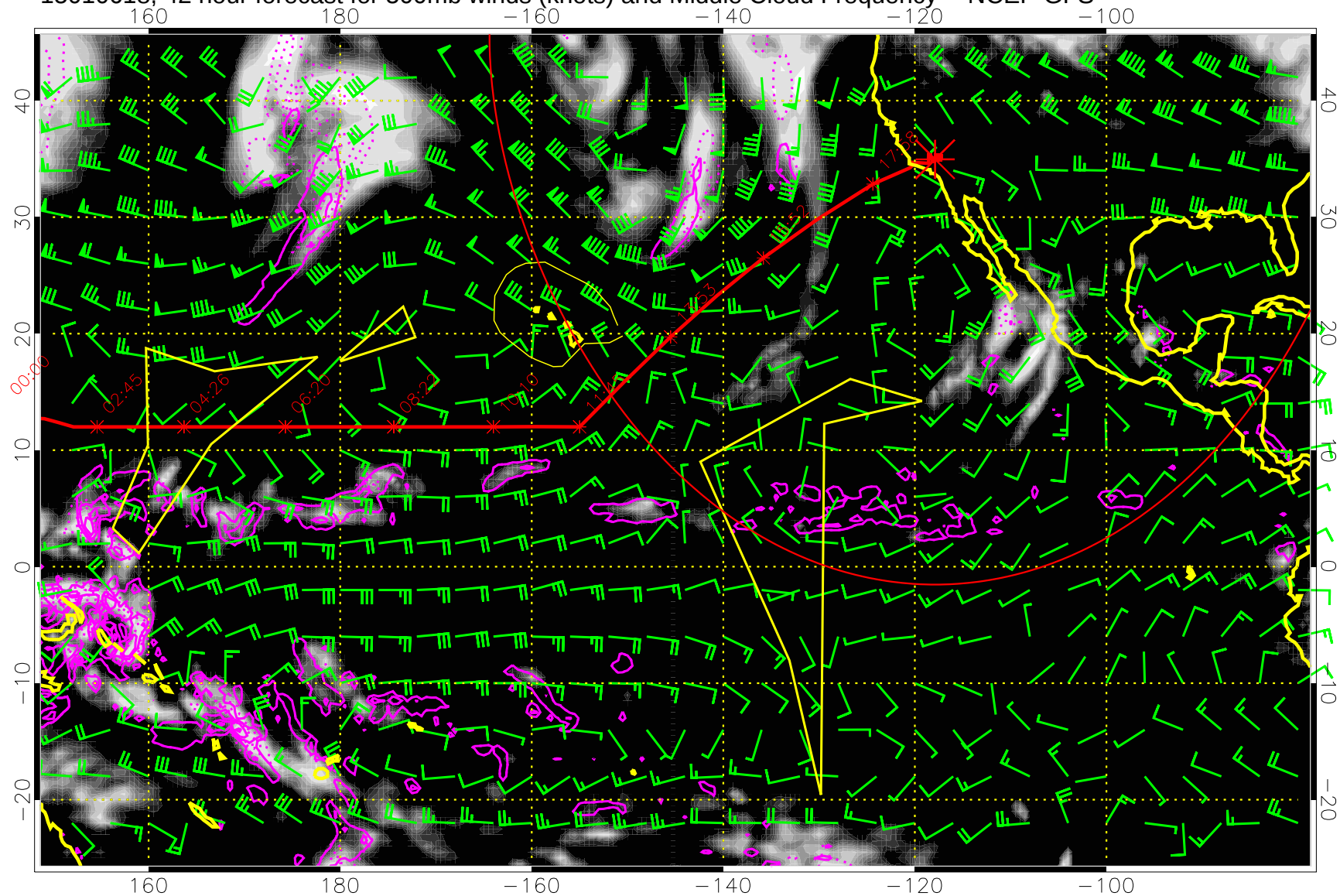
15010618, 42 hour forecast for 500mb winds (knots) and Middle Cloud Frequency -- NCEP GFS
