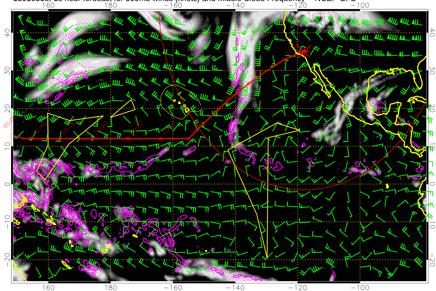
15010518, 18 hour forecast for 500mb winds (knots) and Middle Cloud Frequency -- NCEP GFS
