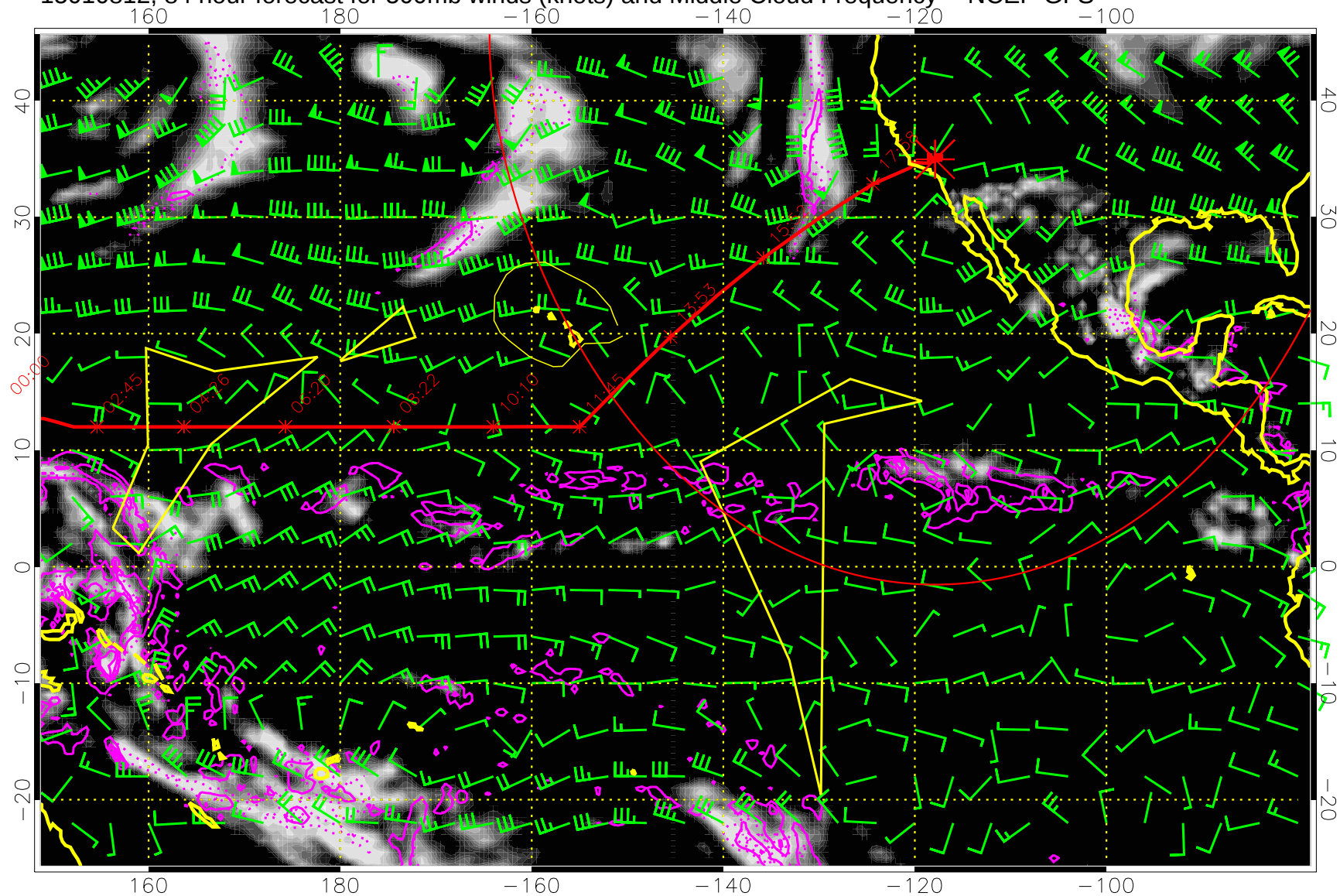
15010812, 84 hour forecast for 500mb winds (knots) and Middle Cloud Frequency -- NCEP GFS
