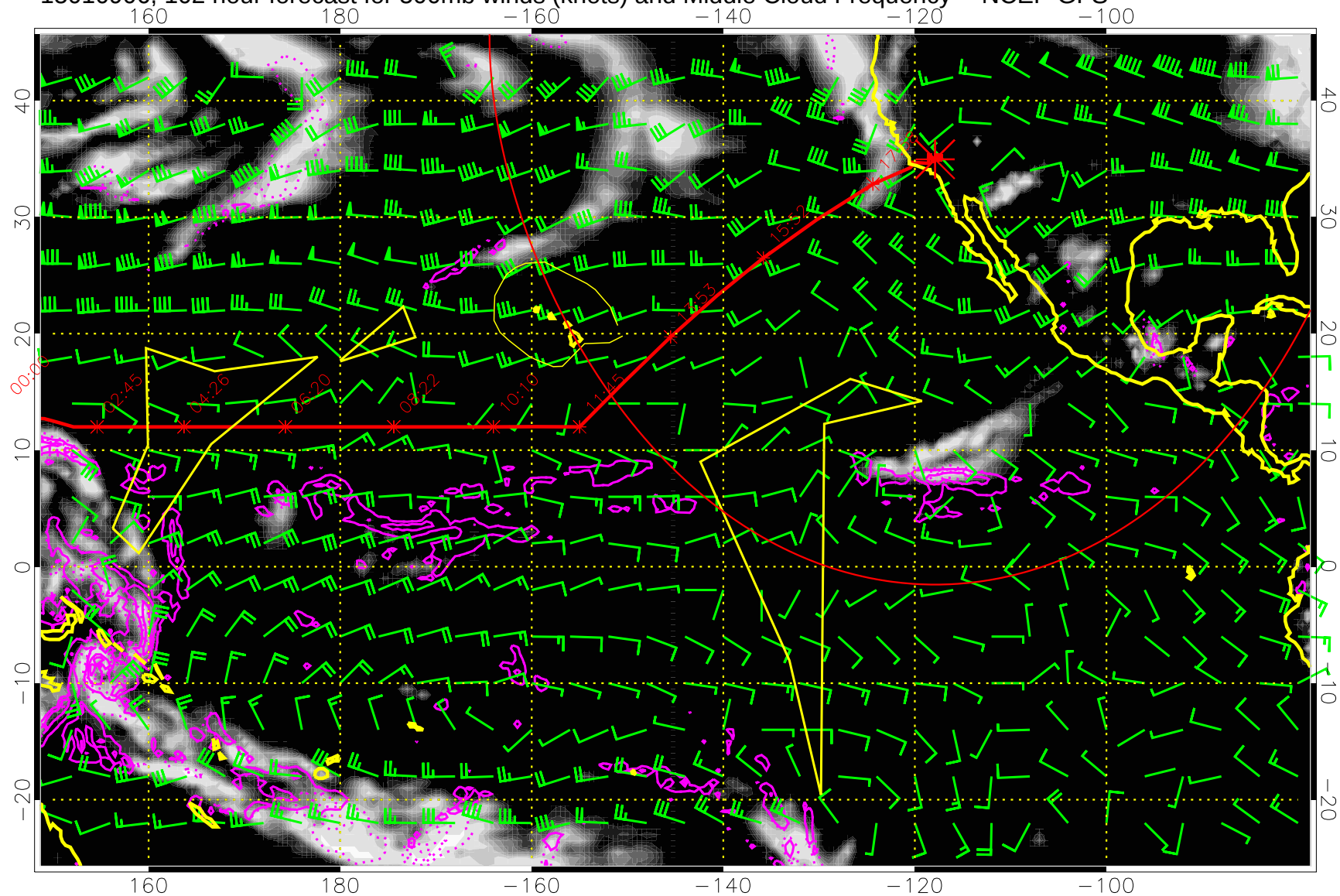
15010906, 102 hour forecast for 500mb winds (knots) and Middle Cloud Frequency -- NCEP GFS
