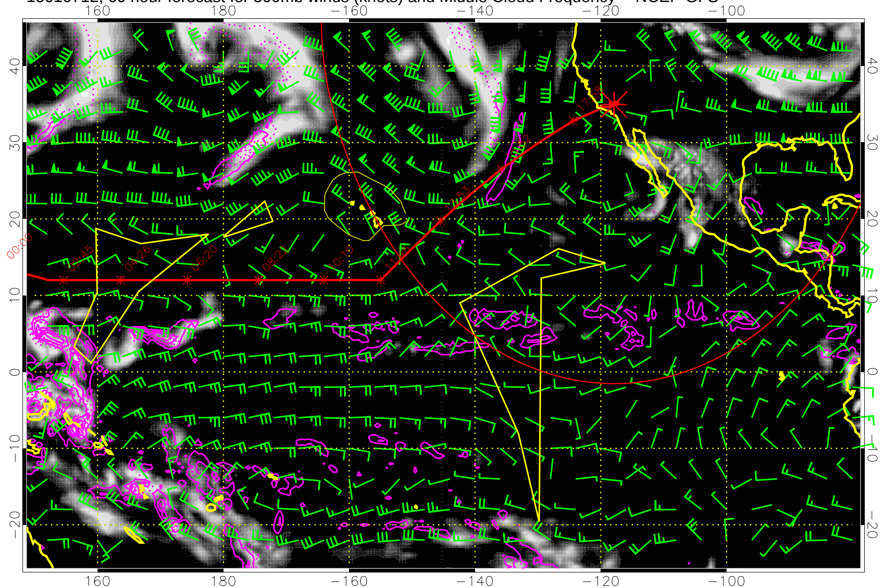
15010712, 60 hour forecast for 500mb winds (knots) and Middle Cloud Frequency -- NCEP GFS
