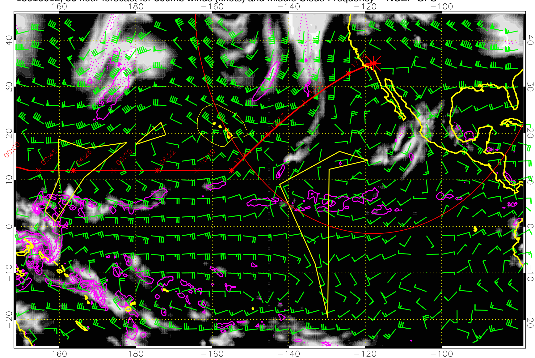
15010612, 36 hour forecast for 500mb winds (knots) and Middle Cloud Frequency -- NCEP GFS
