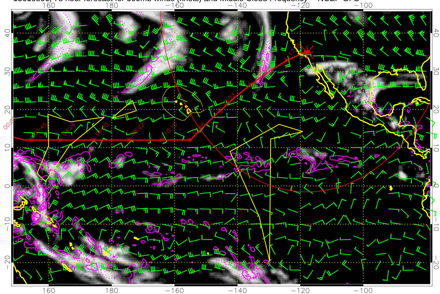
15010806, 78 hour forecast for 500mb winds (knots) and Middle Cloud Frequency -- NCEP GFS
