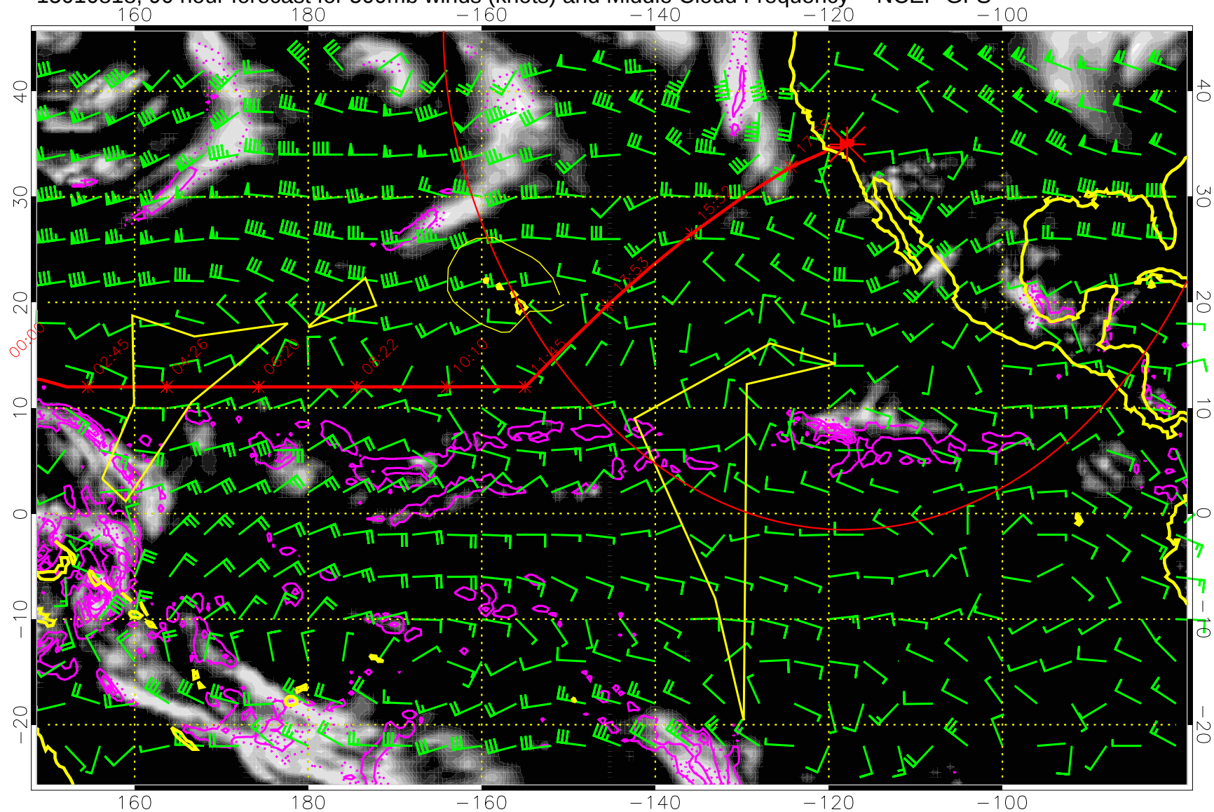
15010818, 90 hour forecast for 500mb winds (knots) and Middle Cloud Frequency -- NCEP GFS
