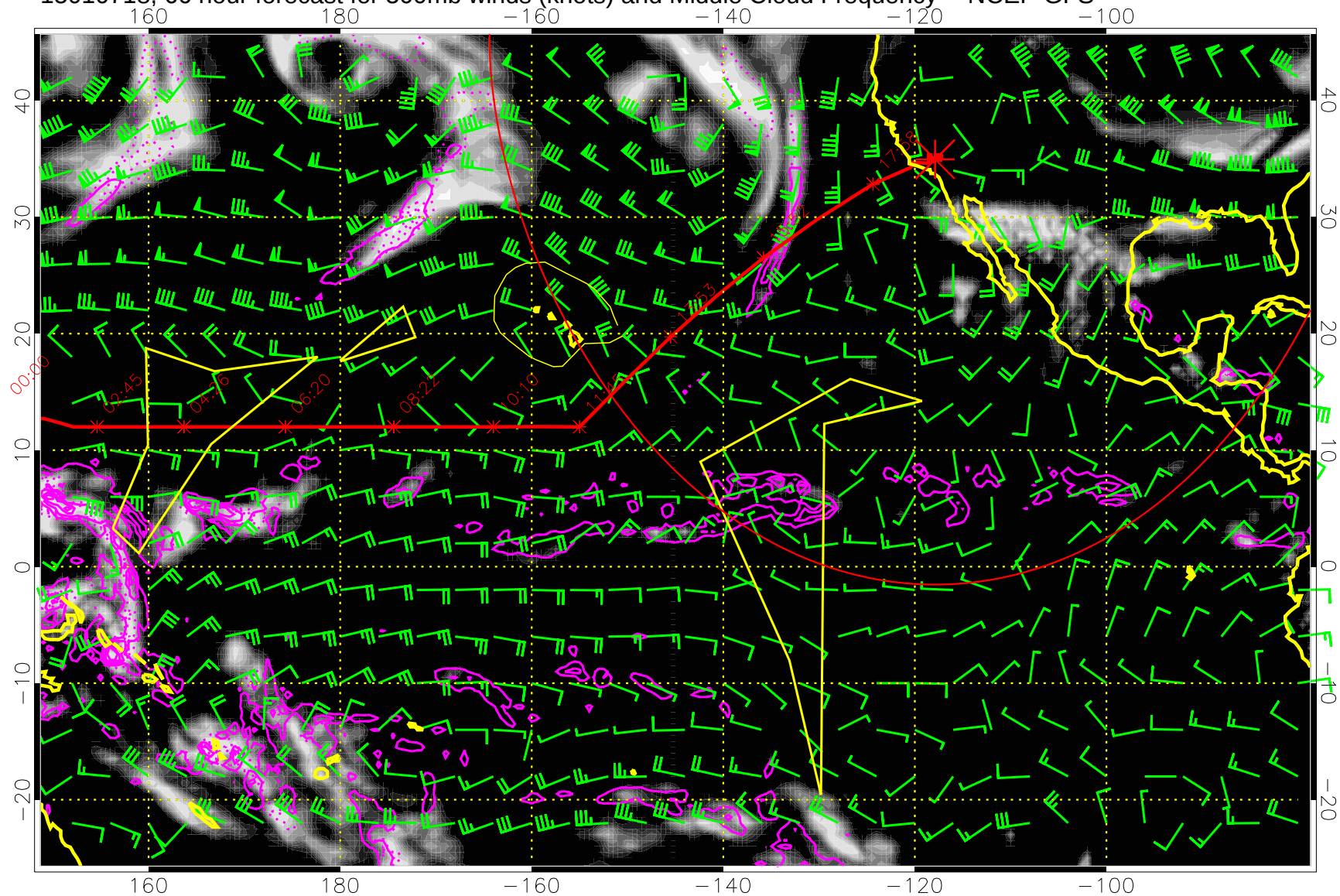
15010718, 66 hour forecast for 500mb winds (knots) and Middle Cloud Frequency -- NCEP GFS
