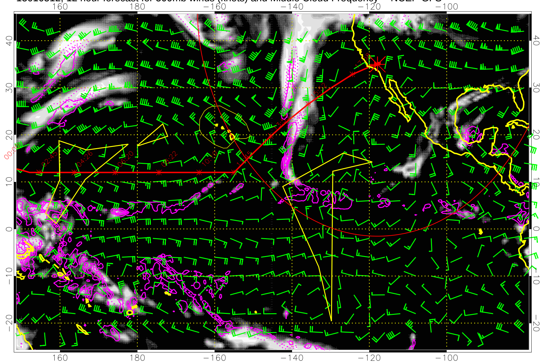
15010512, 12 hour forecast for 500mb winds (knots) and Middle Cloud Frequency -- NCEP GFS
