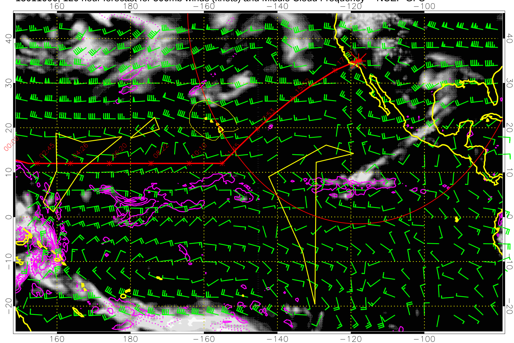
15011000, 120 hour forecast for 500mb winds (knots) and Middle Cloud Frequency -- NCEP GFS
