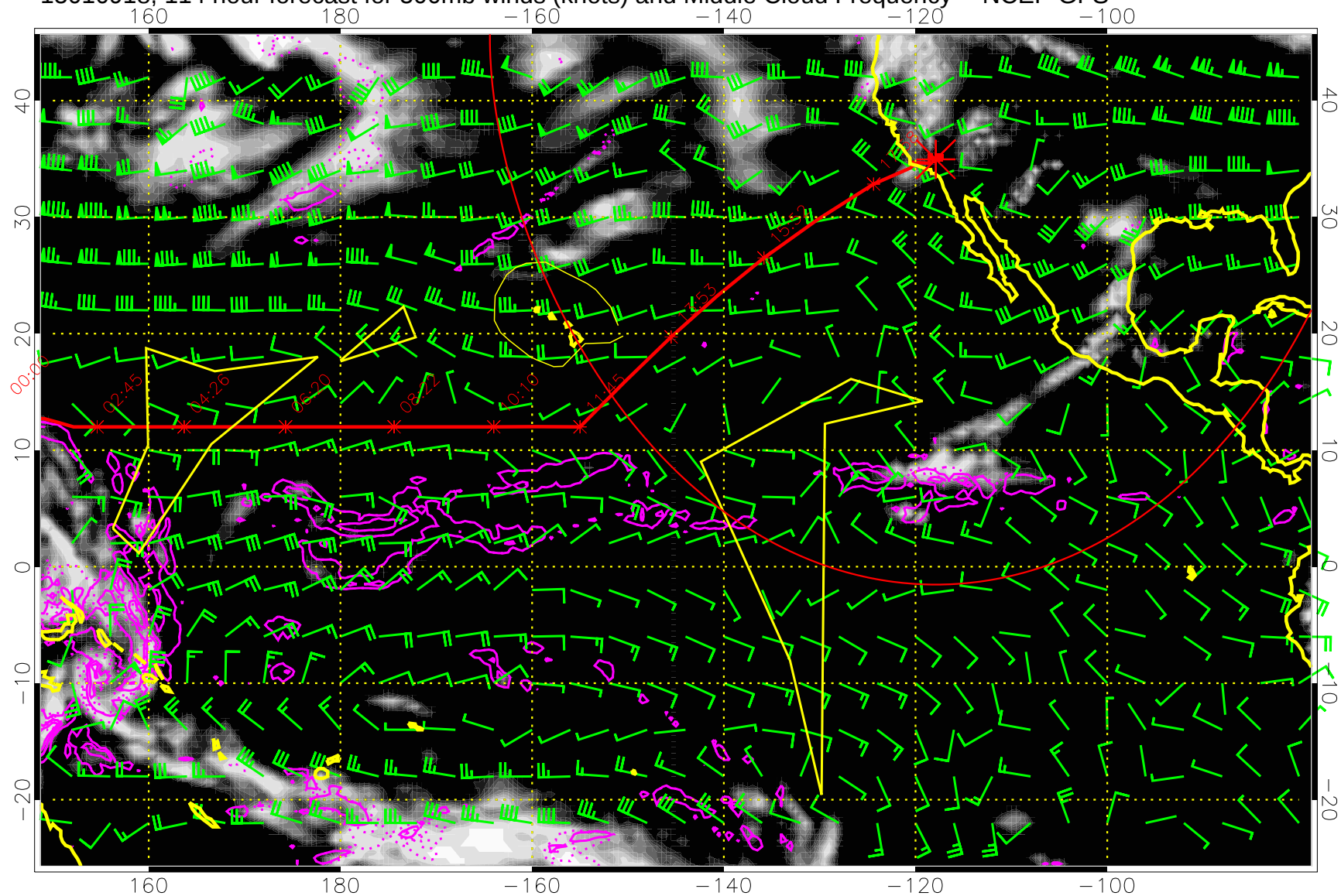
15010918, 114 hour forecast for 500mb winds (knots) and Middle Cloud Frequency -- NCEP GFS
