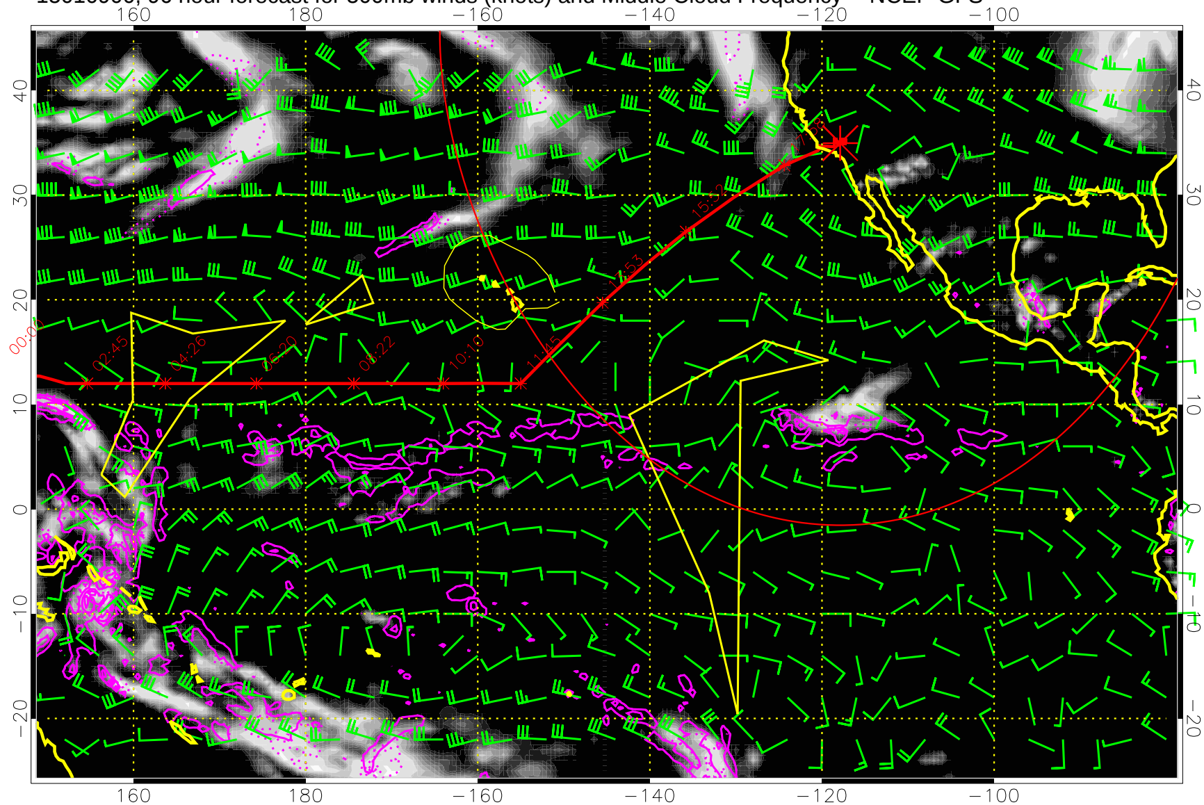
15010900, 96 hour forecast for 500mb winds (knots) and Middle Cloud Frequency -- NCEP GFS
