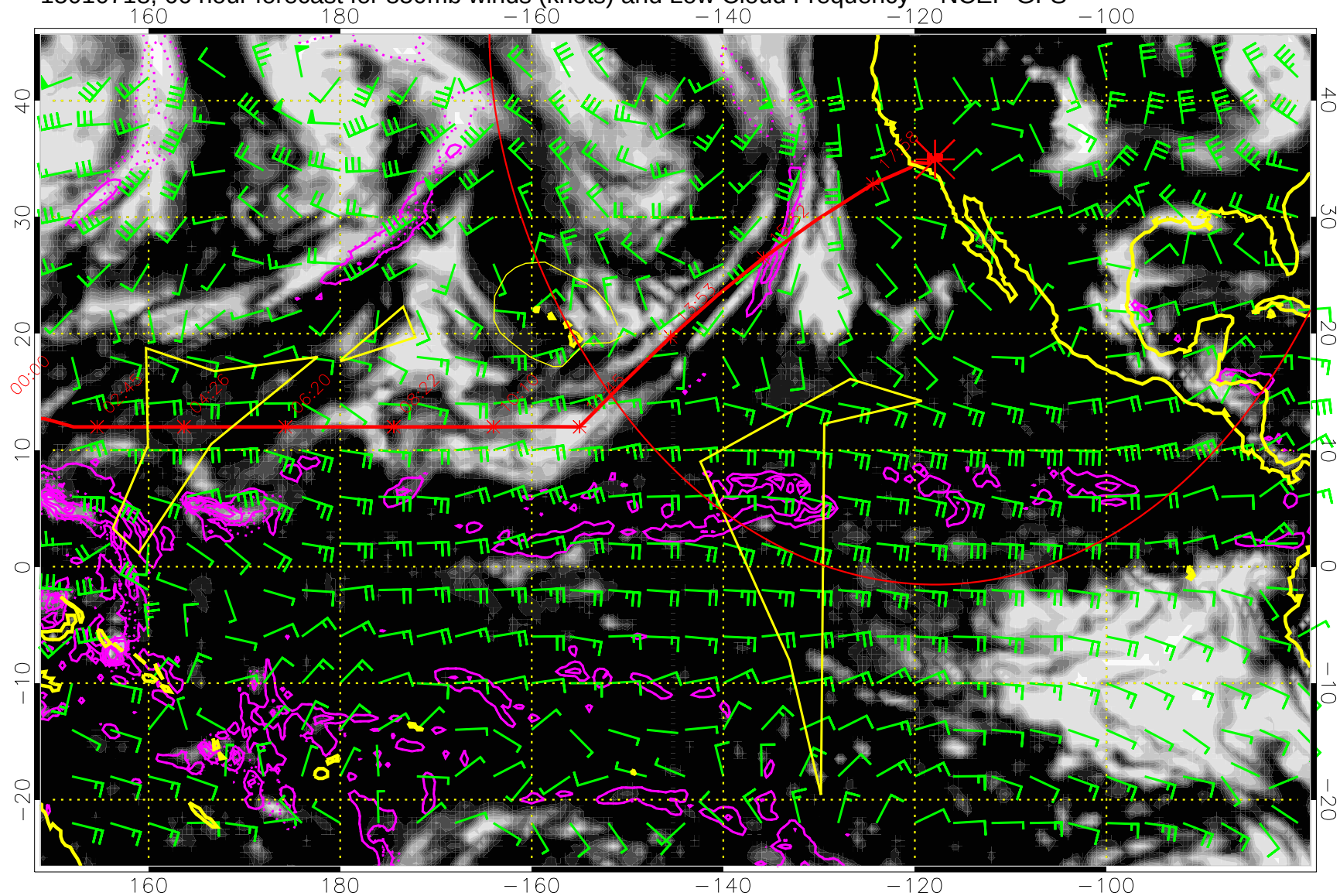
15010718, 66 hour forecast for 850mb winds (knots) and Low Cloud Frequency -- NCEP GFS
