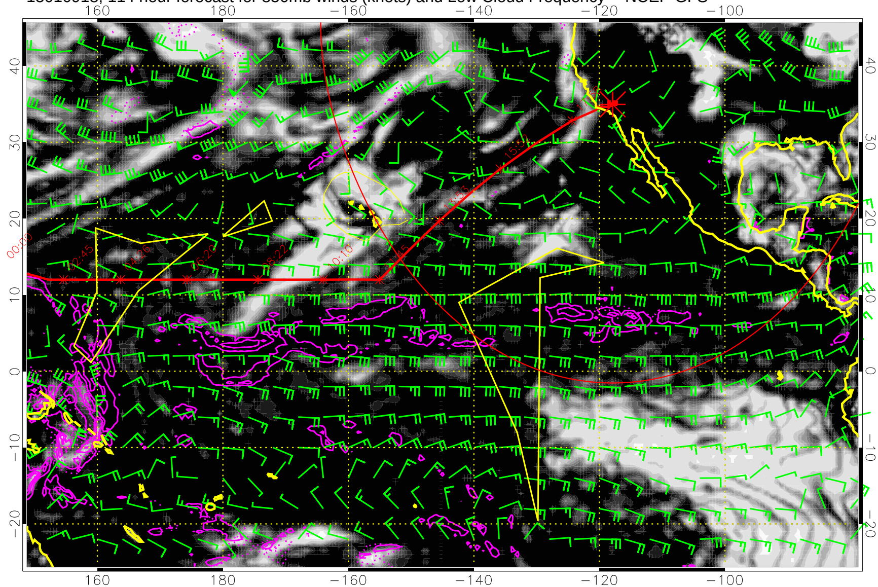
15010918, 114 hour forecast for 850mb winds (knots) and Low Cloud Frequency -- NCEP GFS
