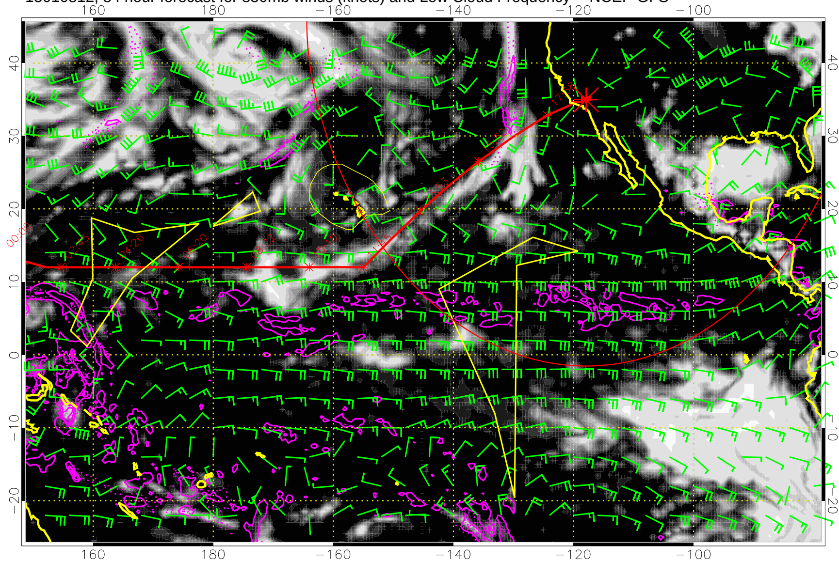
15010812, 84 hour forecast for 850mb winds (knots) and Low Cloud Frequency -- NCEP GFS
