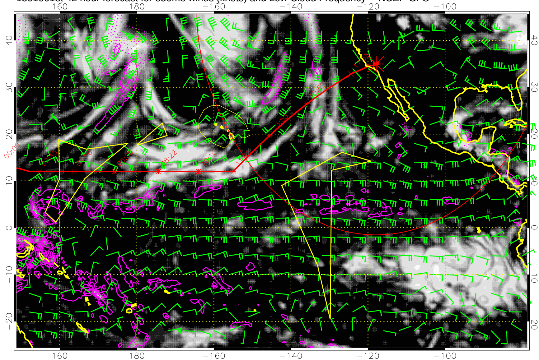
15010618, 42 hour forecast for 850mb winds (knots) and Low Cloud Frequency -- NCEP GFS
