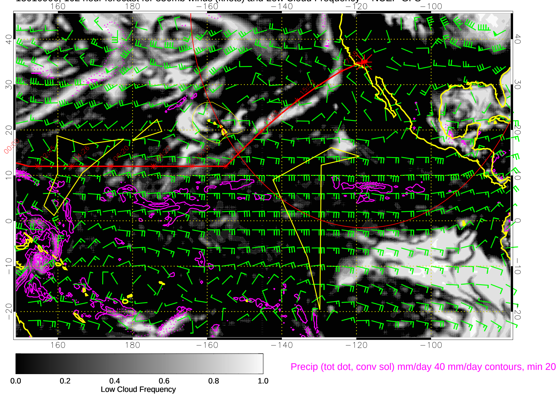
15010906, 102 hour forecast for 850mb winds (knots) and Low Cloud Frequency -- NCEP GFS
