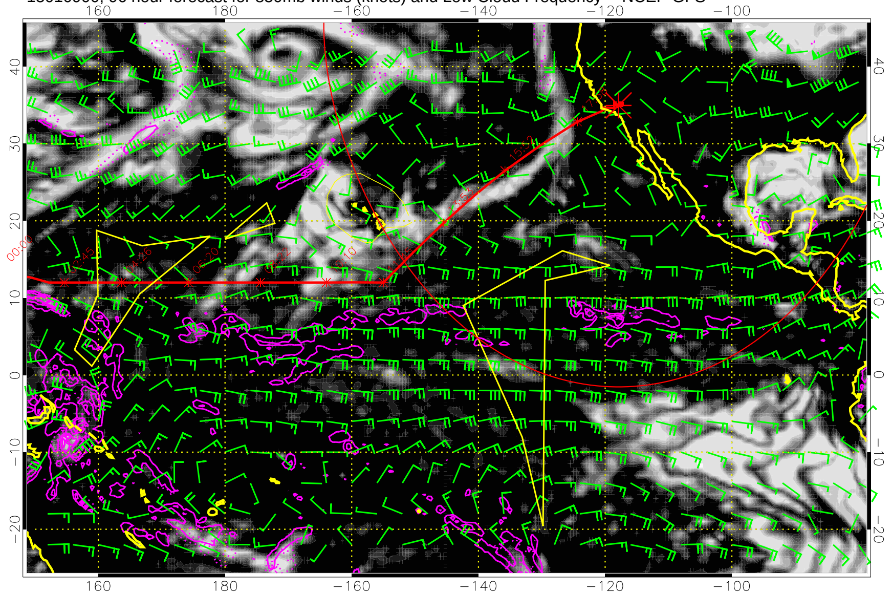
15010900, 96 hour forecast for 850mb winds (knots) and Low Cloud Frequency -- NCEP GFS
