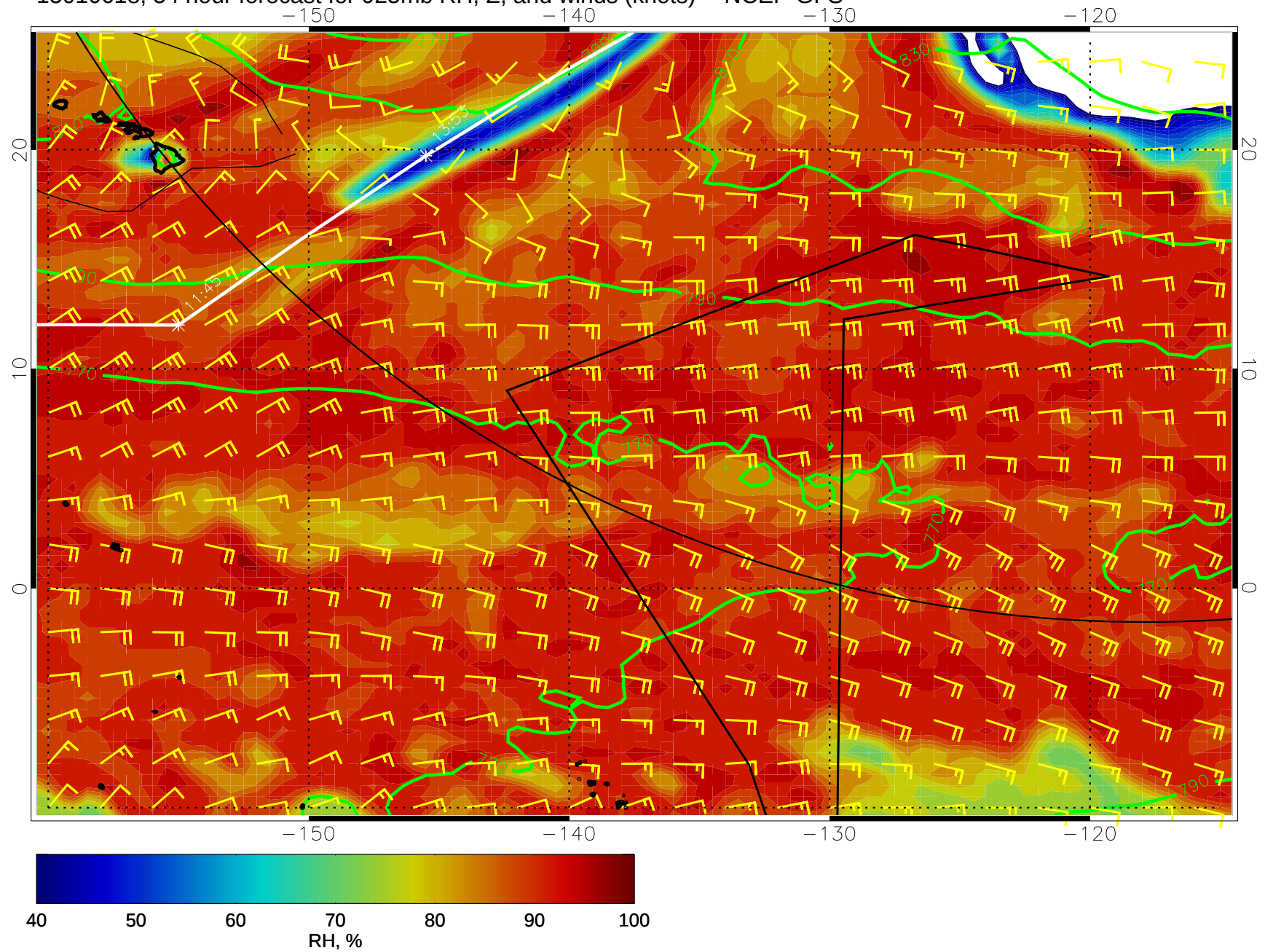
15010618, 54 hour forecast for 925mb RH, Z, and winds (knots) -- NCEP GFS
