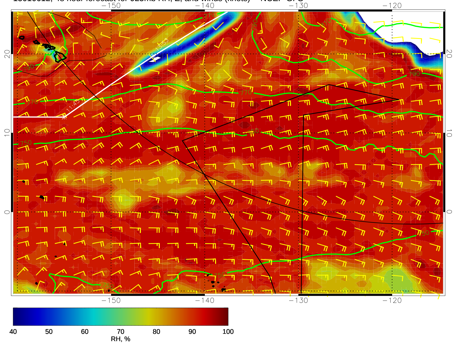
15010612, 48 hour forecast for 925mb RH, Z, and winds (knots) -- NCEP GFS
