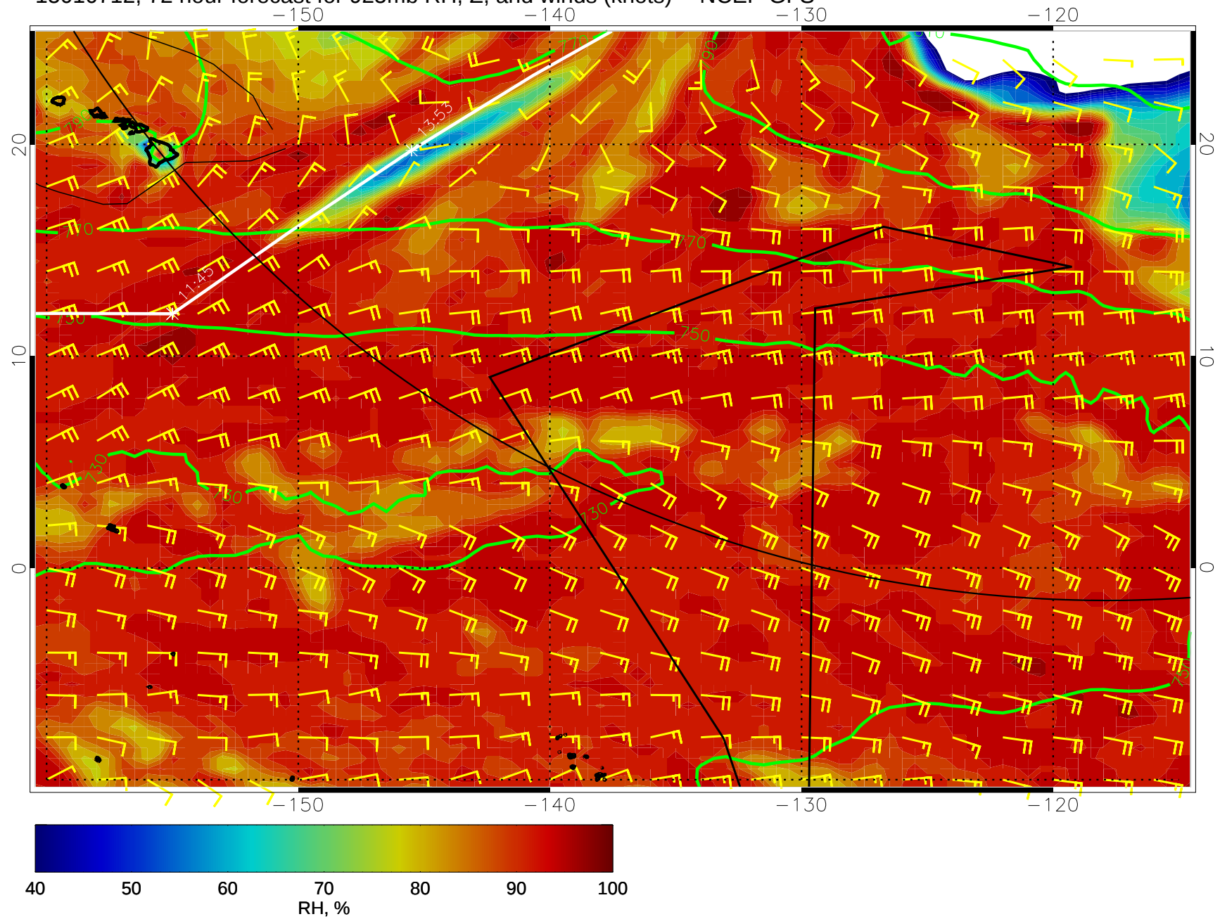
15010712, 72 hour forecast for 925mb RH, Z, and winds (knots) -- NCEP GFS
