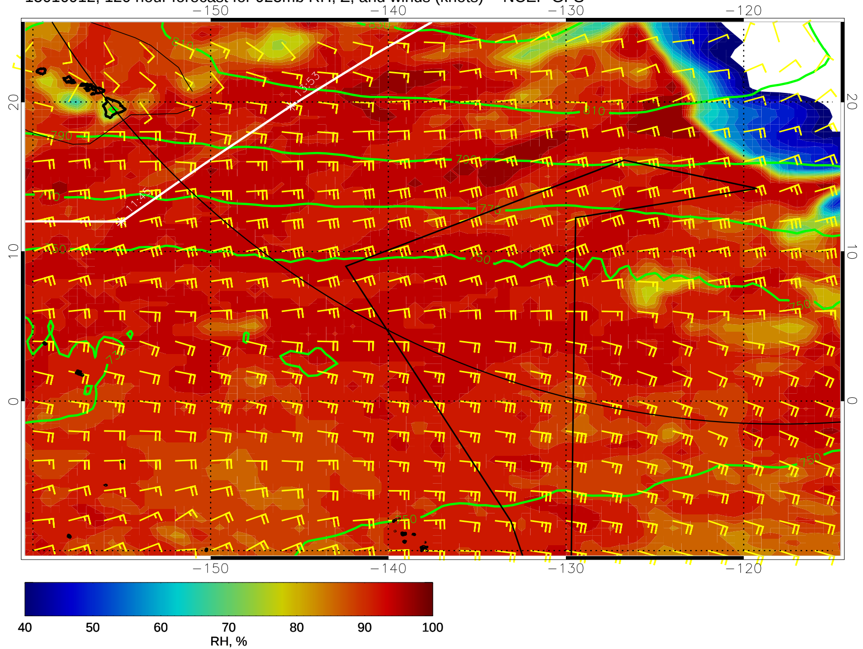
15010912, 120 hour forecast for 925mb RH, Z, and winds (knots) -- NCEP GFS
