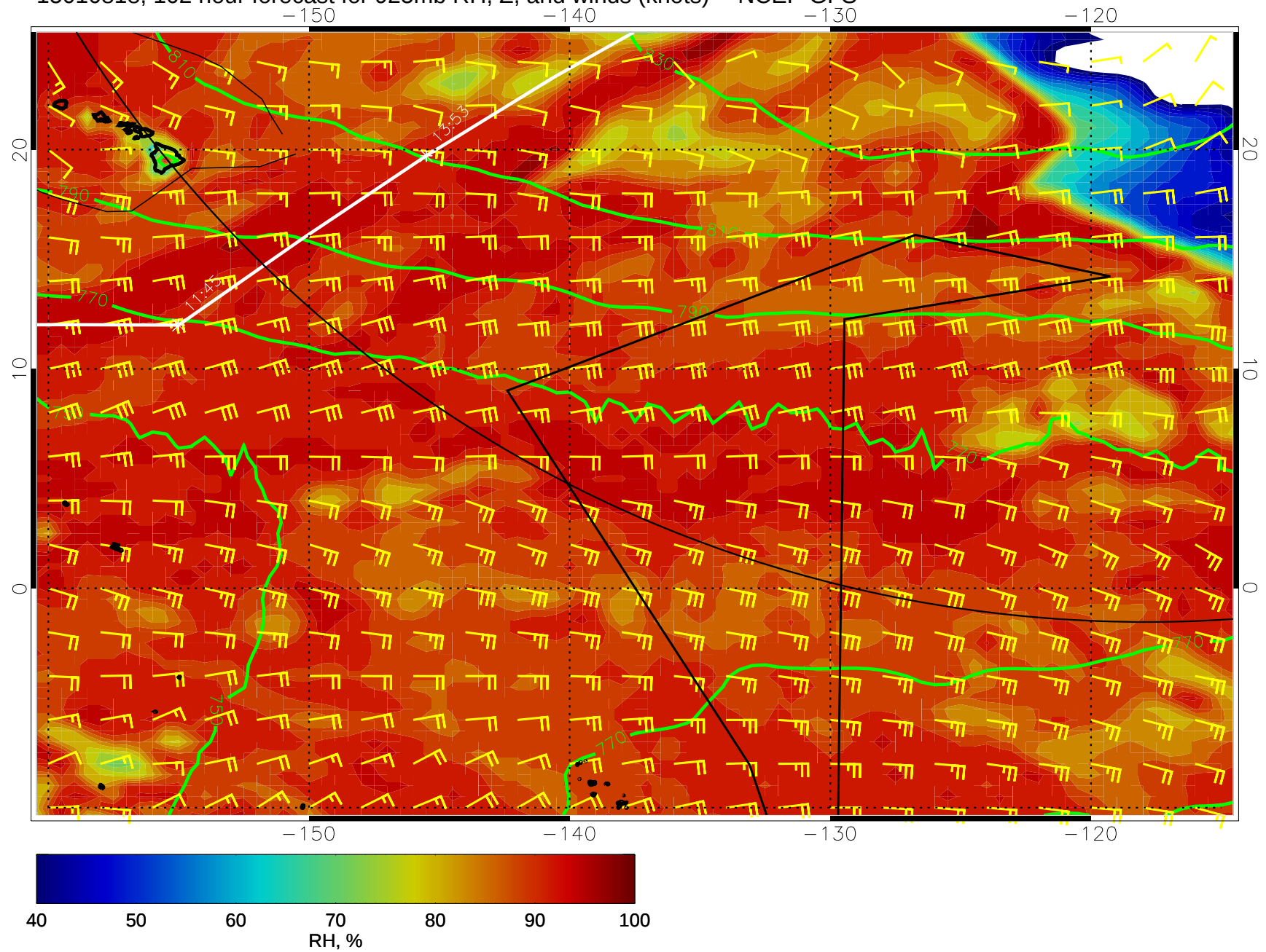
15010818, 102 hour forecast for 925mb RH, Z, and winds (knots) -- NCEP GFS
