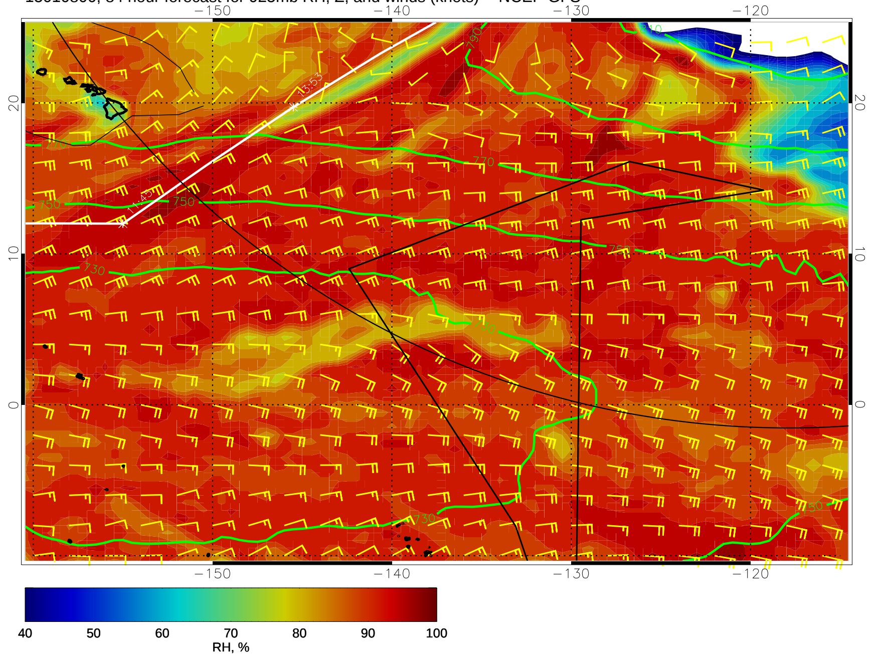
15010800, 84 hour forecast for 925mb RH, Z, and winds (knots) -- NCEP GFS
