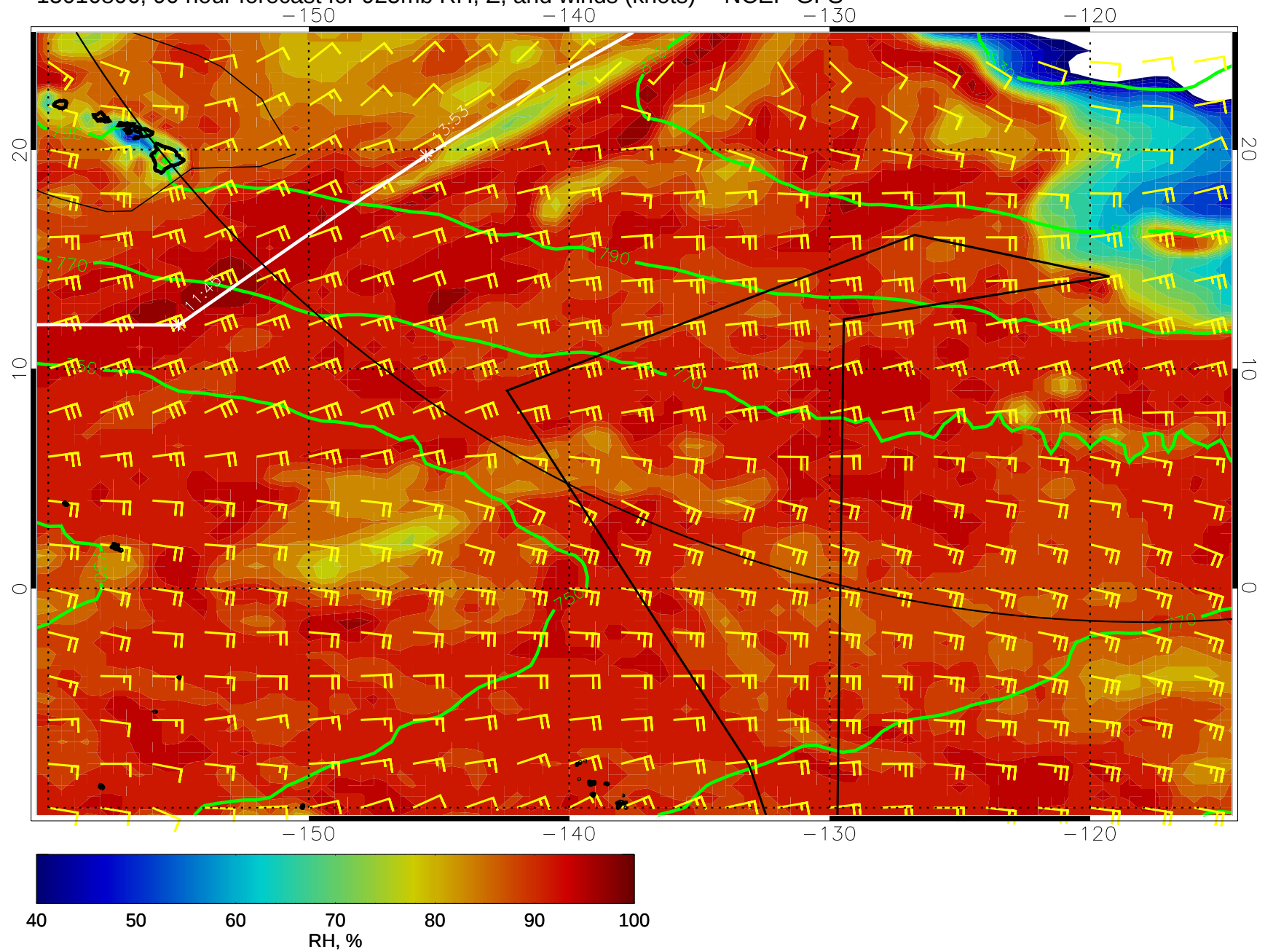
15010806, 90 hour forecast for 925mb RH, Z, and winds (knots) -- NCEP GFS
