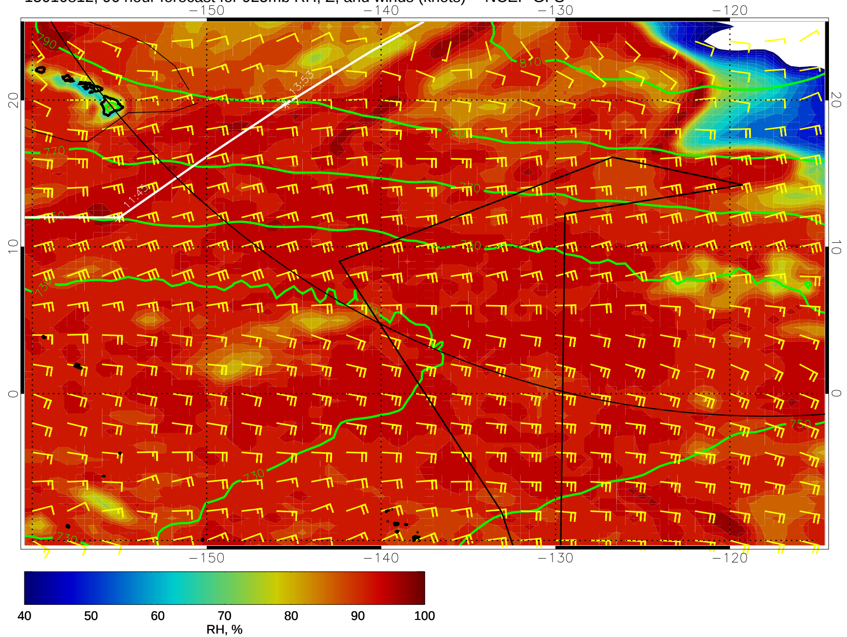
15010812, 96 hour forecast for 925mb RH, Z, and winds (knots) -- NCEP GFS
