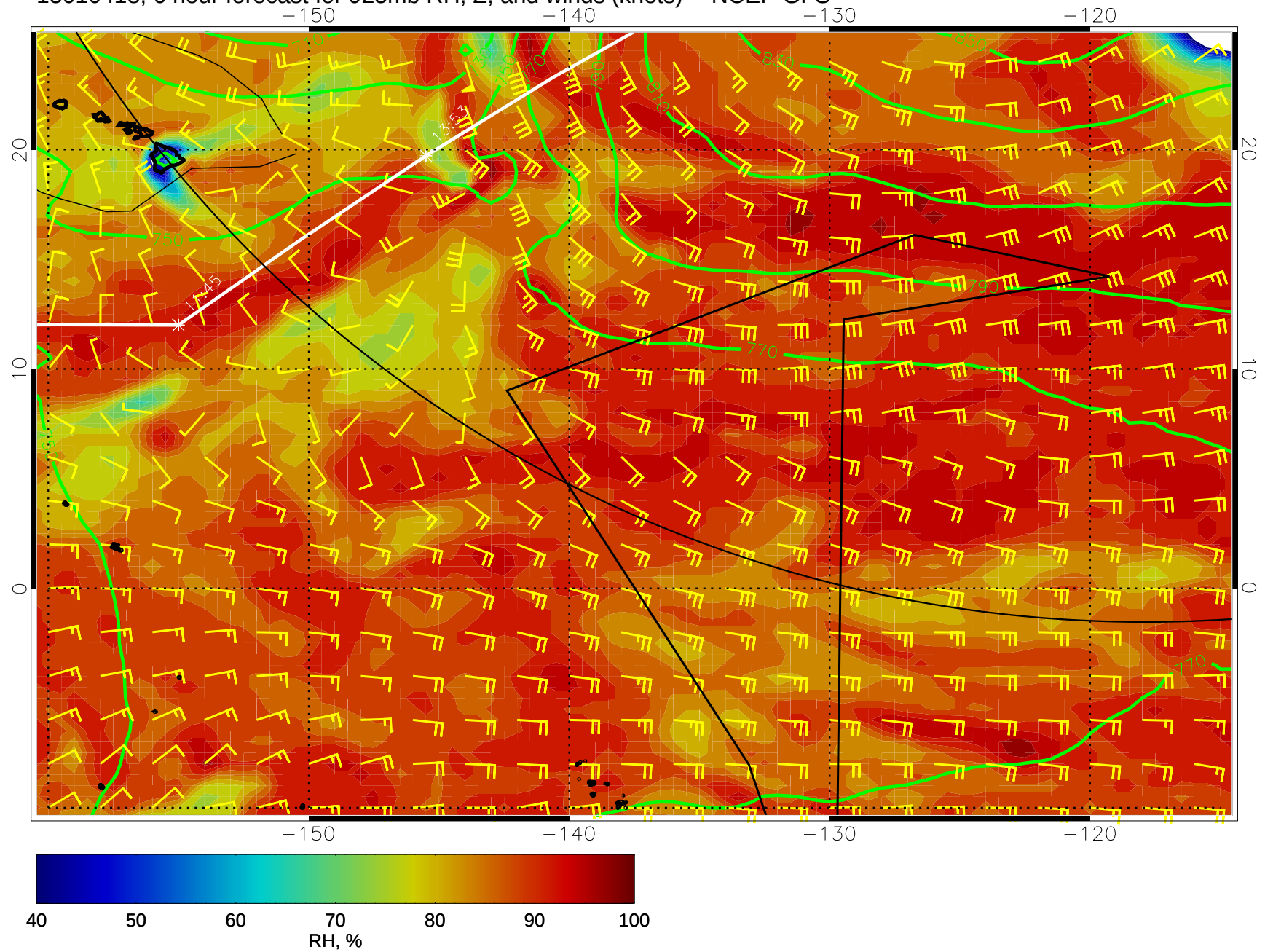
15010418, 6 hour forecast for 925mb RH, Z, and winds (knots) -- NCEP GFS
