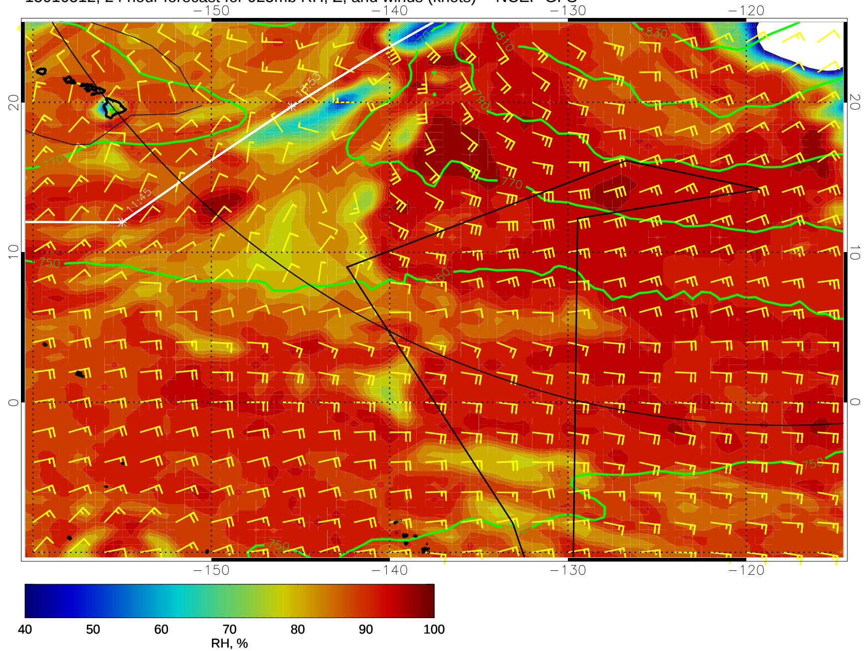
15010512, 24 hour forecast for 925mb RH, Z, and winds (knots) -- NCEP GFS
