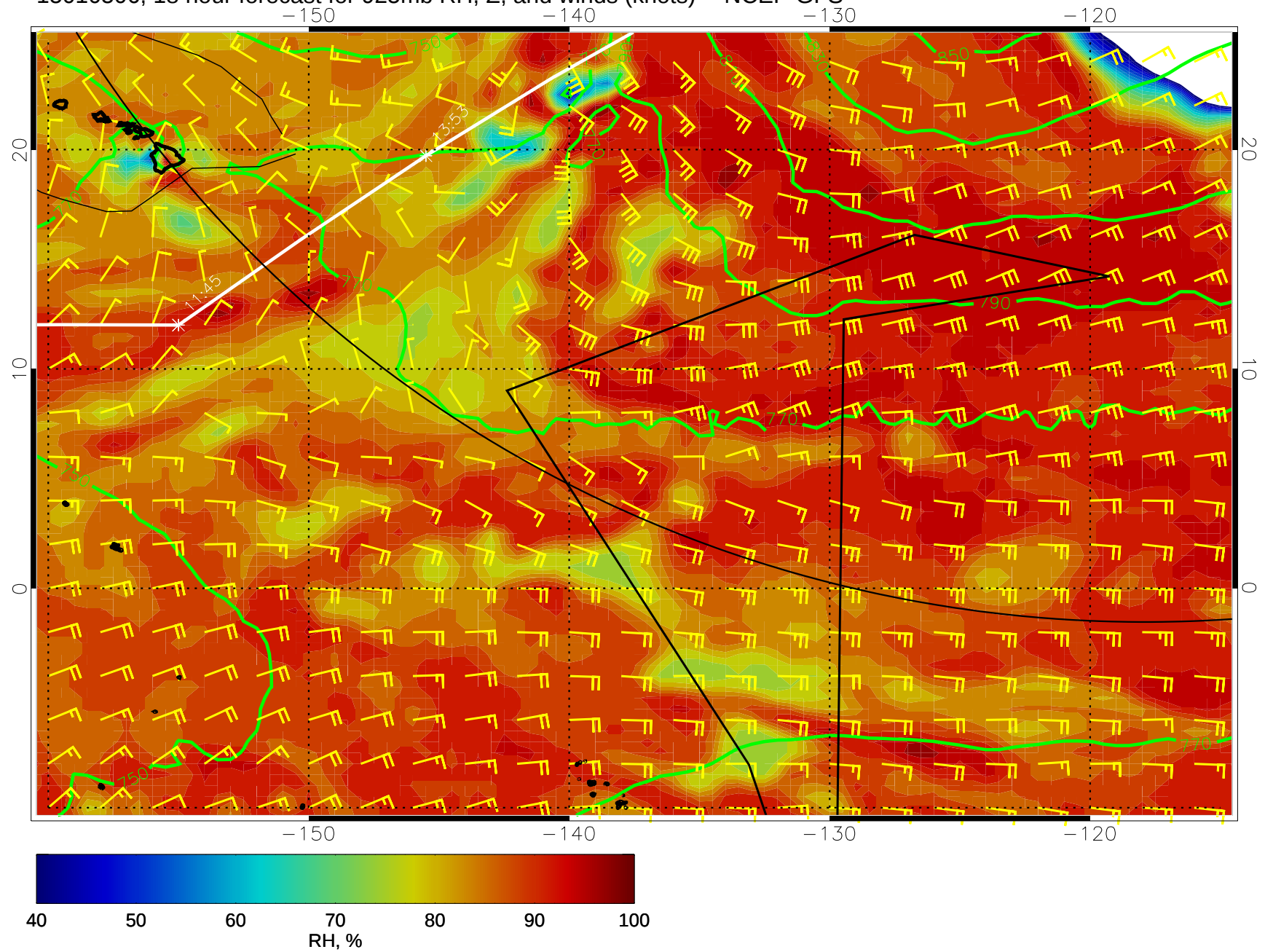
15010506, 18 hour forecast for 925mb RH, Z, and winds (knots) -- NCEP GFS
