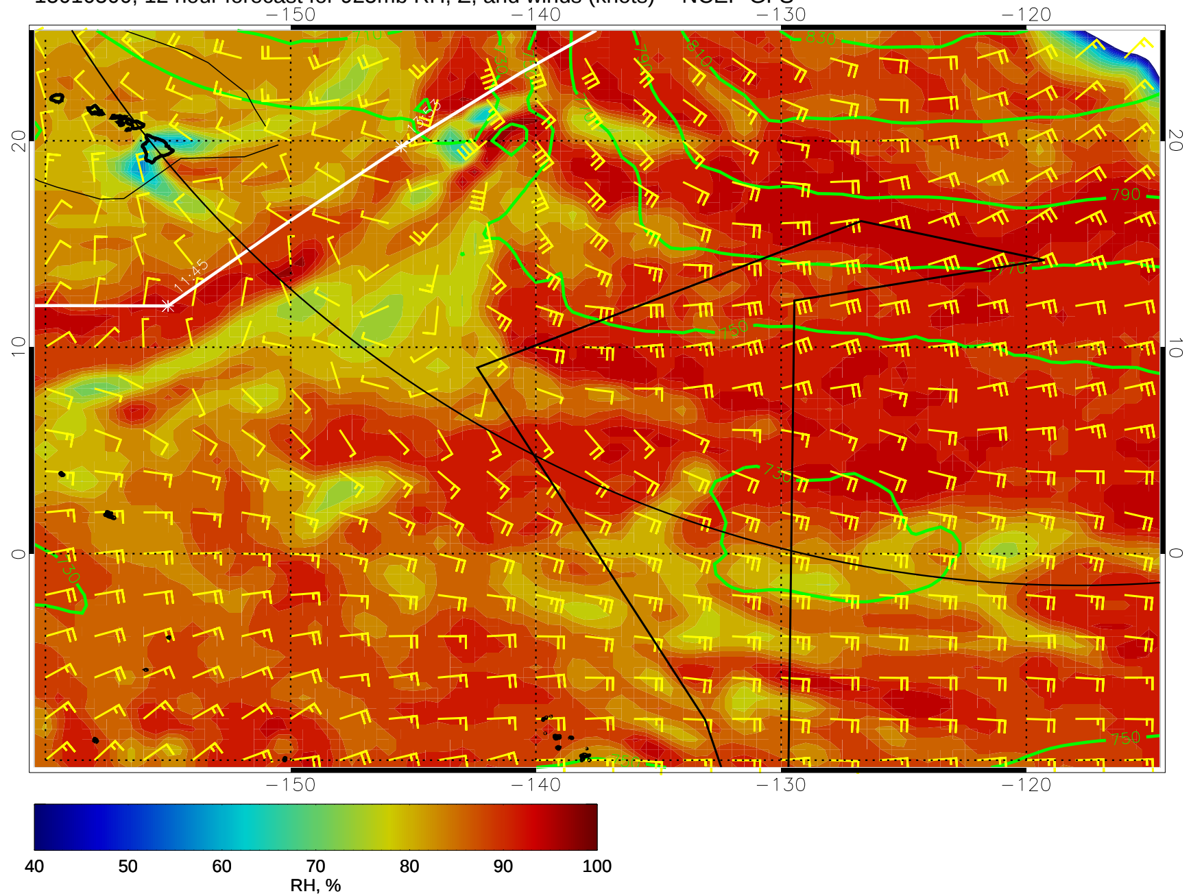
15010500, 12 hour forecast for 925mb RH, Z, and winds (knots) -- NCEP GFS
