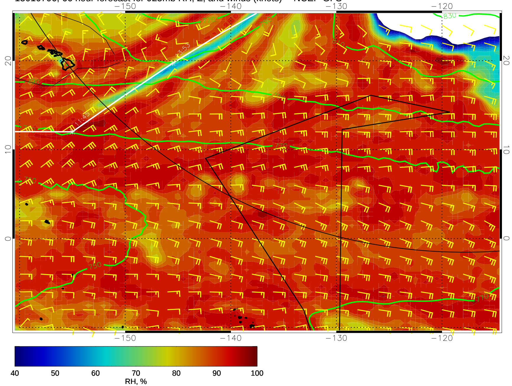
15010706, 66 hour forecast for 925mb RH, Z, and winds (knots) -- NCEP GFS
