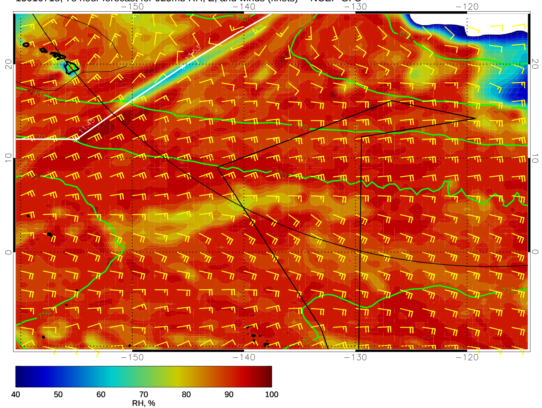
15010718, 78 hour forecast for 925mb RH, Z, and winds (knots) -- NCEP GFS
