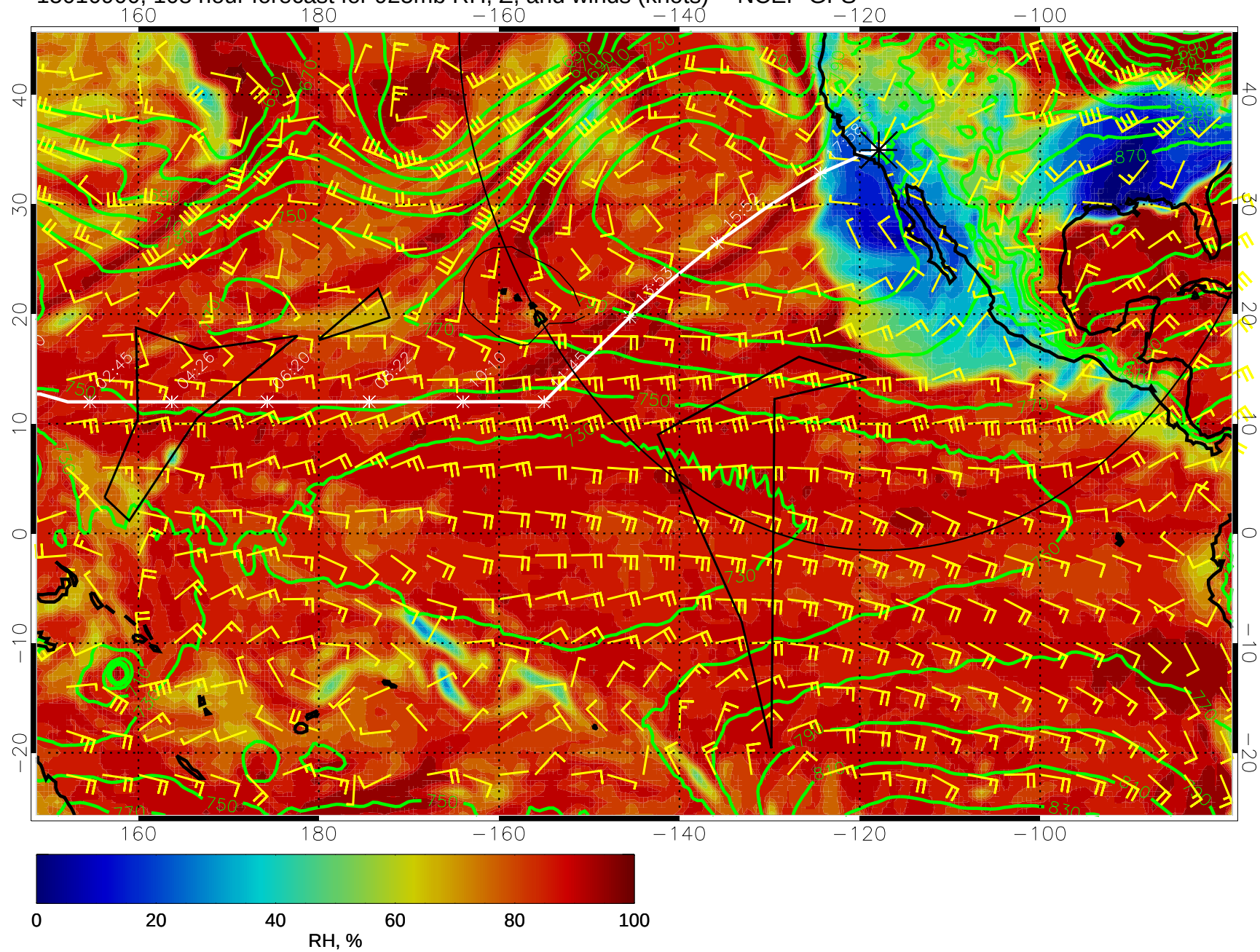
15010900, 108 hour forecast for 925mb RH, Z, and winds (knots) -- NCEP GFS
