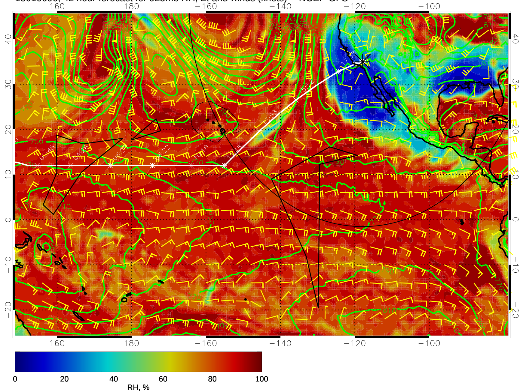
15010606, 42 hour forecast for 925mb RH, Z, and winds (knots) -- NCEP GFS
