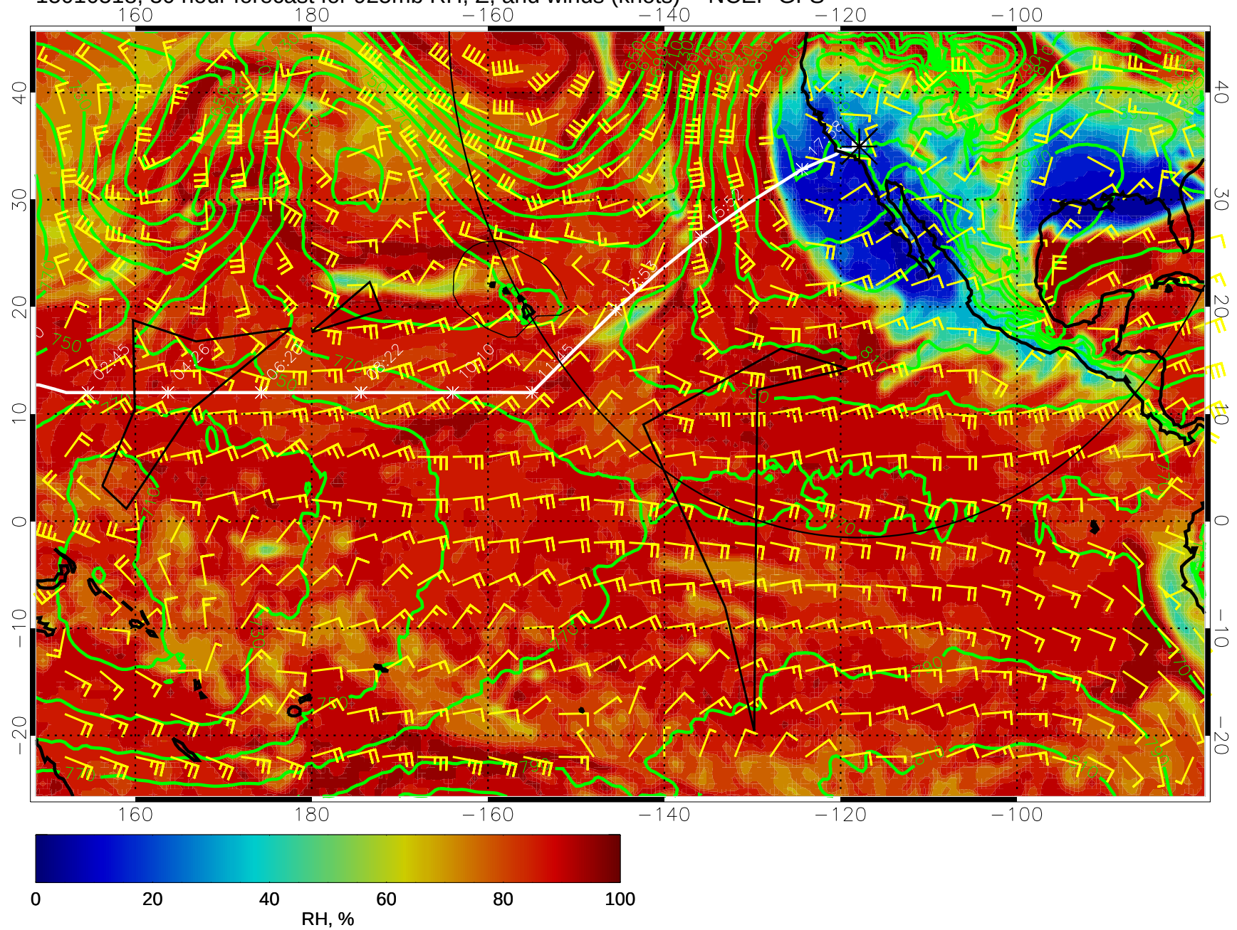
15010518, 30 hour forecast for 925mb RH, Z, and winds (knots) -- NCEP GFS
