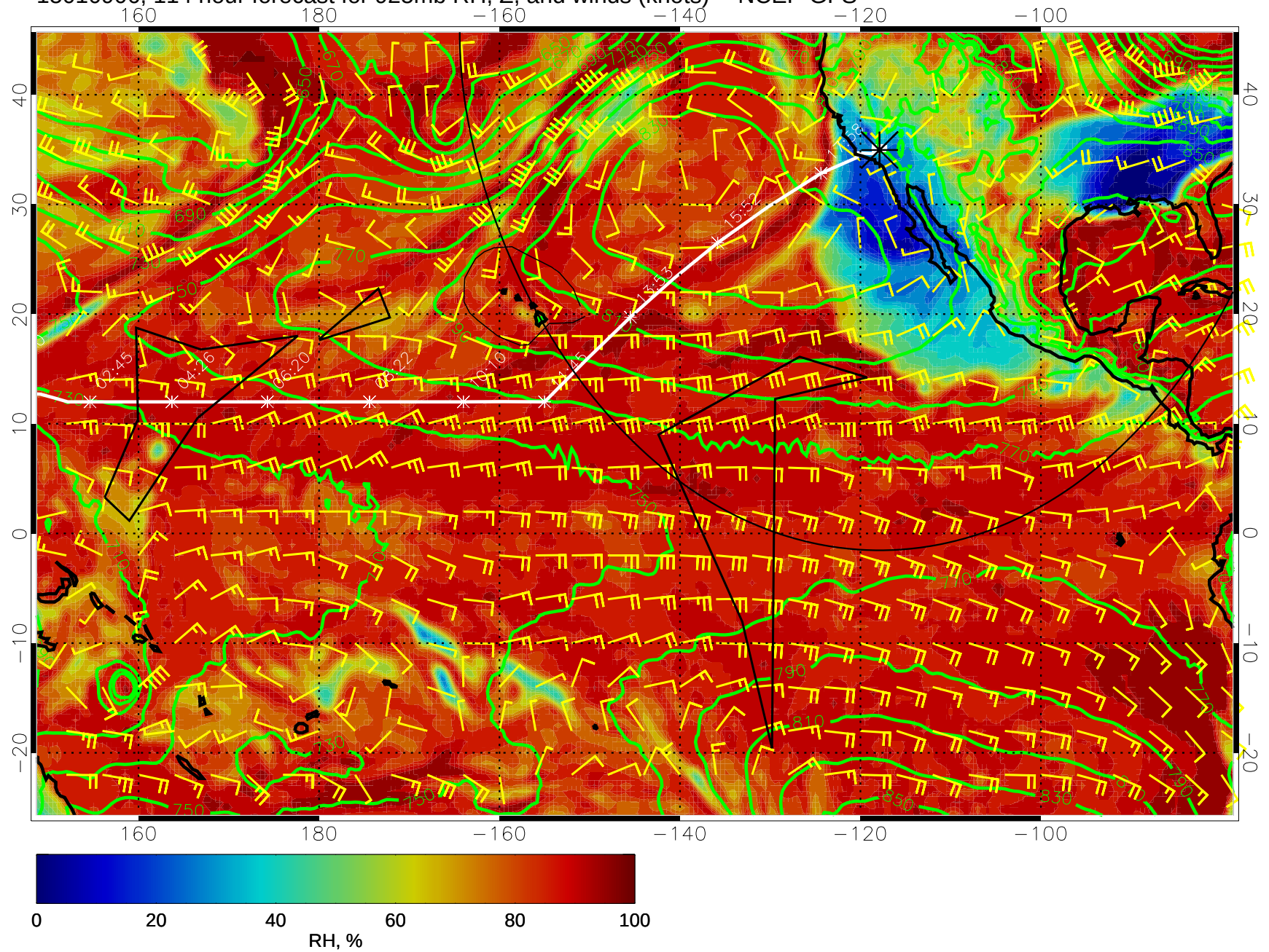
15010906, 114 hour forecast for 925mb RH, Z, and winds (knots) -- NCEP GFS
