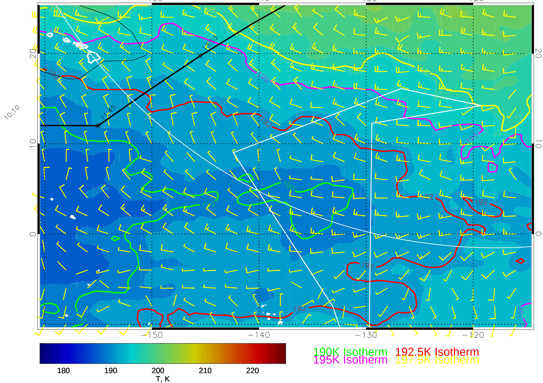
15010818, 102 hour forecast for 70mb T and winds (knots) -- NCEP GFS
