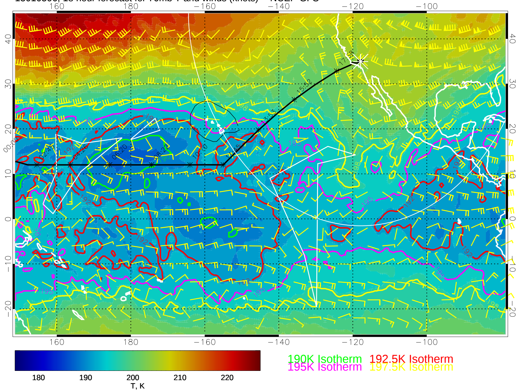
15010506, 18 hour forecast for 70mb T and winds (knots) -- NCEP GFS
