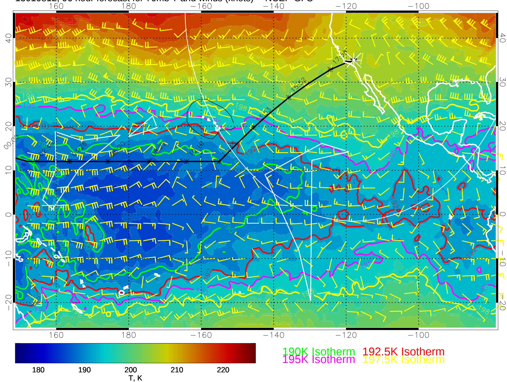
15010812, 96 hour forecast for 70mb T and winds (knots) -- NCEP GFS
