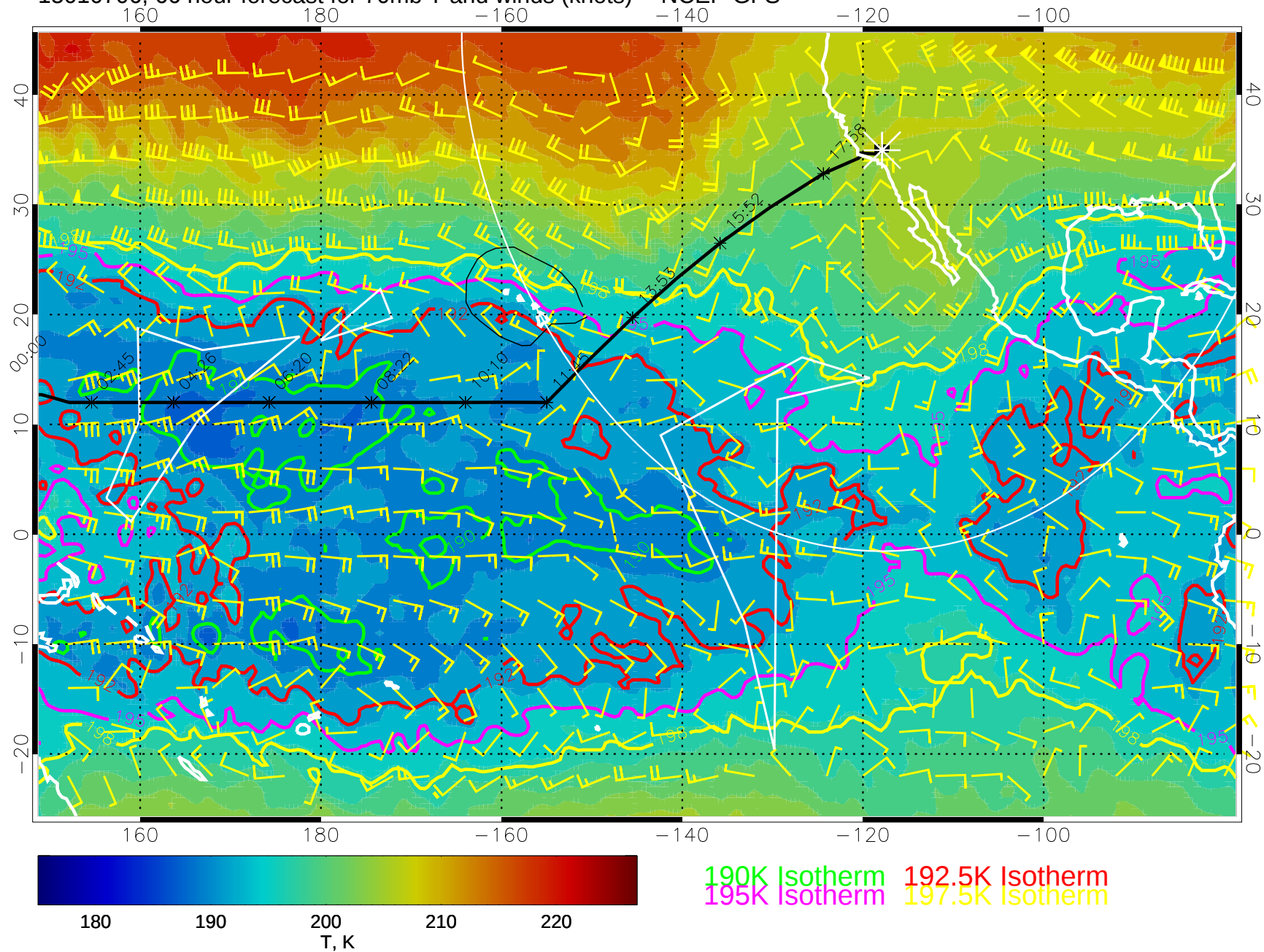
15010706, 66 hour forecast for 70mb T and winds (knots) -- NCEP GFS
