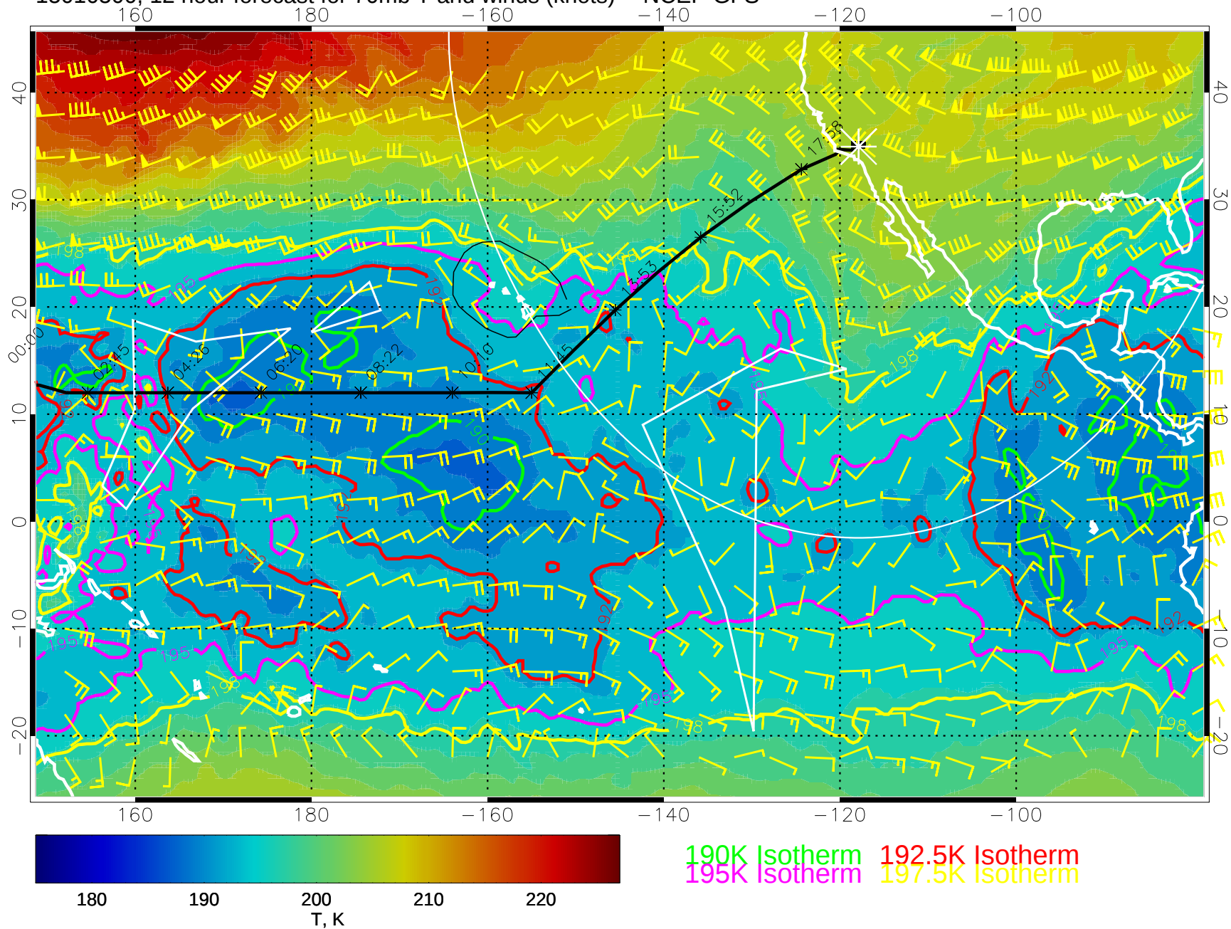
15010500, 12 hour forecast for 70mb T and winds (knots) -- NCEP GFS
