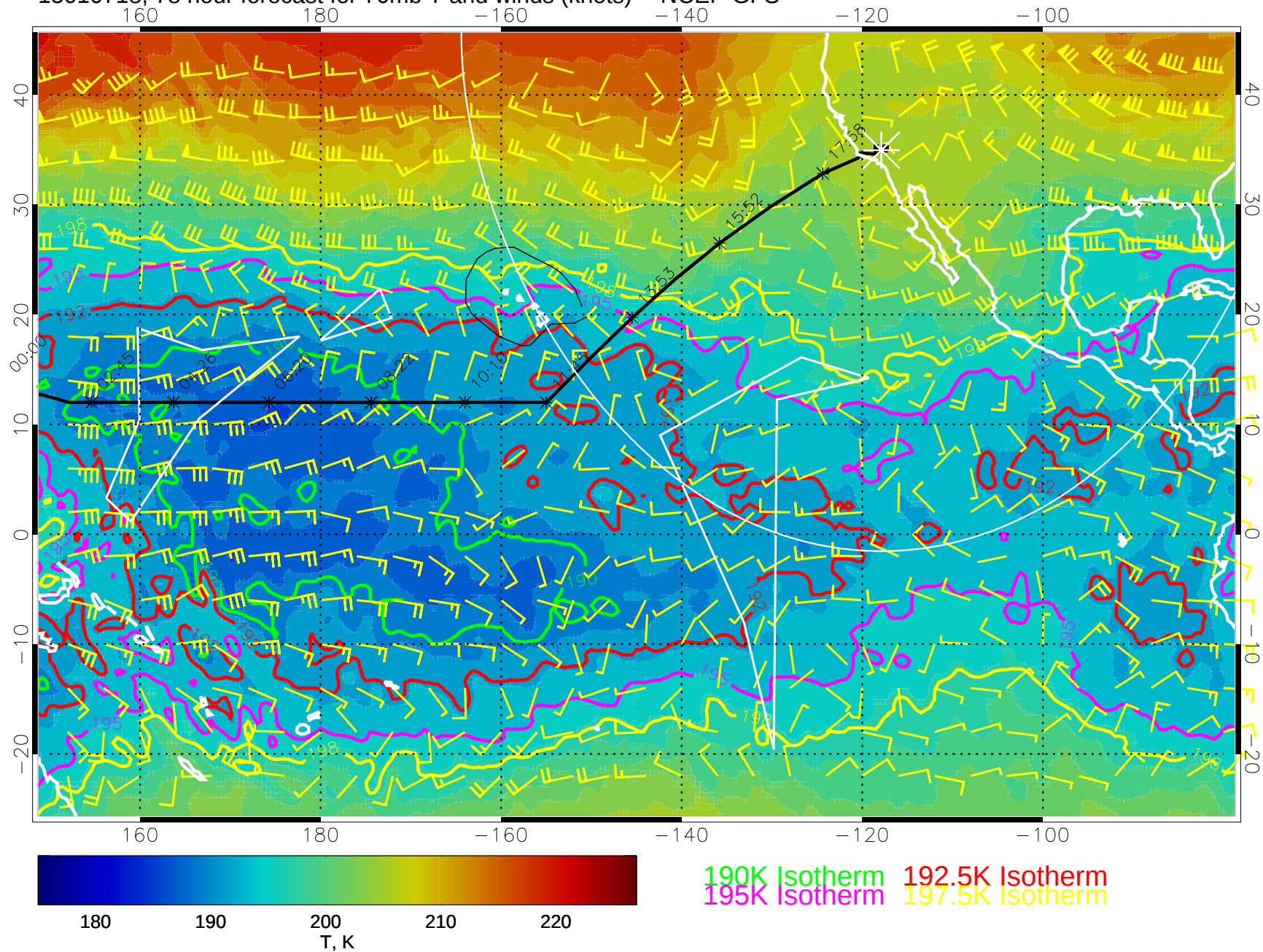
15010718, 78 hour forecast for 70mb T and winds (knots) -- NCEP GFS
