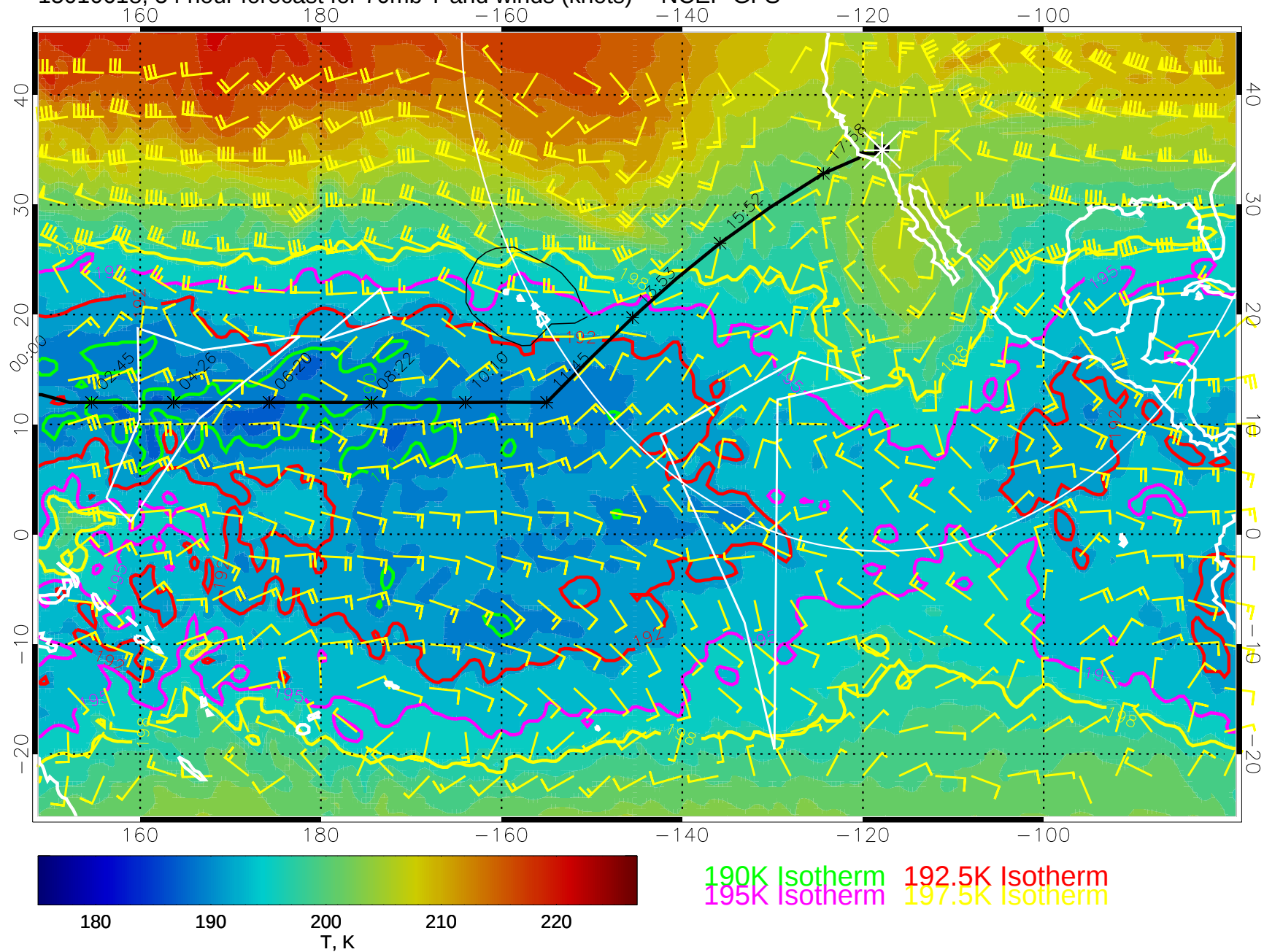
15010618, 54 hour forecast for 70mb T and winds (knots) -- NCEP GFS
