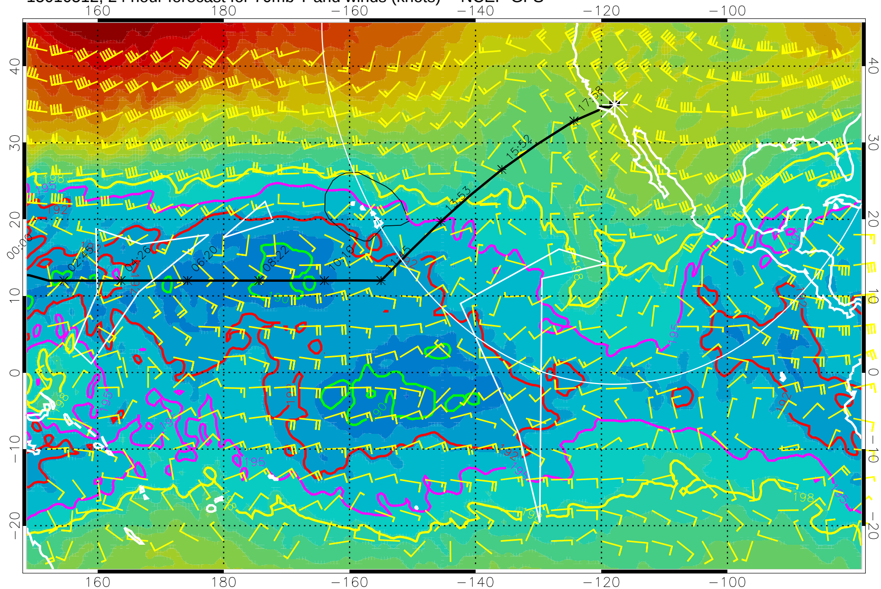
15010512, 24 hour forecast for 70mb T and winds (knots) -- NCEP GFS
