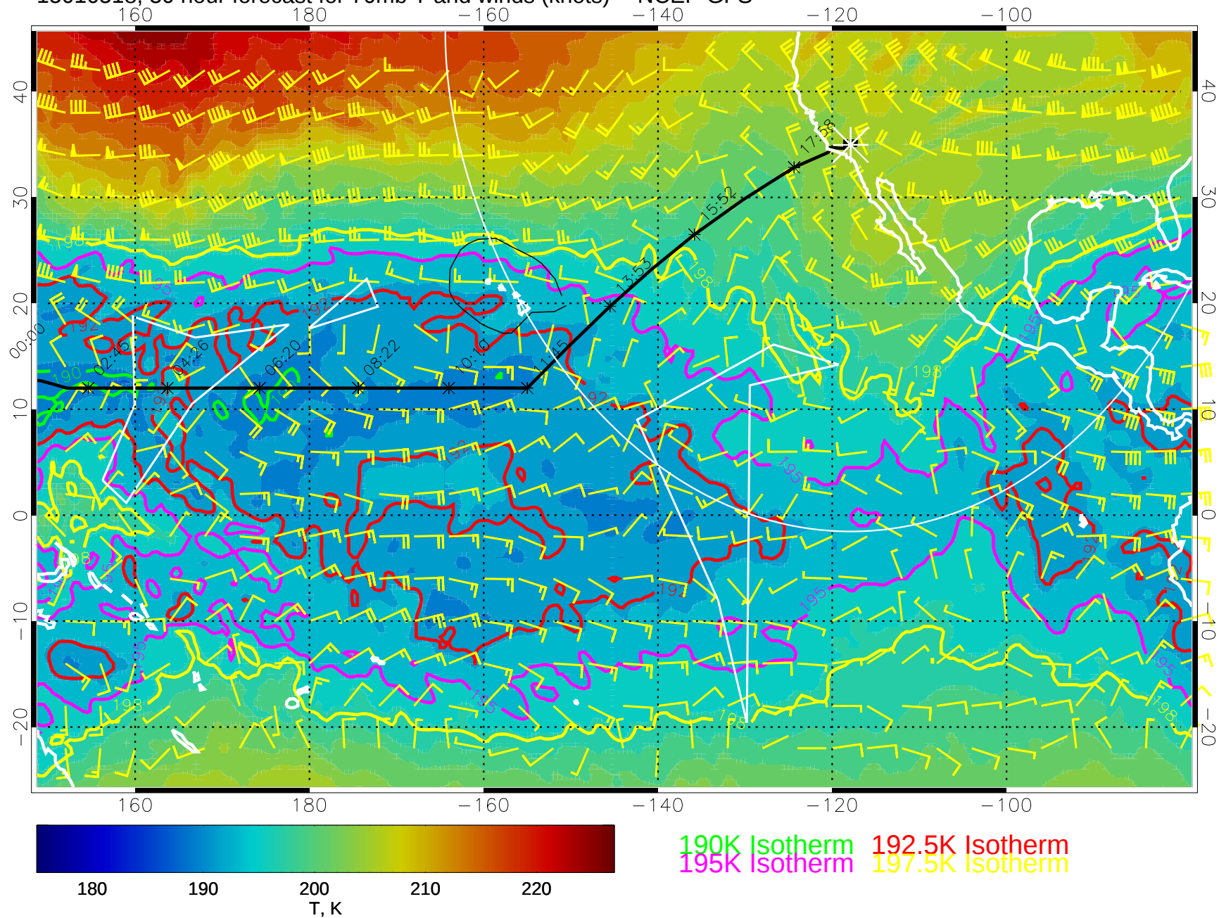
15010518, 30 hour forecast for 70mb T and winds (knots) -- NCEP GFS
