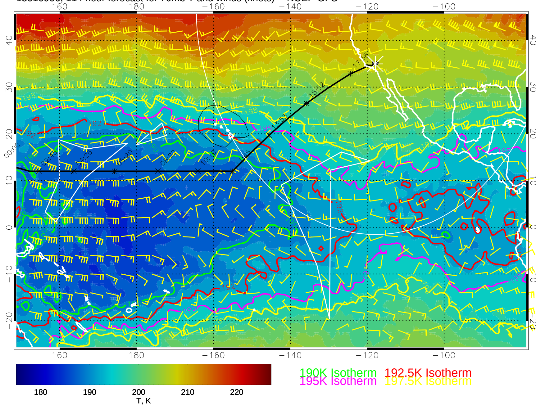
15010906, 114 hour forecast for 70mb T and winds (knots) -- NCEP GFS
