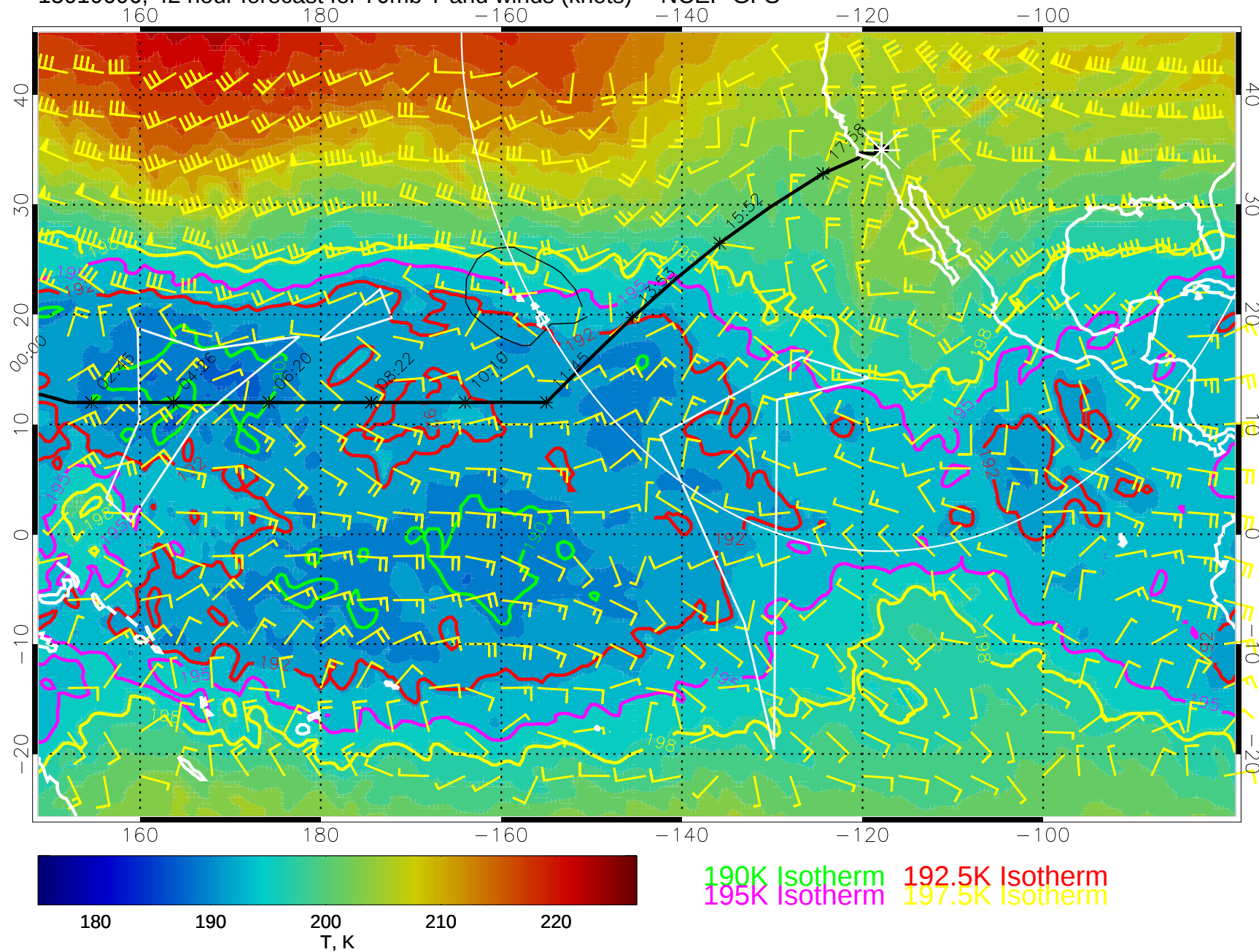
15010606, 42 hour forecast for 70mb T and winds (knots) -- NCEP GFS
