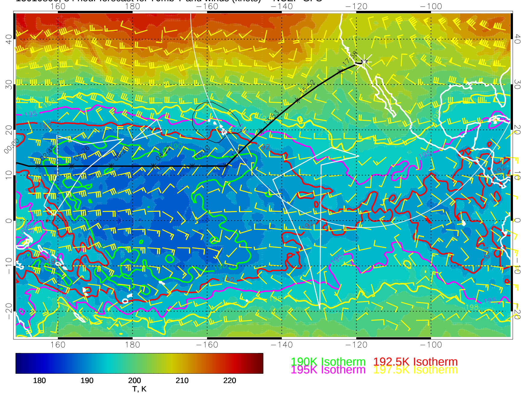
15010800, 84 hour forecast for 70mb T and winds (knots) -- NCEP GFS
