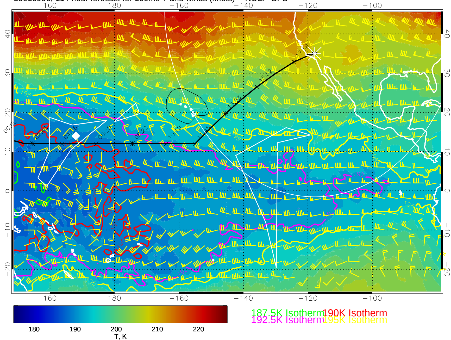
15010906, 114 hour forecast for 100mb T and winds (knots) -- NCEP GFS
