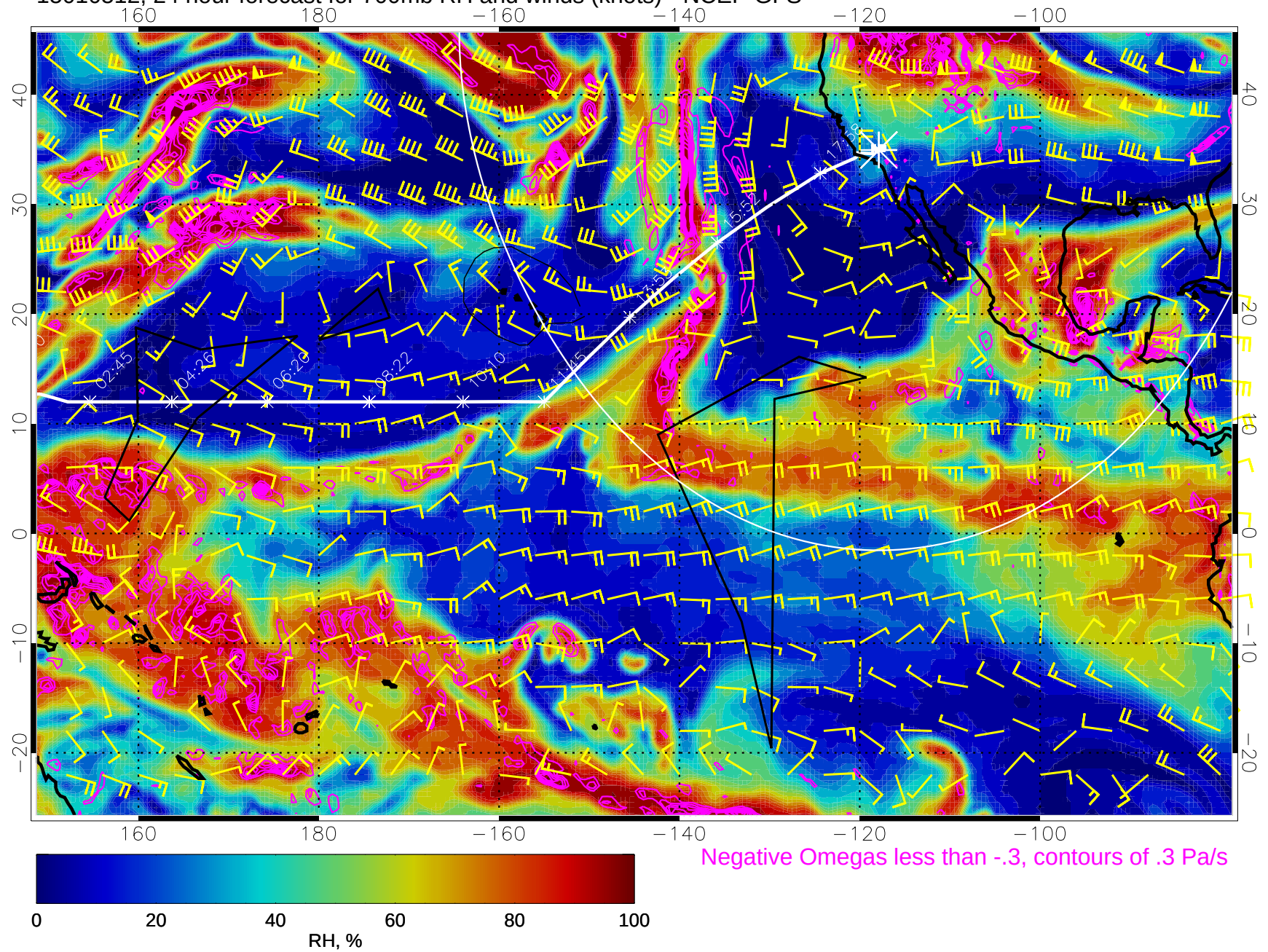
15010512, 24 hour forecast for 700mb RH and winds (knots) - NCEP GFS
