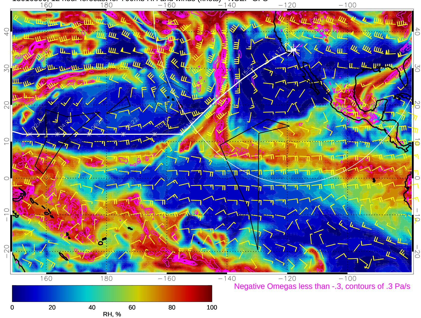
15010500, 12 hour forecast for 700mb RH and winds (knots) - NCEP GFS
