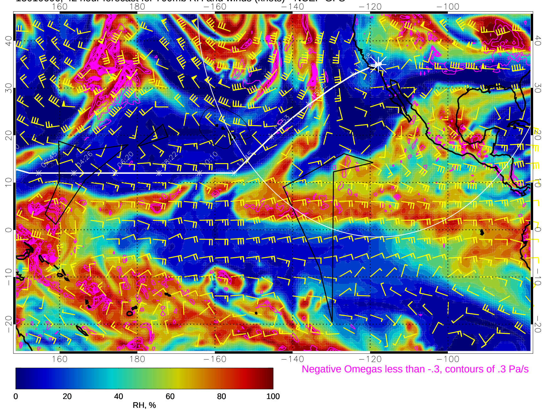
15010606, 42 hour forecast for 700mb RH and winds (knots) - NCEP GFS
