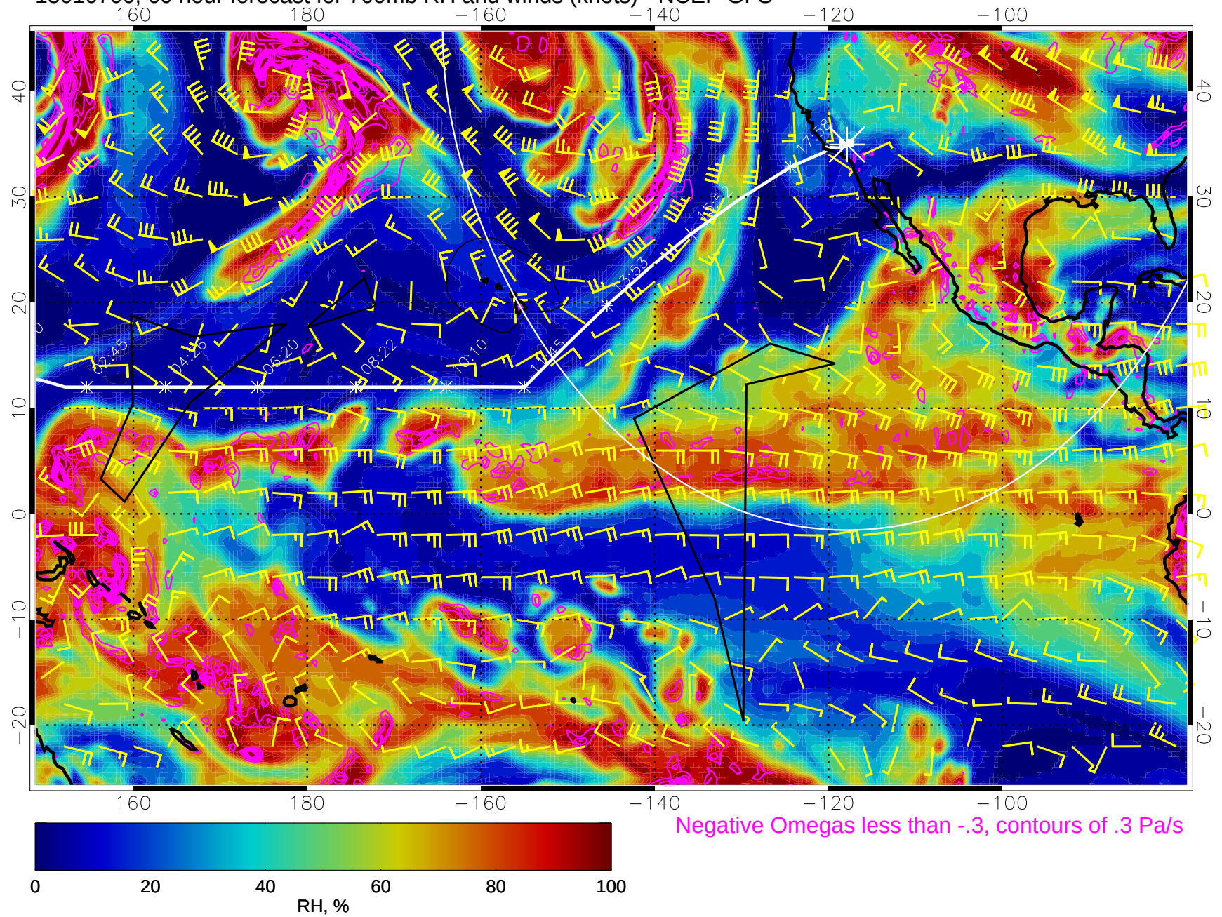
15010700, 60 hour forecast for 700mb RH and winds (knots) - NCEP GFS
