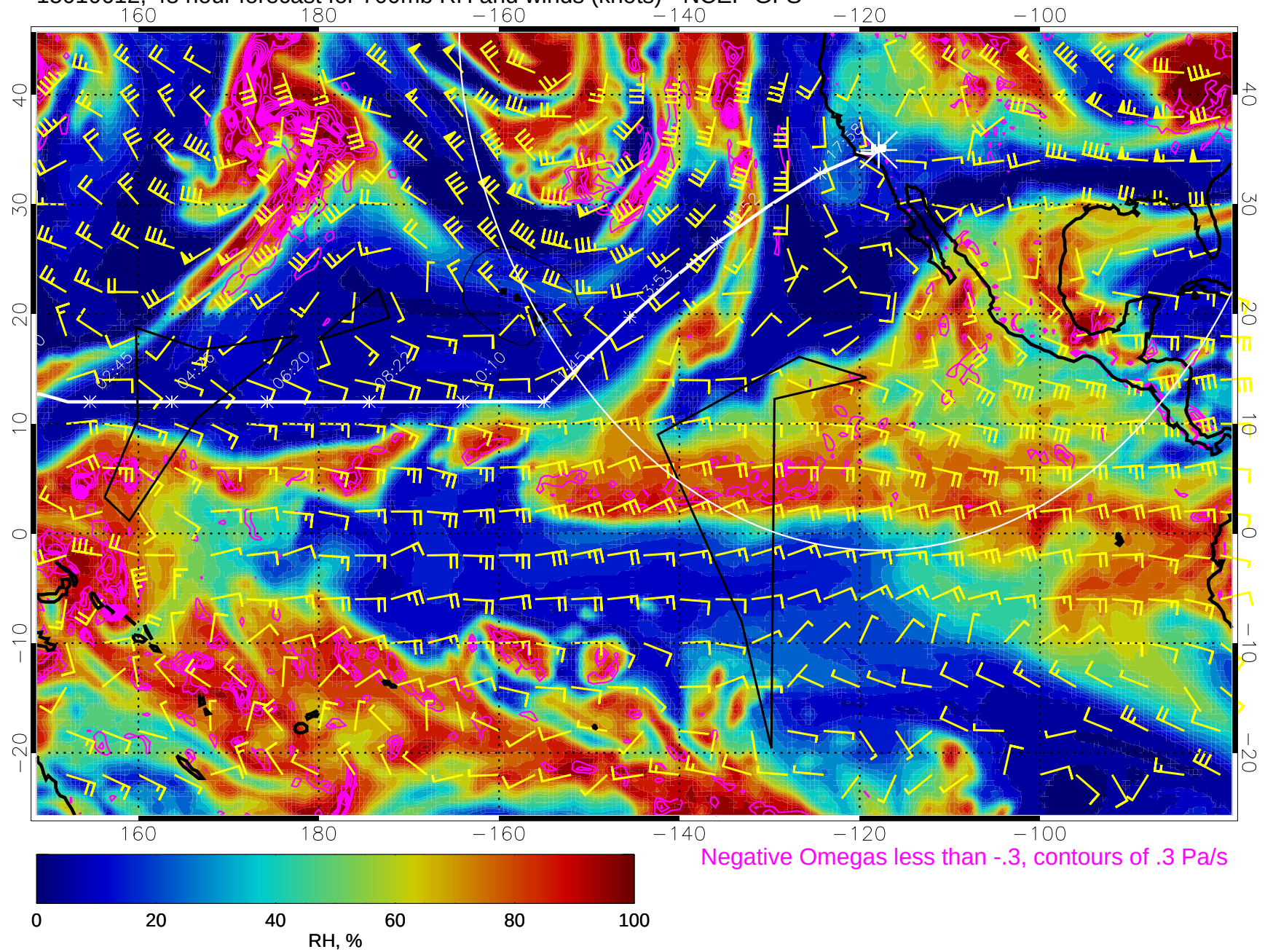
15010612, 48 hour forecast for 700mb RH and winds (knots) - NCEP GFS
