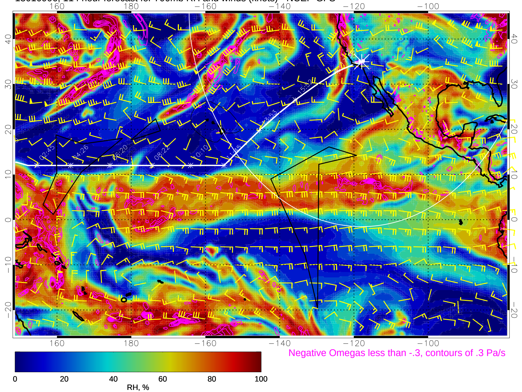
15010906, 114 hour forecast for 700mb RH and winds (knots) - NCEP GFS
