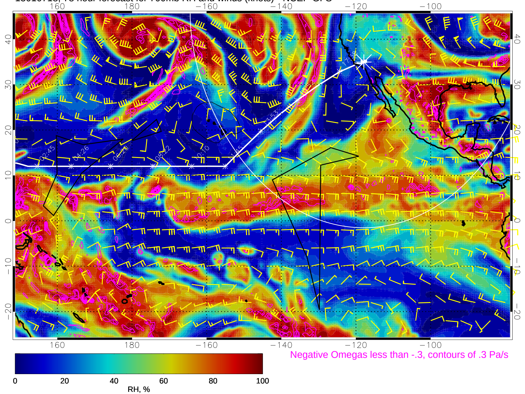
15010718, 78 hour forecast for 700mb RH and winds (knots) - NCEP GFS
