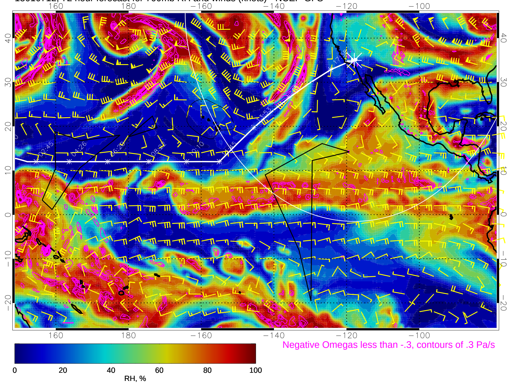
15010712, 72 hour forecast for 700mb RH and winds (knots) - NCEP GFS
