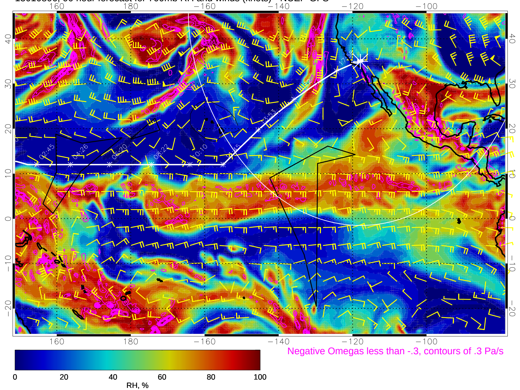
15010806, 90 hour forecast for 700mb RH and winds (knots) - NCEP GFS
