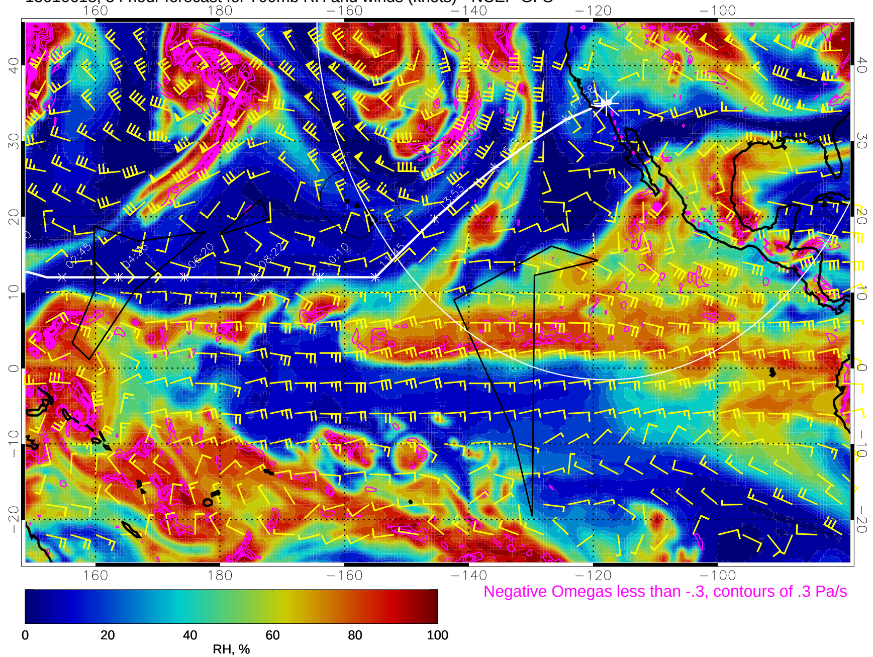
15010618, 54 hour forecast for 700mb RH and winds (knots) - NCEP GFS
