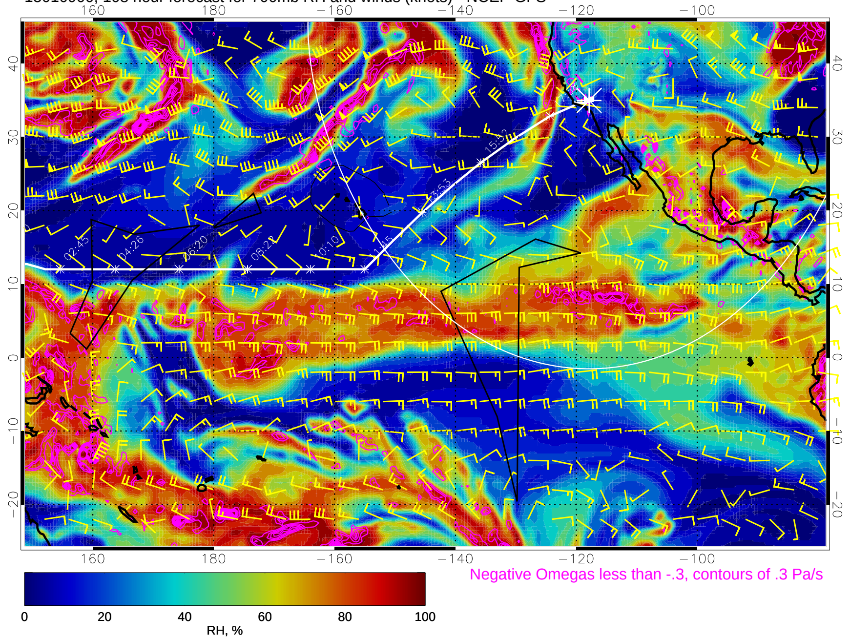
15010900, 108 hour forecast for 700mb RH and winds (knots) - NCEP GFS
