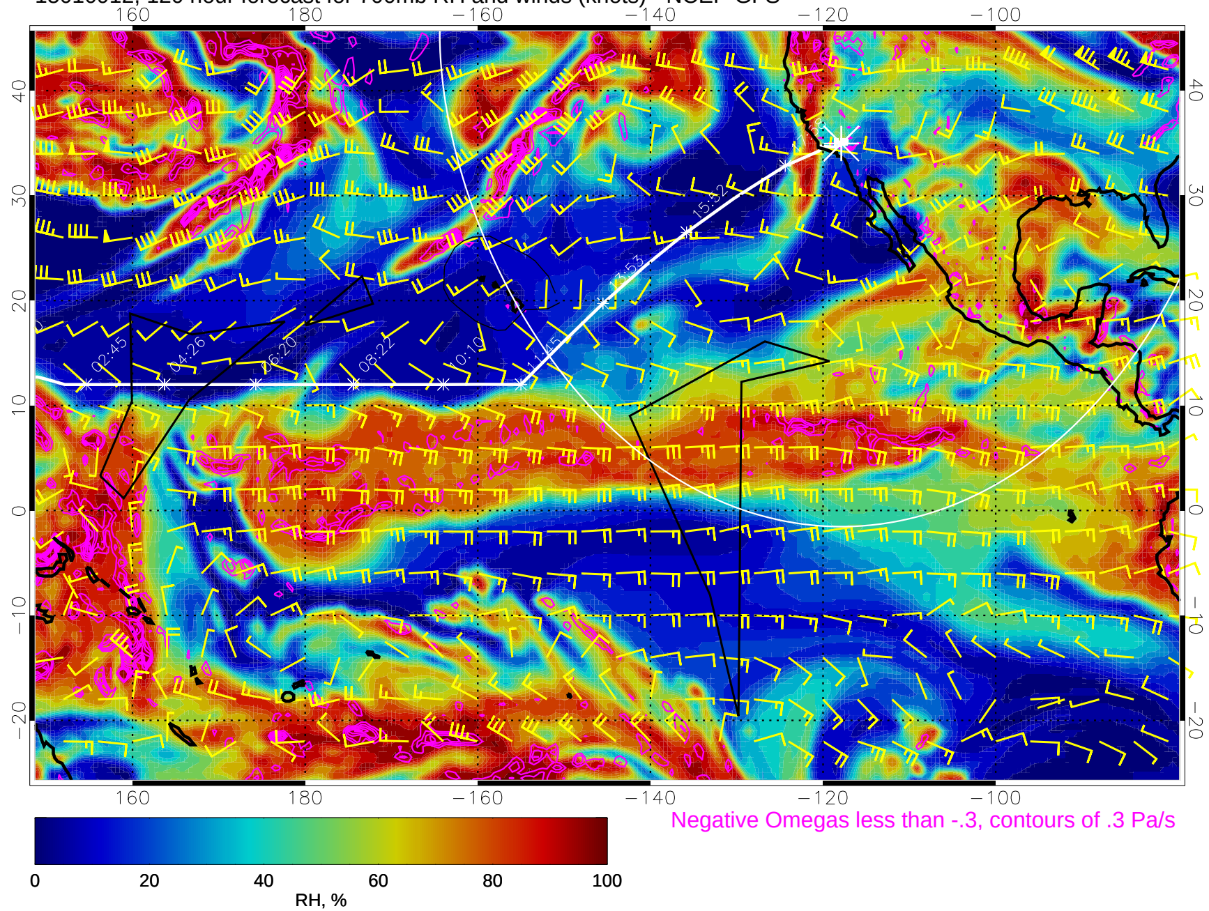
15010912, 120 hour forecast for 700mb RH and winds (knots) - NCEP GFS
