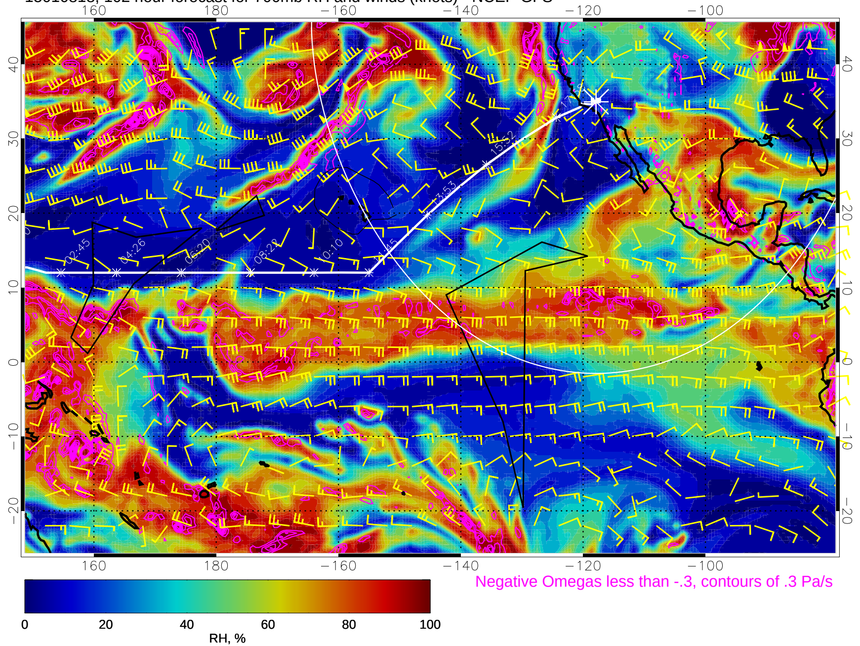
15010818, 102 hour forecast for 700mb RH and winds (knots) - NCEP GFS
