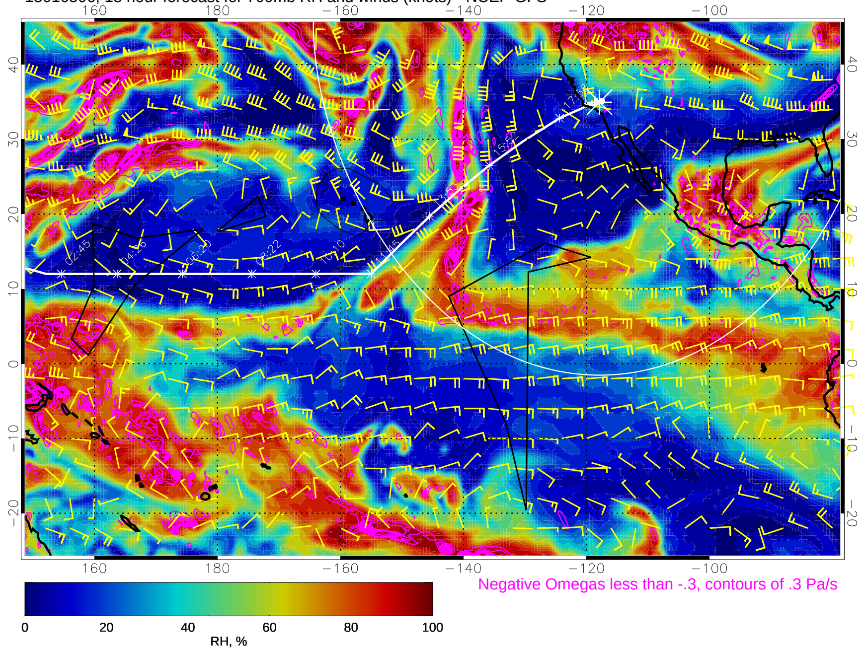
15010506, 18 hour forecast for 700mb RH and winds (knots) - NCEP GFS
