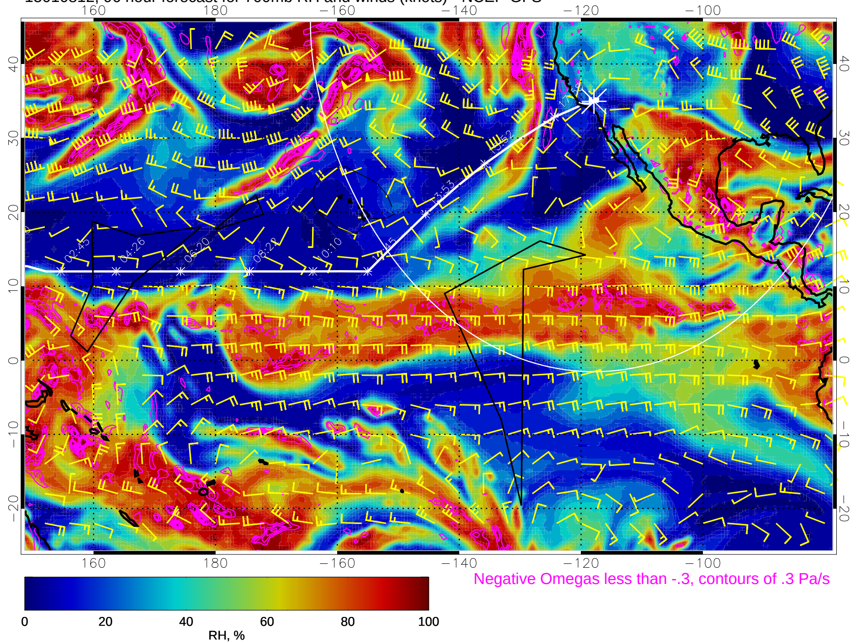
15010812, 96 hour forecast for 700mb RH and winds (knots) - NCEP GFS
