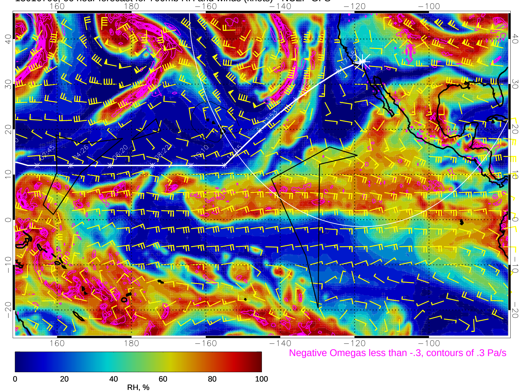
15010706, 66 hour forecast for 700mb RH and winds (knots) - NCEP GFS
