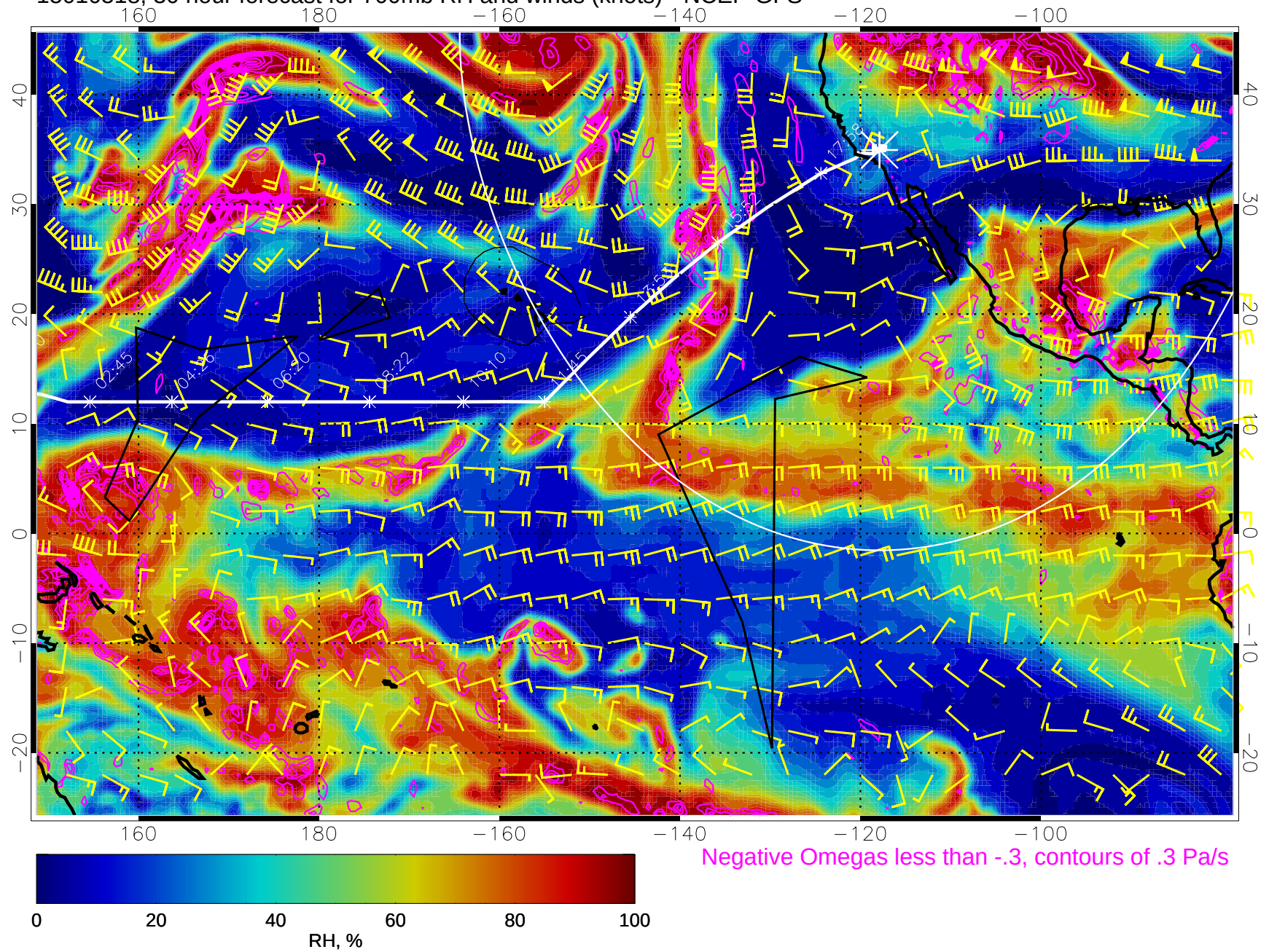
15010518, 30 hour forecast for 700mb RH and winds (knots) - NCEP GFS
