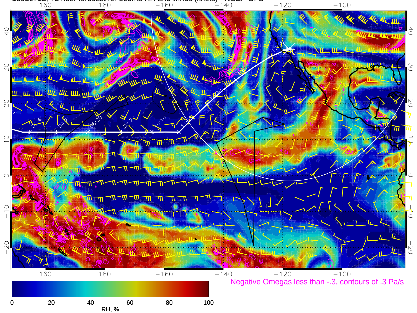
15010712, 72 hour forecast for 500mb RH and winds (knots) - NCEP GFS
