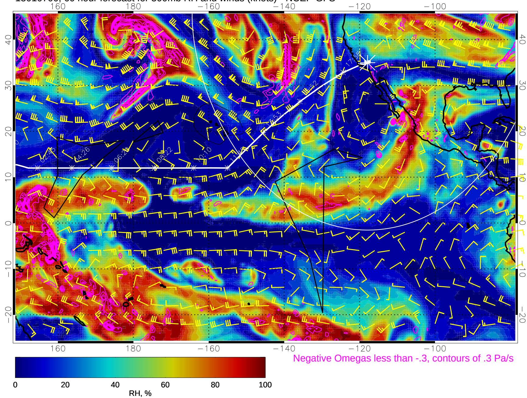
15010700, 60 hour forecast for 500mb RH and winds (knots) - NCEP GFS
