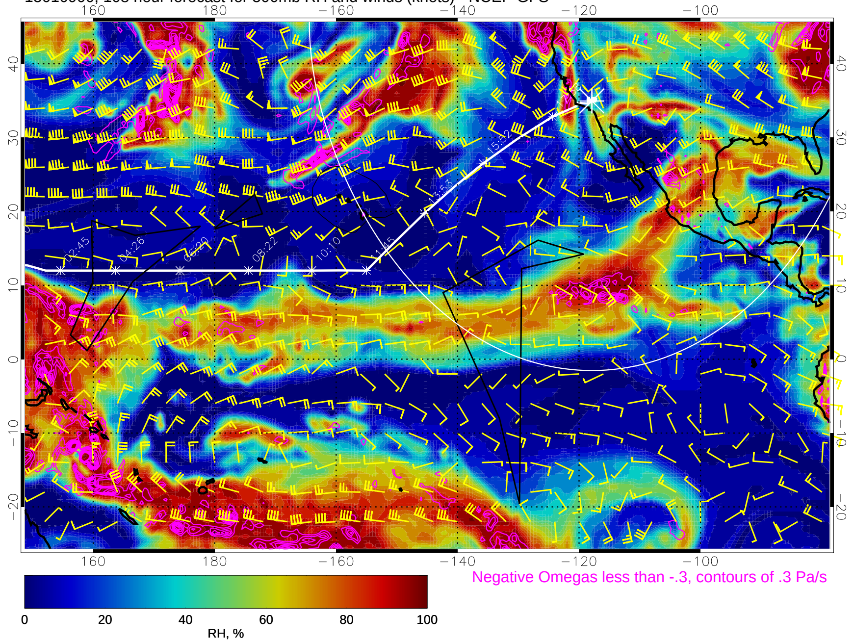
15010900, 108 hour forecast for 500mb RH and winds (knots) - NCEP GFS
