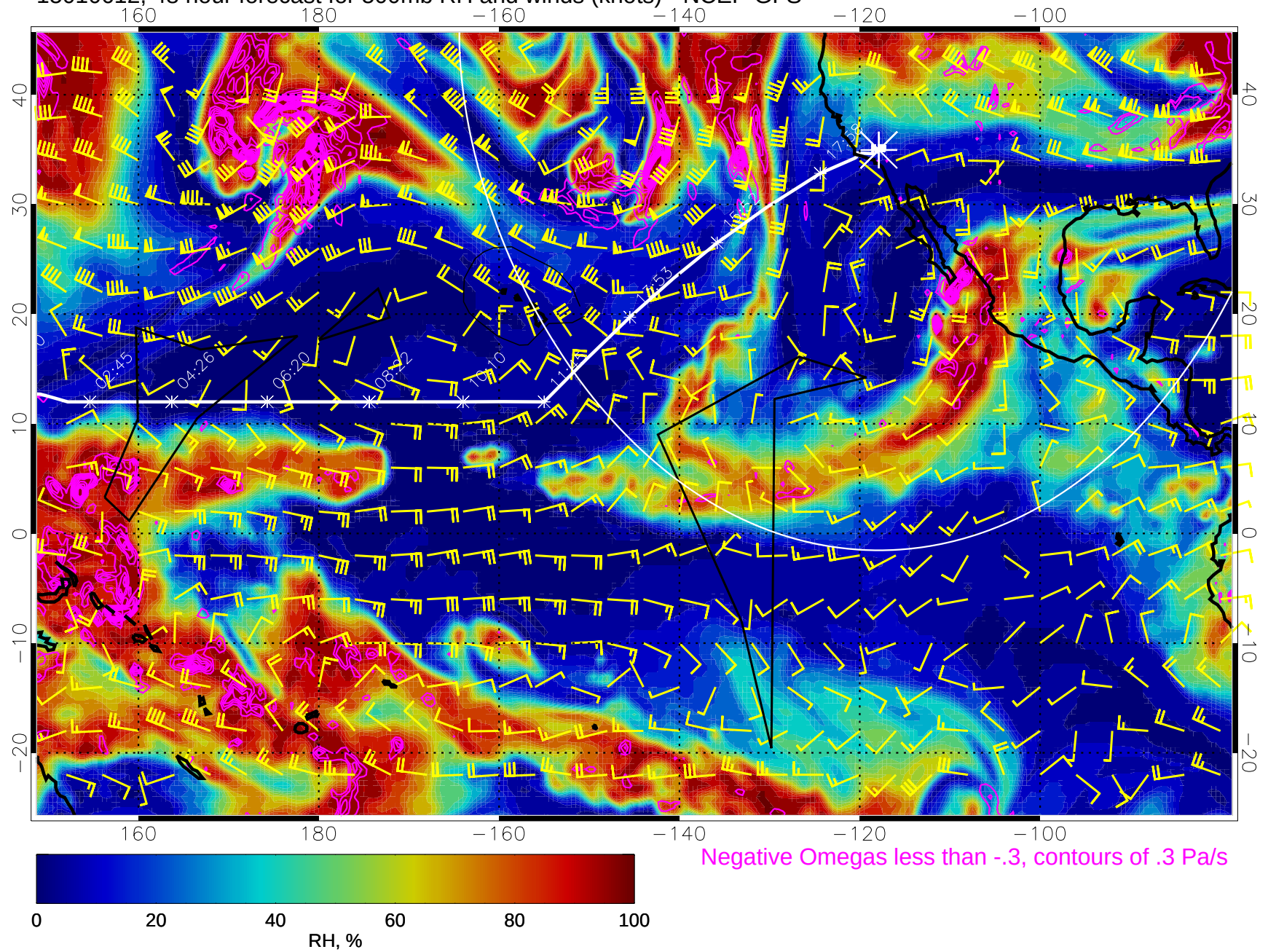
15010612, 48 hour forecast for 500mb RH and winds (knots) - NCEP GFS
