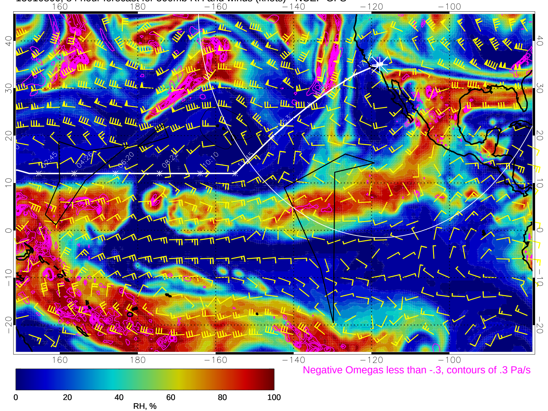
15010800, 84 hour forecast for 500mb RH and winds (knots) - NCEP GFS
