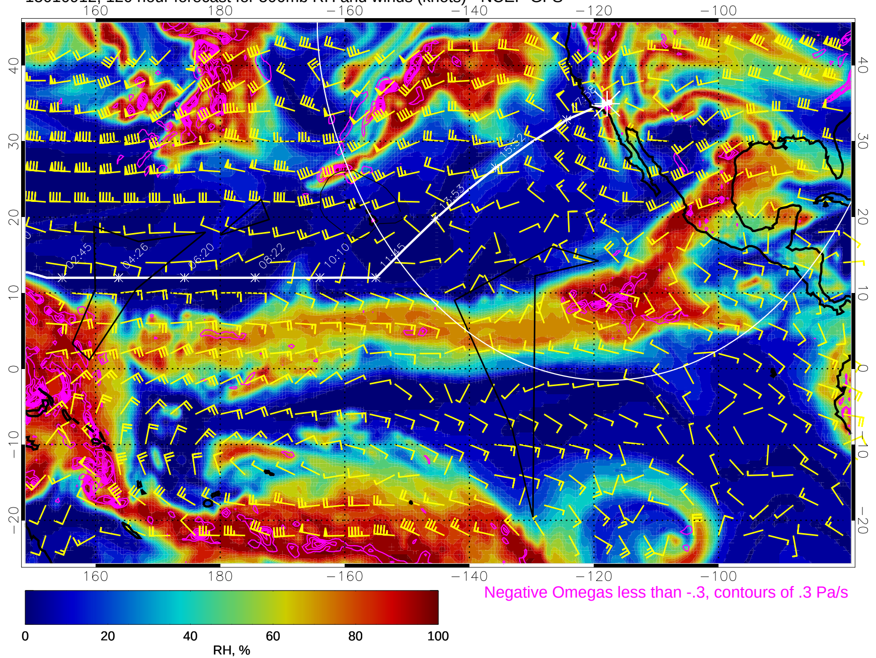
15010912, 120 hour forecast for 500mb RH and winds (knots) - NCEP GFS
