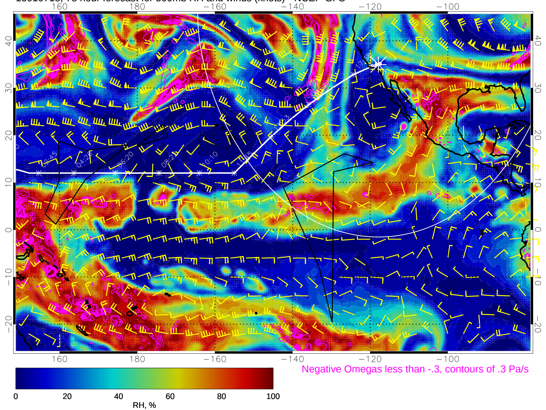
15010718, 78 hour forecast for 500mb RH and winds (knots) - NCEP GFS
