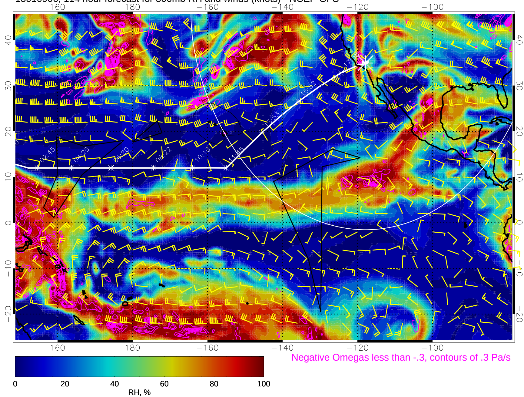
15010906, 114 hour forecast for 500mb RH and winds (knots) - NCEP GFS
