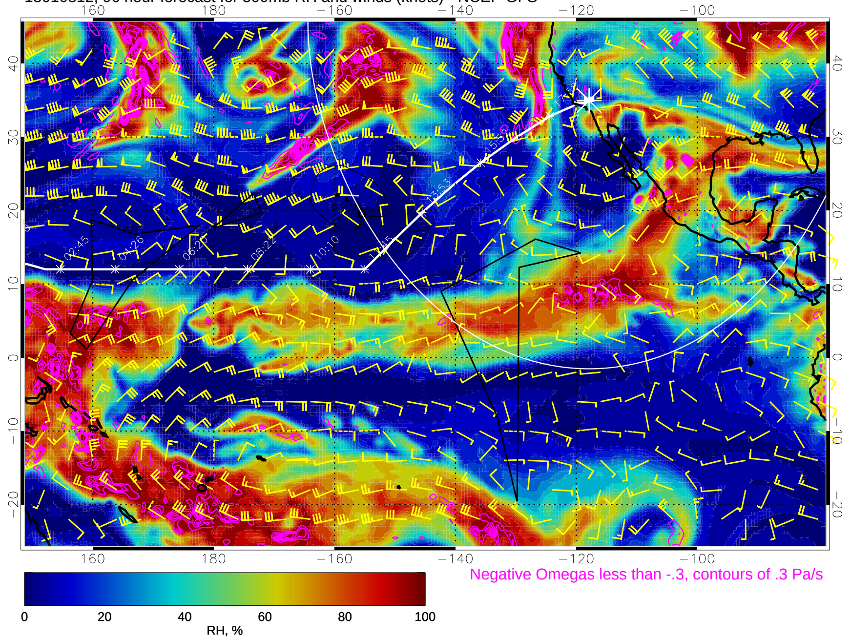
15010812, 96 hour forecast for 500mb RH and winds (knots) - NCEP GFS
