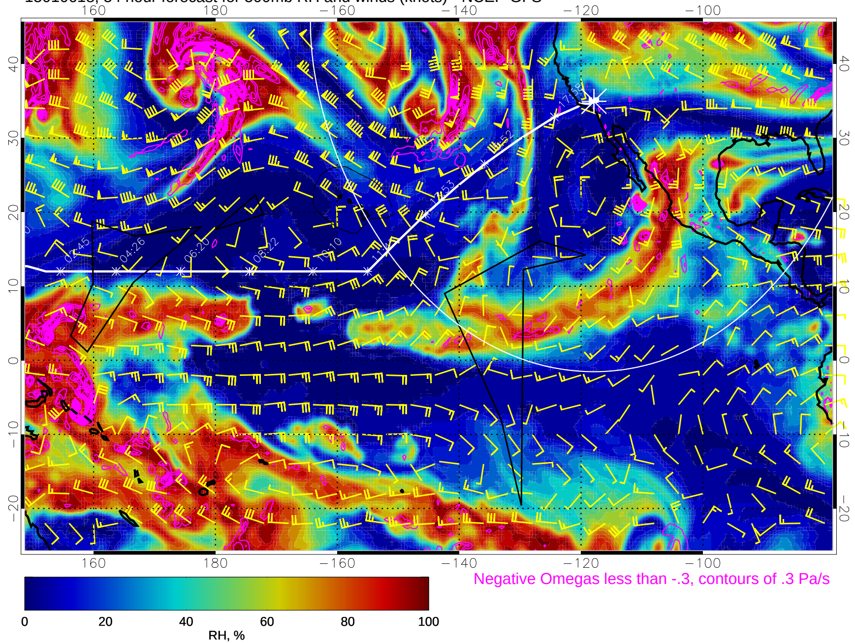
15010618, 54 hour forecast for 500mb RH and winds (knots) - NCEP GFS
