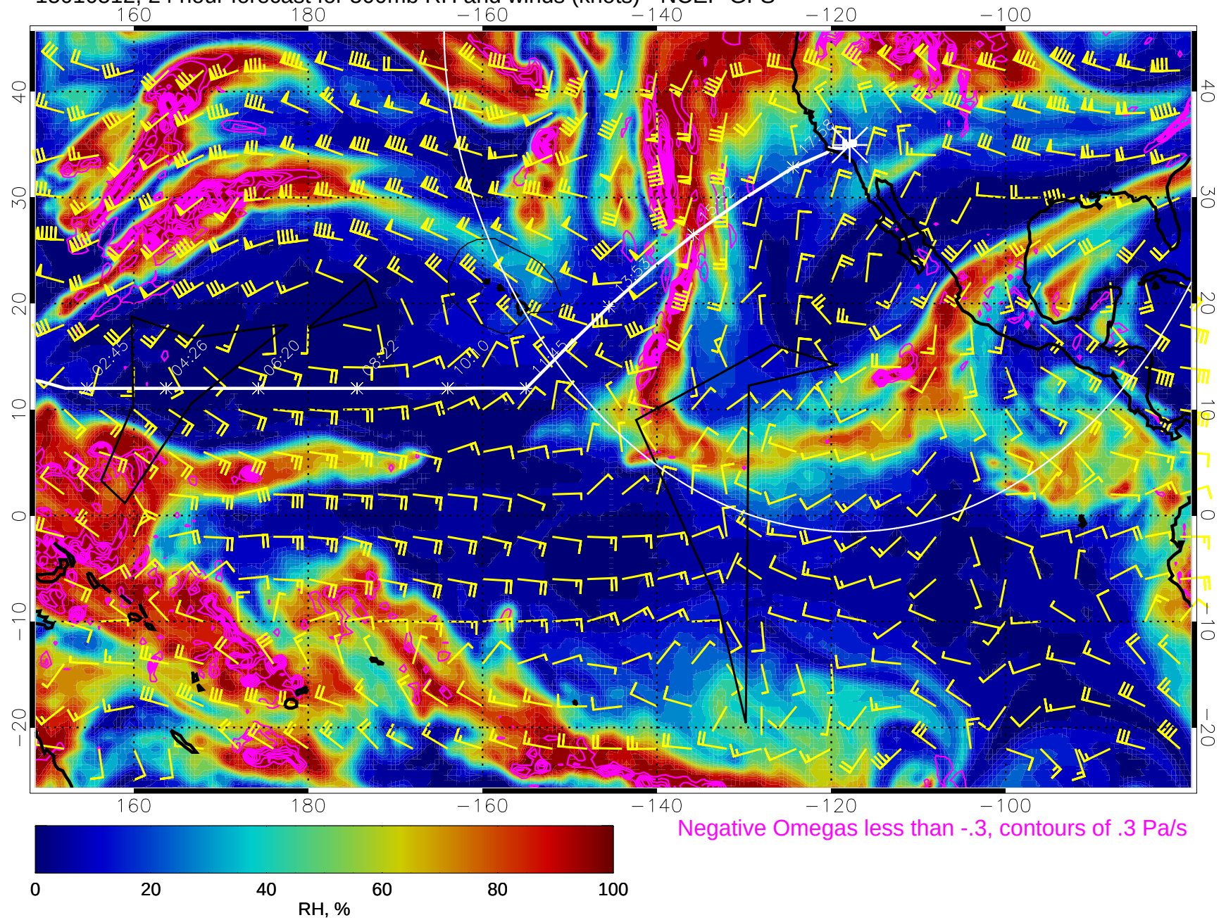
15010512, 24 hour forecast for 500mb RH and winds (knots) - NCEP GFS
