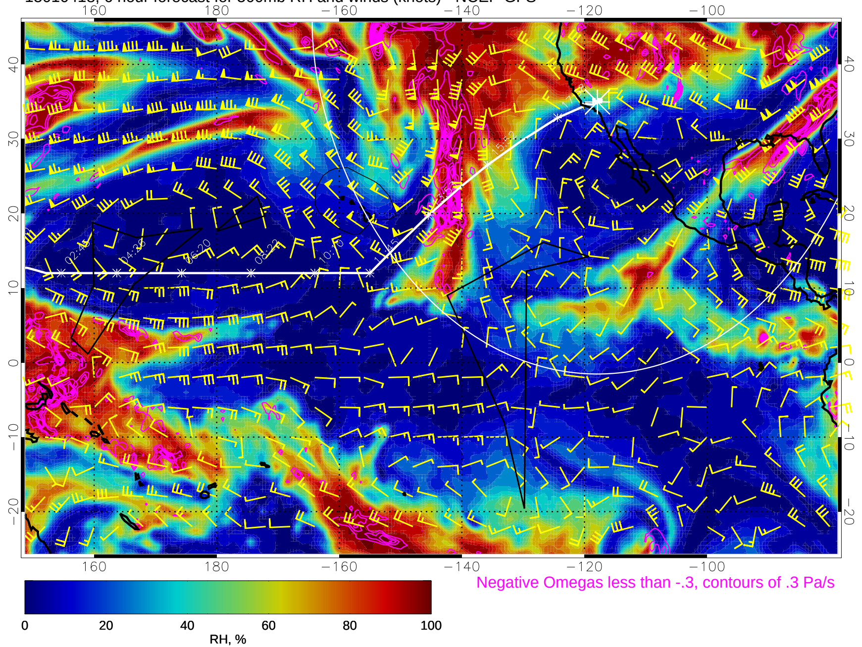
15010418, 6 hour forecast for 500mb RH and winds (knots) - NCEP GFS
