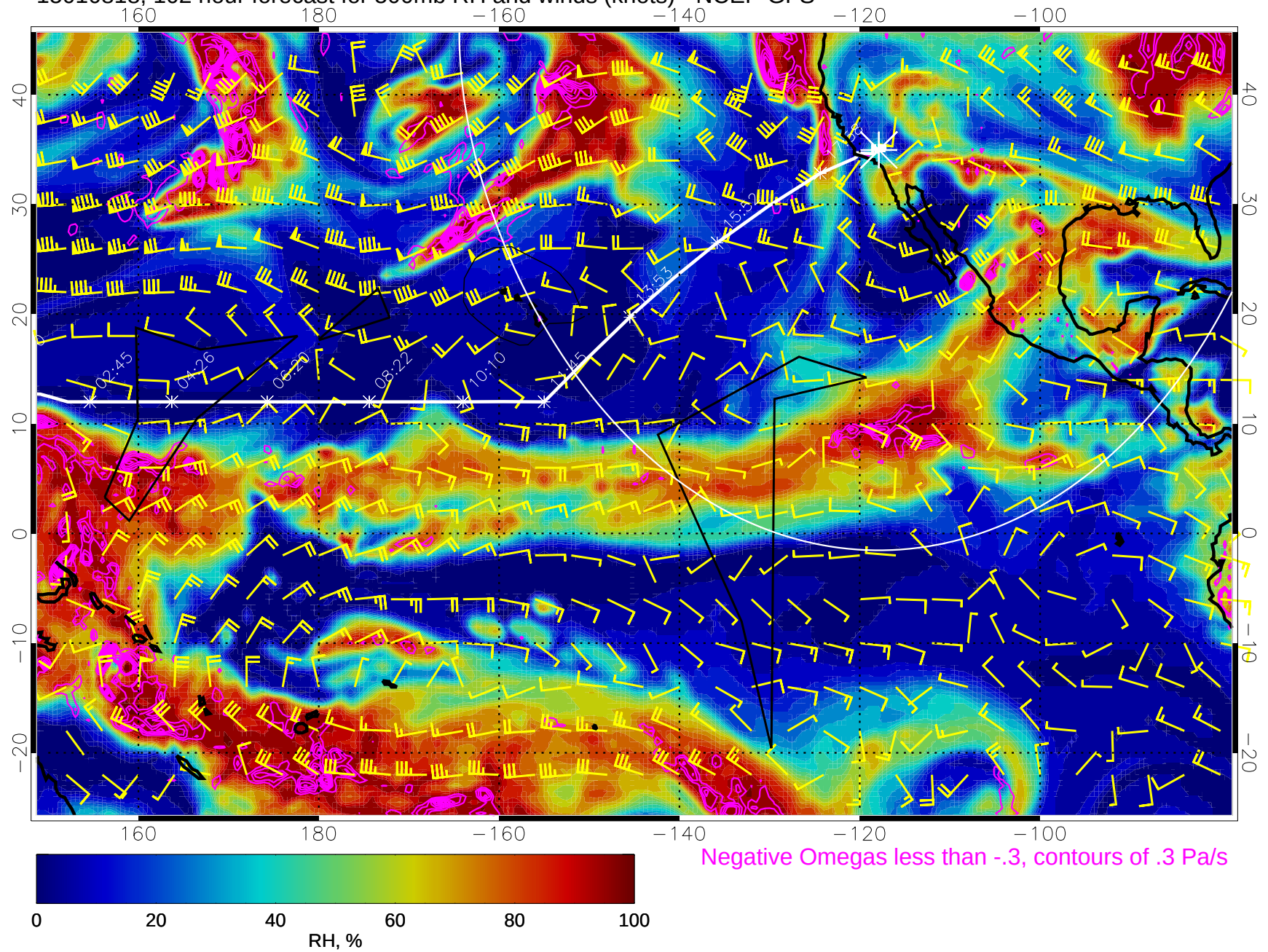
15010818, 102 hour forecast for 500mb RH and winds (knots) - NCEP GFS
