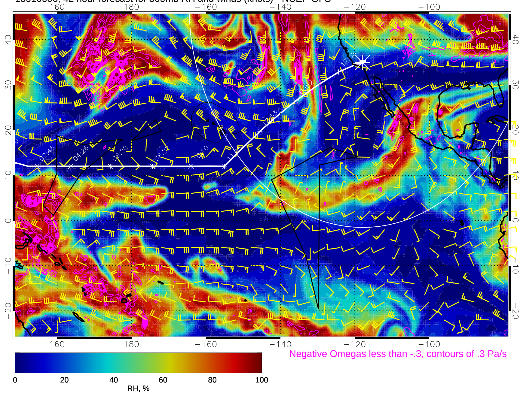
15010606, 42 hour forecast for 500mb RH and winds (knots) - NCEP GFS
