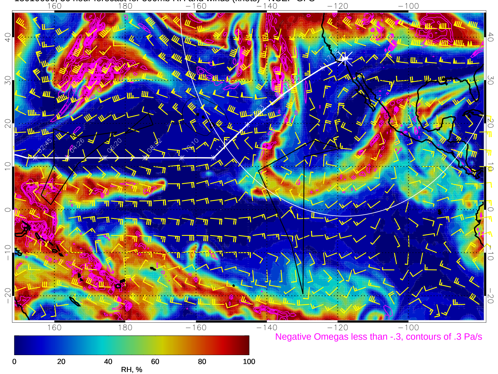
15010600, 36 hour forecast for 500mb RH and winds (knots) - NCEP GFS
