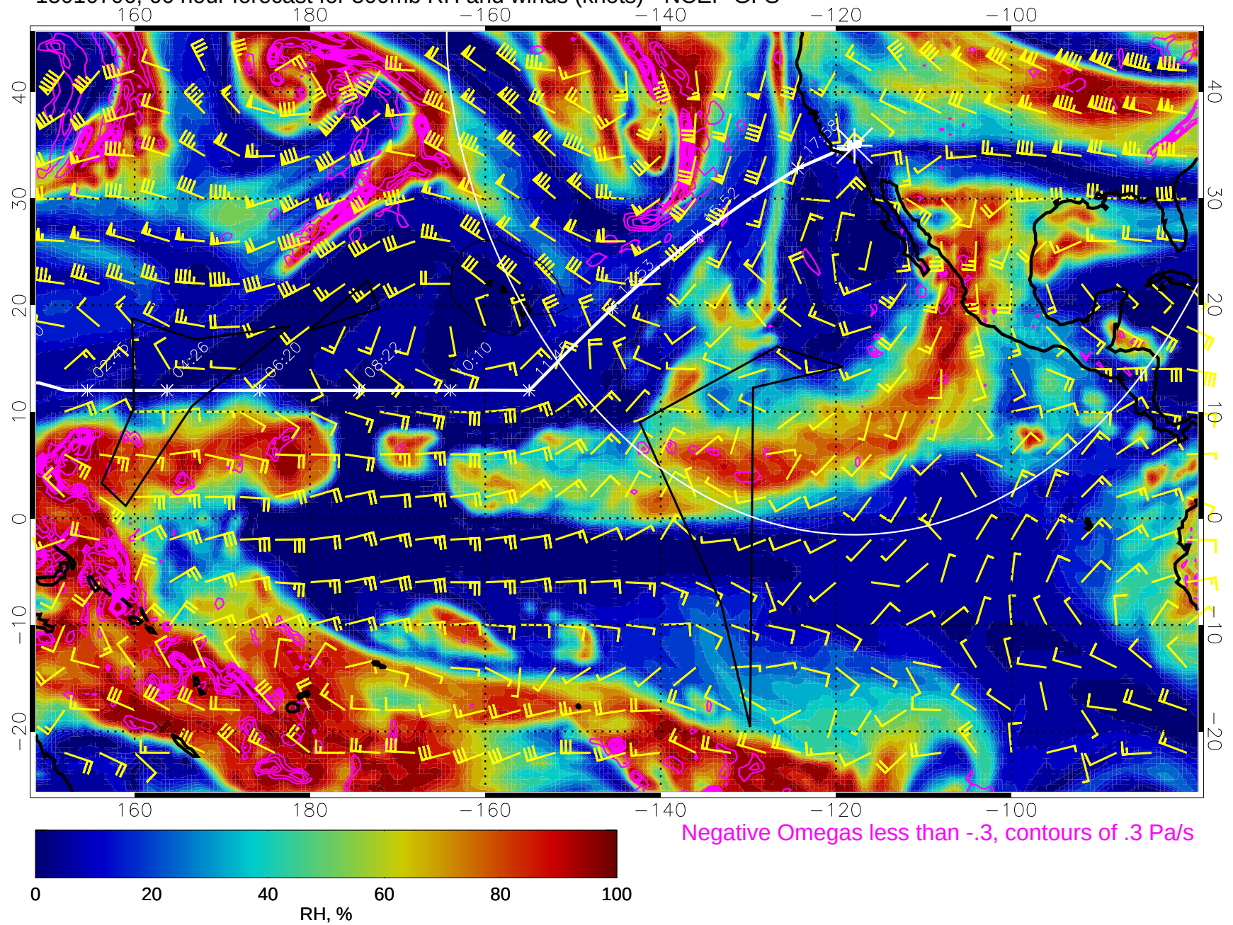
15010706, 66 hour forecast for 500mb RH and winds (knots) - NCEP GFS
