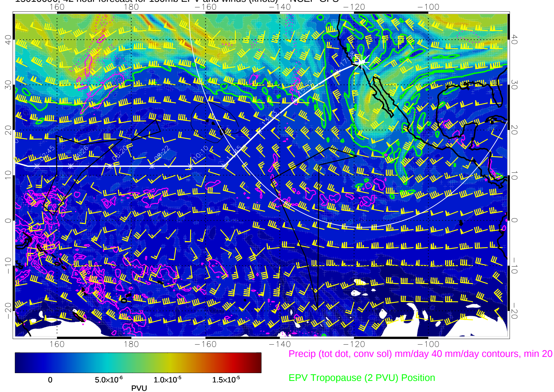
15010606, 42 hour forecast for 150mb EPV and winds (knots) -- NCEP GFS
