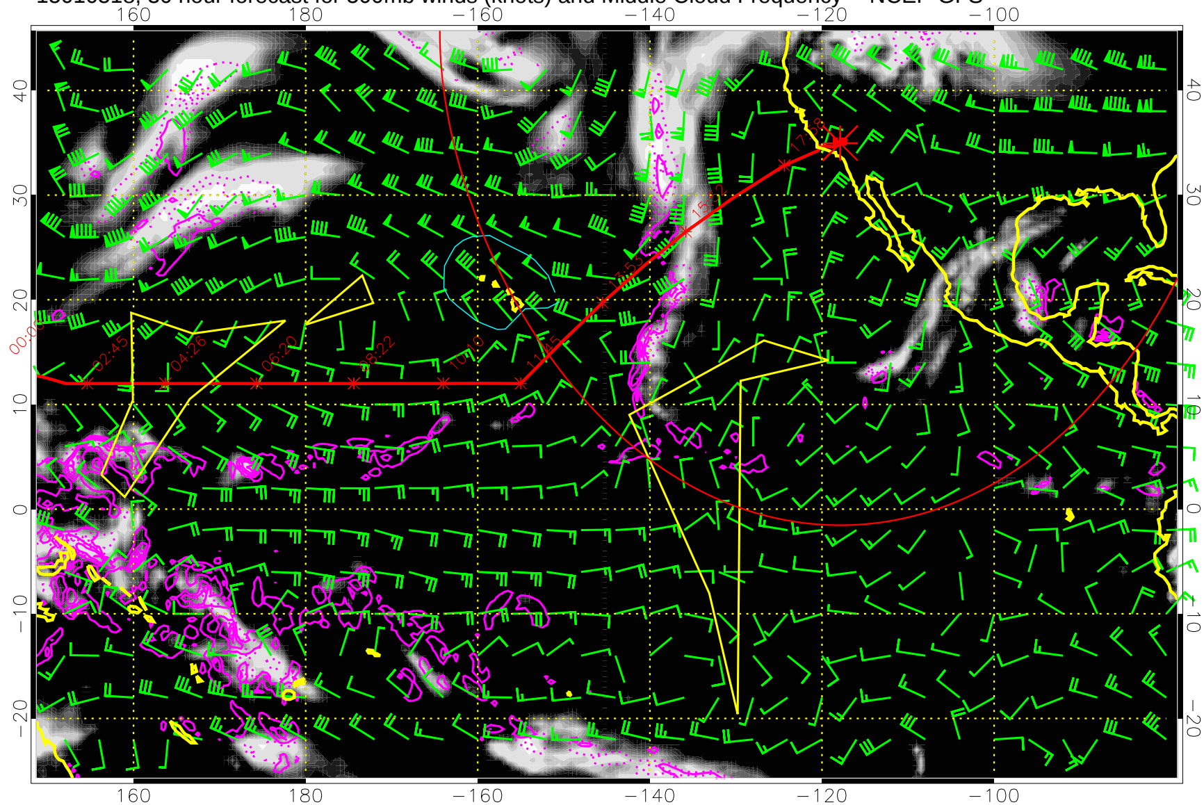
15010518, 30 hour forecast for 500mb winds (knots) and Middle Cloud Frequency -- NCEP GFS
