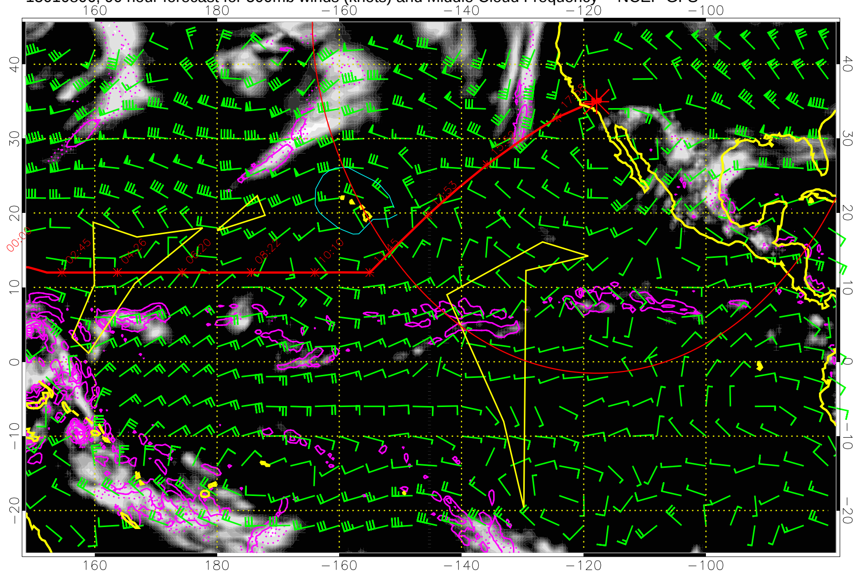
15010806, 90 hour forecast for 500mb winds (knots) and Middle Cloud Frequency -- NCEP GFS
