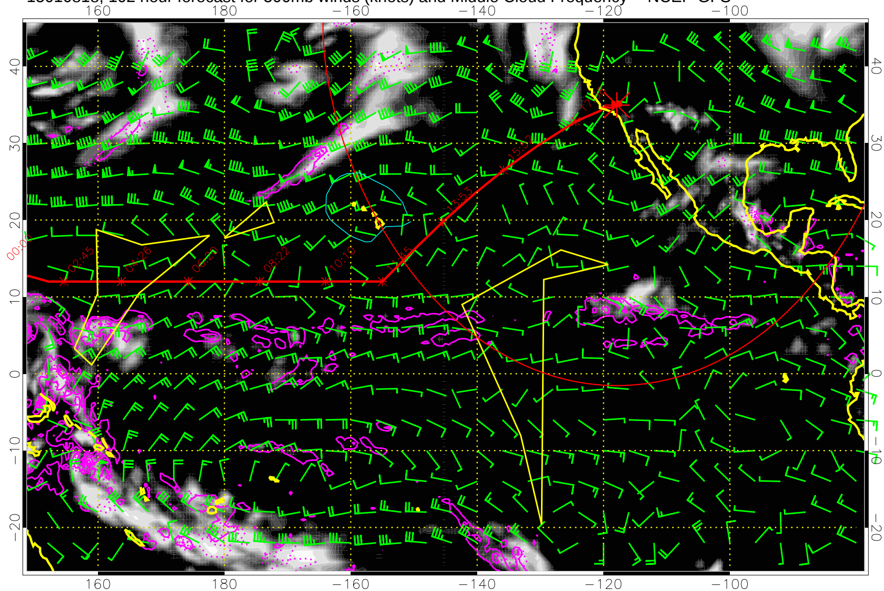
15010818, 102 hour forecast for 500mb winds (knots) and Middle Cloud Frequency -- NCEP GFS
