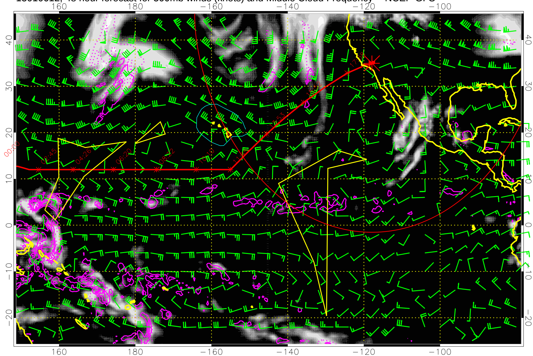
15010612, 48 hour forecast for 500mb winds (knots) and Middle Cloud Frequency -- NCEP GFS
