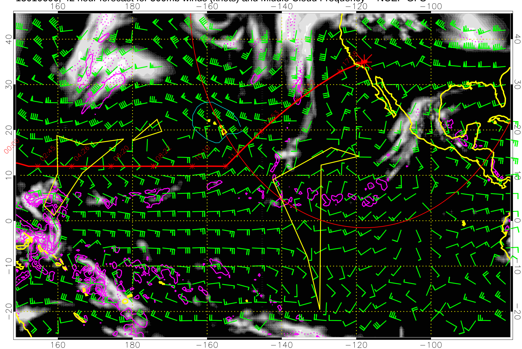
15010606, 42 hour forecast for 500mb winds (knots) and Middle Cloud Frequency -- NCEP GFS
