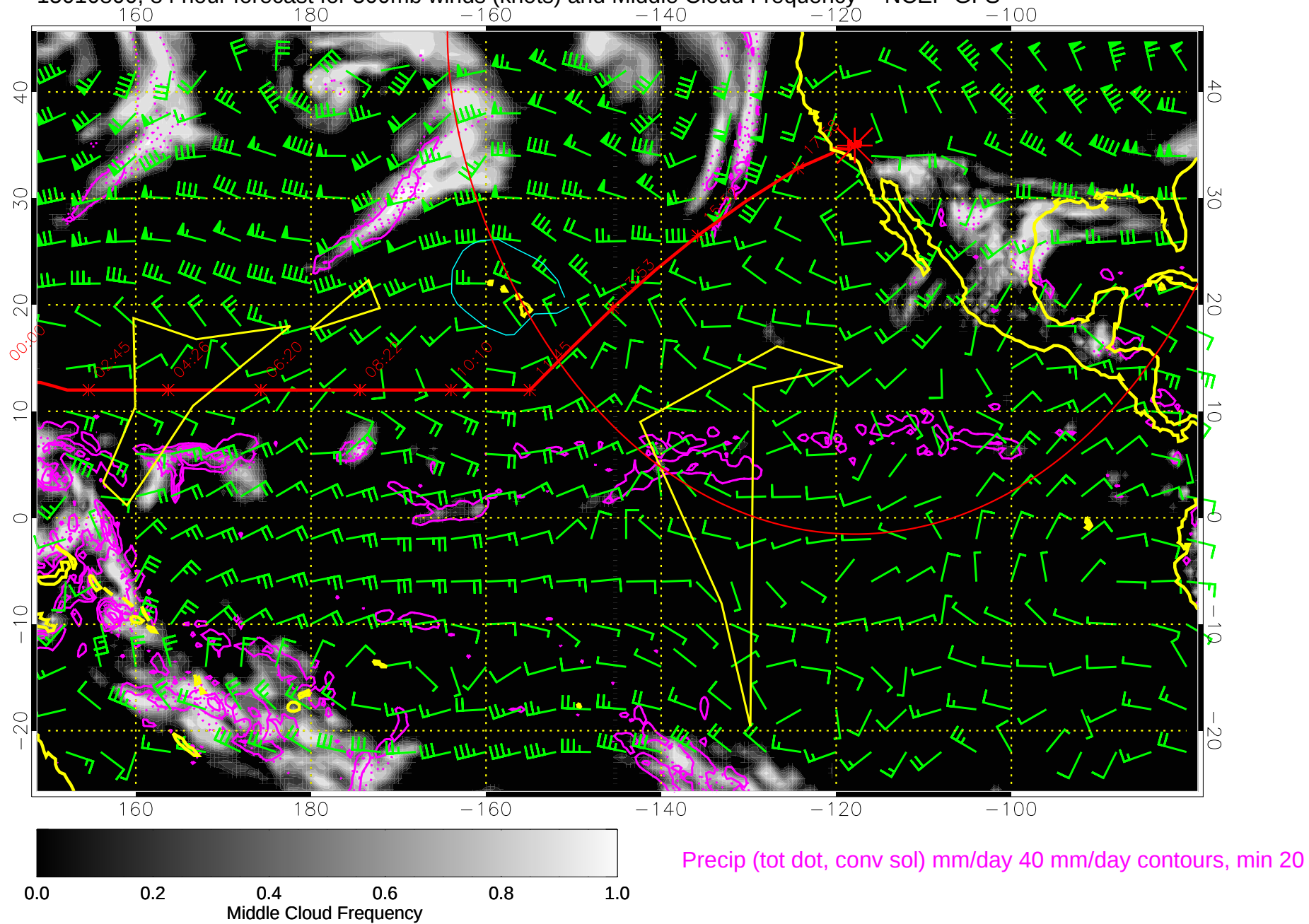
15010800, 84 hour forecast for 500mb winds (knots) and Middle Cloud Frequency -- NCEP GFS
