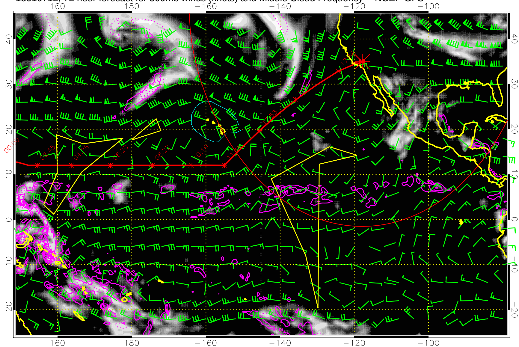
15010712, 72 hour forecast for 500mb winds (knots) and Middle Cloud Frequency -- NCEP GFS
