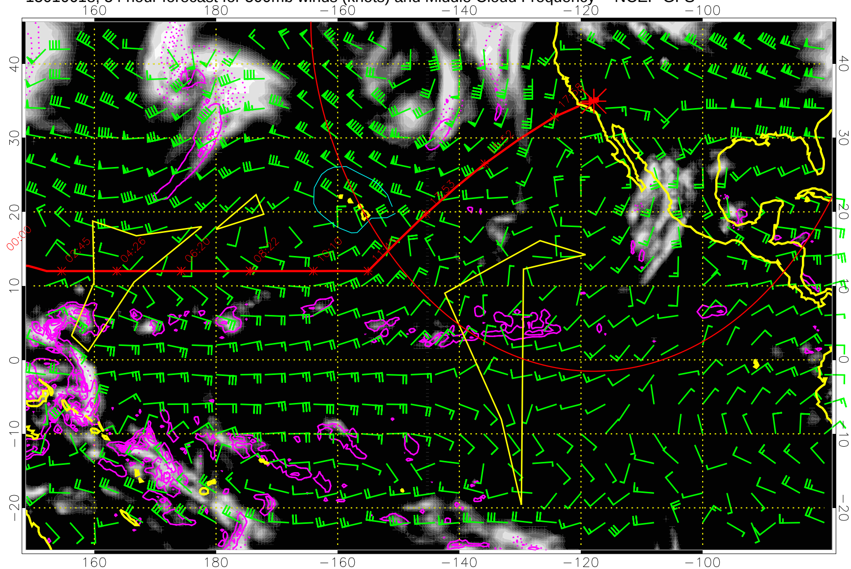
15010618, 54 hour forecast for 500mb winds (knots) and Middle Cloud Frequency -- NCEP GFS
