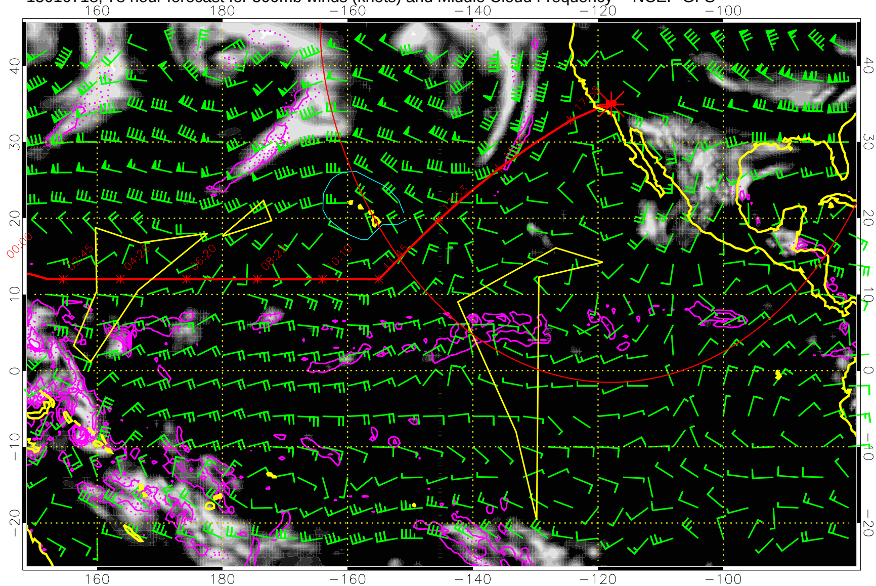
15010718, 78 hour forecast for 500mb winds (knots) and Middle Cloud Frequency -- NCEP GFS
