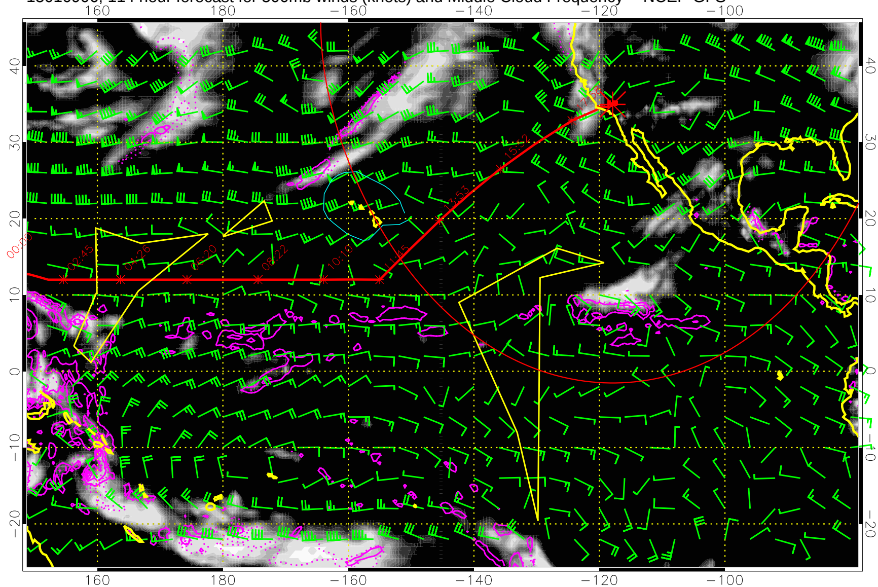
15010906, 114 hour forecast for 500mb winds (knots) and Middle Cloud Frequency -- NCEP GFS
