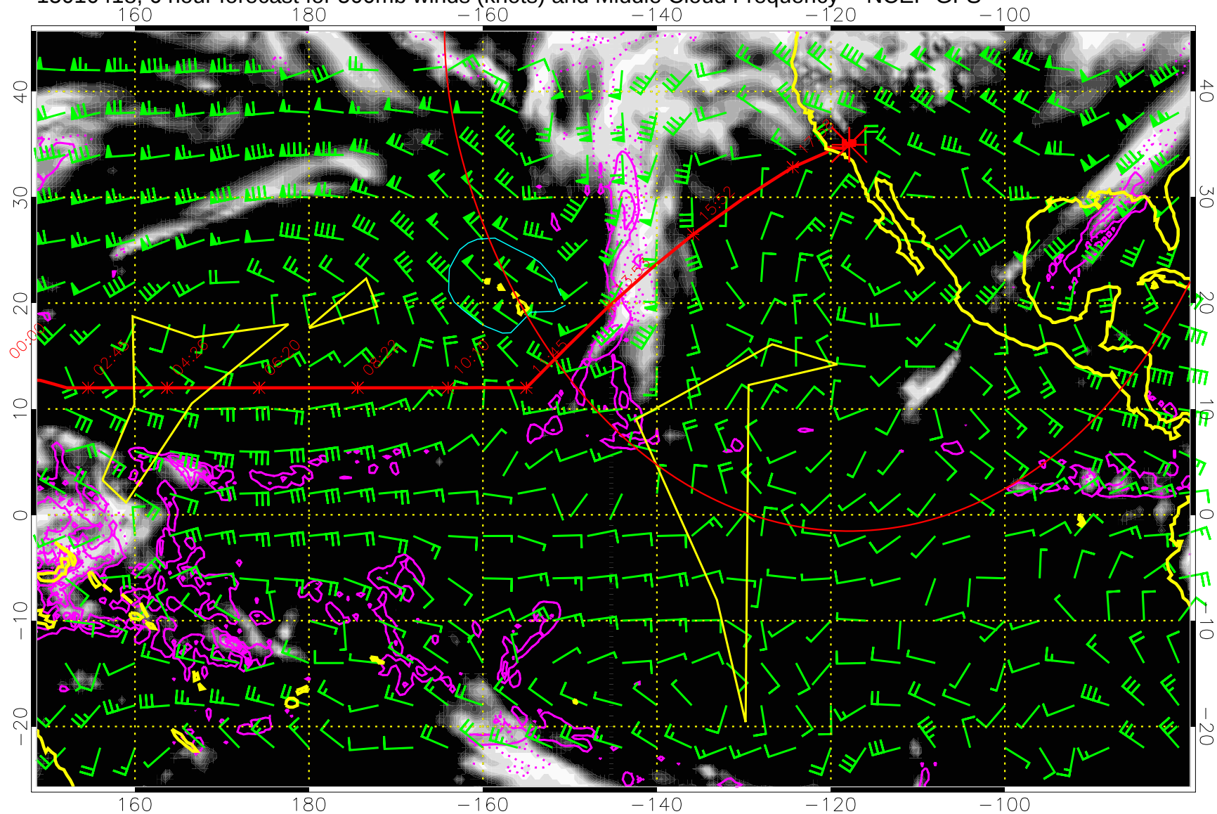
15010418, 6 hour forecast for 500mb winds (knots) and Middle Cloud Frequency -- NCEP GFS
