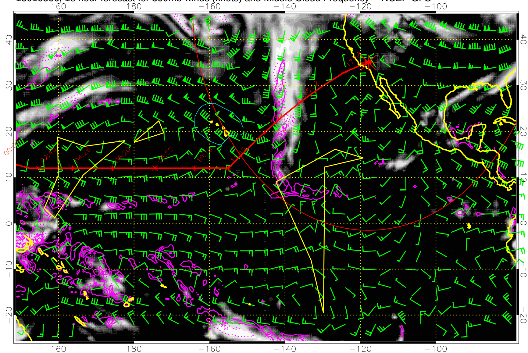
15010506, 18 hour forecast for 500mb winds (knots) and Middle Cloud Frequency -- NCEP GFS
