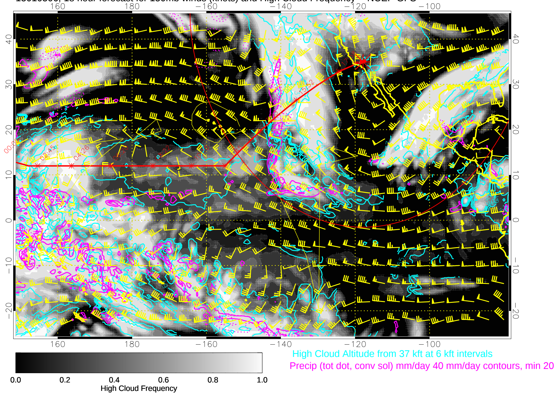
15010506, 18 hour forecast for 150mb winds (knots) and High Cloud Frequency -- NCEP GFS
