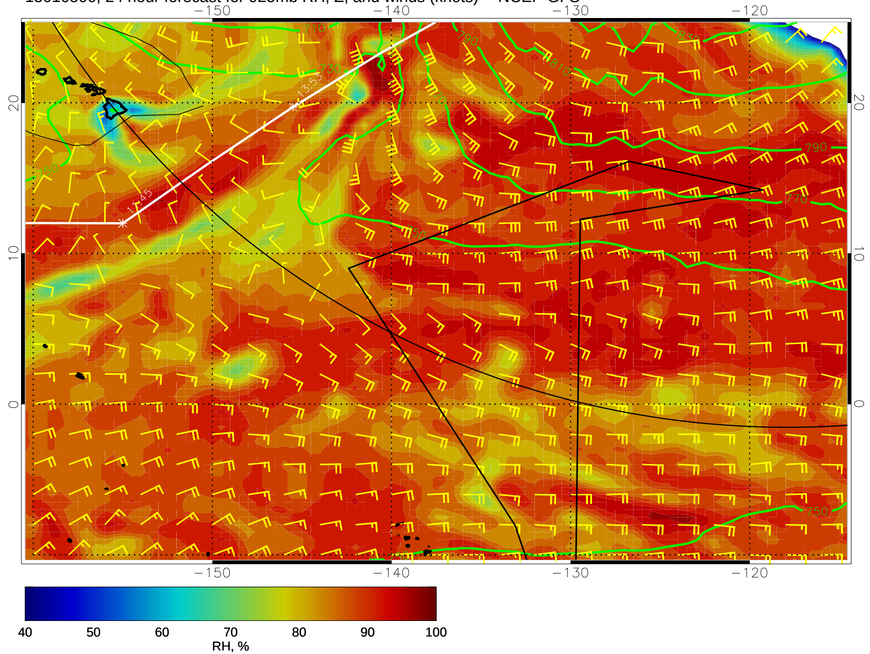
15010500, 24 hour forecast for 925mb RH, Z, and winds (knots) -- NCEP GFS
