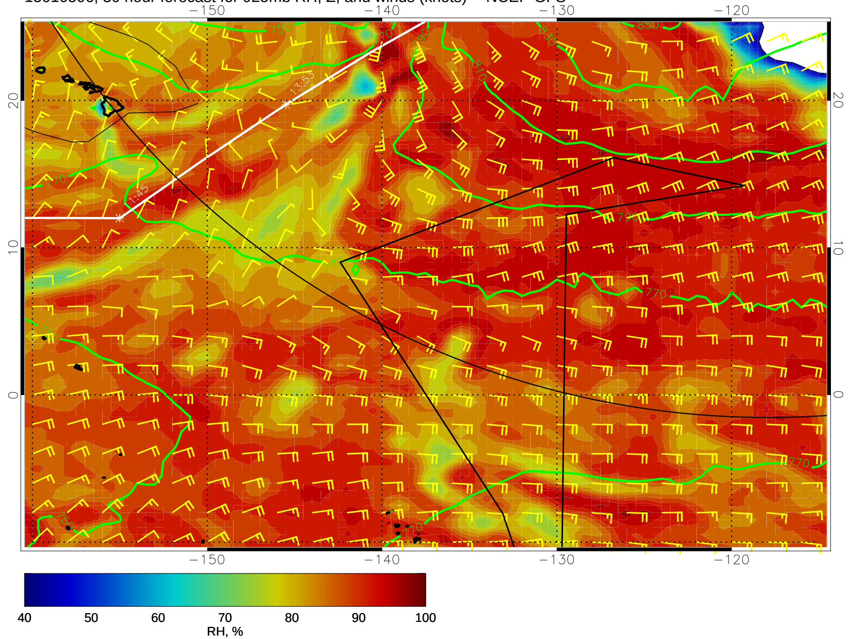
15010506, 30 hour forecast for 925mb RH, Z, and winds (knots) -- NCEP GFS
