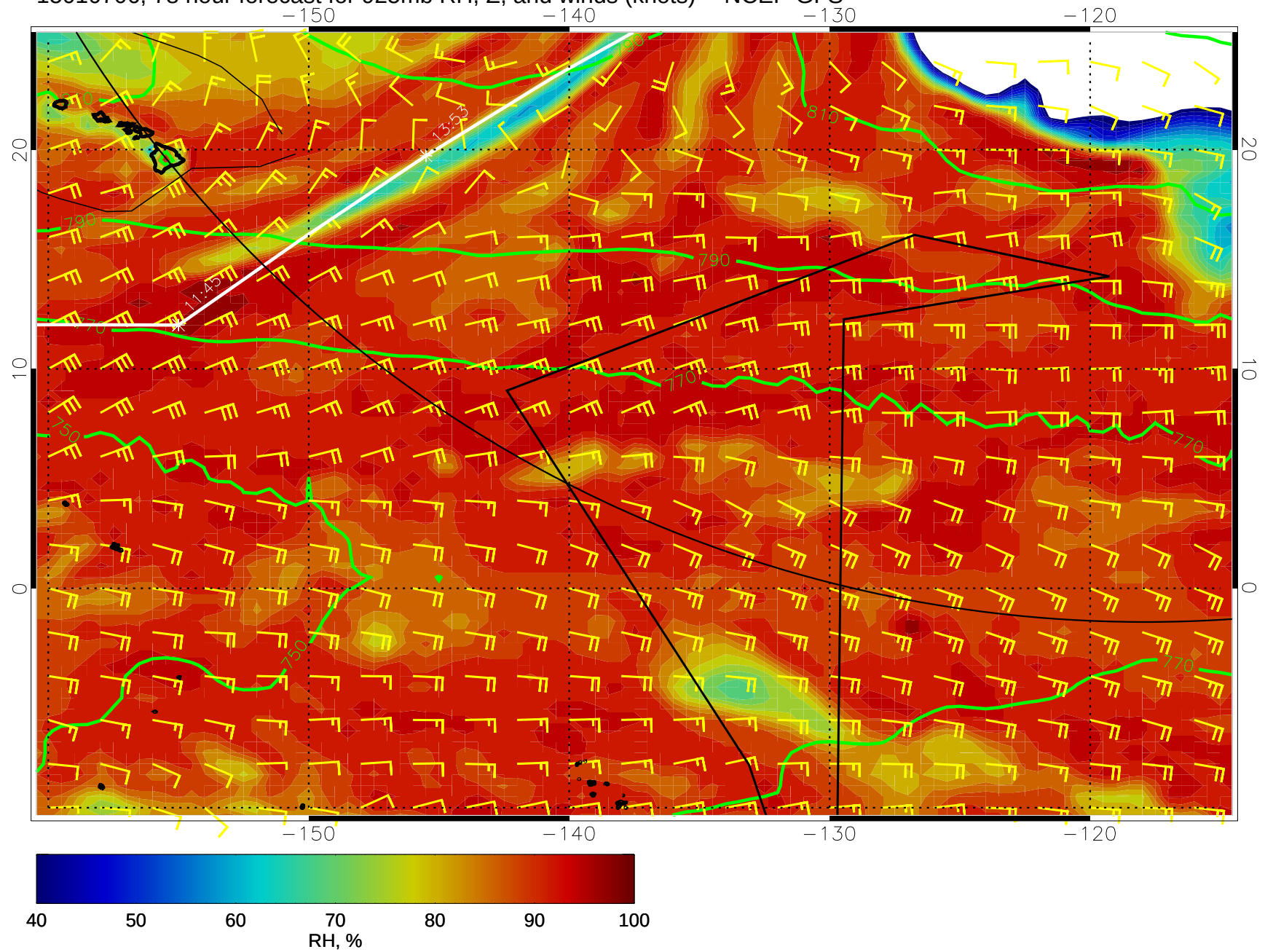
15010706, 78 hour forecast for 925mb RH, Z, and winds (knots) -- NCEP GFS
