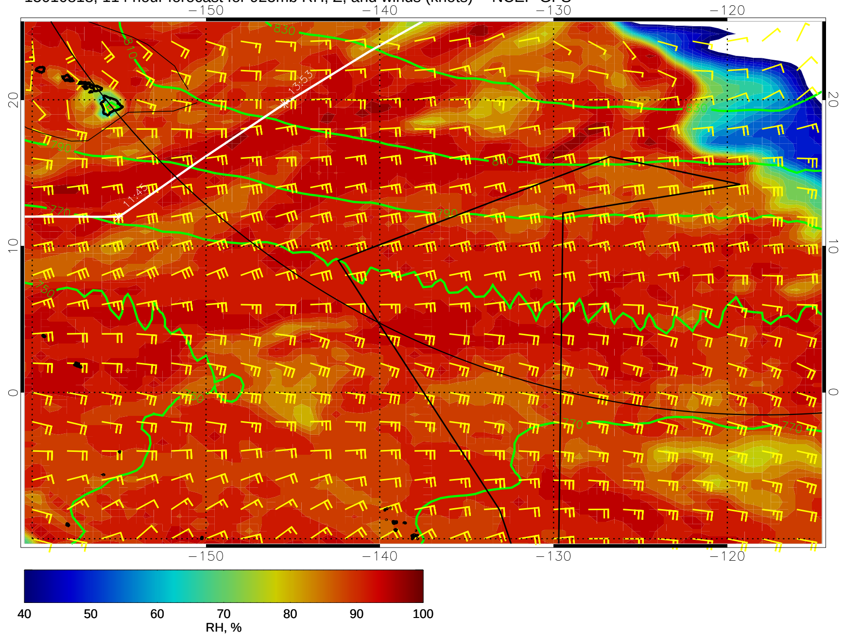
15010818, 114 hour forecast for 925mb RH, Z, and winds (knots) -- NCEP GFS
