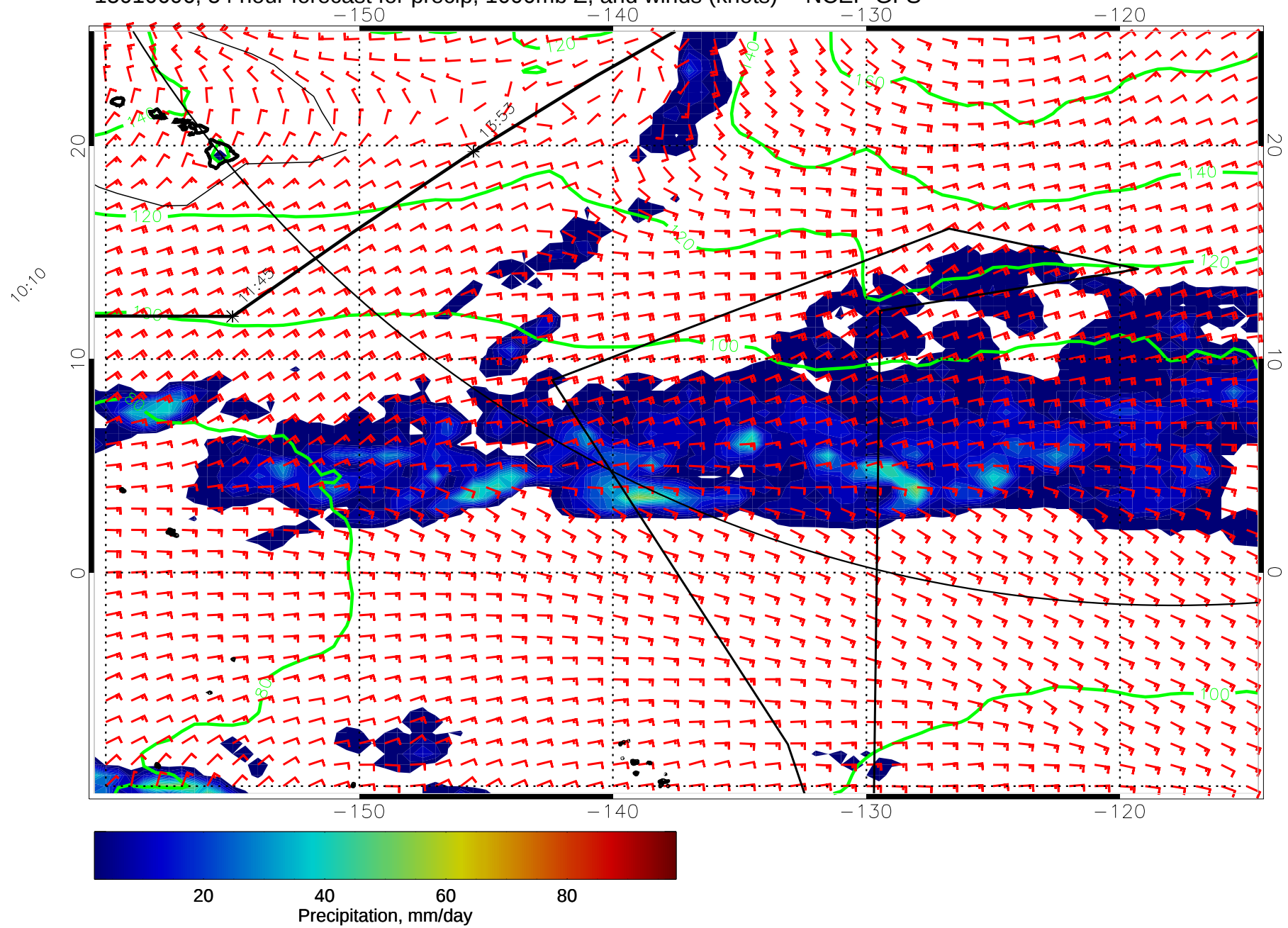
15010606, 54 hour forecast for precip, 1000mb Z, and winds (knots) -- NCEP GFS
