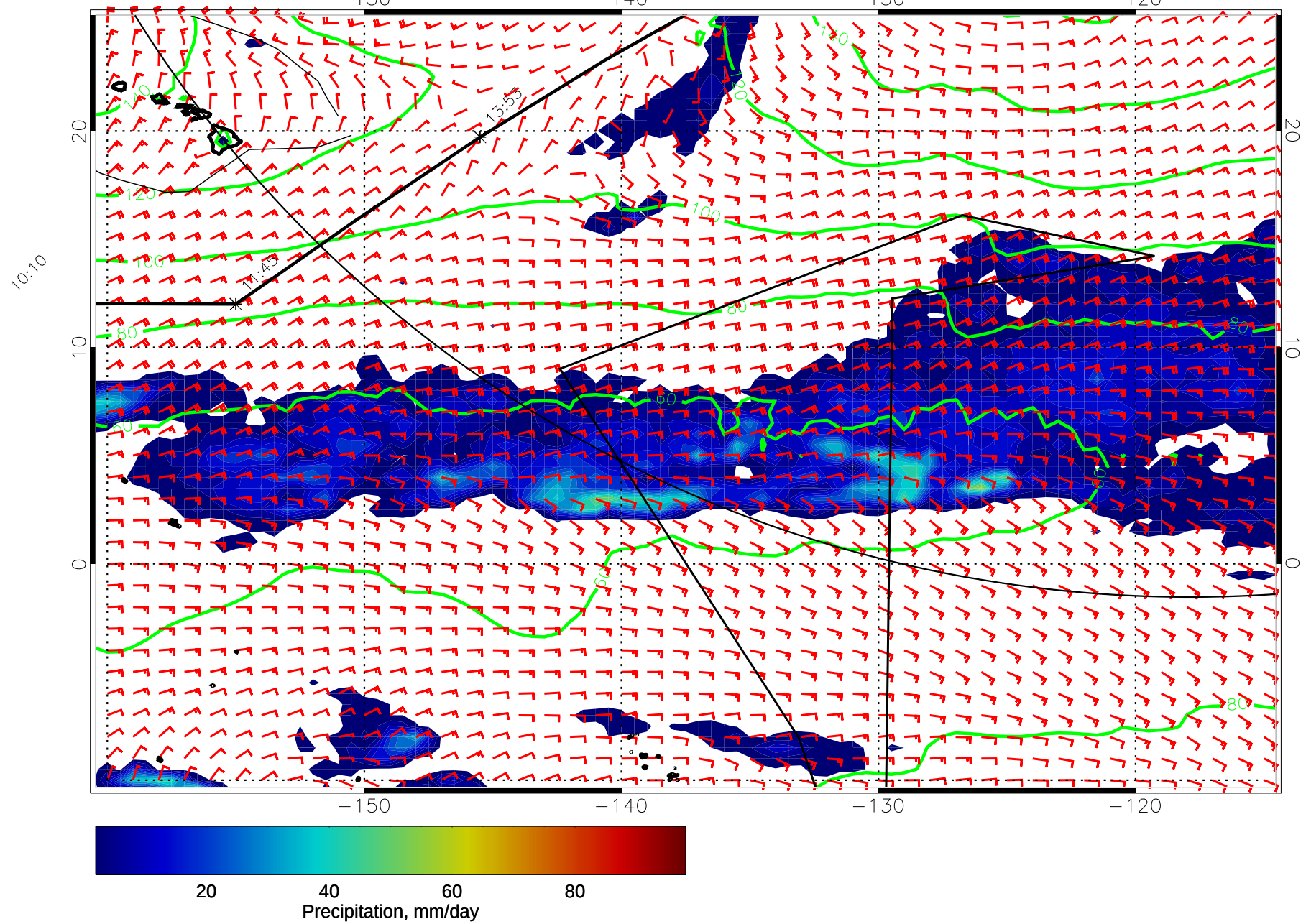
15010612, 60 hour forecast for precip, 1000mb Z, and winds (knots) -- NCEP GFS
