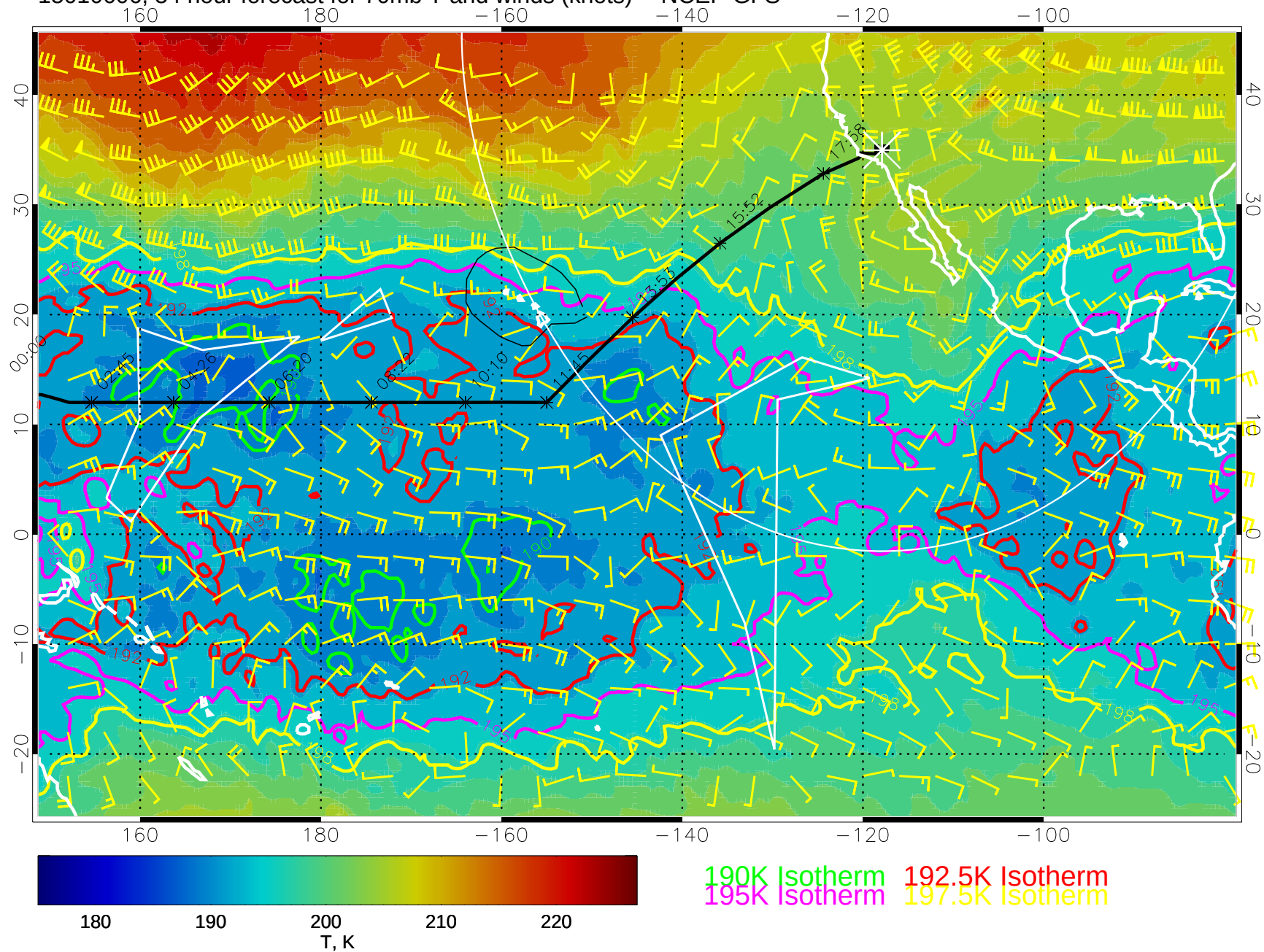
15010606, 54 hour forecast for 70mb T and winds (knots) -- NCEP GFS
