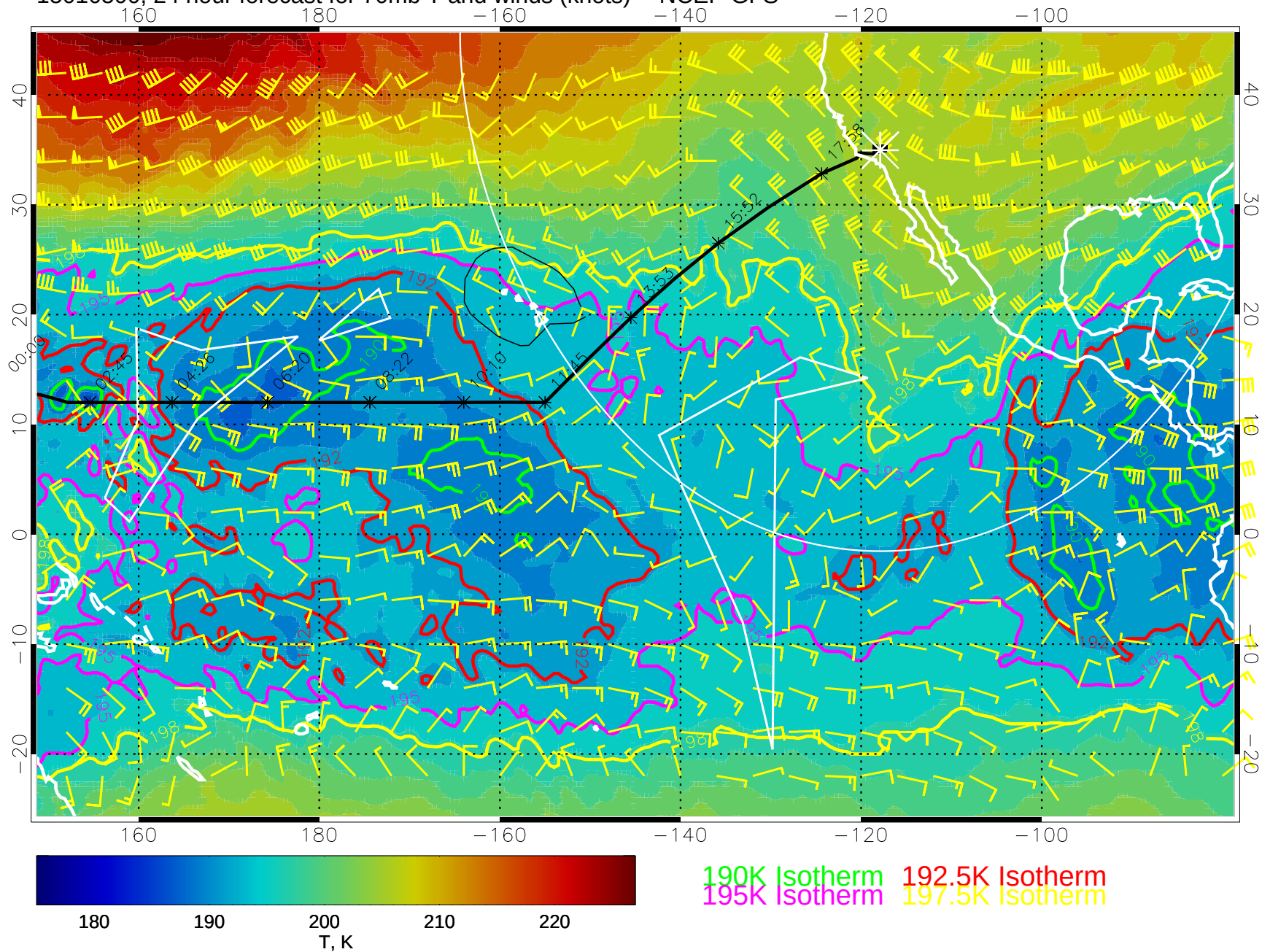
15010500, 24 hour forecast for 70mb T and winds (knots) -- NCEP GFS
