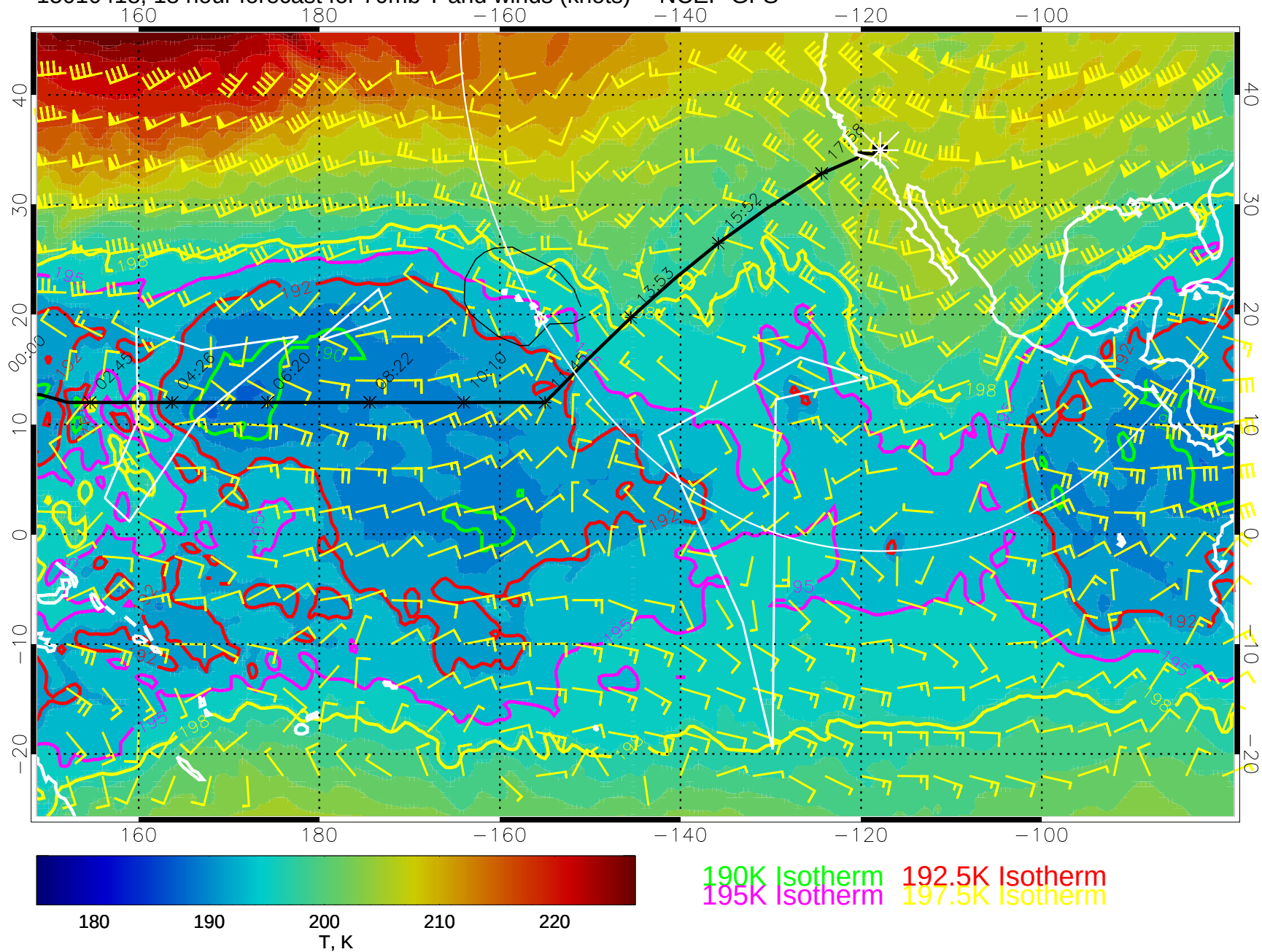
15010418, 18 hour forecast for 70mb T and winds (knots) -- NCEP GFS
