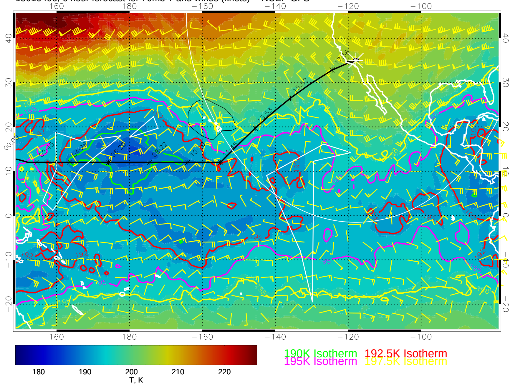
15010406, 6 hour forecast for 70mb T and winds (knots) -- NCEP GFS
