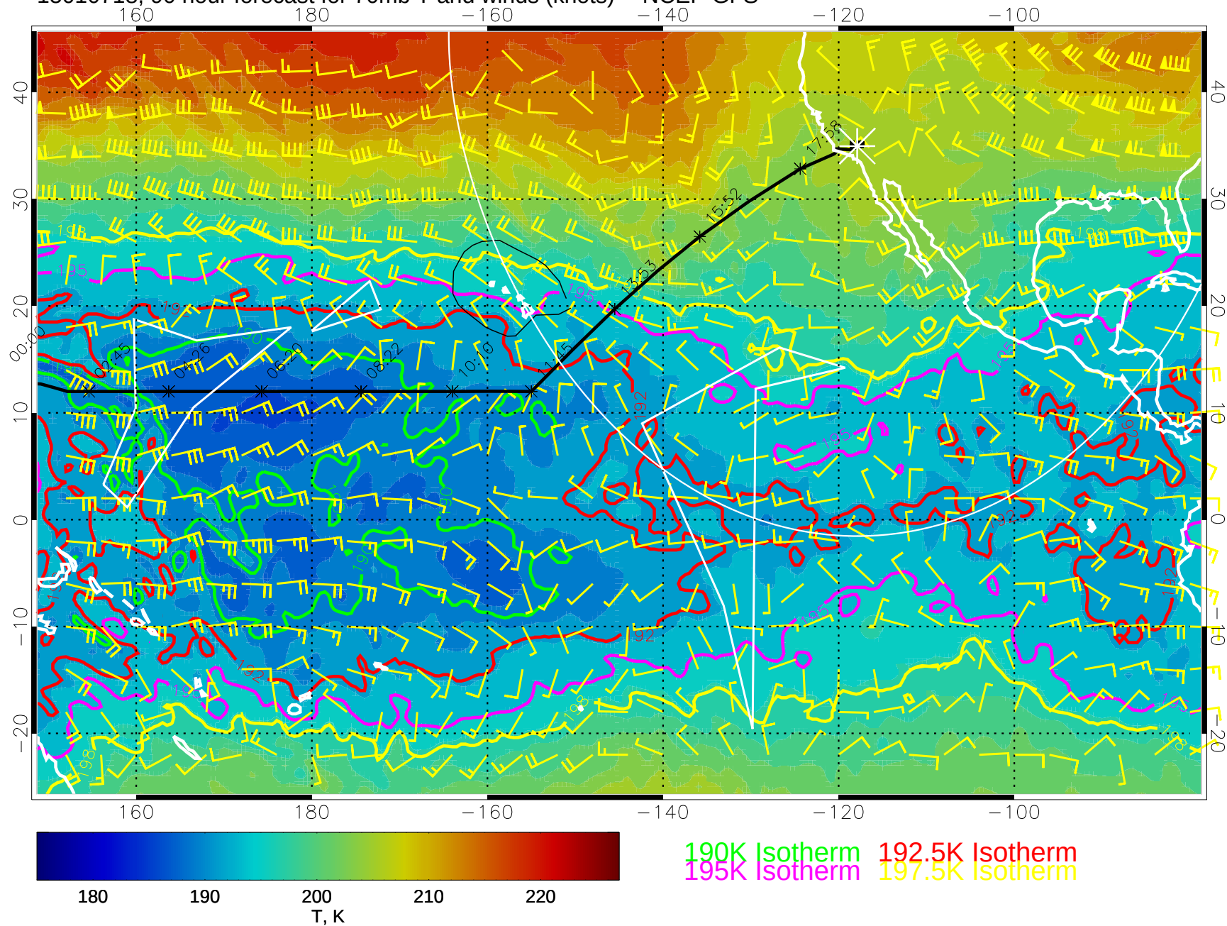
15010718, 90 hour forecast for 70mb T and winds (knots) -- NCEP GFS
