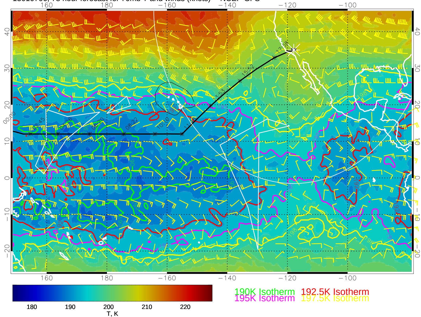
15010706, 78 hour forecast for 70mb T and winds (knots) -- NCEP GFS
