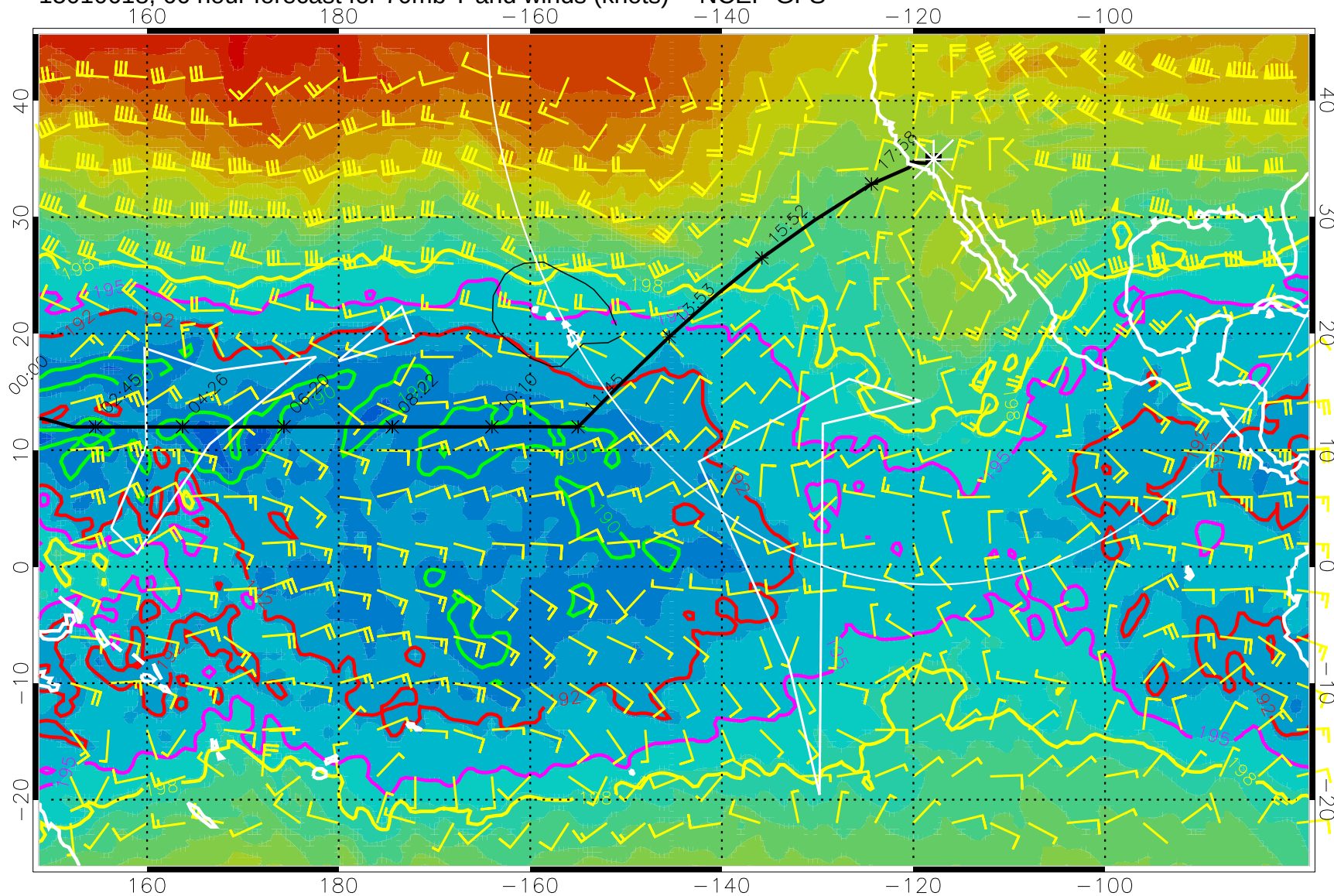
15010618, 66 hour forecast for 70mb T and winds (knots) -- NCEP GFS
