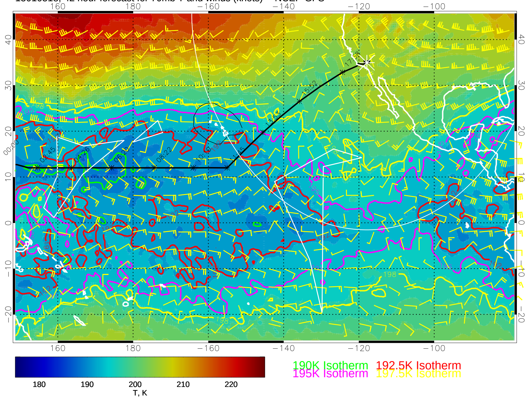
15010518, 42 hour forecast for 70mb T and winds (knots) -- NCEP GFS
