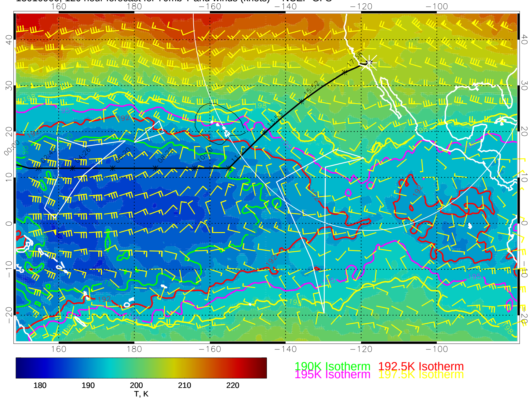
15010900, 120 hour forecast for 70mb T and winds (knots) -- NCEP GFS
