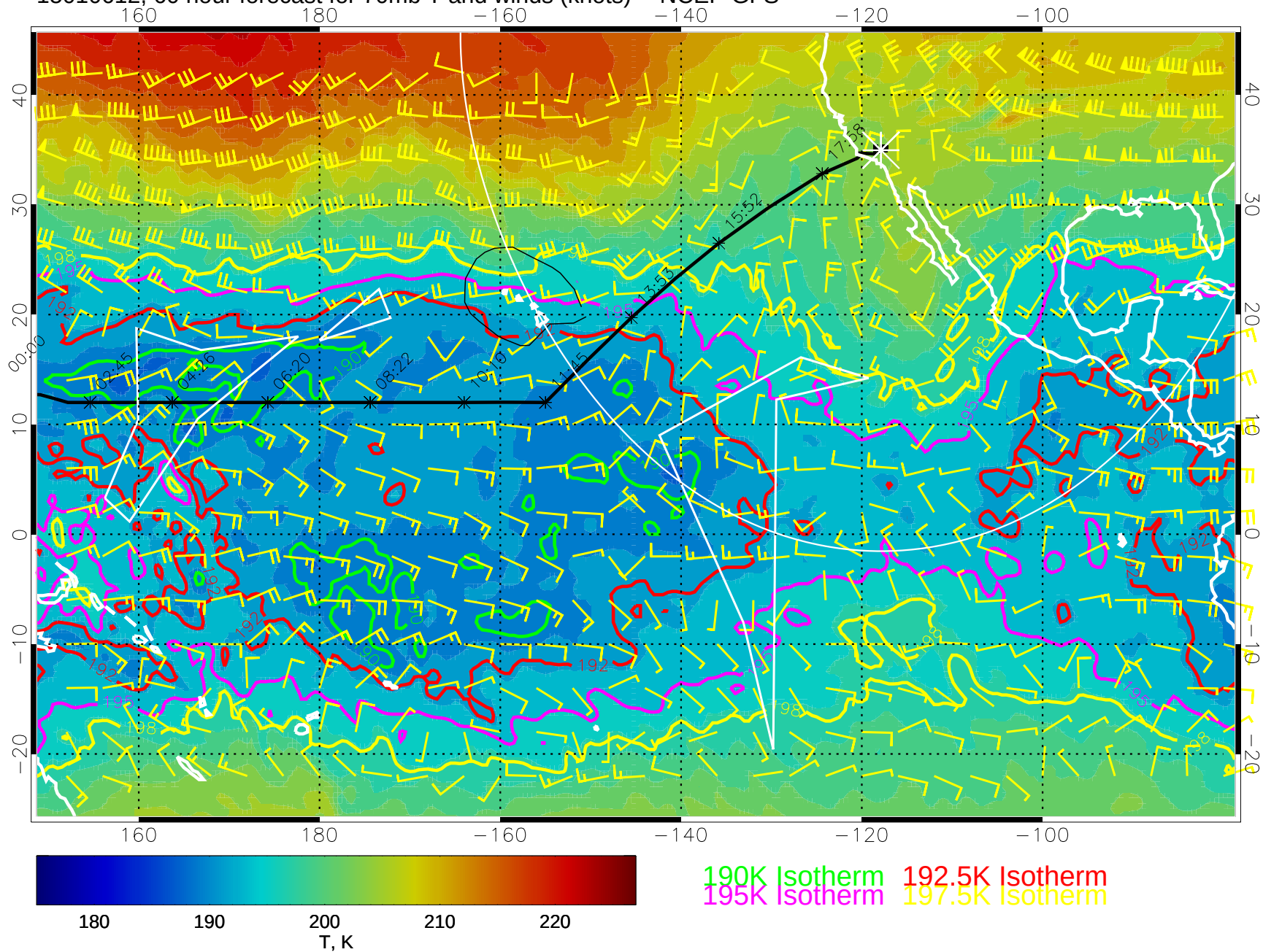
15010612, 60 hour forecast for 70mb T and winds (knots) -- NCEP GFS
