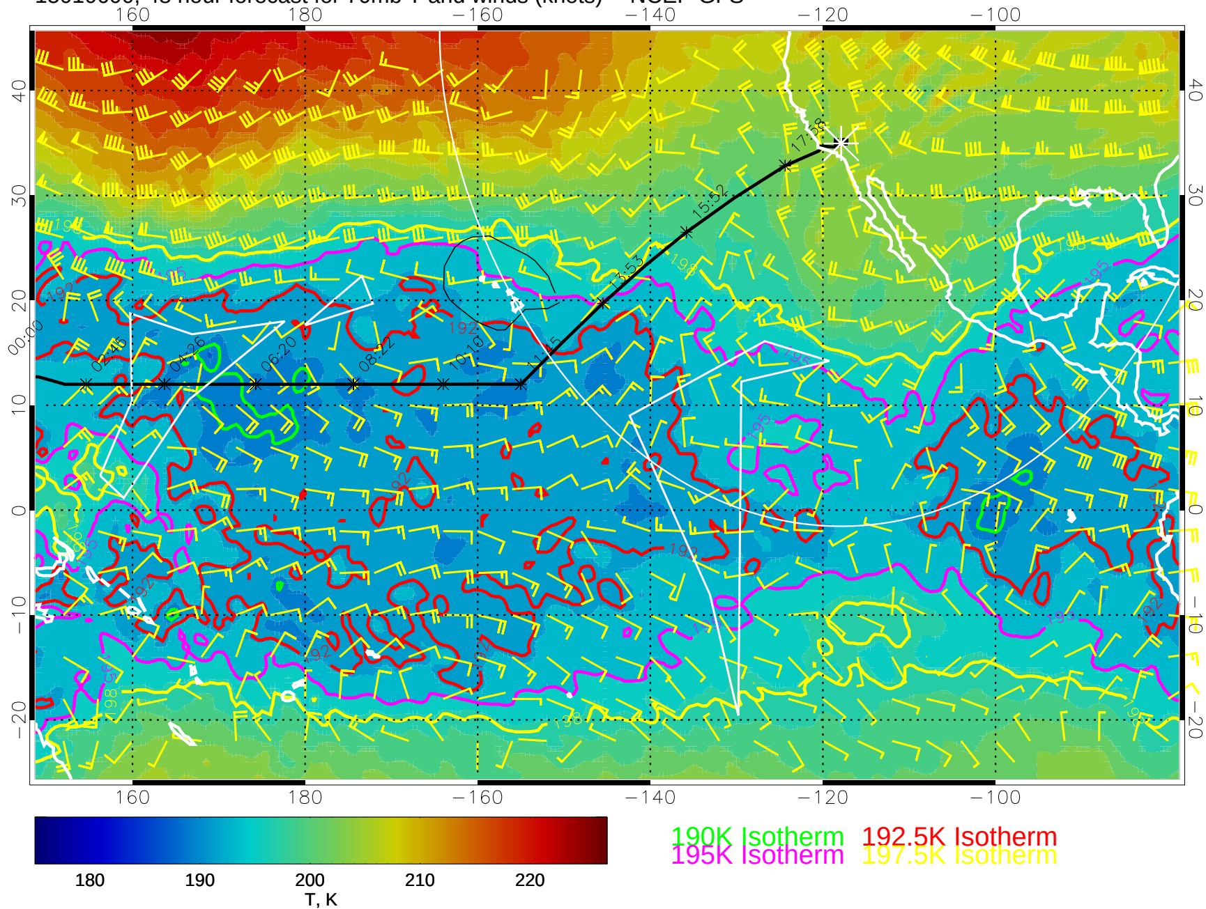
15010600, 48 hour forecast for 70mb T and winds (knots) -- NCEP GFS
