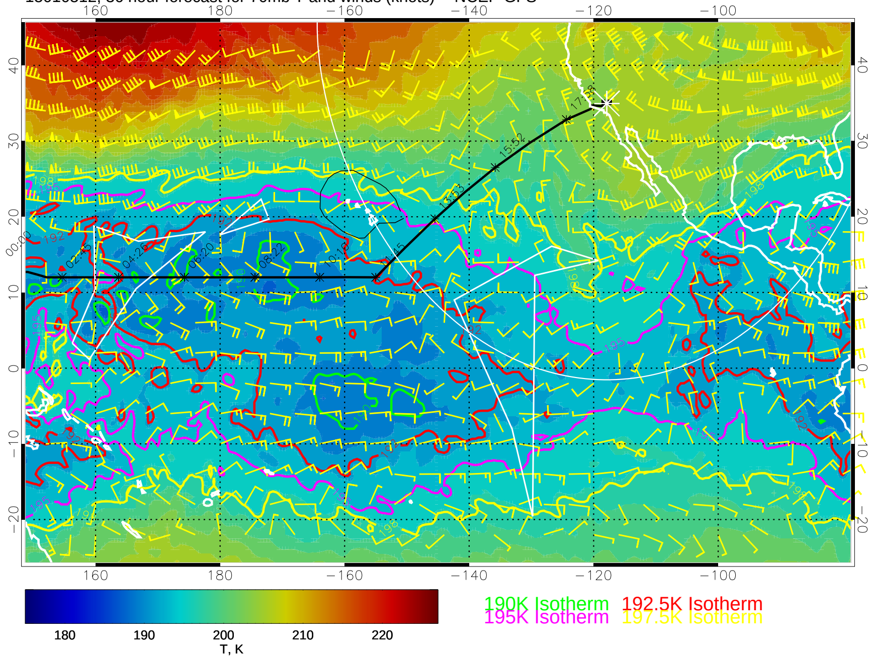
15010512, 36 hour forecast for 70mb T and winds (knots) -- NCEP GFS
