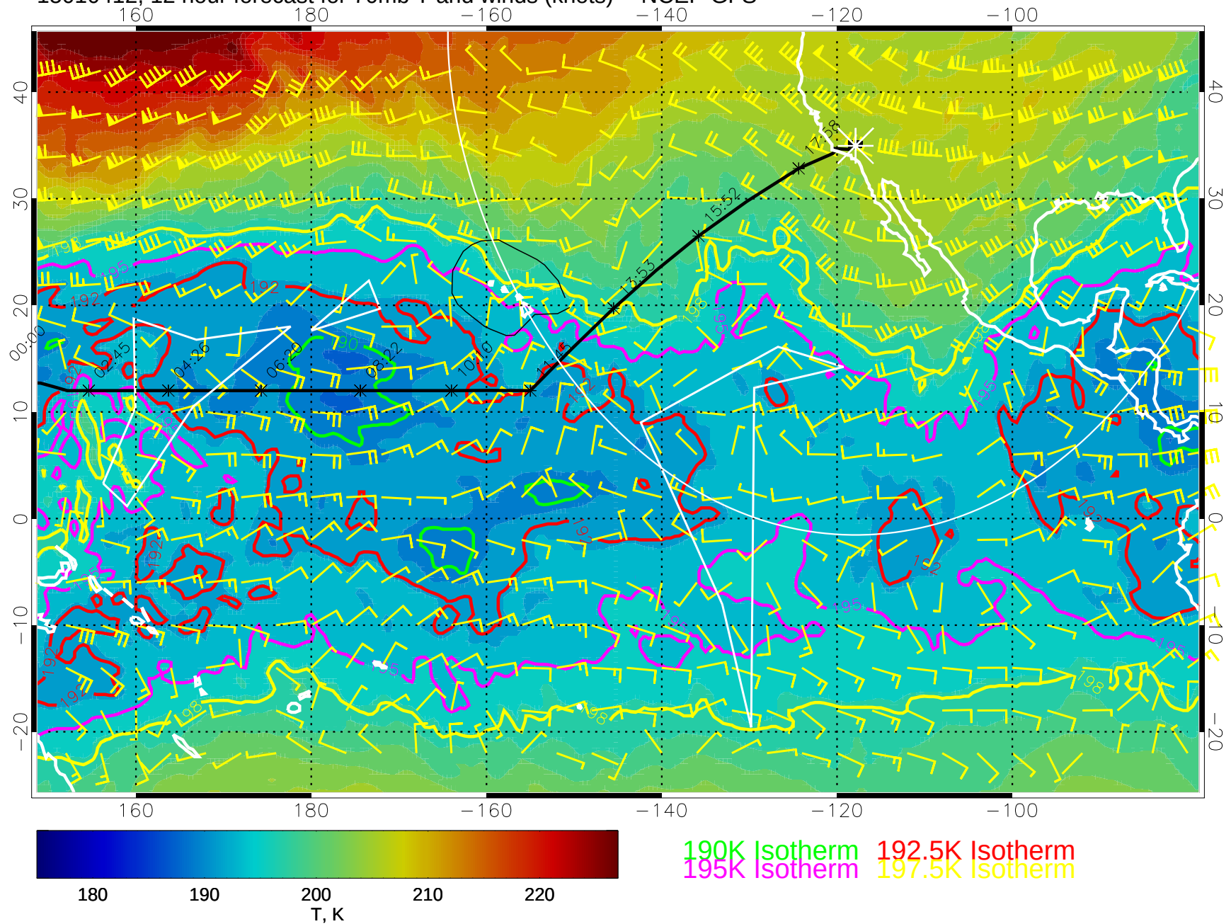
15010412, 12 hour forecast for 70mb T and winds (knots) -- NCEP GFS
