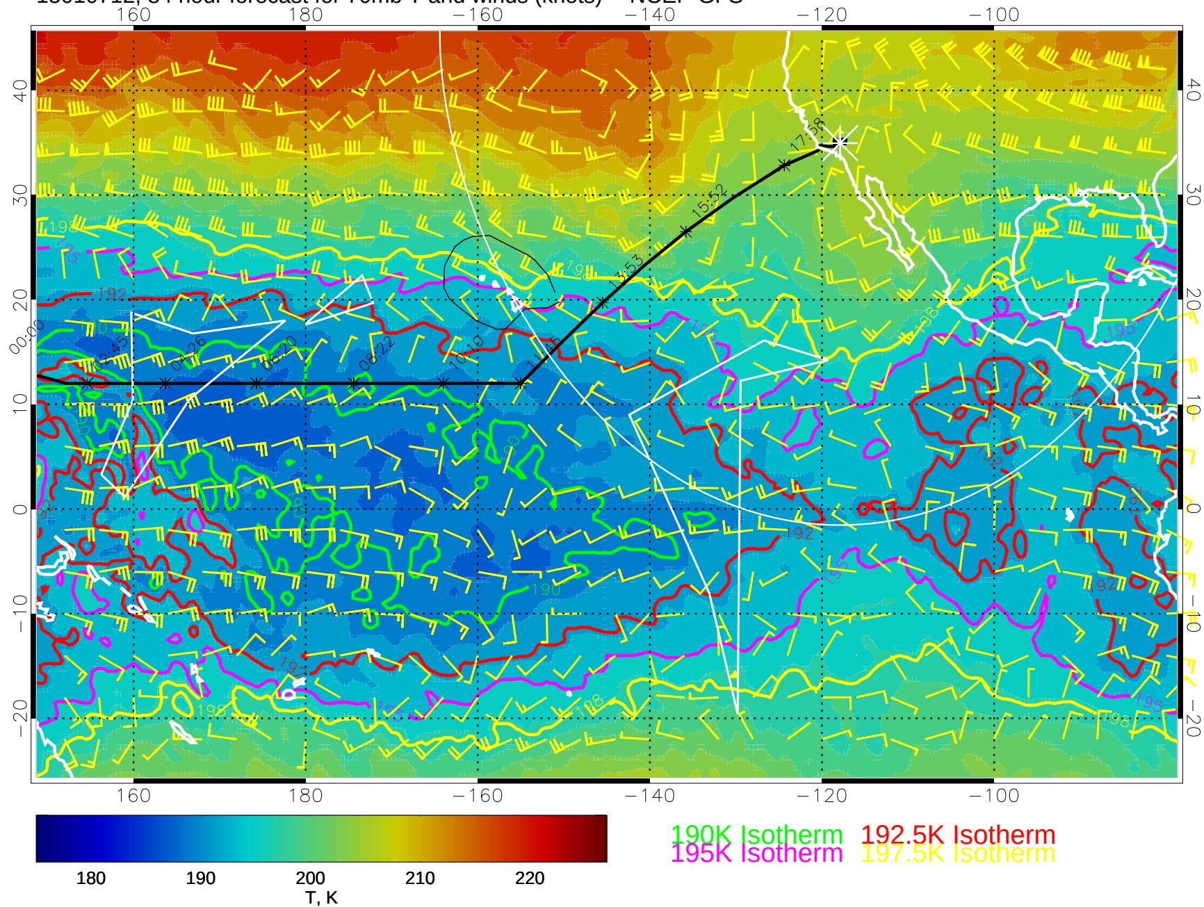
15010712, 84 hour forecast for 70mb T and winds (knots) -- NCEP GFS
