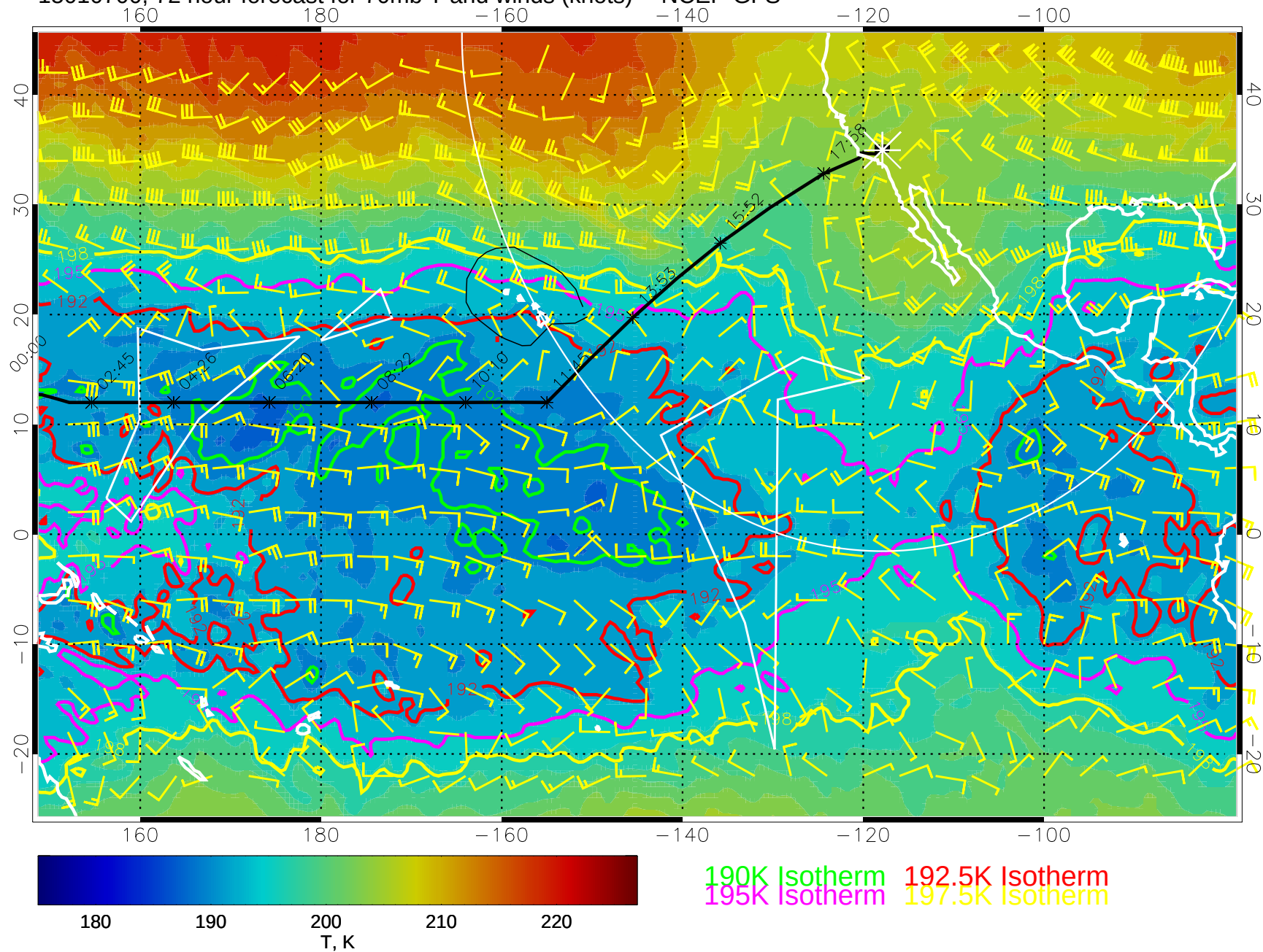
15010700, 72 hour forecast for 70mb T and winds (knots) -- NCEP GFS
