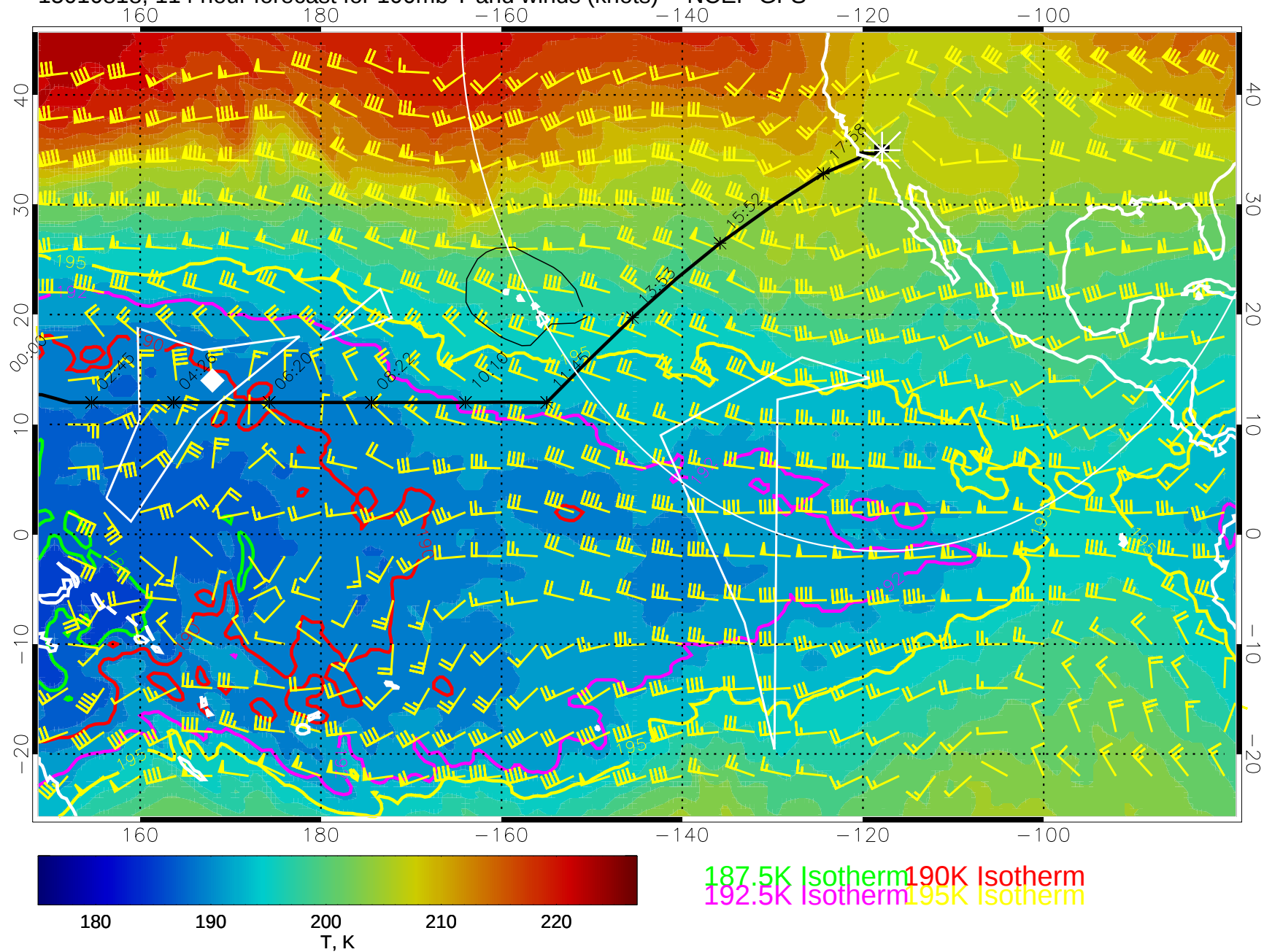
15010818, 114 hour forecast for 100mb T and winds (knots) -- NCEP GFS
