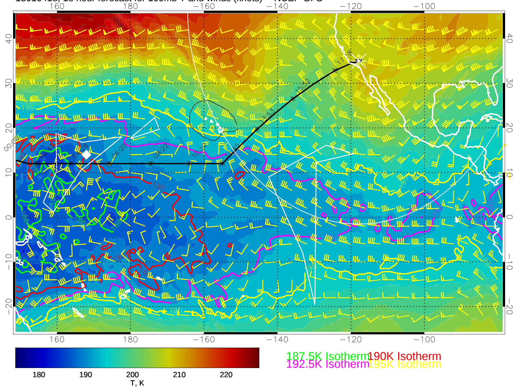
15010418, 18 hour forecast for 100mb T and winds (knots) -- NCEP GFS
