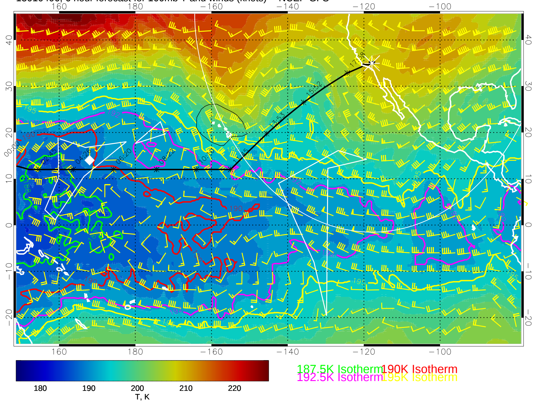
15010406, 6 hour forecast for 100mb T and winds (knots) -- NCEP GFS
