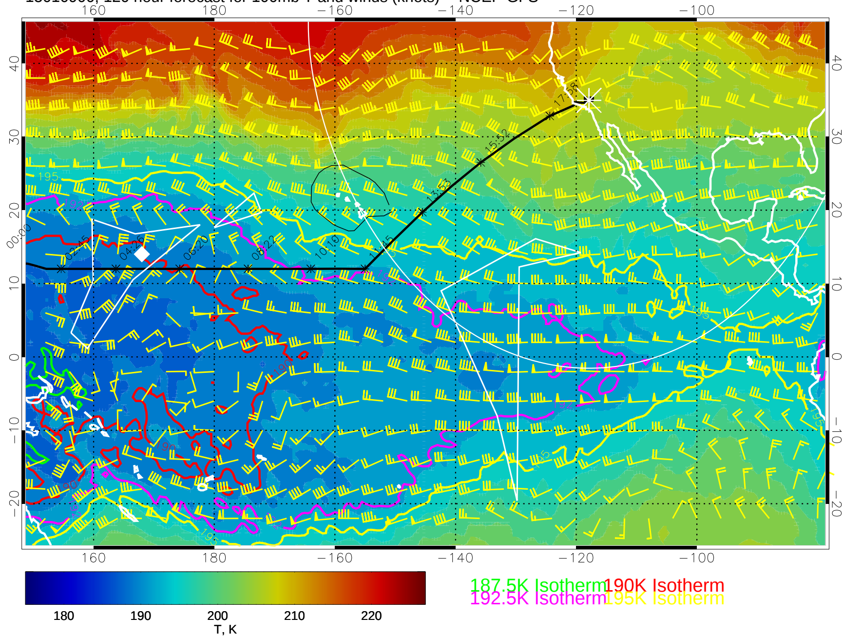
15010900, 12 hour forecast for 100mb T and winds (knots) -- NCEP GFS
