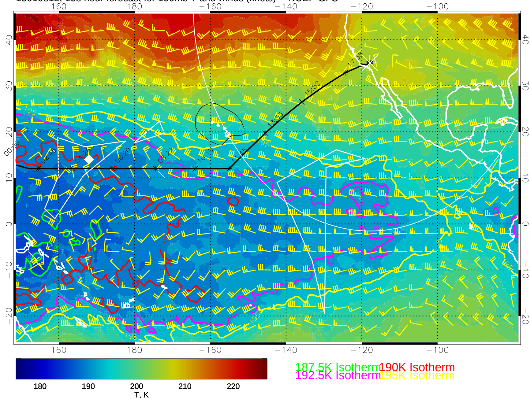
15010812, 108 hour forecast for 100mb T and winds (knots) -- NCEP GFS
