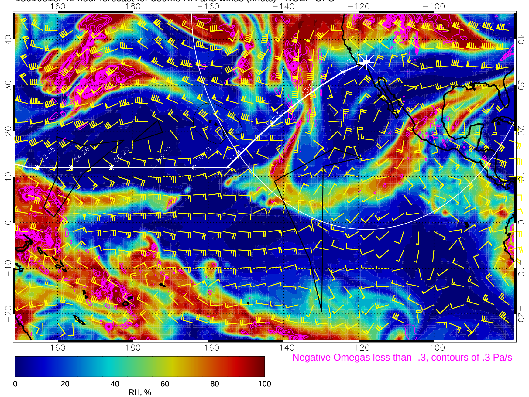
15010518, 42 hour forecast for 500mb RH and winds (knots) - NCEP GFS
