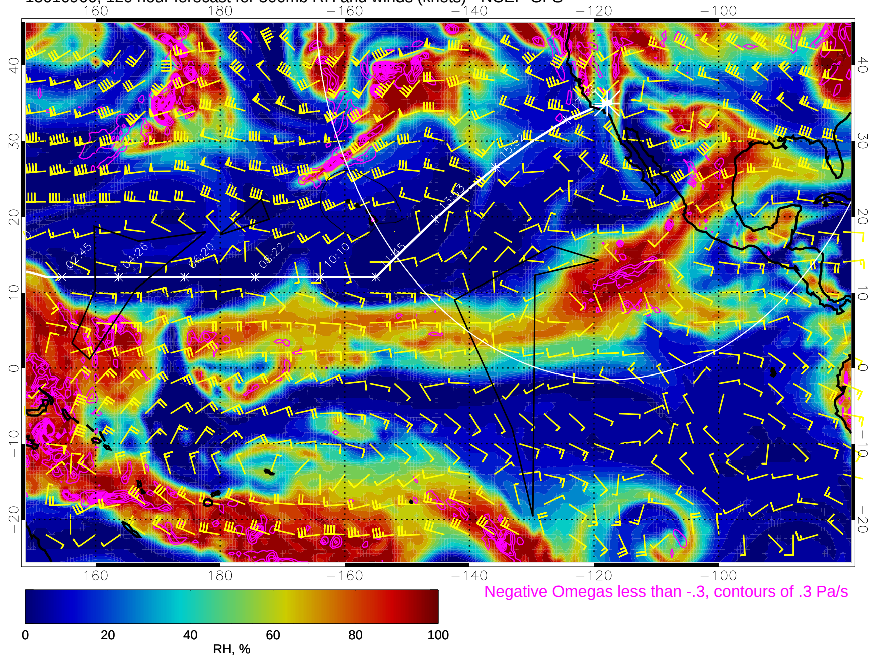
15010900, 120 hour forecast for 500mb RH and winds (knots) - NCEP GFS
