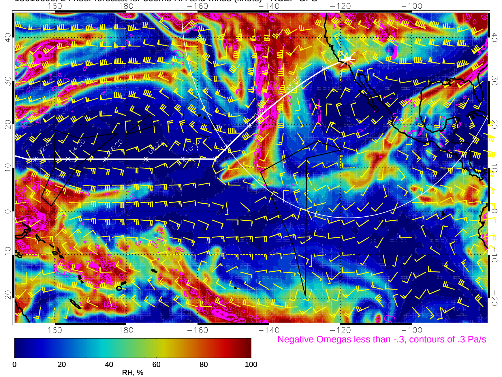
15010500, 24 hour forecast for 500mb RH and winds (knots) - NCEP GFS
