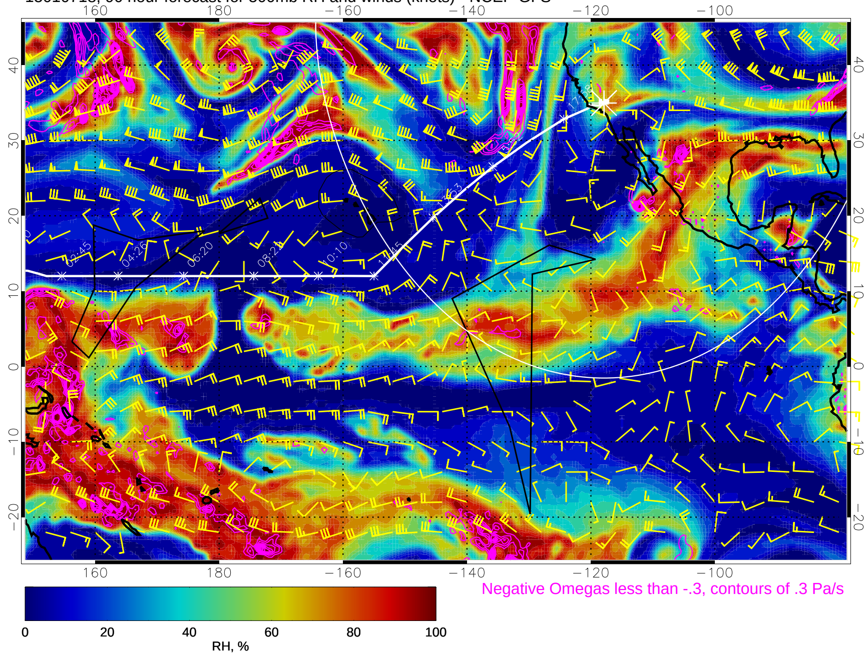
15010718, 90 hour forecast for 500mb RH and winds (knots) - NCEP GFS
