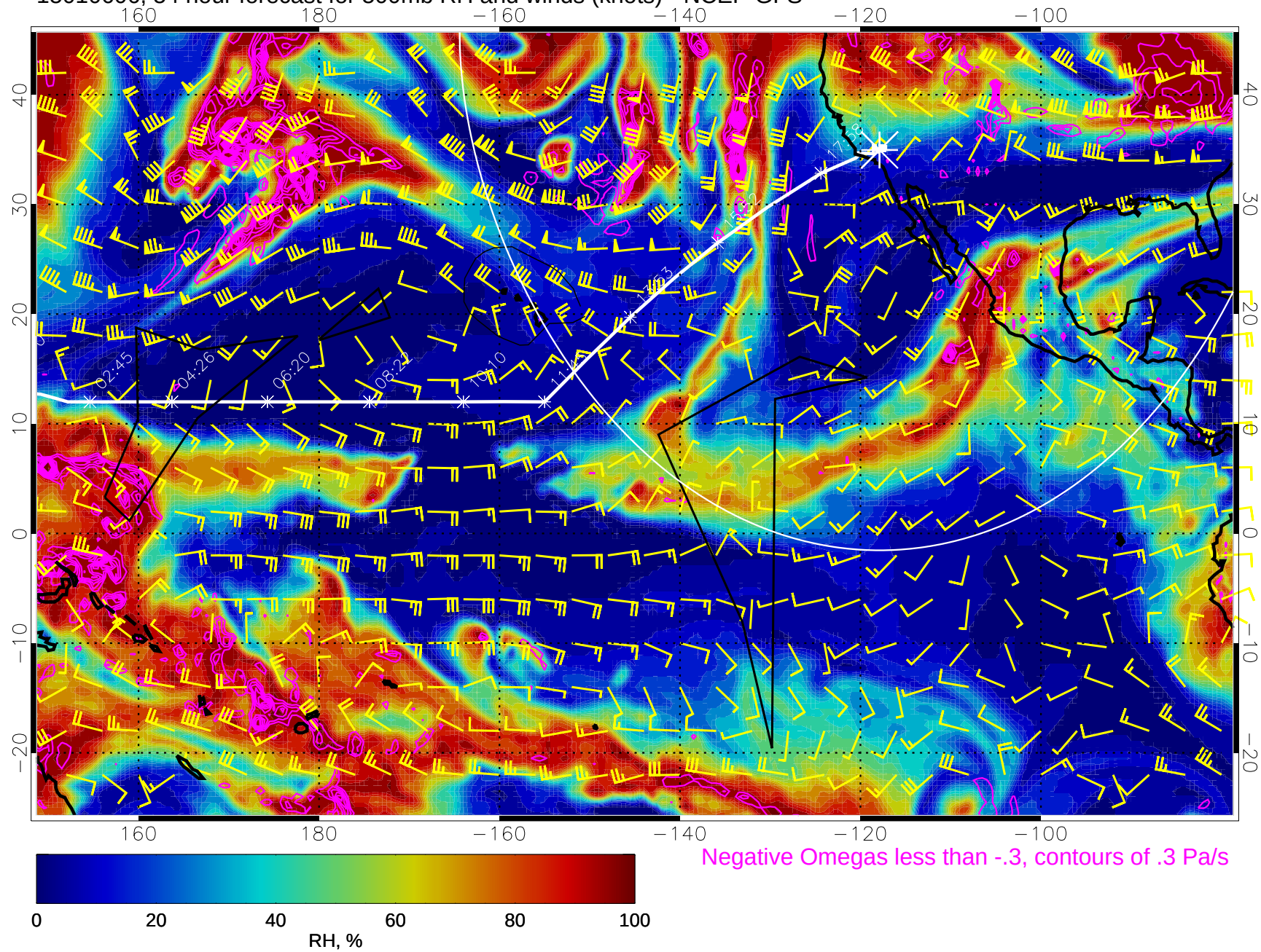
15010606, 54 hour forecast for 500mb RH and winds (knots) - NCEP GFS
