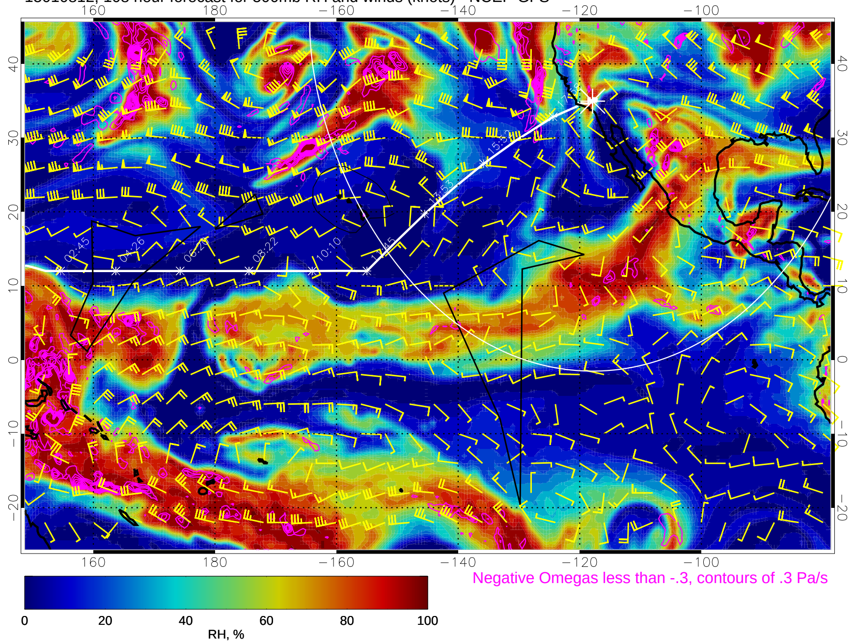
15010812, 108 hour forecast for 500mb RH and winds (knots) - NCEP GFS
