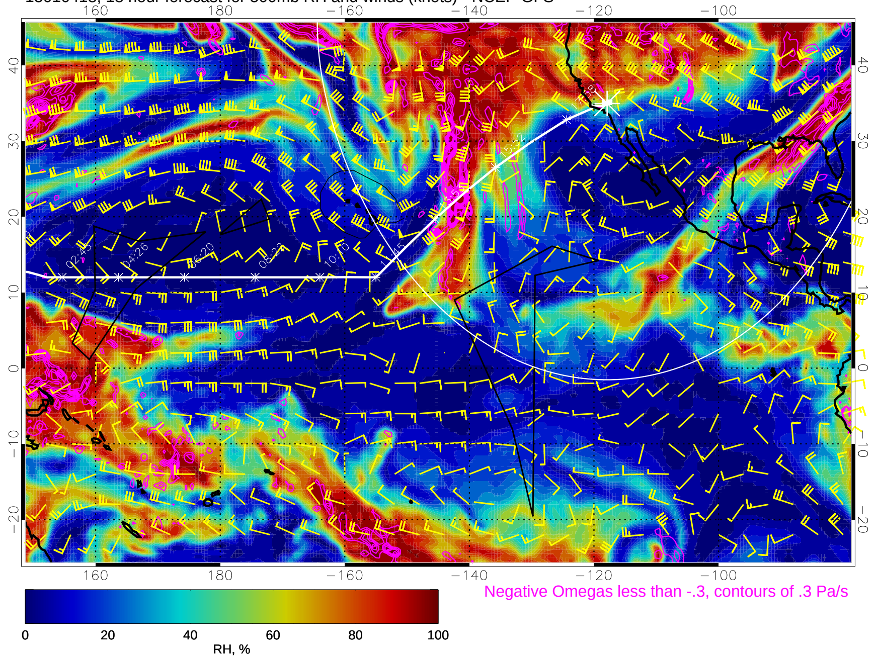
15010418, 18 hour forecast for 500mb RH and winds (knots) - NCEP GFS
