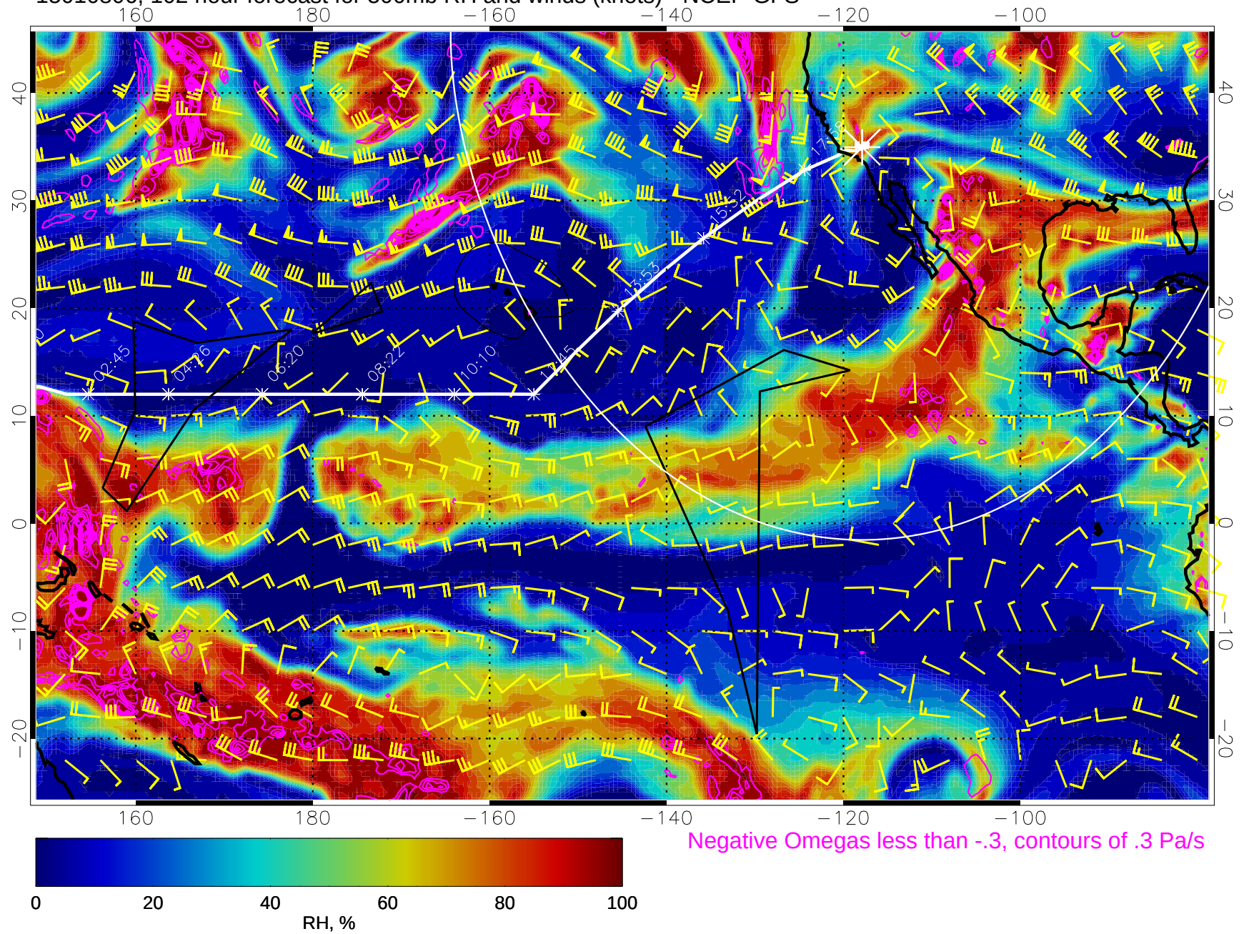
15010806, 102 hour forecast for 500mb RH and winds (knots) - NCEP GFS
