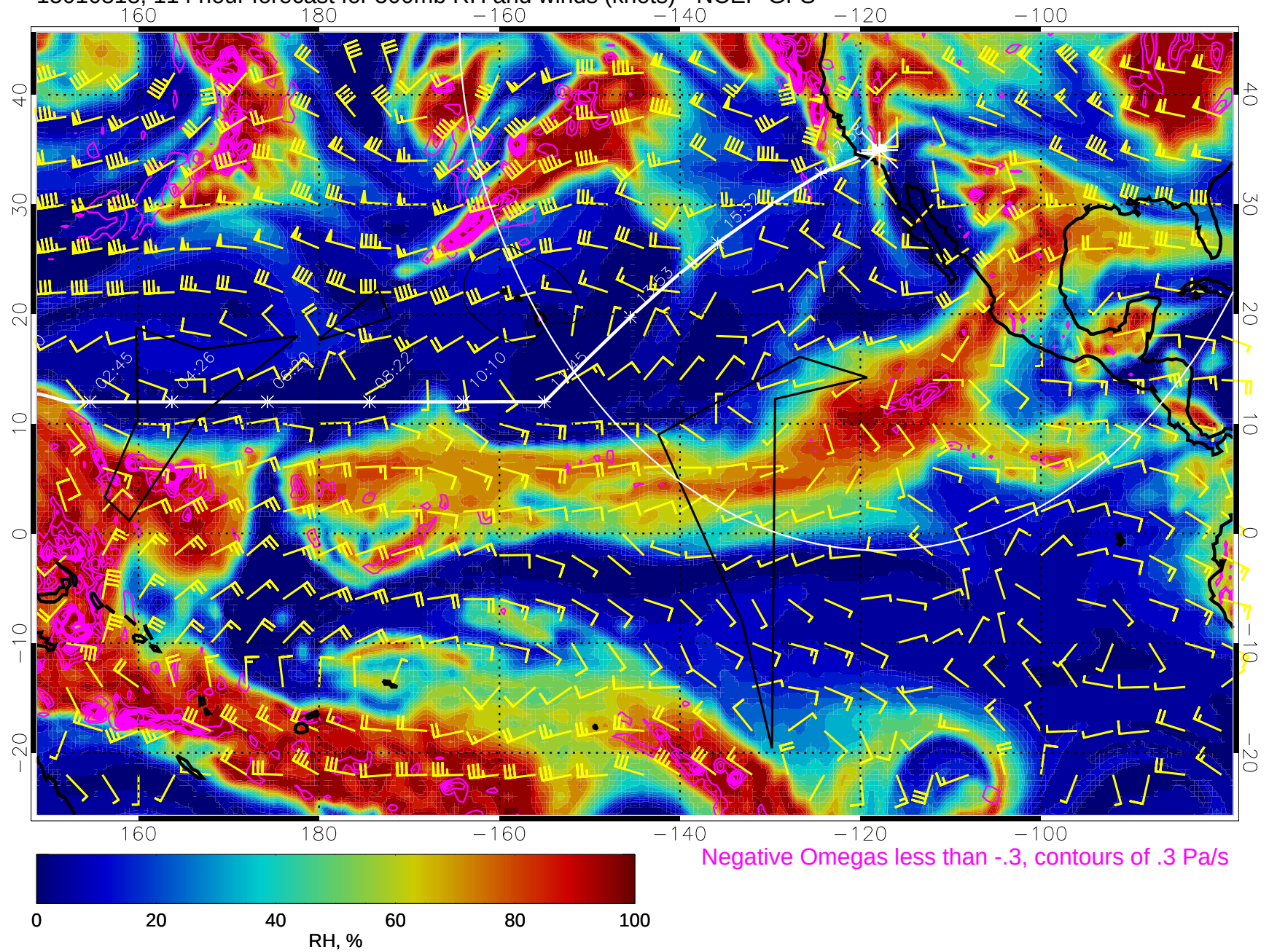
15010818, 114 hour forecast for 500mb RH and winds (knots) - NCEP GFS
