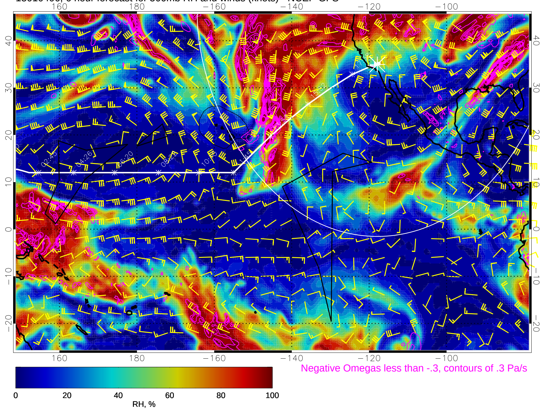
15010406, 6 hour forecast for 500mb RH and winds (knots) - NCEP GFS
