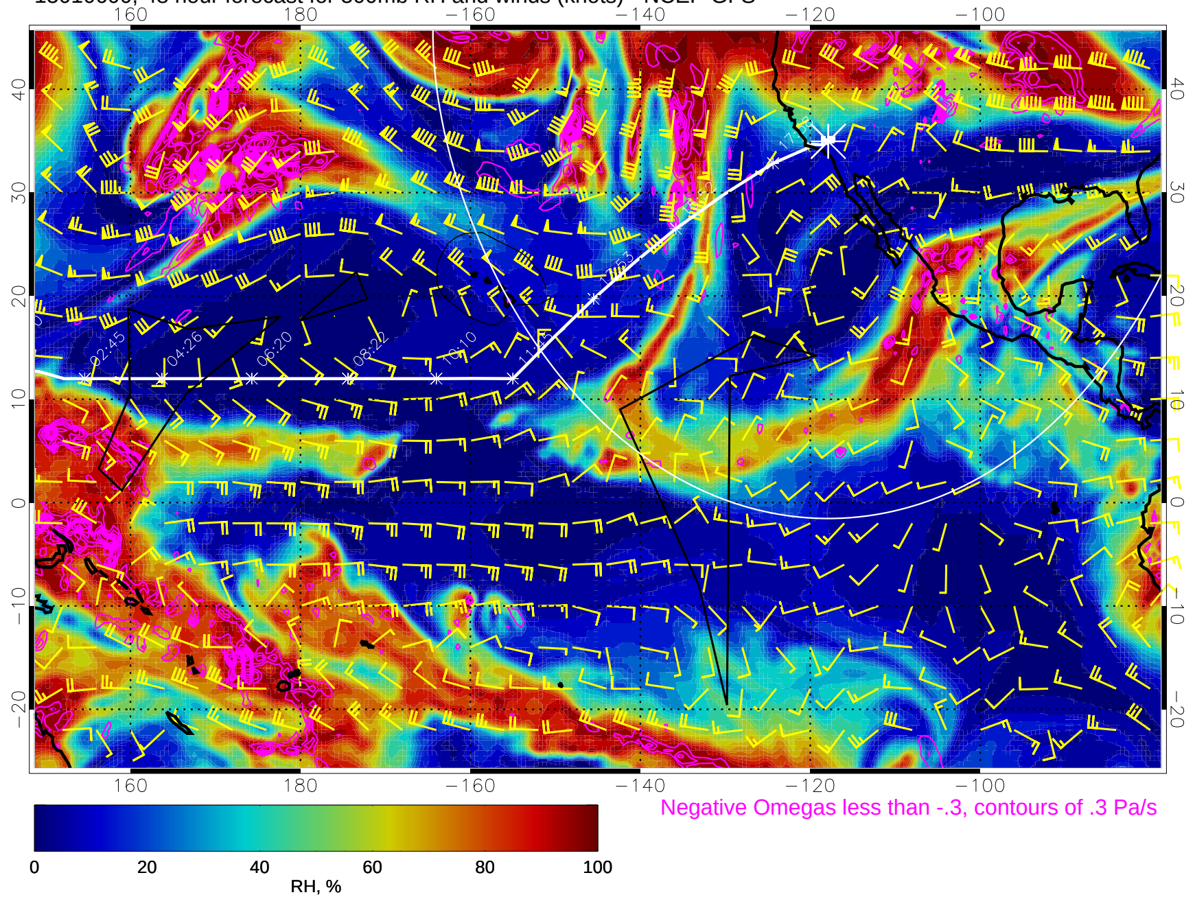
15010600, 48 hour forecast for 500mb RH and winds (knots) - NCEP GFS
