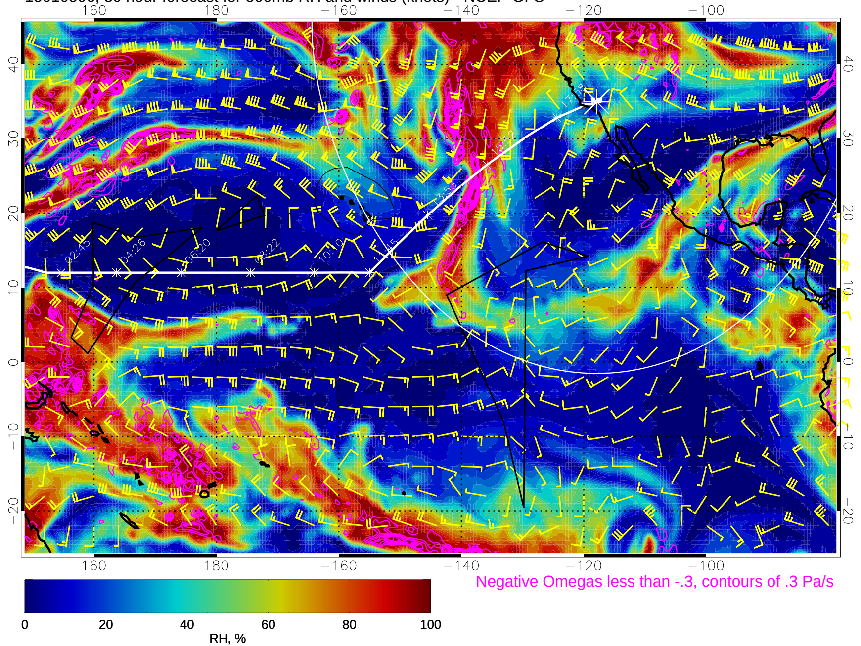
15010506, 30 hour forecast for 500mb RH and winds (knots) - NCEP GFS
