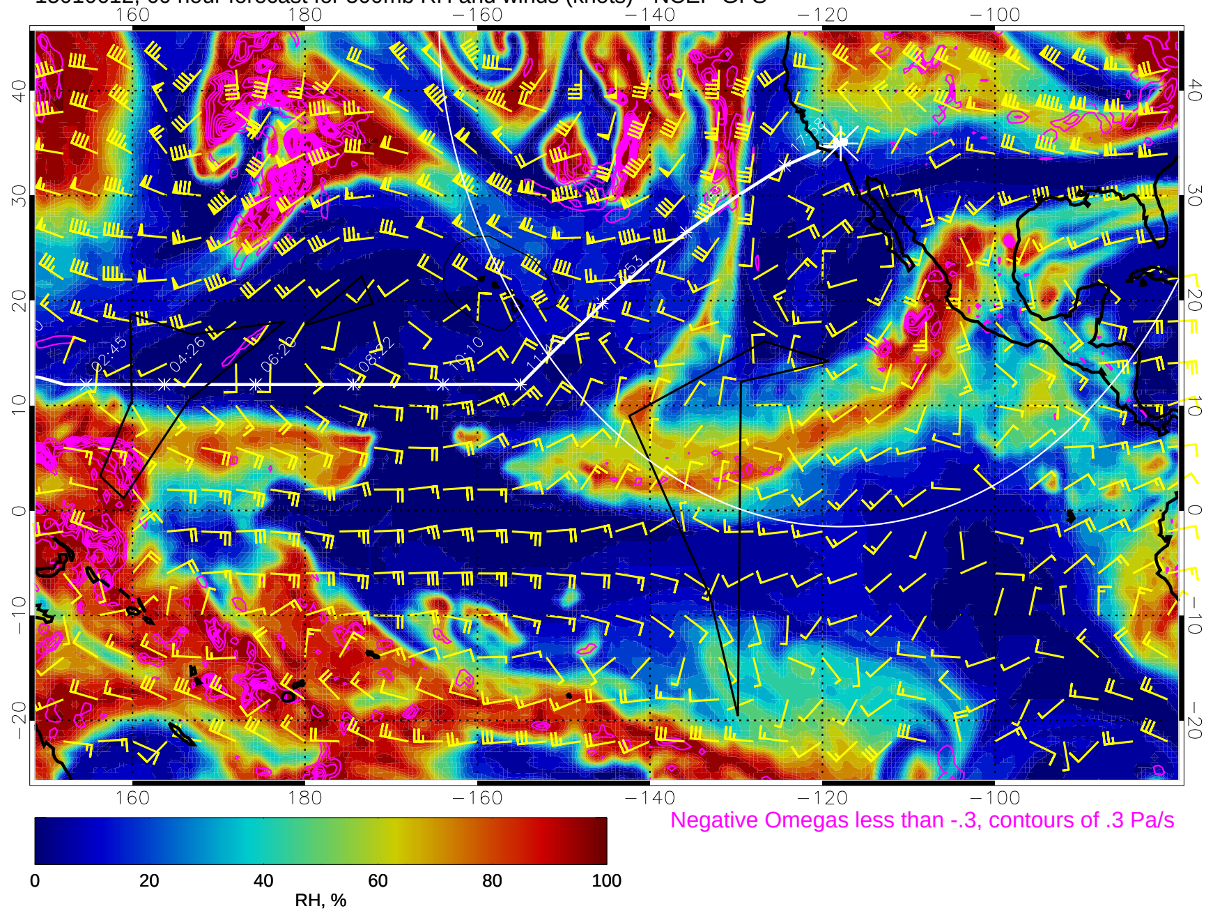
15010612, 60 hour forecast for 500mb RH and winds (knots) - NCEP GFS
