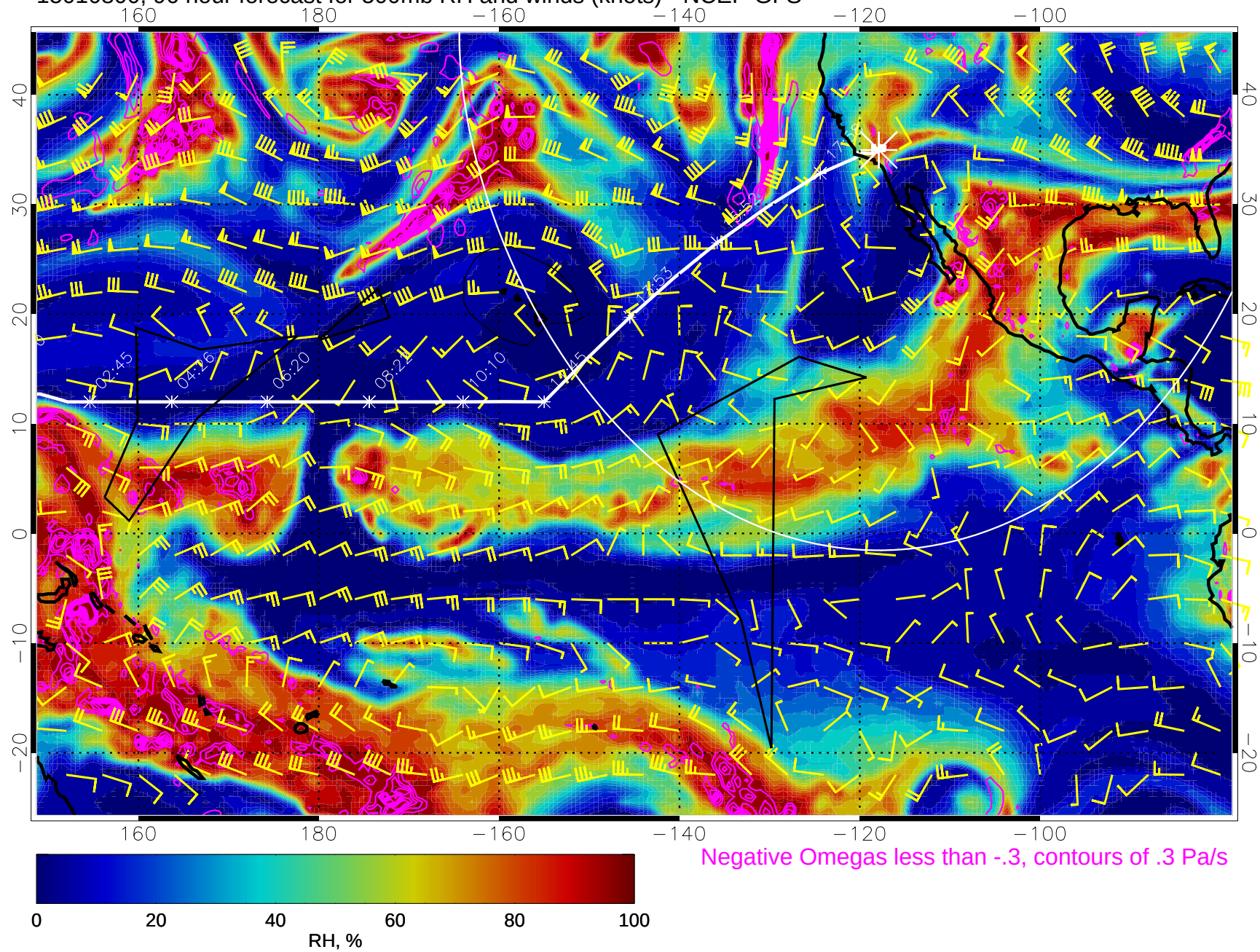
15010800, 96 hour forecast for 500mb RH and winds (knots) - NCEP GFS
