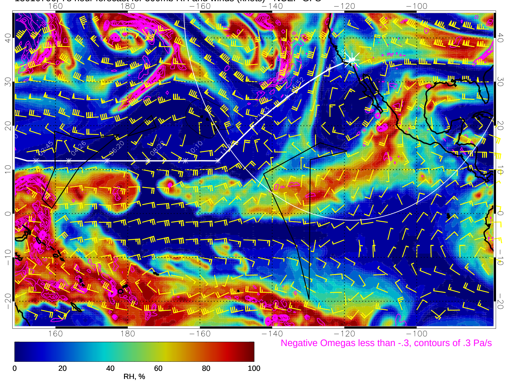
15010706, 78 hour forecast for 500mb RH and winds (knots) - NCEP GFS
