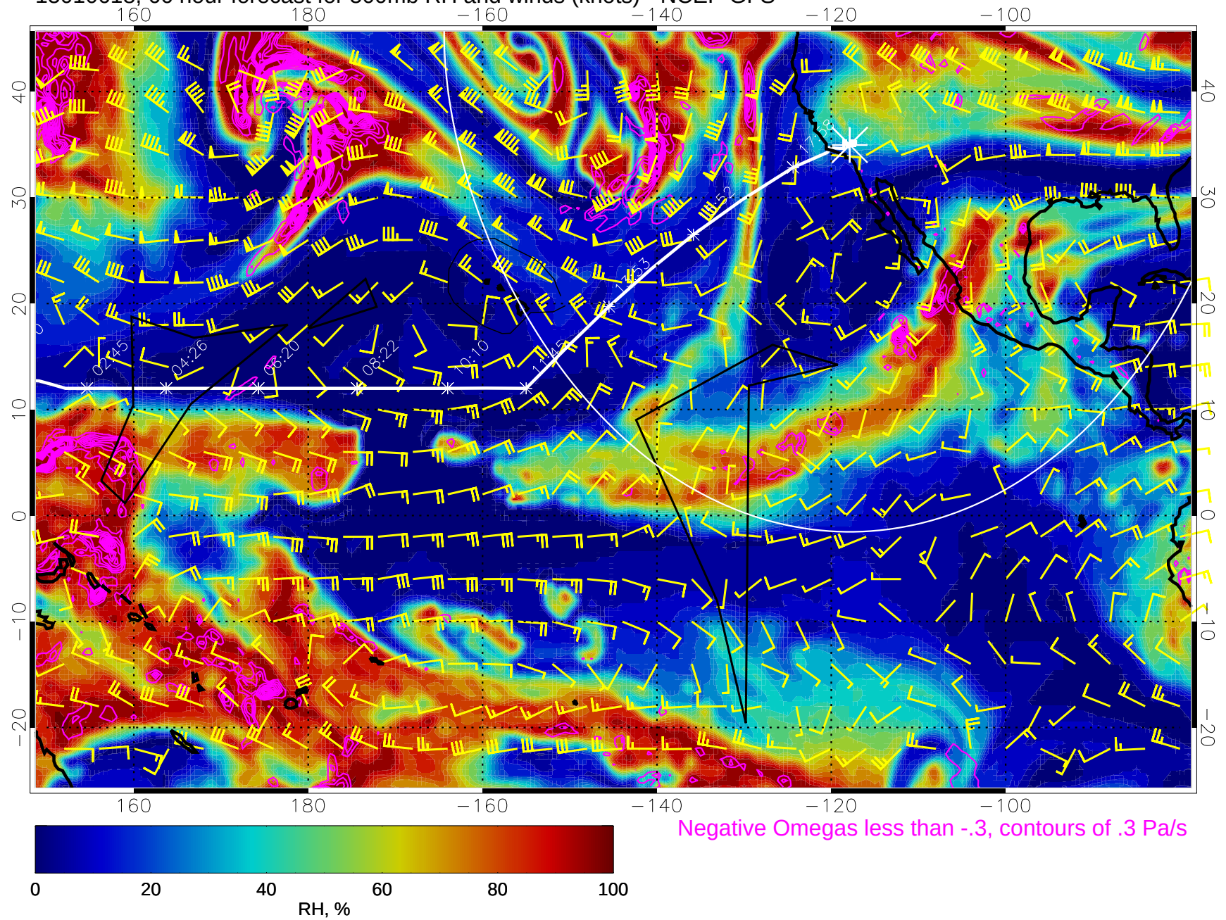
15010618, 66 hour forecast for 500mb RH and winds (knots) - NCEP GFS
