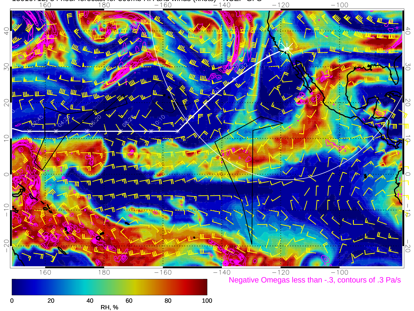
15010712, 84 hour forecast for 500mb RH and winds (knots) - NCEP GFS
