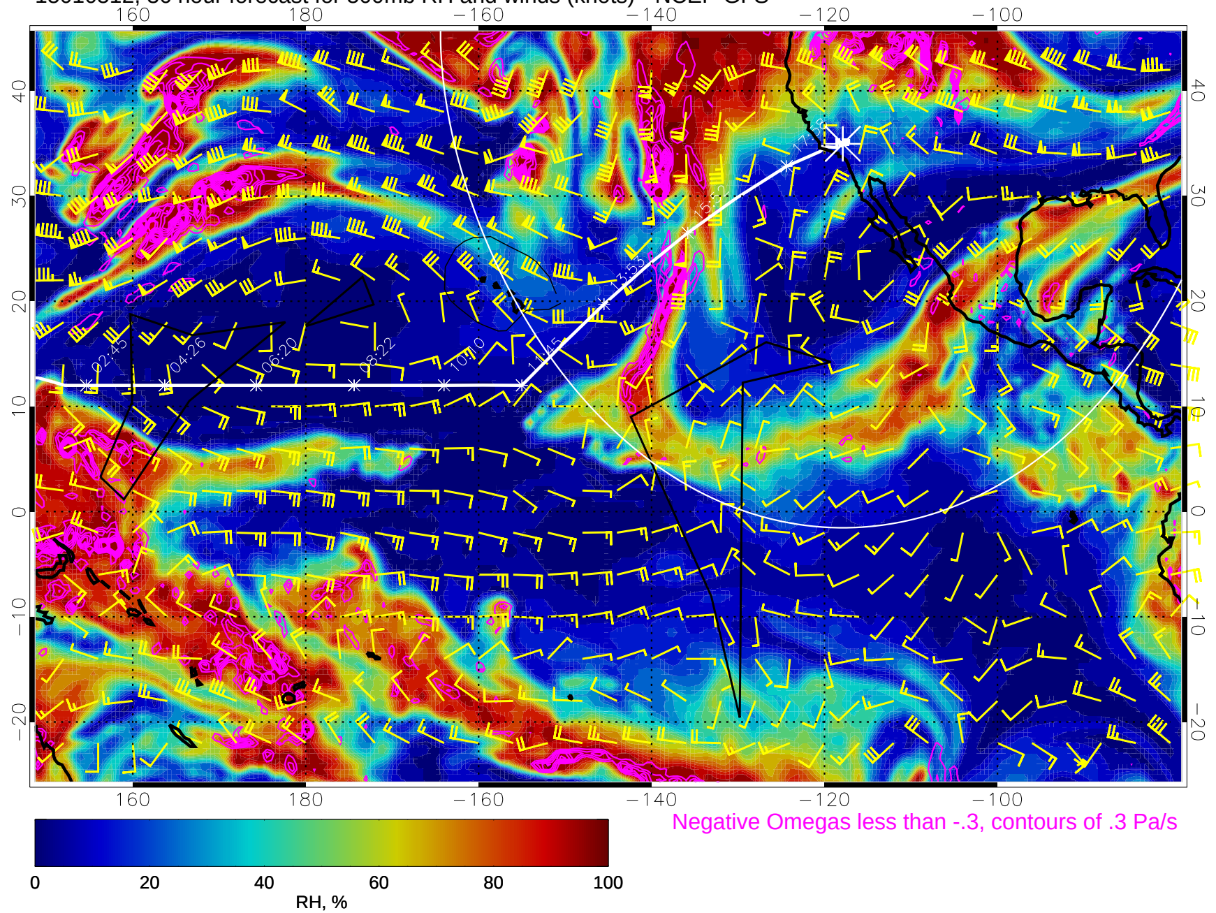
15010512, 36 hour forecast for 500mb RH and winds (knots) - NCEP GFS
