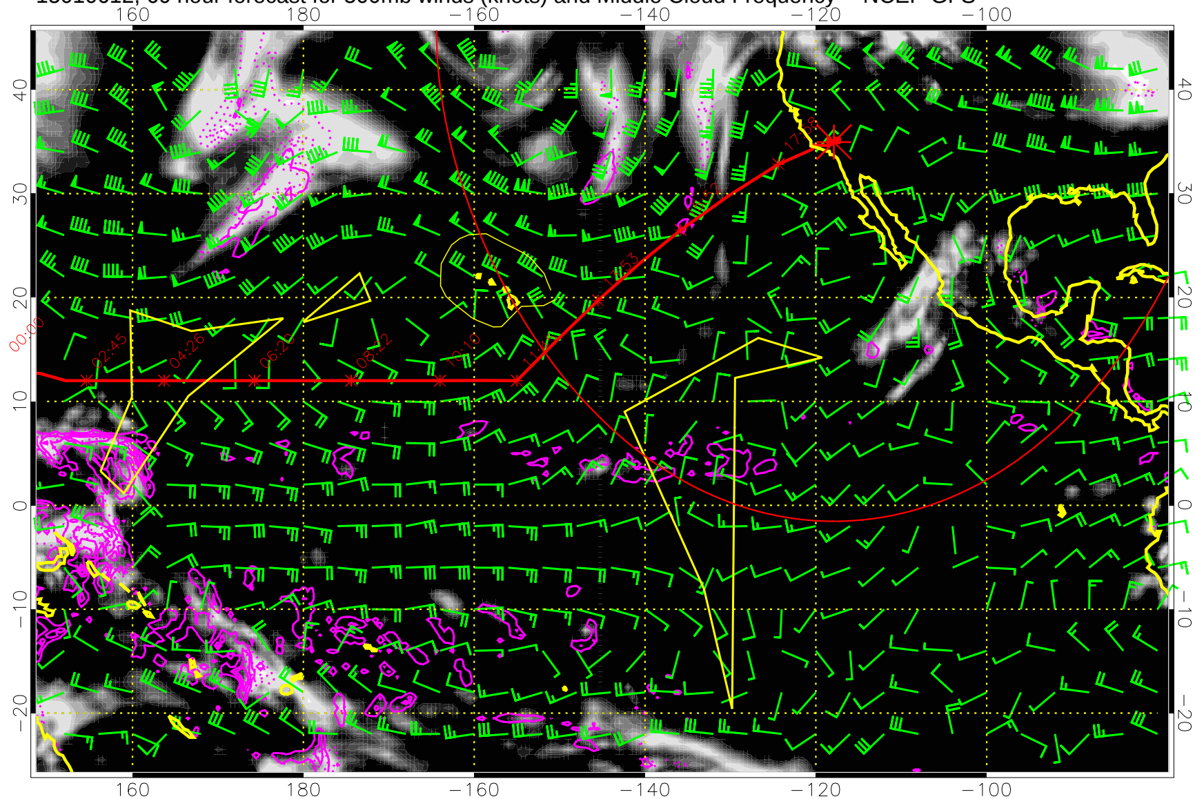
15010612, 60 hour forecast for 500mb winds (knots) and Middle Cloud Frequency -- NCEP GFS
