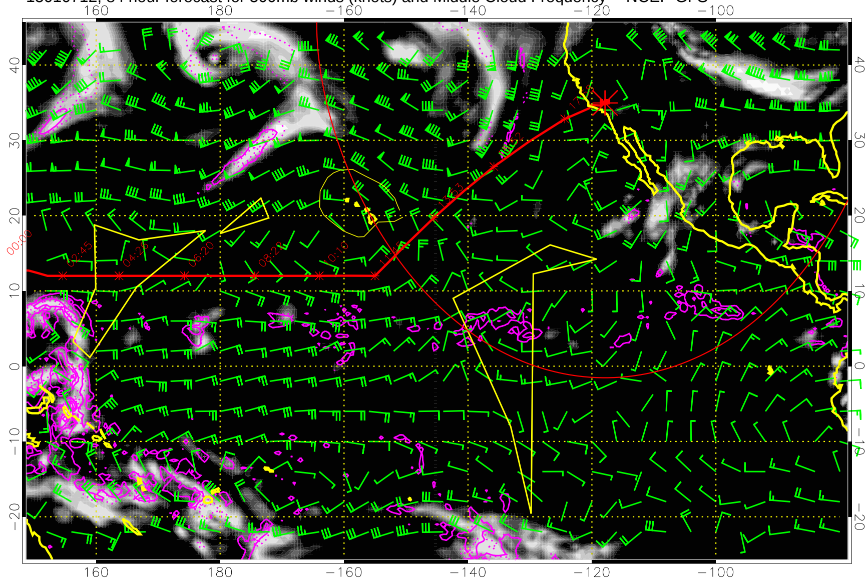
15010712, 84 hour forecast for 500mb winds (knots) and Middle Cloud Frequency -- NCEP GFS
