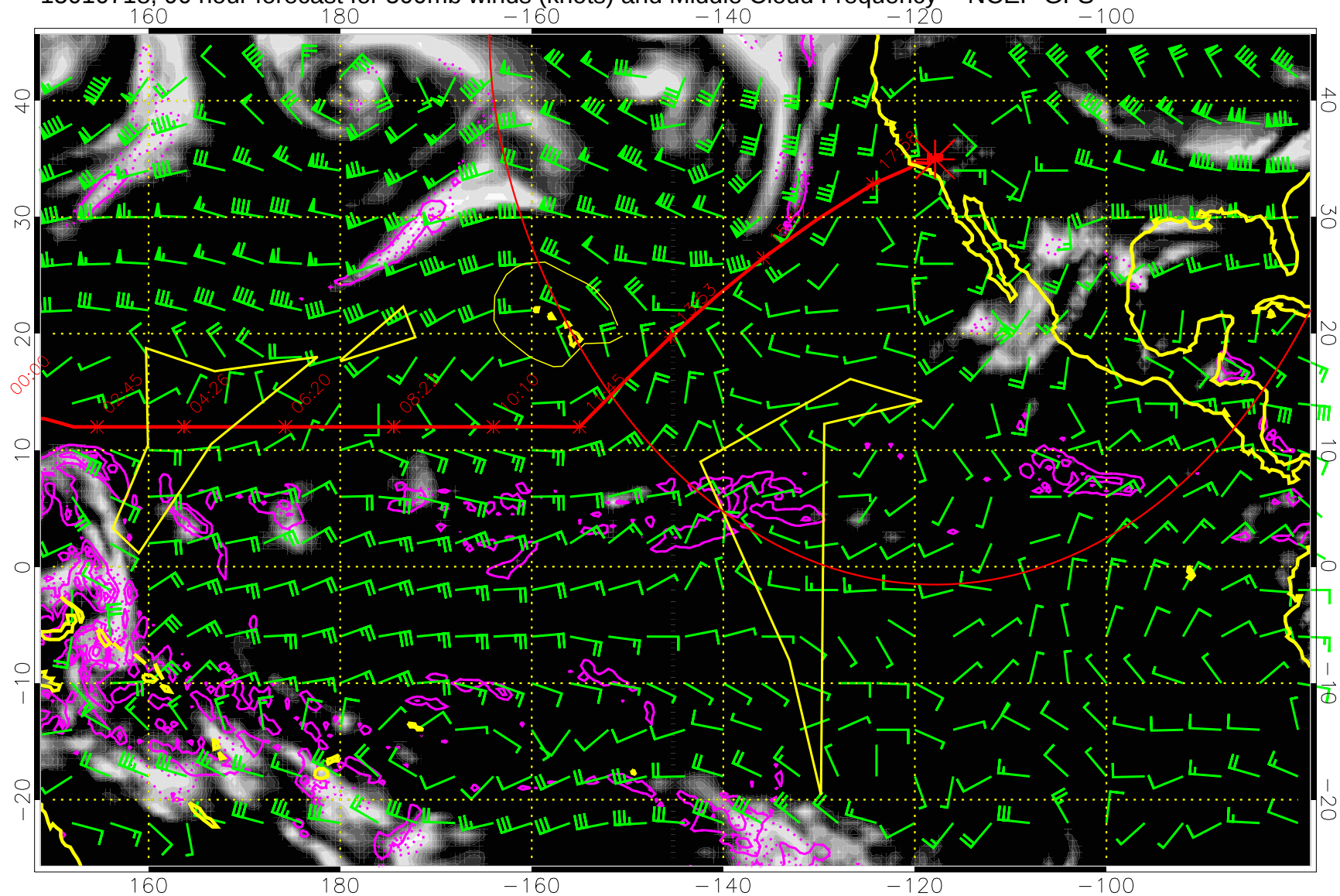
15010718, 90 hour forecast for 500mb winds (knots) and Middle Cloud Frequency -- NCEP GFS
