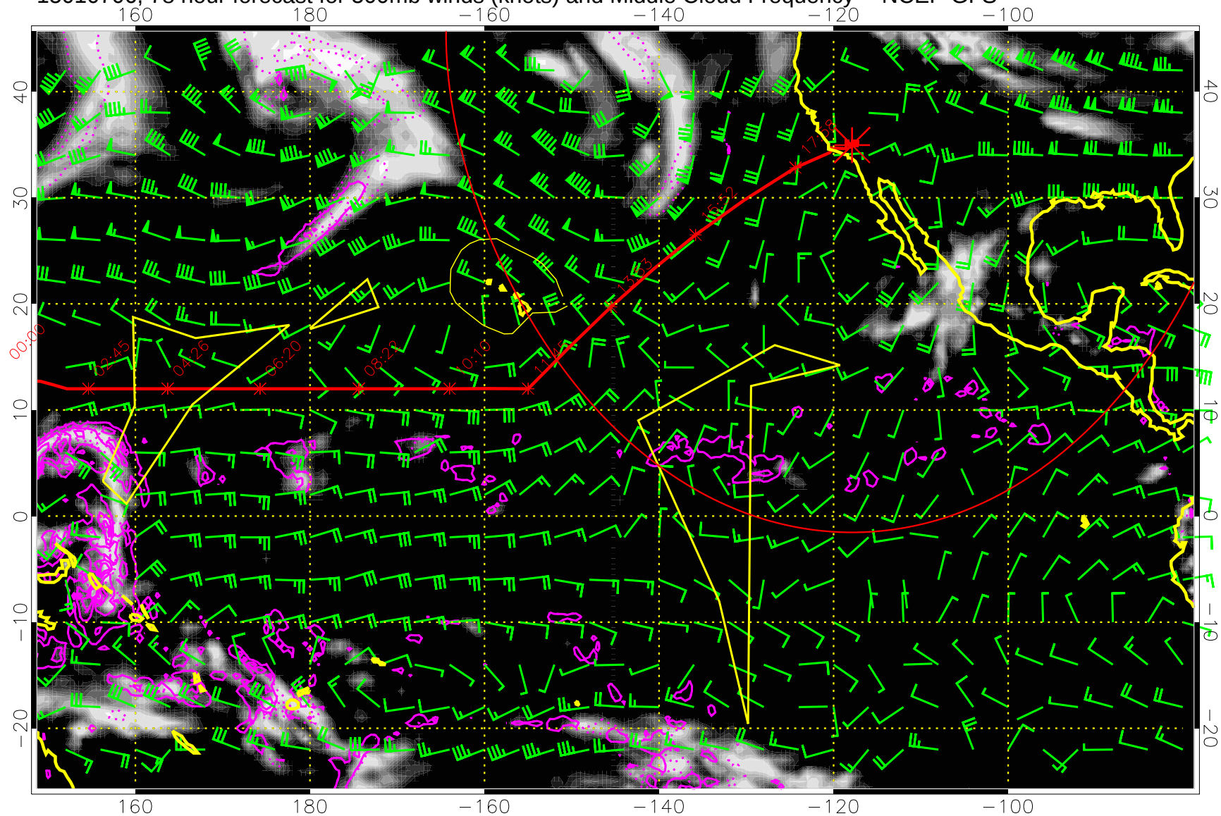
15010706, 78 hour forecast for 500mb winds (knots) and Middle Cloud Frequency -- NCEP GFS
