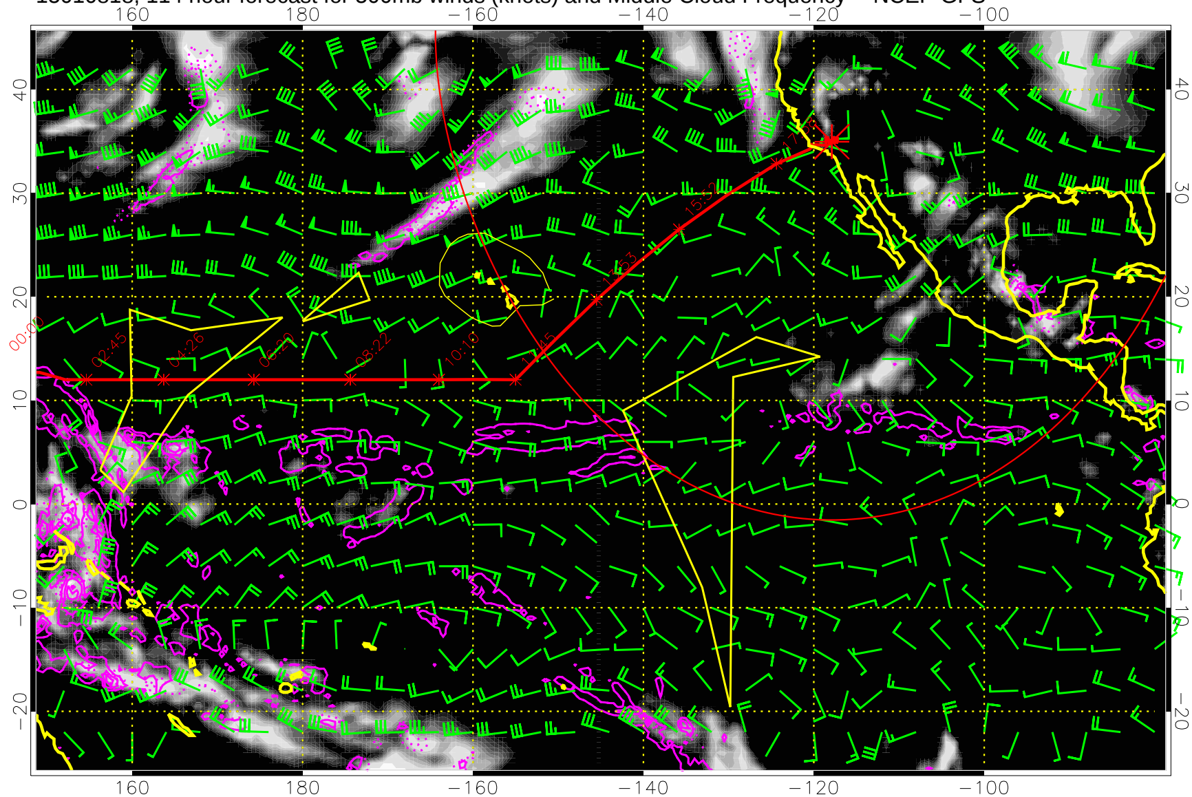
15010818, 114 hour forecast for 500mb winds (knots) and Middle Cloud Frequency -- NCEP GFS
