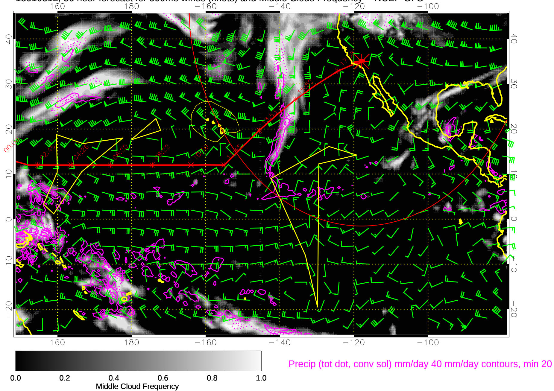
15010512, 36 hour forecast for 500mb winds (knots) and Middle Cloud Frequency -- NCEP GFS
