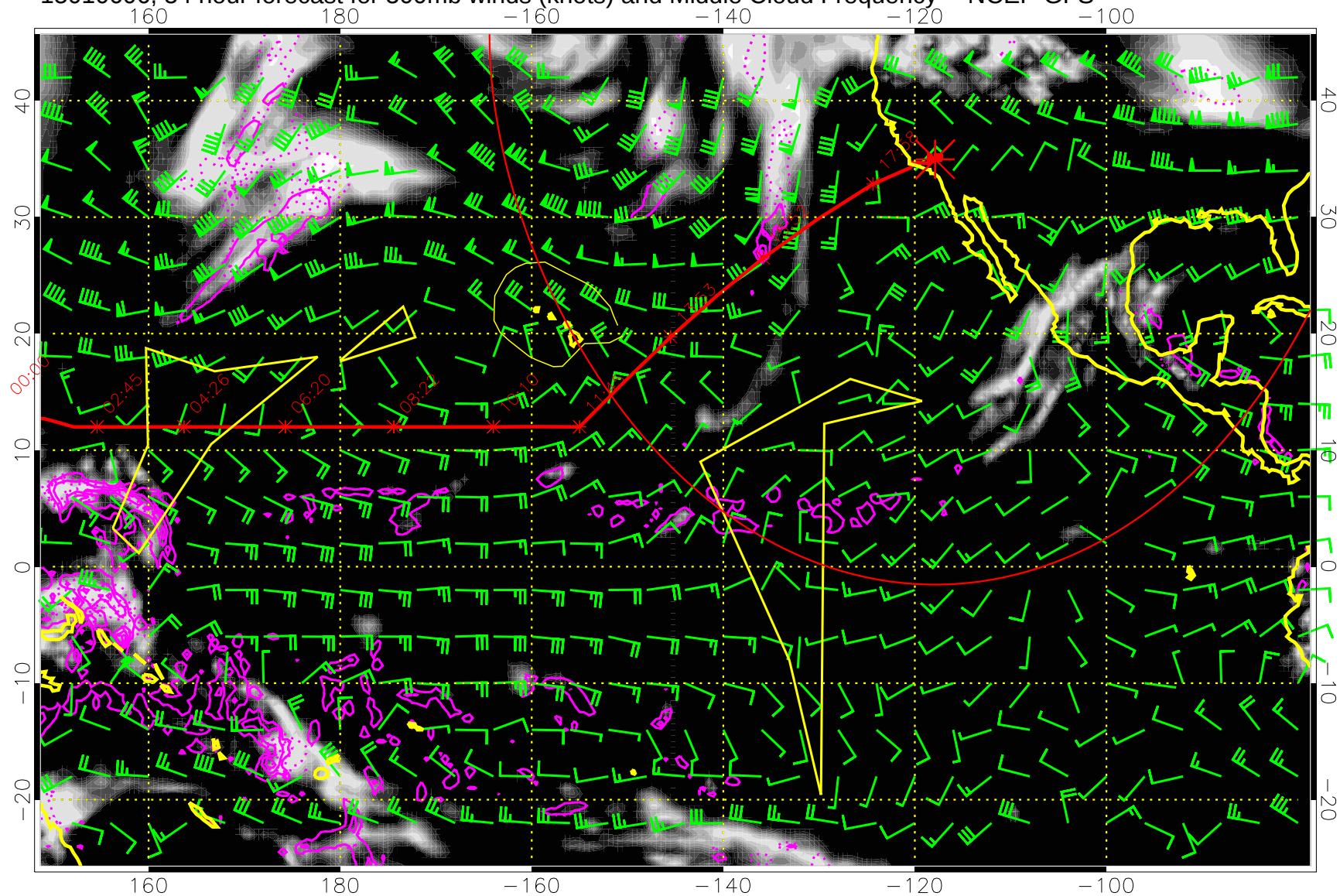
15010606, 54 hour forecast for 500mb winds (knots) and Middle Cloud Frequency -- NCEP GFS
