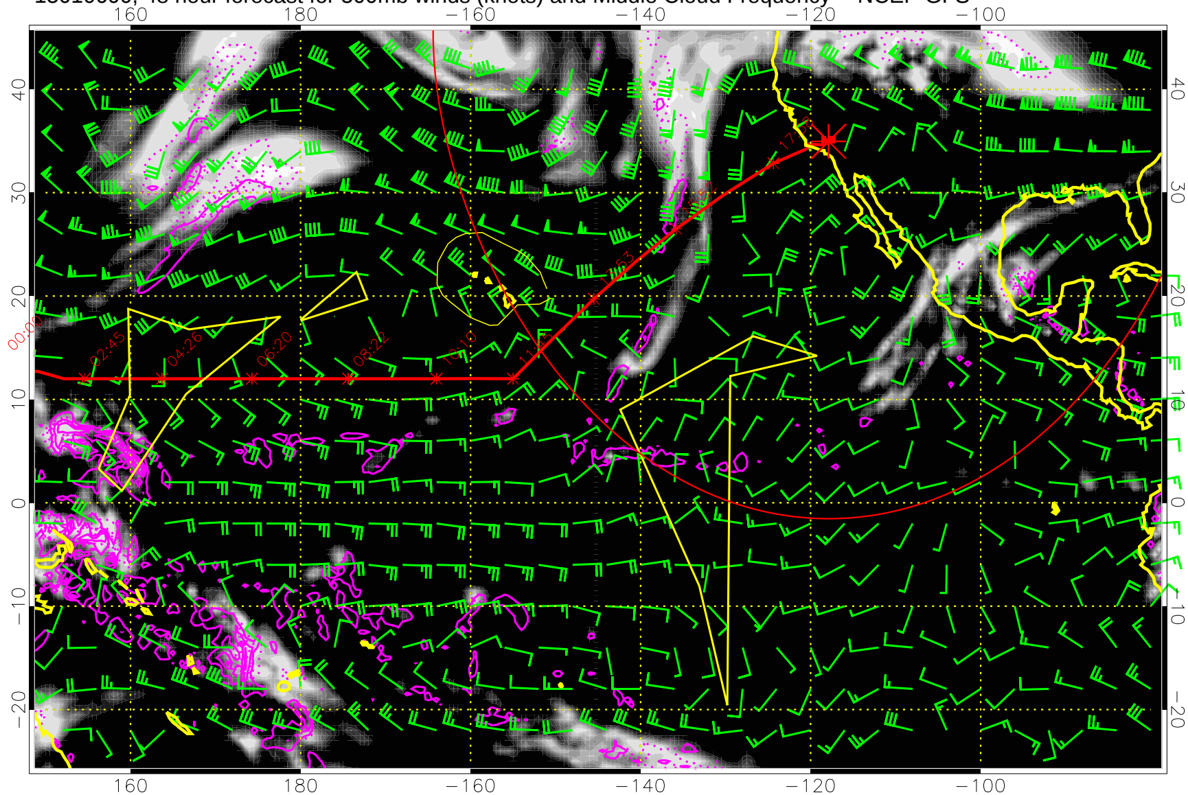
15010600, 48 hour forecast for 500mb winds (knots) and Middle Cloud Frequency -- NCEP GFS
