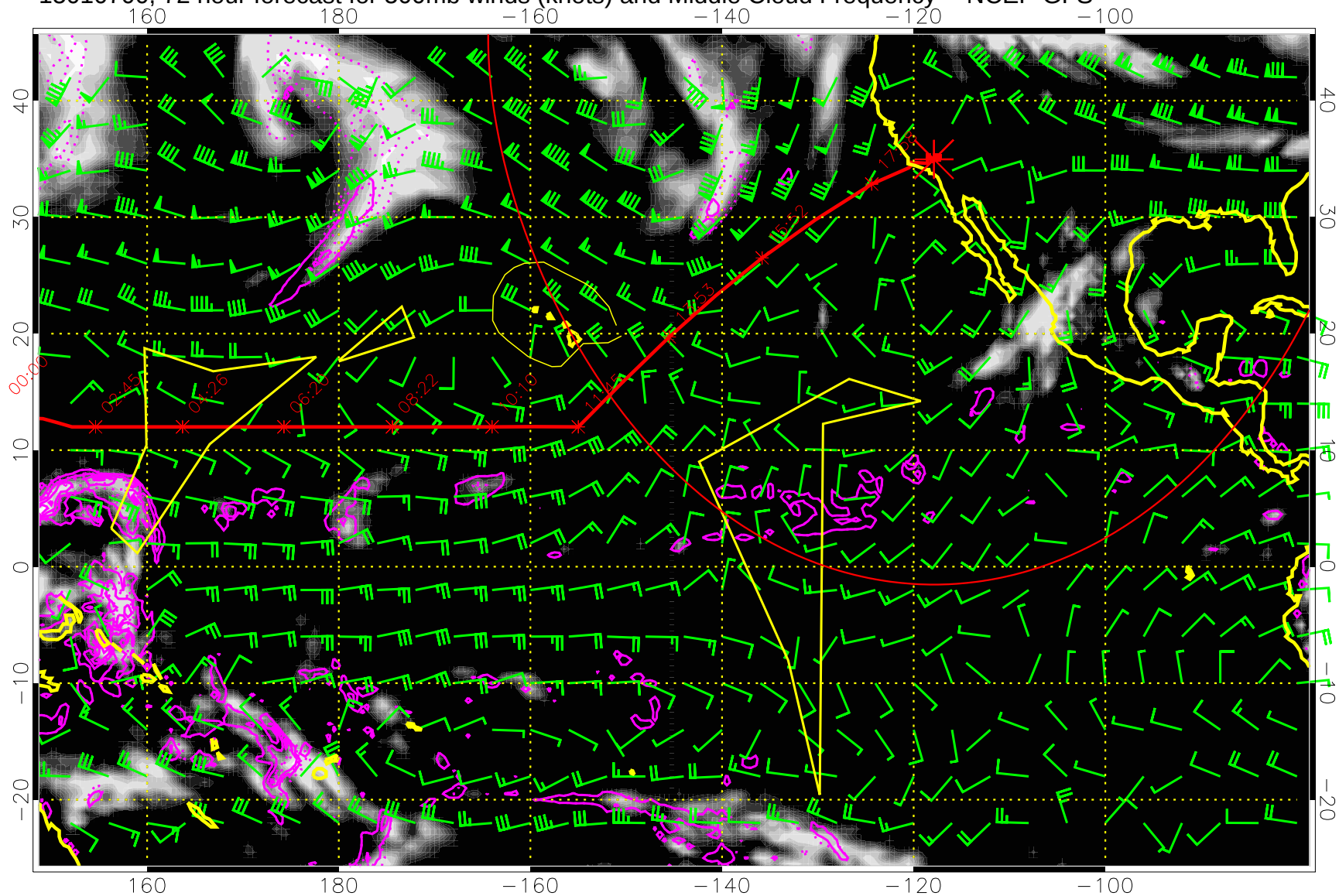
15010700, 72 hour forecast for 500mb winds (knots) and Middle Cloud Frequency -- NCEP GFS
