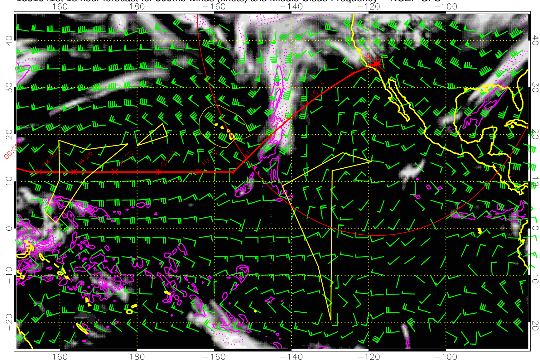
15010418, 18 hour forecast for 500mb winds (knots) and Middle Cloud Frequency -- NCEP GFS
