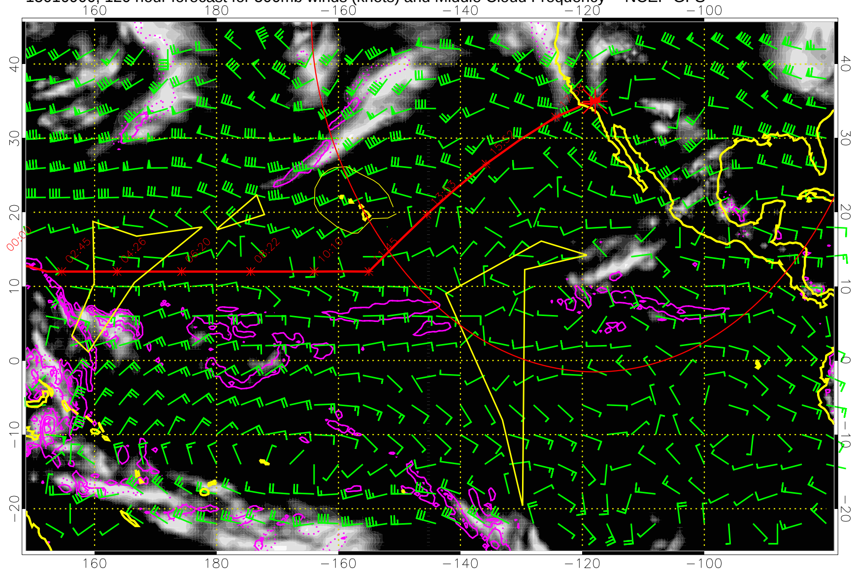
15010900, 120 hour forecast for 500mb winds (knots) and Middle Cloud Frequency -- NCEP GFS
