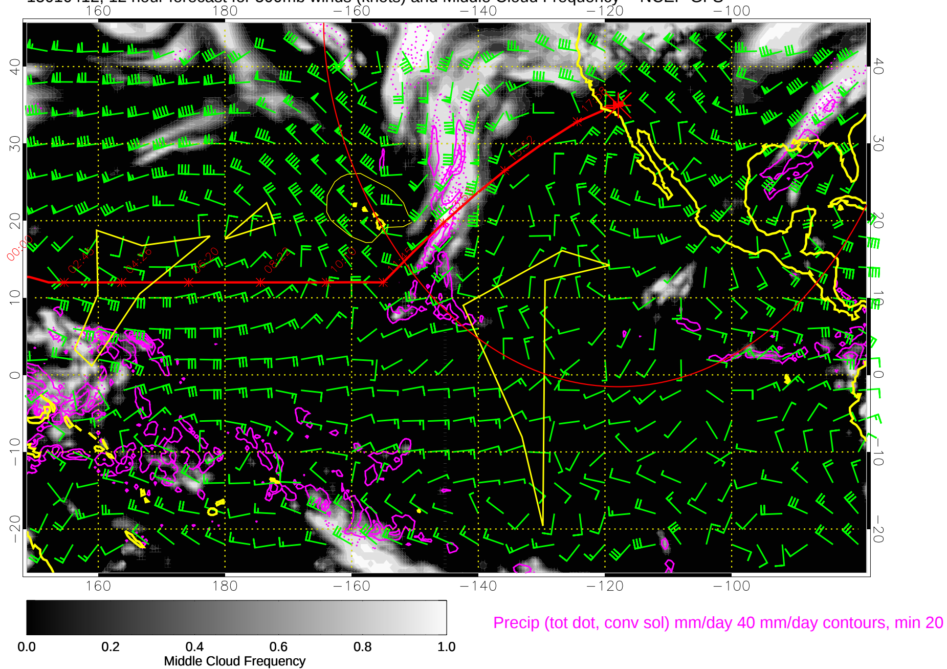
15010412, 12 hour forecast for 500mb winds (knots) and Middle Cloud Frequency -- NCEP GFS
