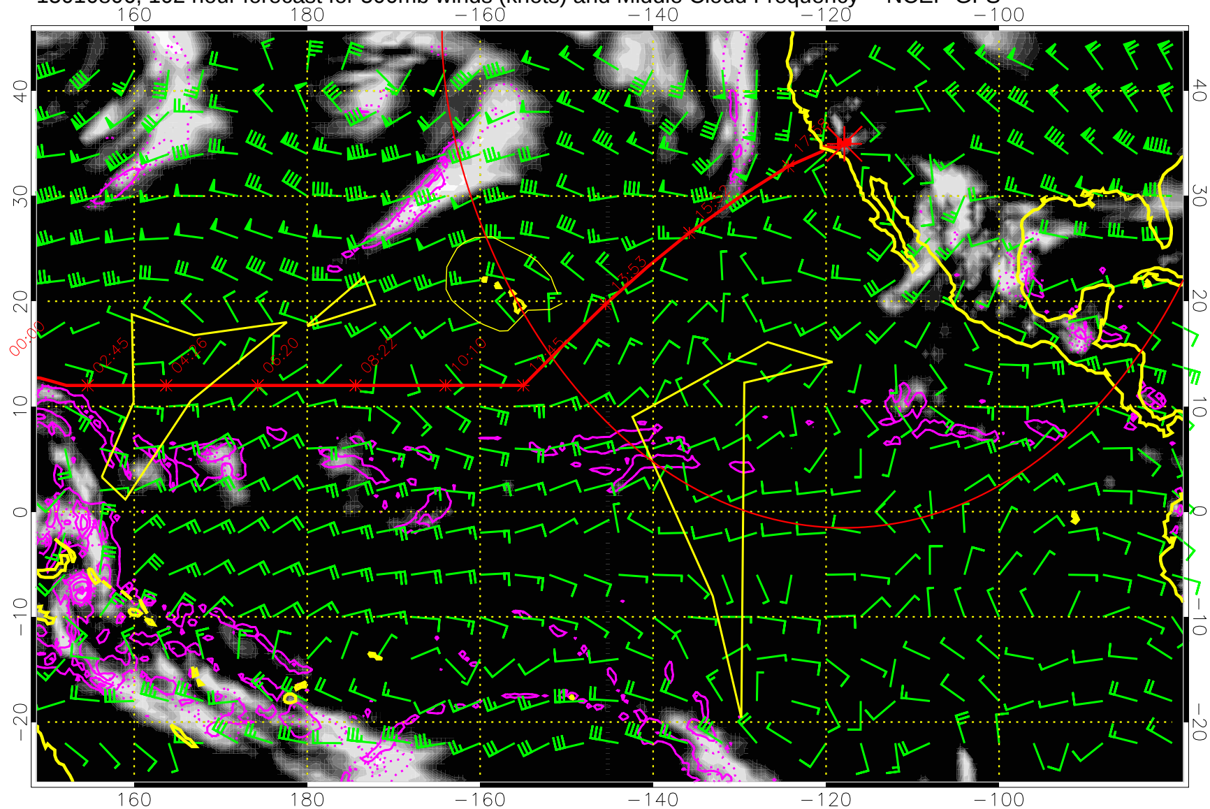
15010806, 102 hour forecast for 500mb winds (knots) and Middle Cloud Frequency -- NCEP GFS
