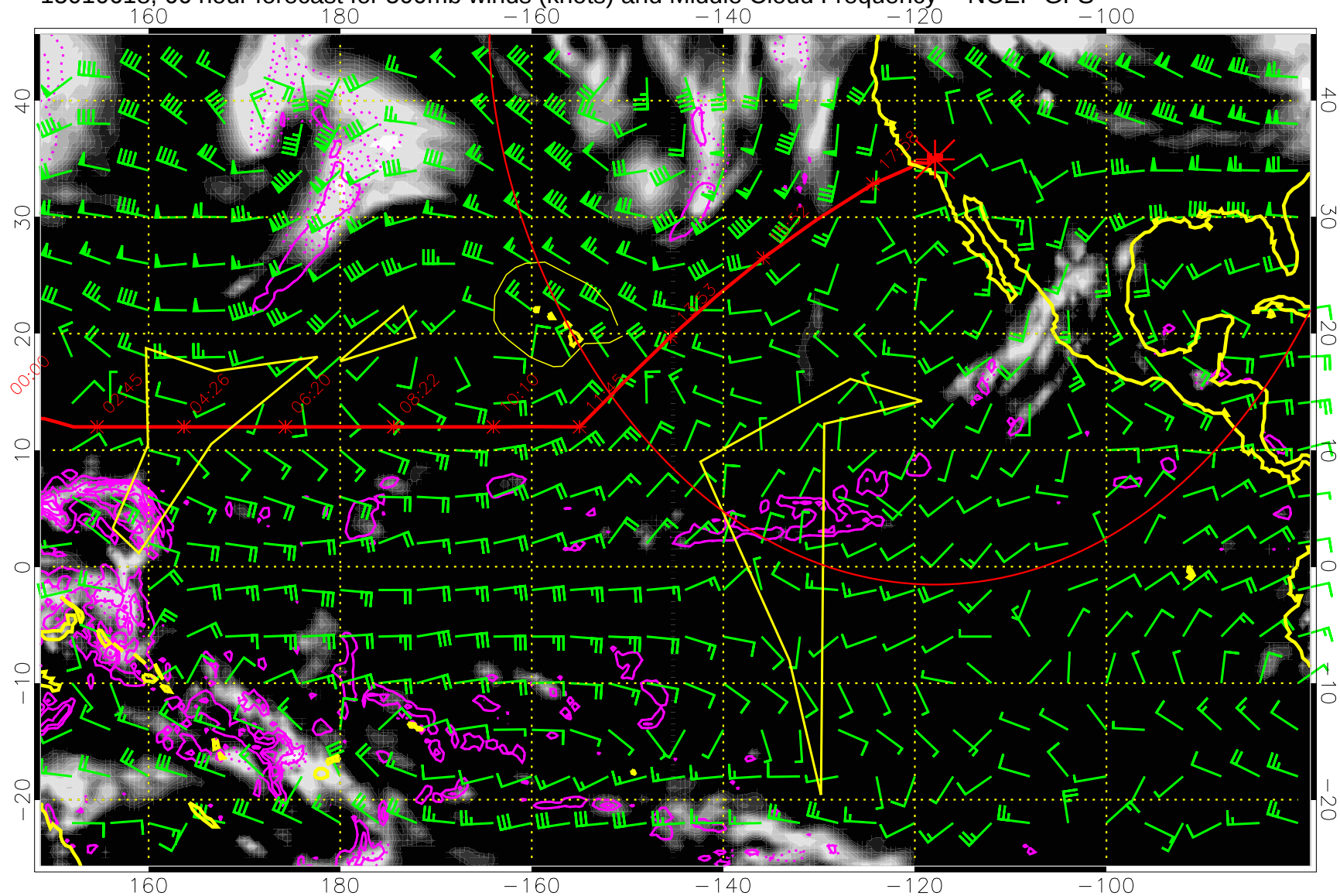
15010618, 66 hour forecast for 500mb winds (knots) and Middle Cloud Frequency -- NCEP GFS
