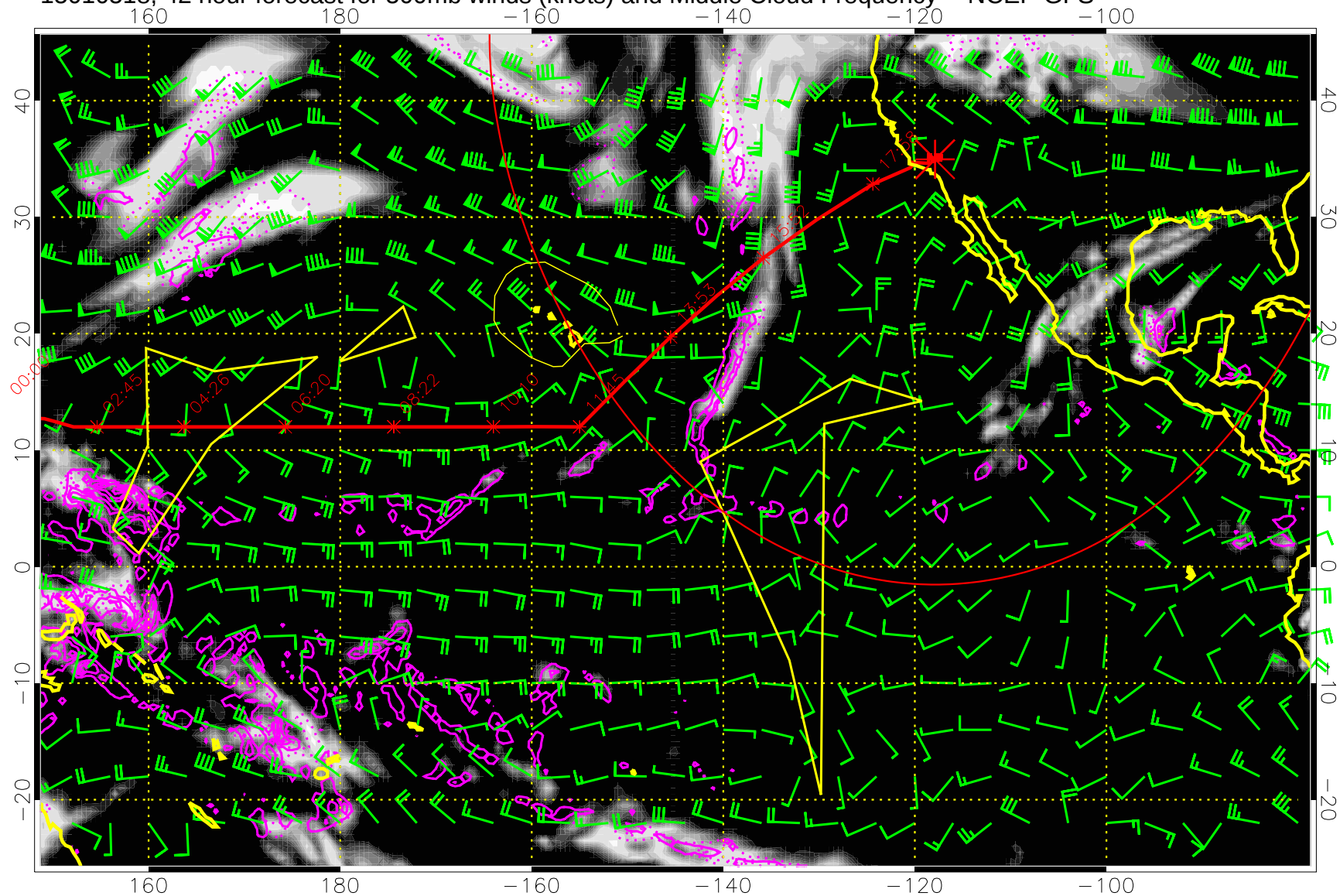
15010518, 42 hour forecast for 500mb winds (knots) and Middle Cloud Frequency -- NCEP GFS
