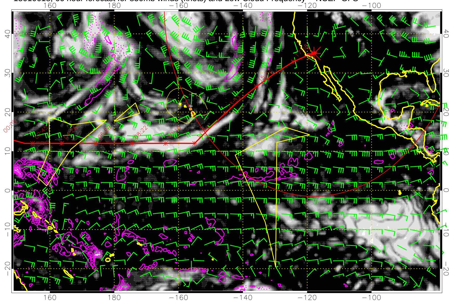
15010618, 66 hour forecast for 850mb winds (knots) and Low Cloud Frequency -- NCEP GFS
