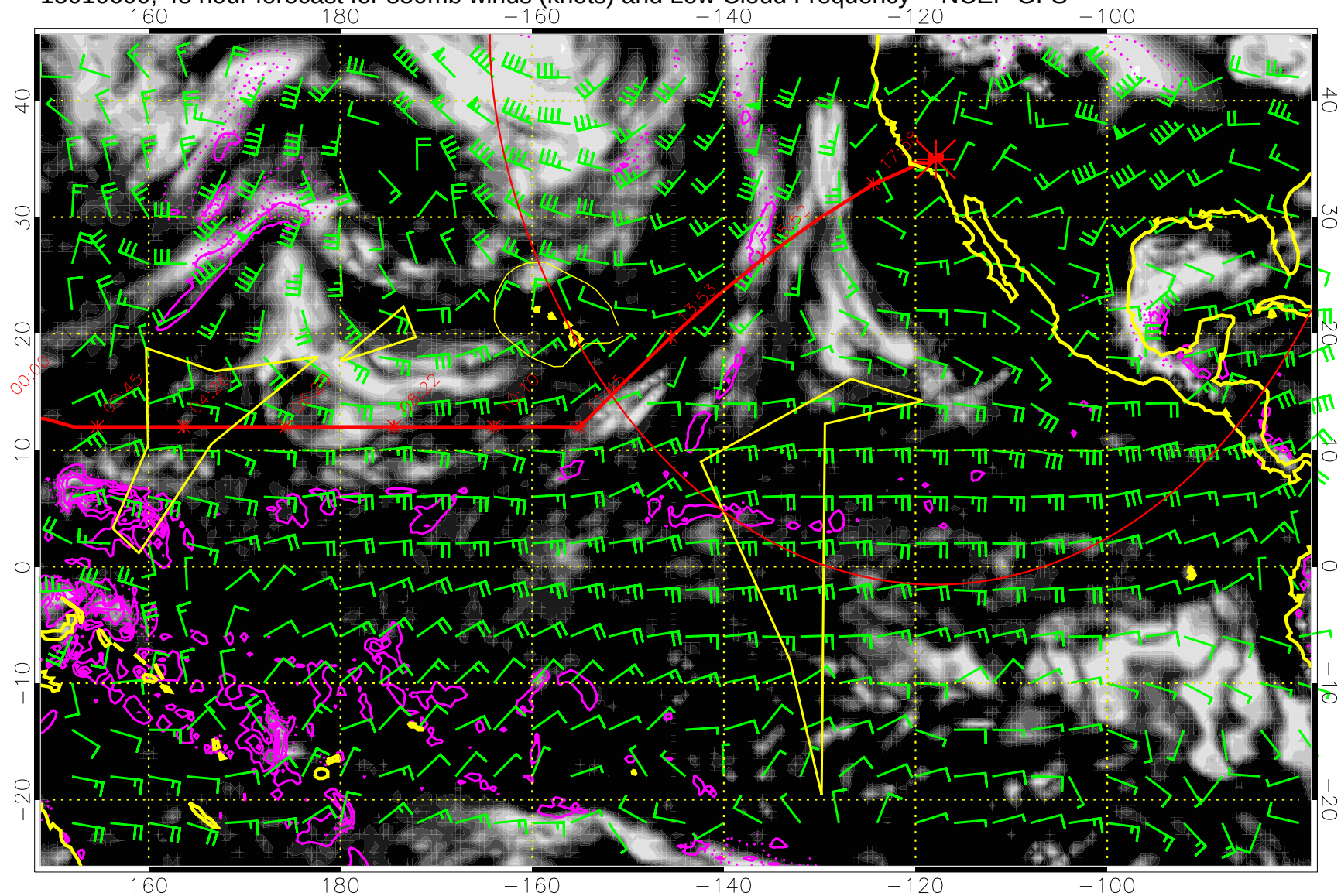
15010600, 48 hour forecast for 850mb winds (knots) and Low Cloud Frequency -- NCEP GFS
