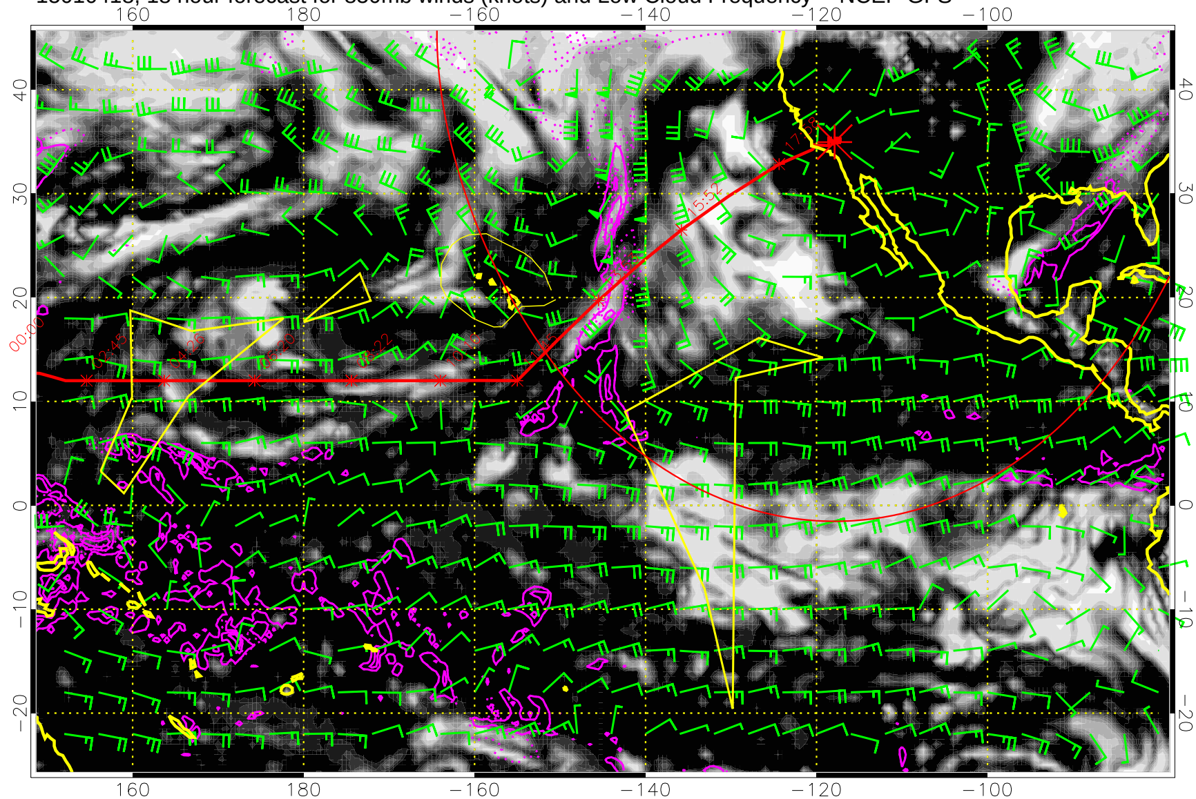
15010418, 18 hour forecast for 850mb winds (knots) and Low Cloud Frequency -- NCEP GFS
