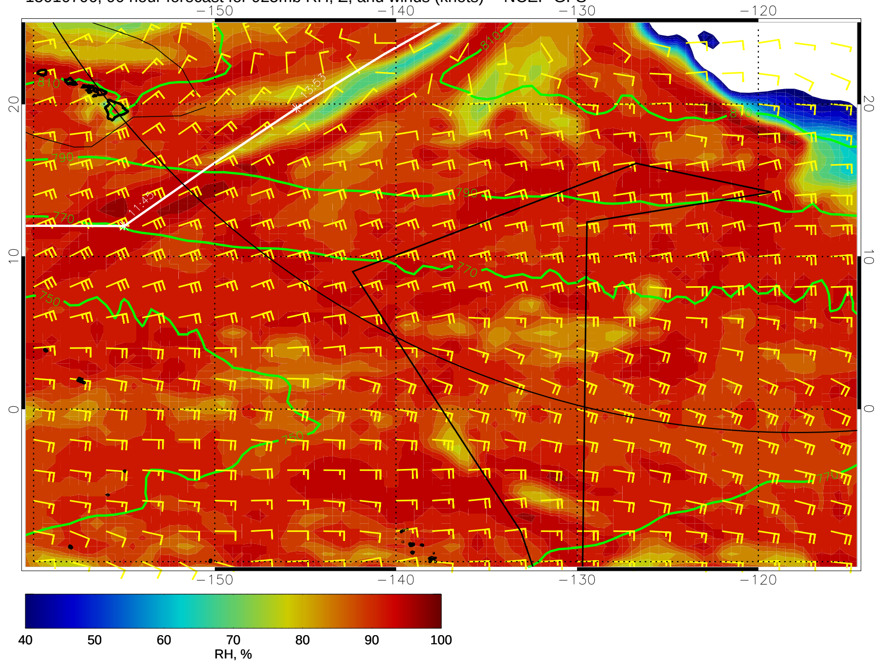
15010706, 90 hour forecast for 925mb RH, Z, and winds (knots) -- NCEP GFS
