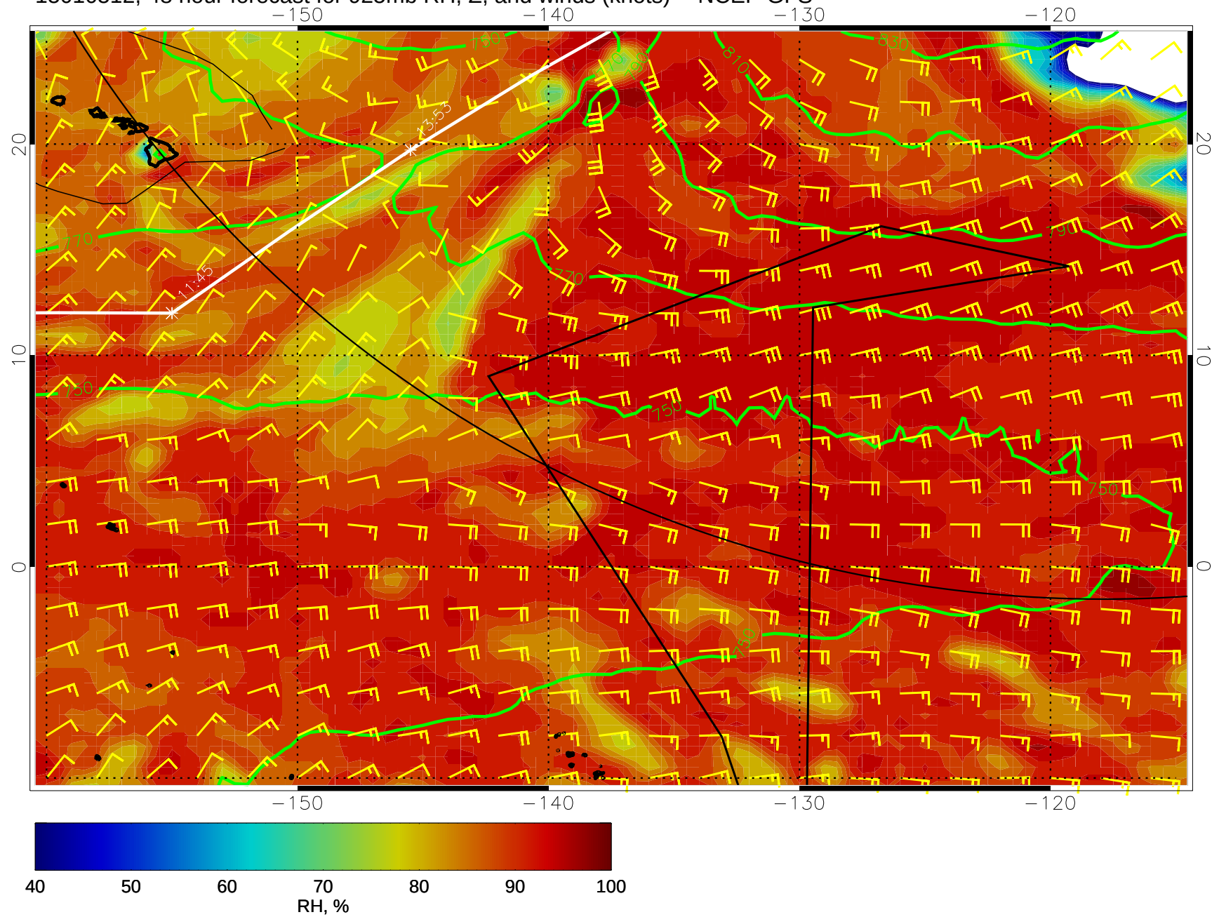
15010512, 48 hour forecast for 925mb RH, Z, and winds (knots) -- NCEP GFS
