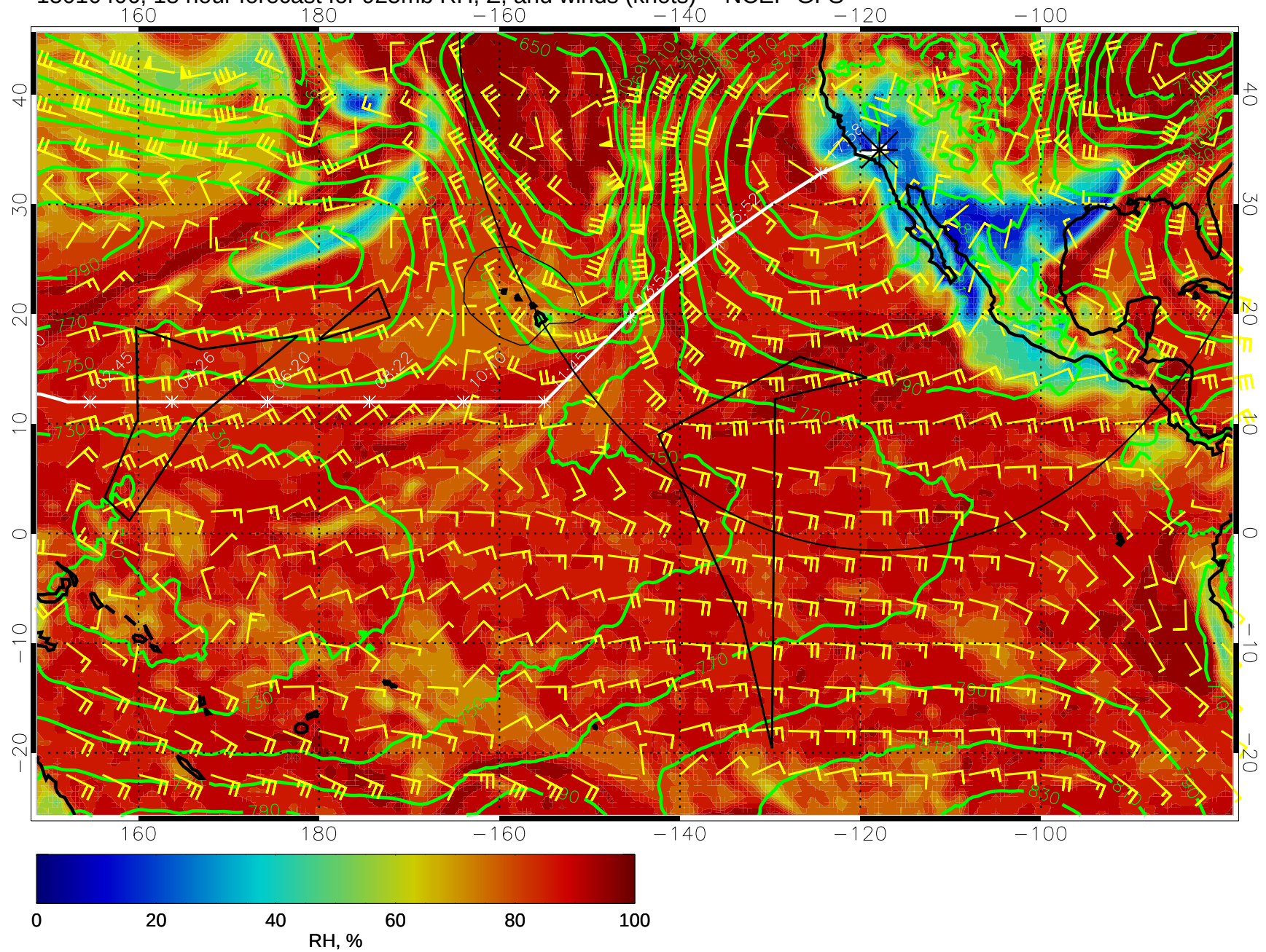
15010406, 18 hour forecast for 925mb RH, Z, and winds (knots) -- NCEP GFS
