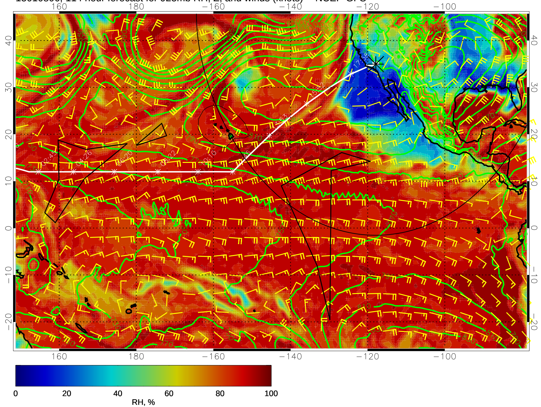
15010806, 114 hour forecast for 925mb RH, Z, and winds (knots) -- NCEP GFS
