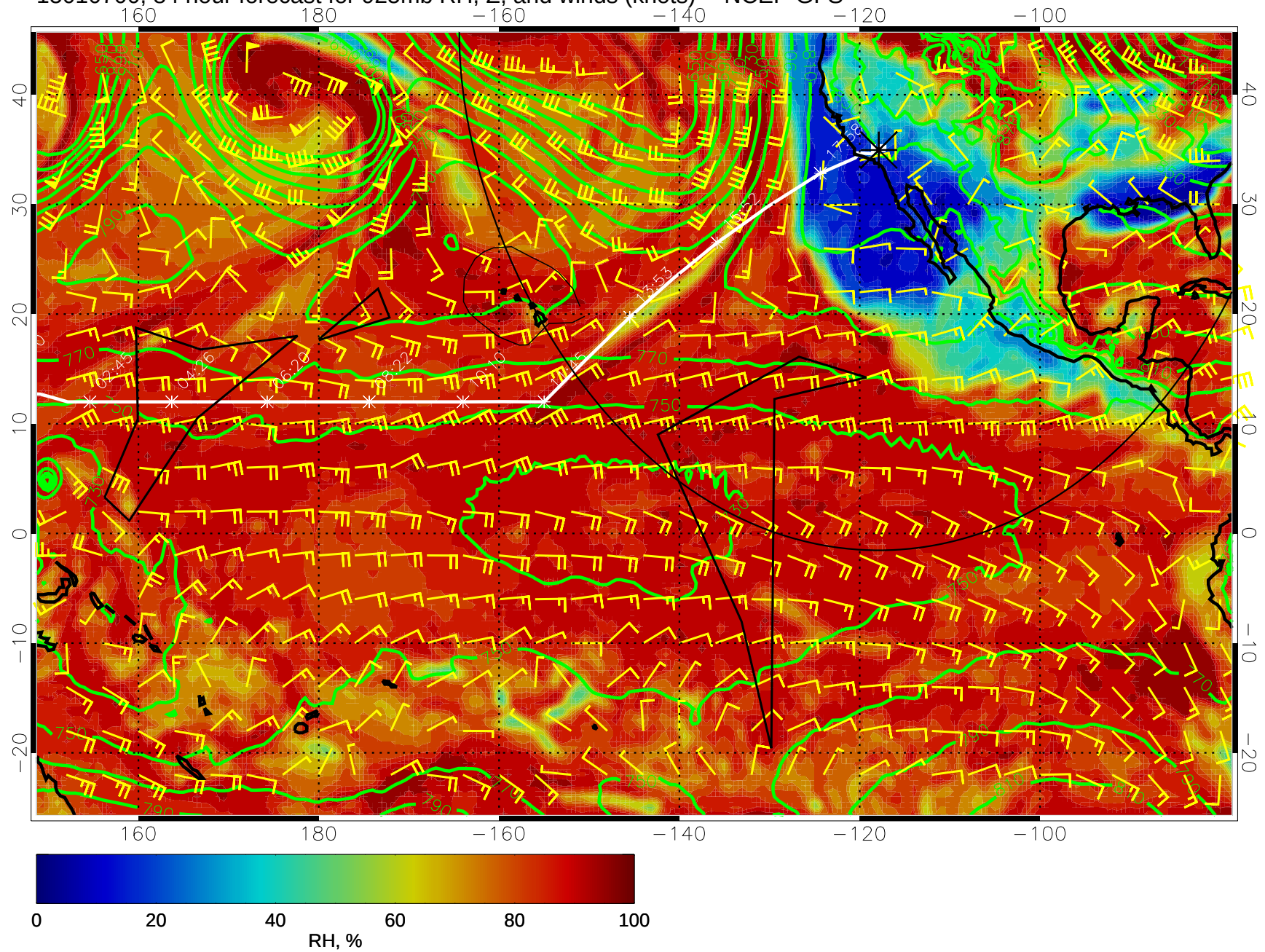
15010700, 84 hour forecast for 925mb RH, Z, and winds (knots) -- NCEP GFS
