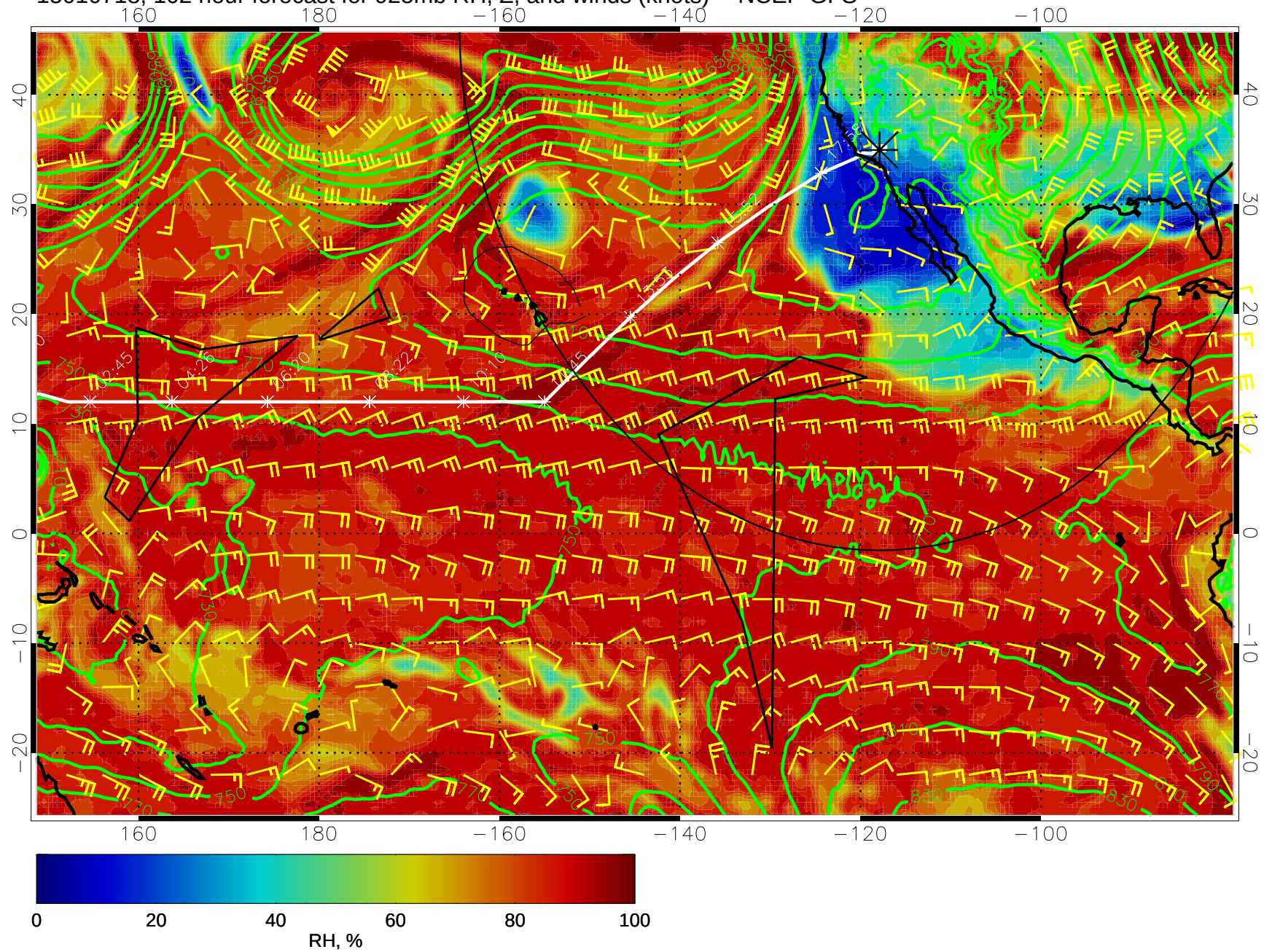
15010718, 102 hour forecast for 925mb RH, Z, and winds (knots) -- NCEP GFS
