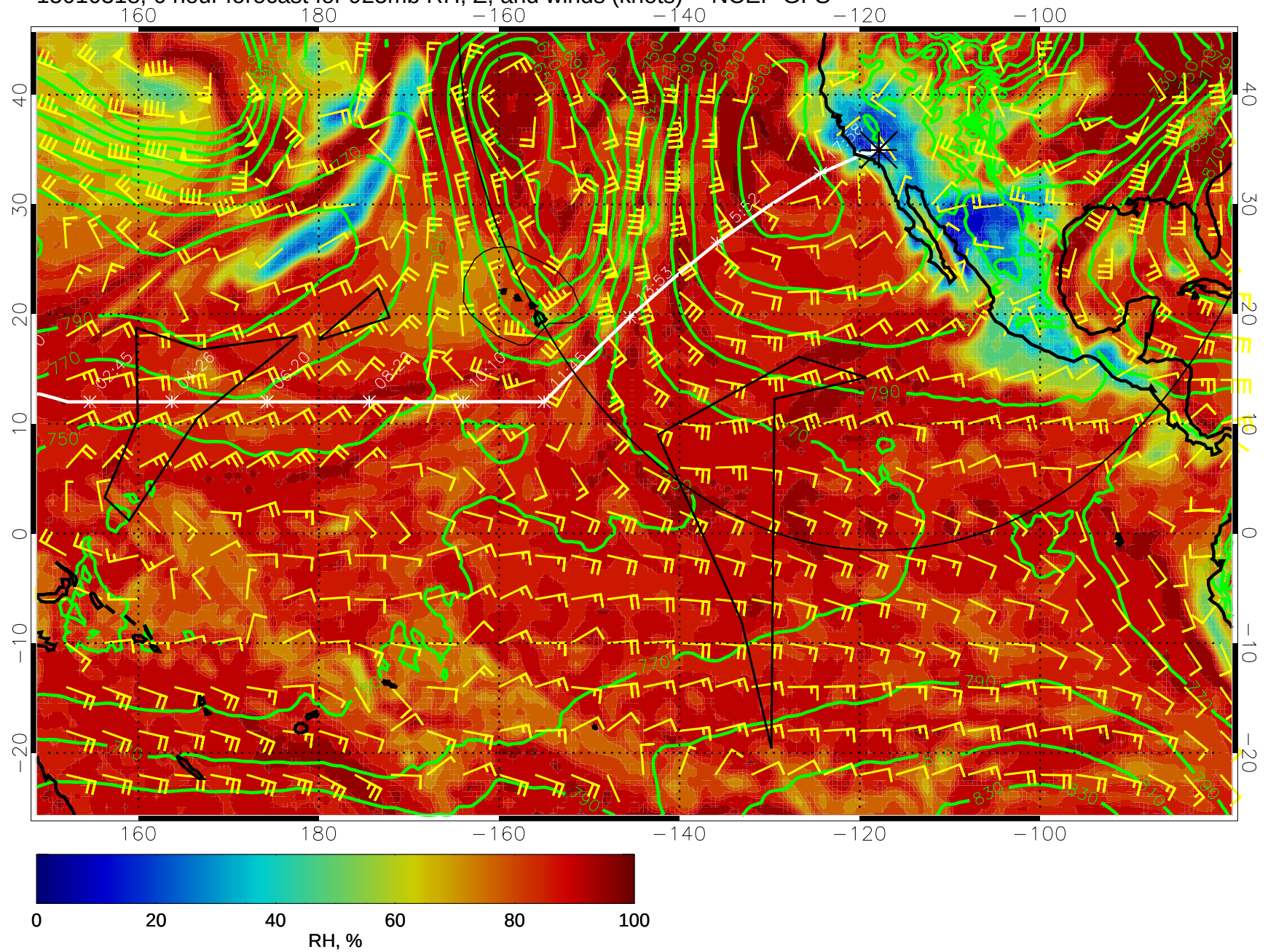
15010318, 6 hour forecast for 925mb RH, Z, and winds (knots) -- NCEP GFS
