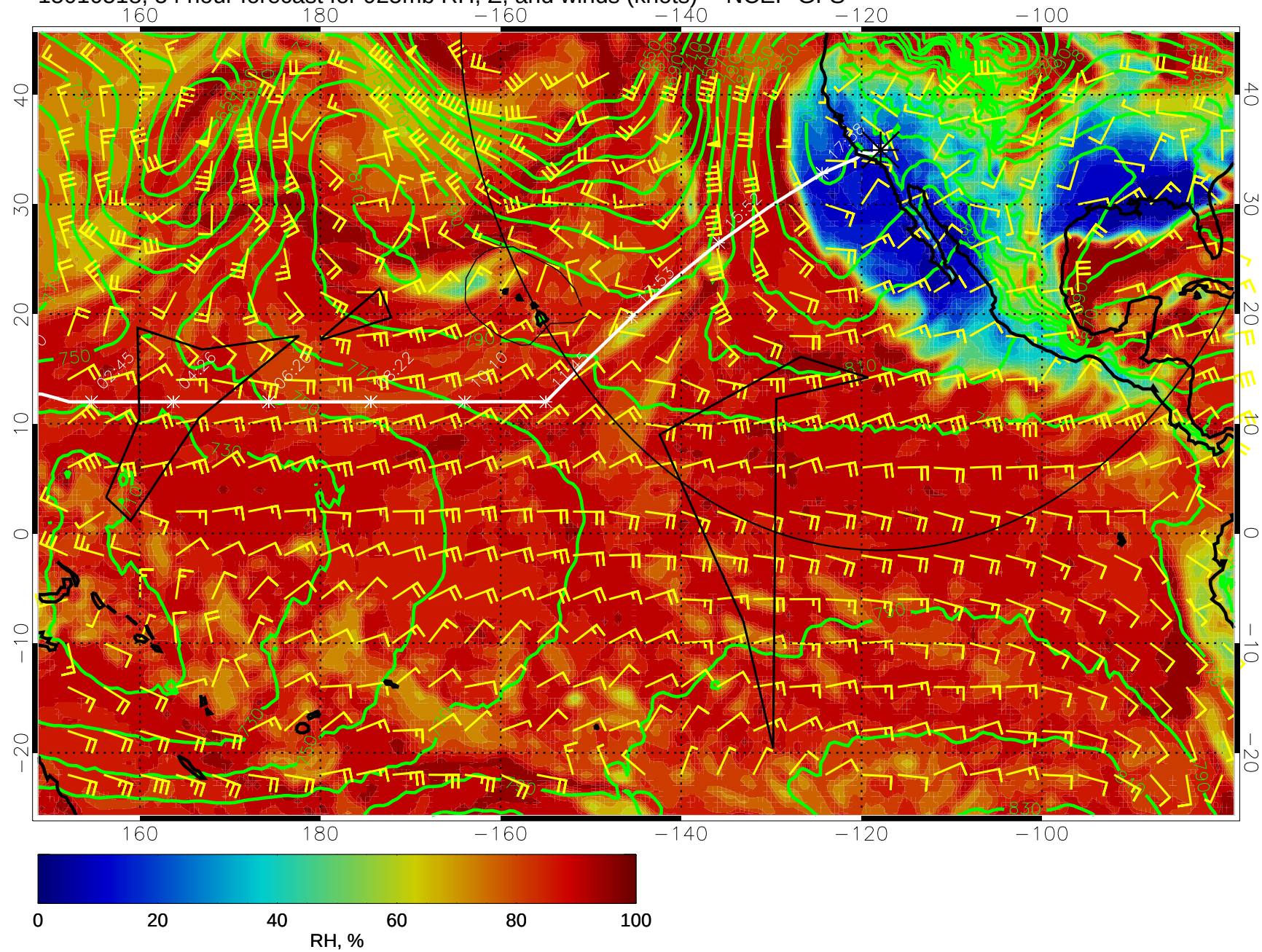
15010518, 54 hour forecast for 925mb RH, Z, and winds (knots) -- NCEP GFS
