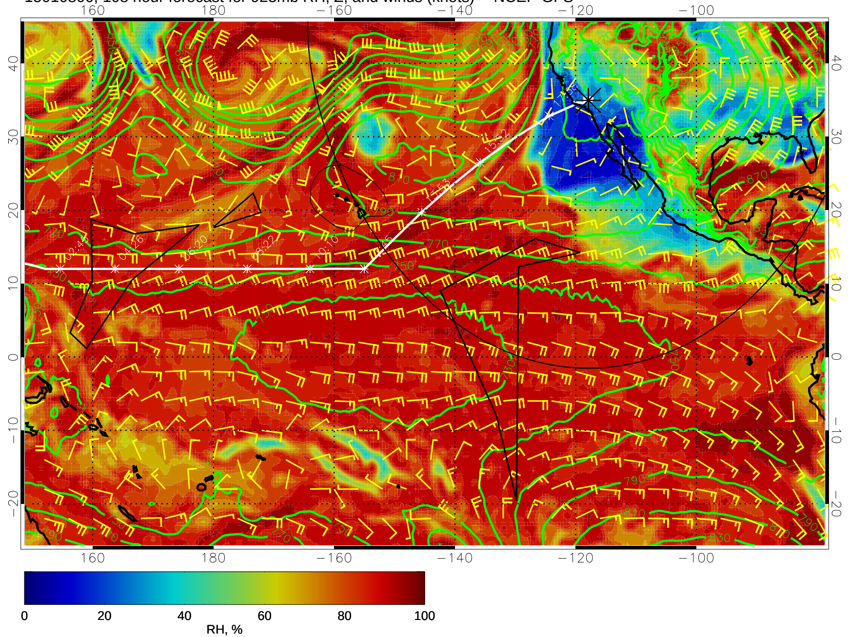
15010800, 108 hour forecast for 925mb RH, Z, and winds (knots) -- NCEP GFS
