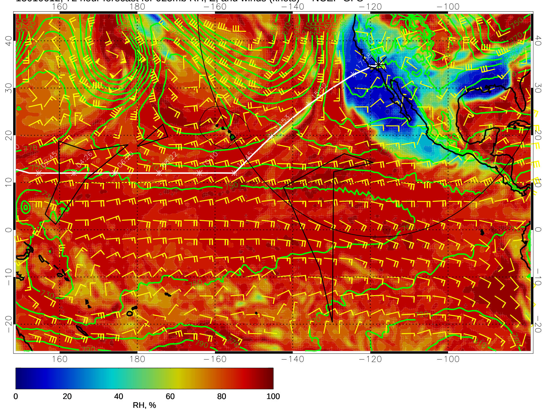
15010612, 72 hour forecast for 925mb RH, Z, and winds (knots) -- NCEP GFS
