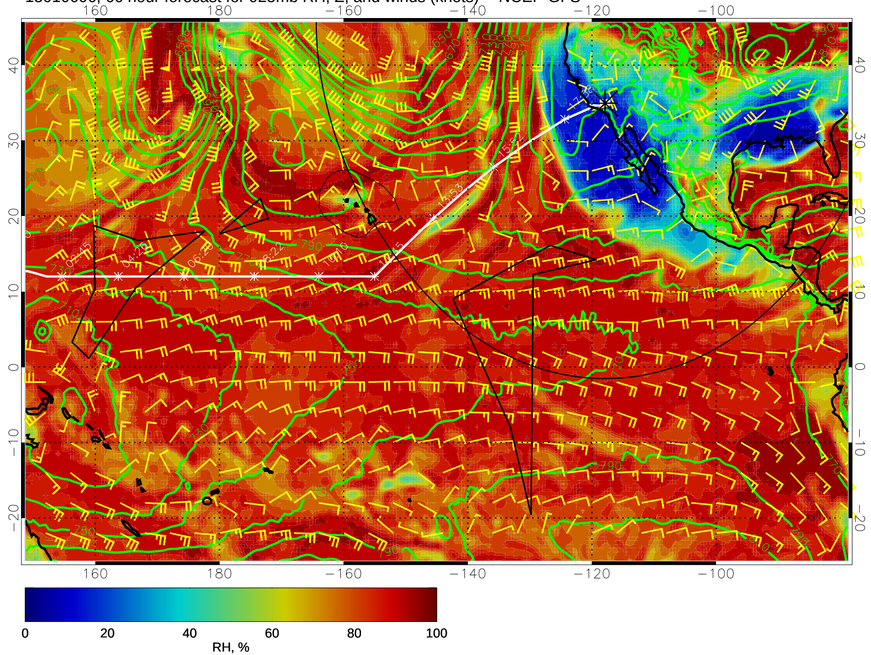
15010606, 66 hour forecast for 925mb RH, Z, and winds (knots) -- NCEP GFS
