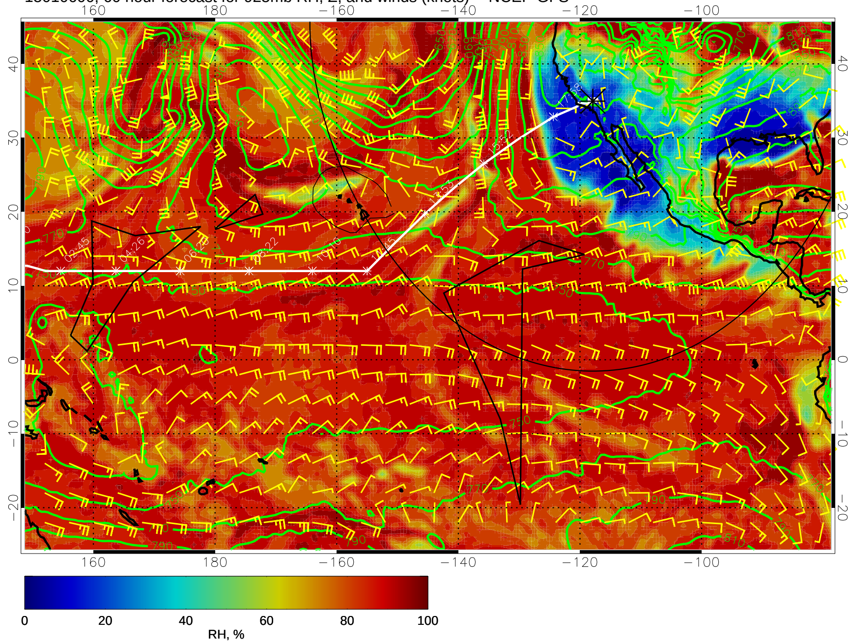
15010600, 60 hour forecast for 925mb RH, Z, and winds (knots) -- NCEP GFS
