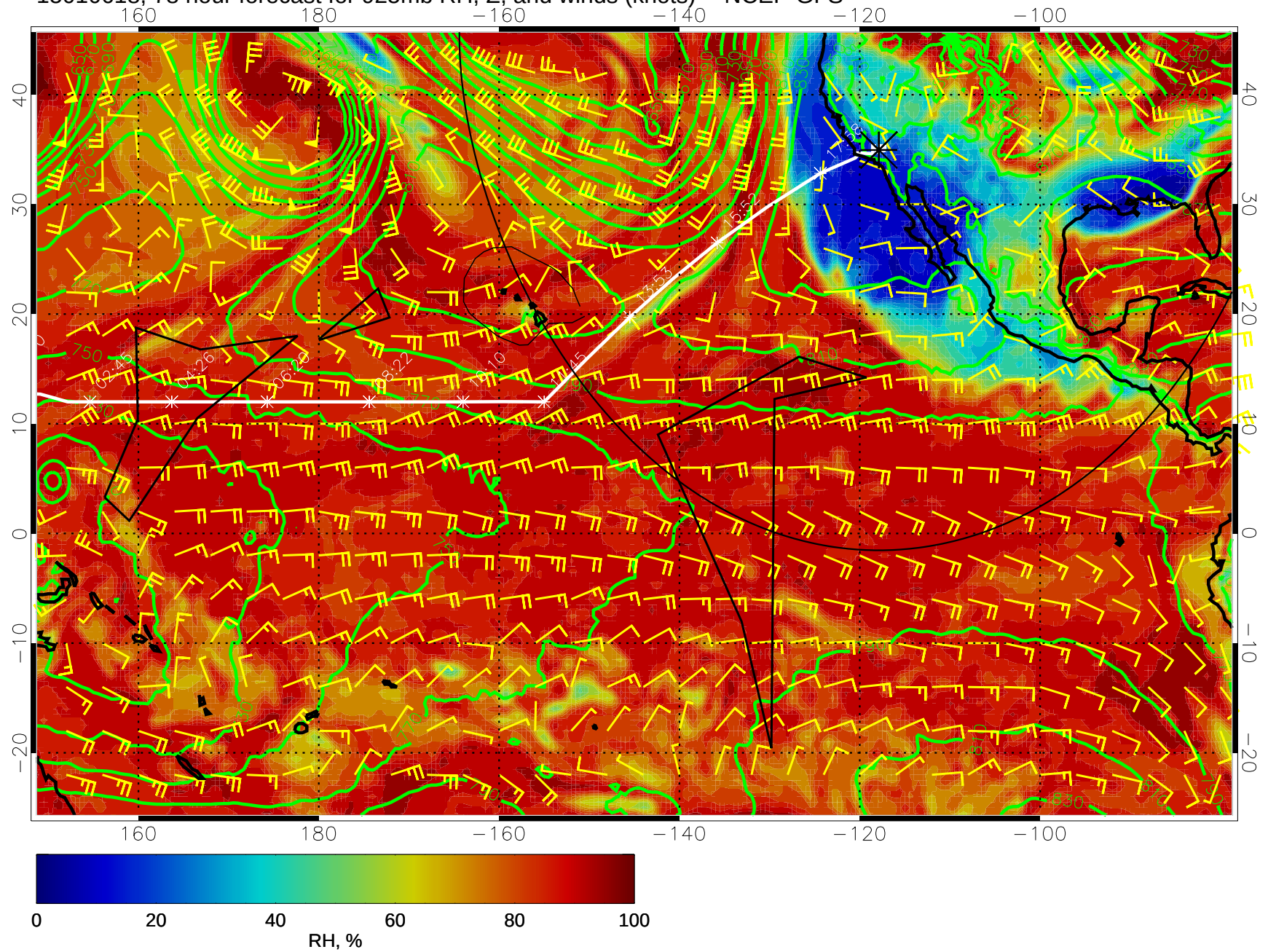
15010618, 78 hour forecast for 925mb RH, Z, and winds (knots) -- NCEP GFS
