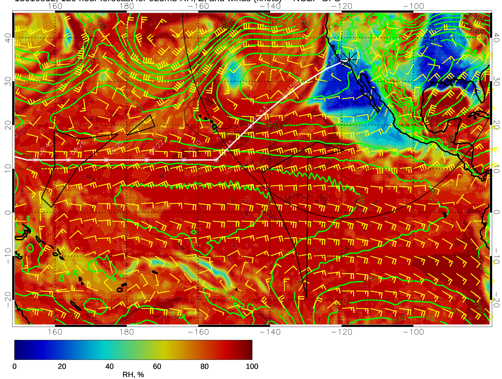
15010812, 120 hour forecast for 925mb RH, Z, and winds (knots) -- NCEP GFS
