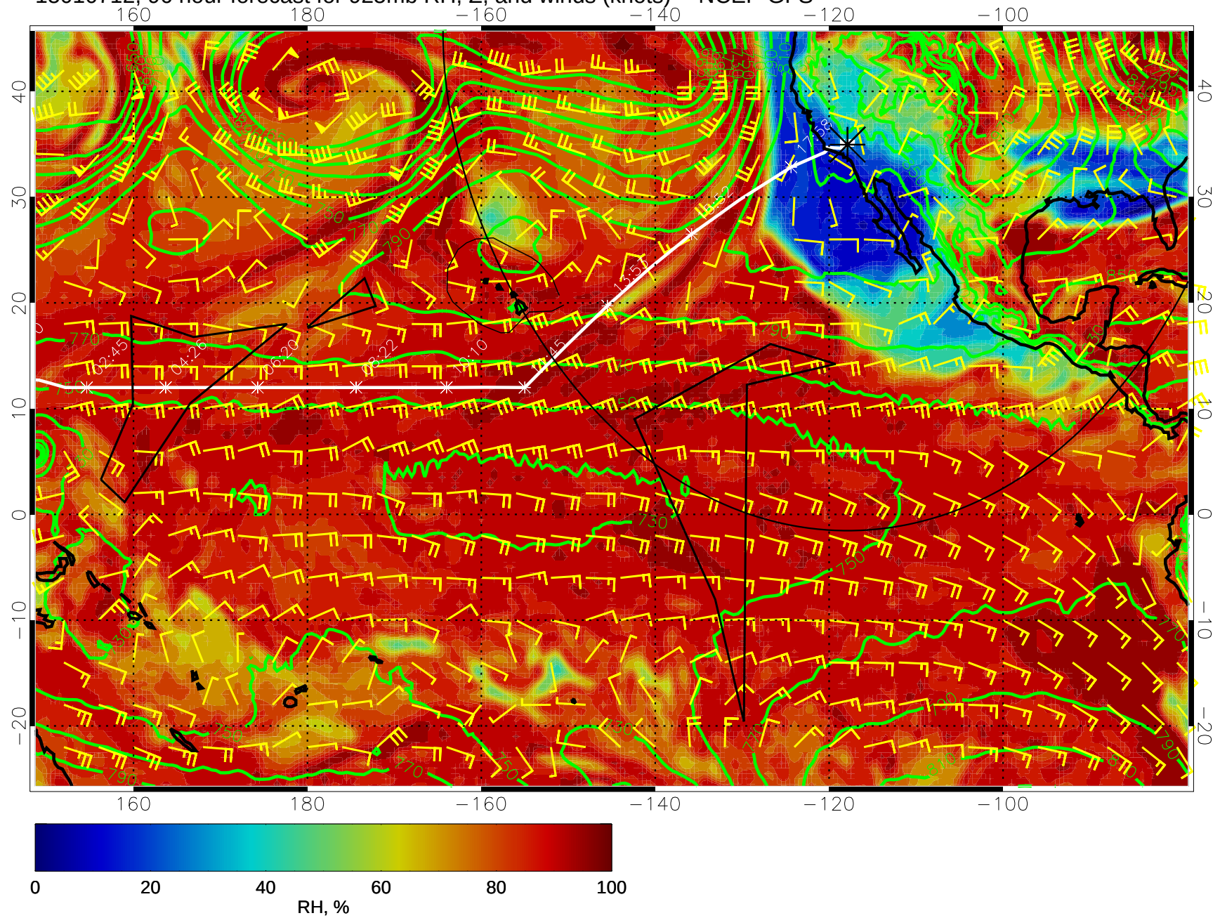
15010712, 96 hour forecast for 925mb RH, Z, and winds (knots) -- NCEP GFS
