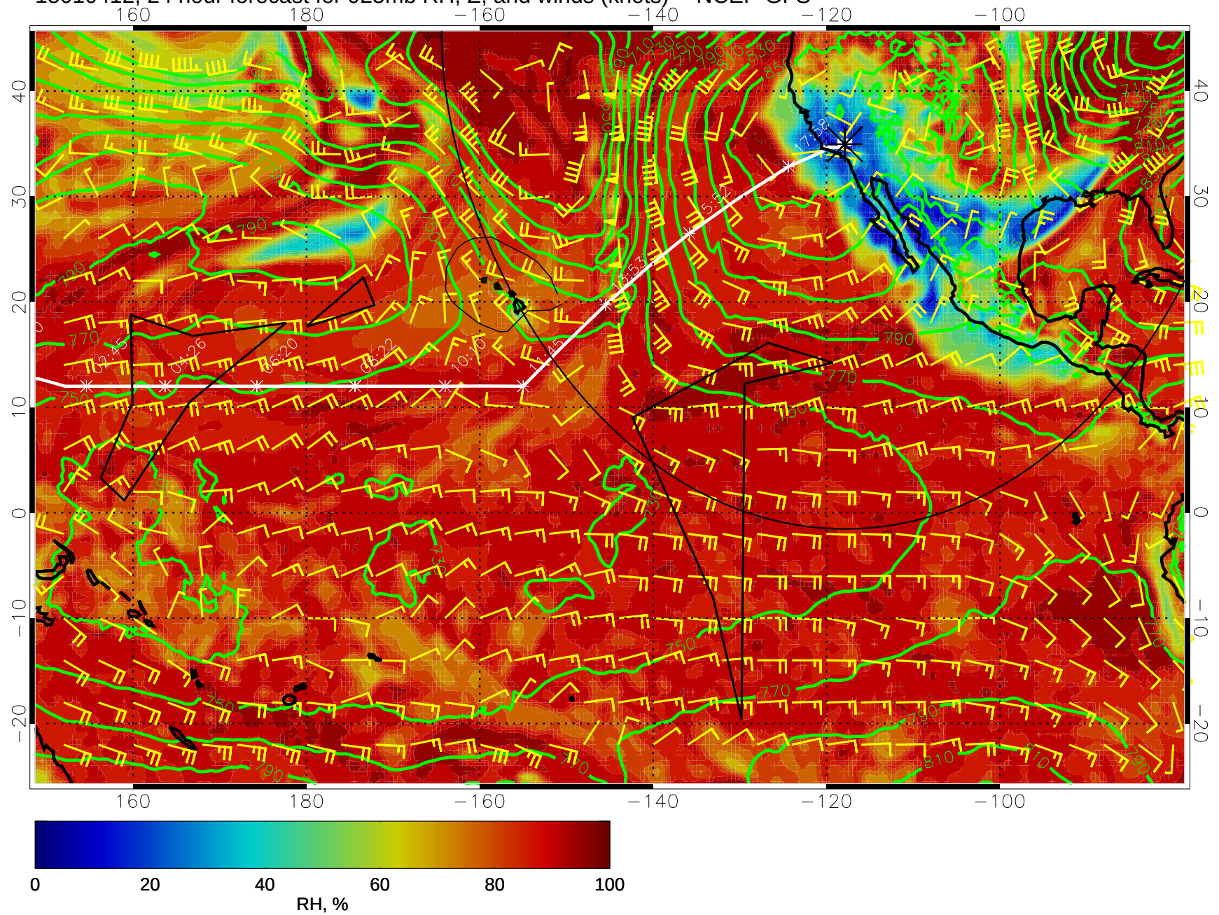
15010412, 24 hour forecast for 925mb RH, Z, and winds (knots) -- NCEP GFS
