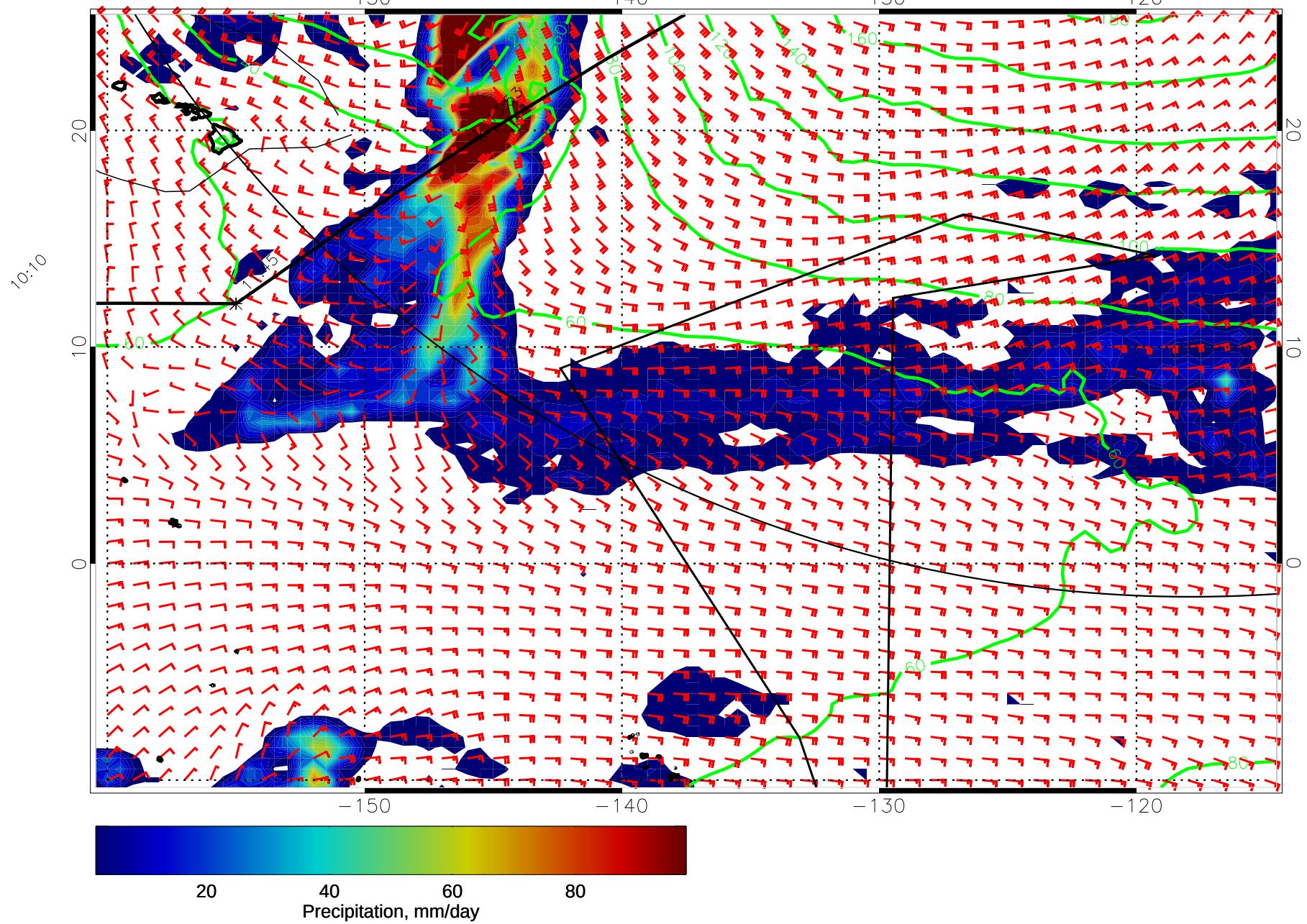
15010412, 24 hour forecast for precip, 1000mb Z, and winds (knots) -- NCEP GFS
