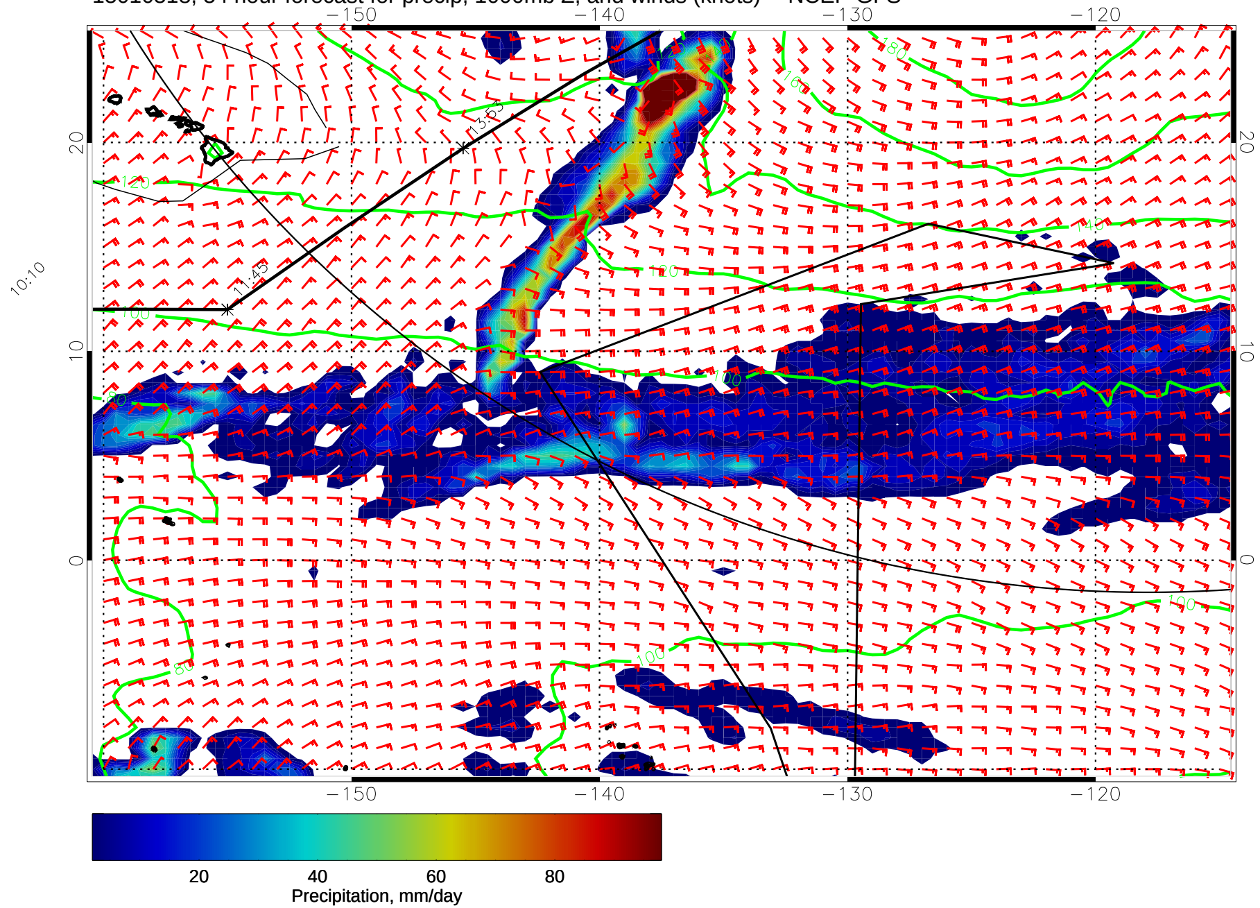
15010518, 54 hour forecast for precip, 1000mb Z, and winds (knots) -- NCEP GFS
