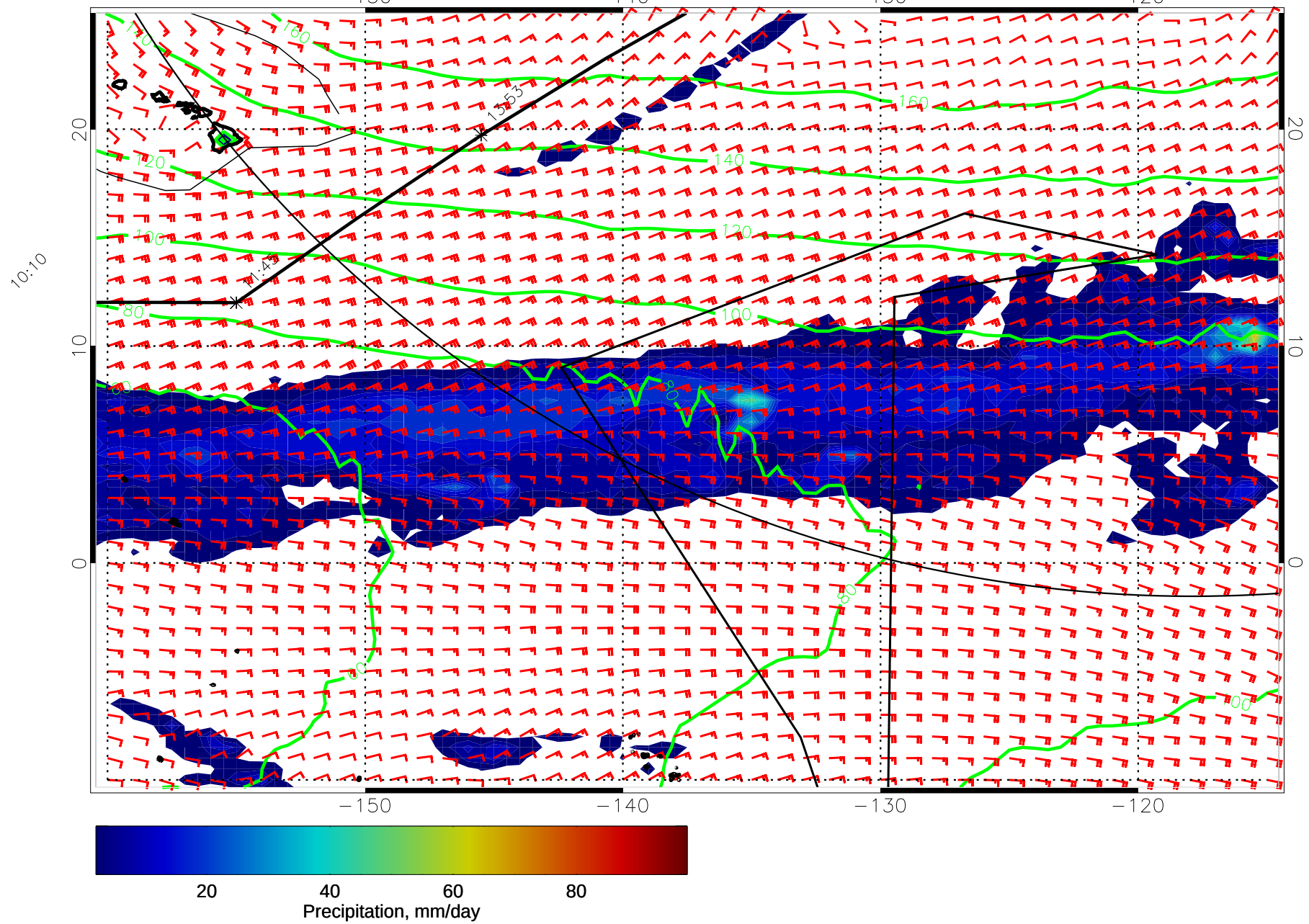
15010806, 114 hour forecast for precip, 1000mb Z, and winds (knots) -- NCEP GFS
