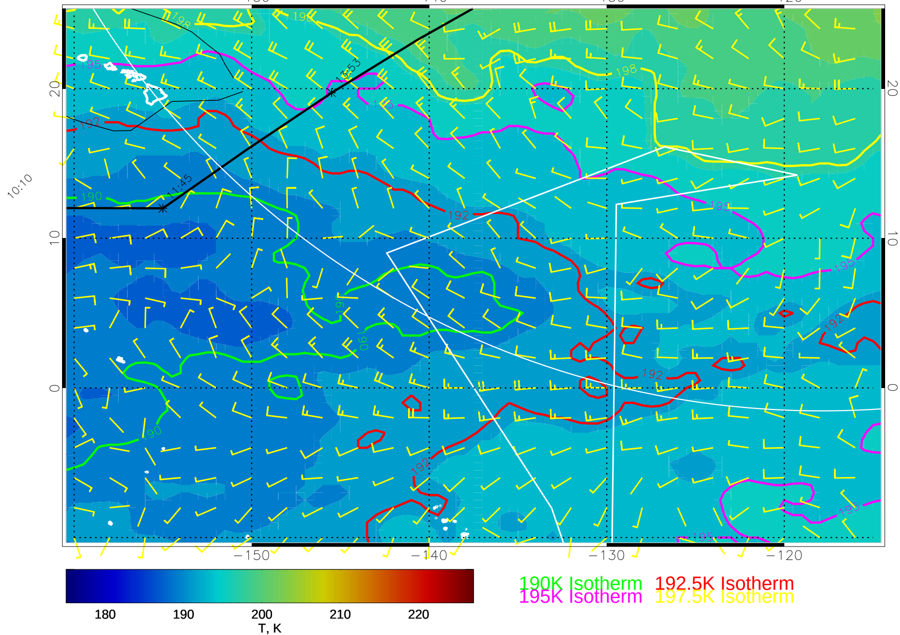
15010800, 108 hour forecast for 70mb T and winds (knots) -- NCEP GFS
