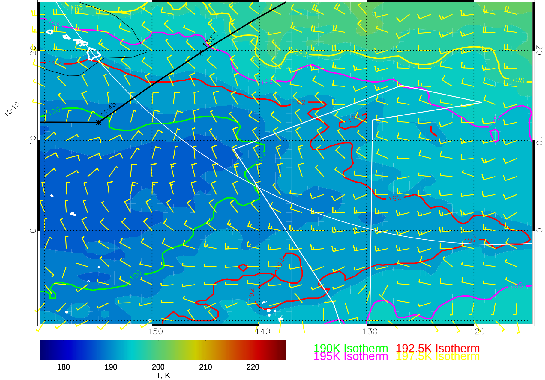
15010812, 120 hour forecast for 70mb T and winds (knots) -- NCEP GFS
