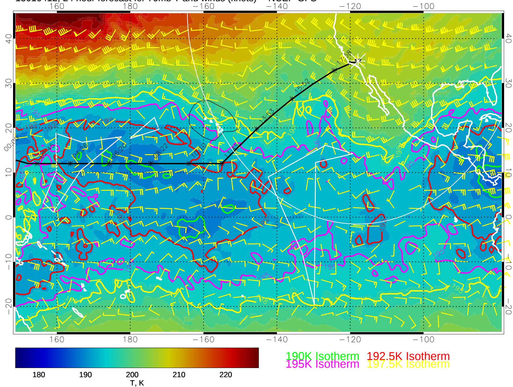
15010412, 24 hour forecast for 70mb T and winds (knots) -- NCEP GFS
