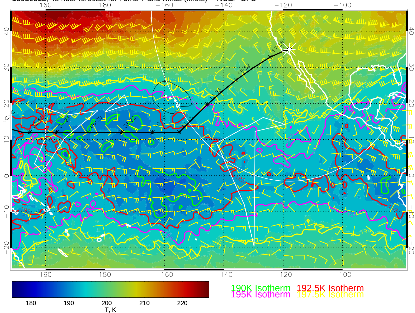
15010512, 48 hour forecast for 70mb T and winds (knots) -- NCEP GFS
