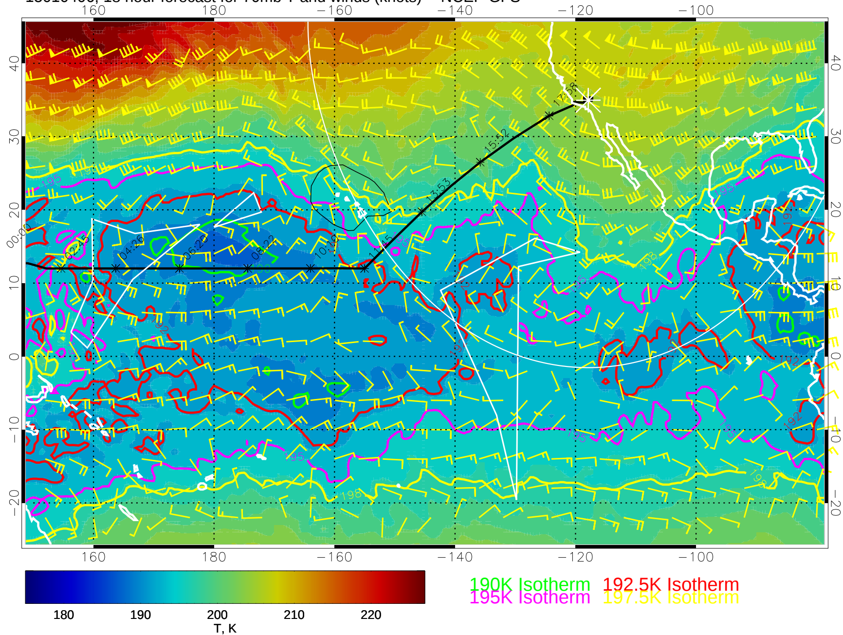
15010406, 18 hour forecast for 70mb T and winds (knots) -- NCEP GFS
