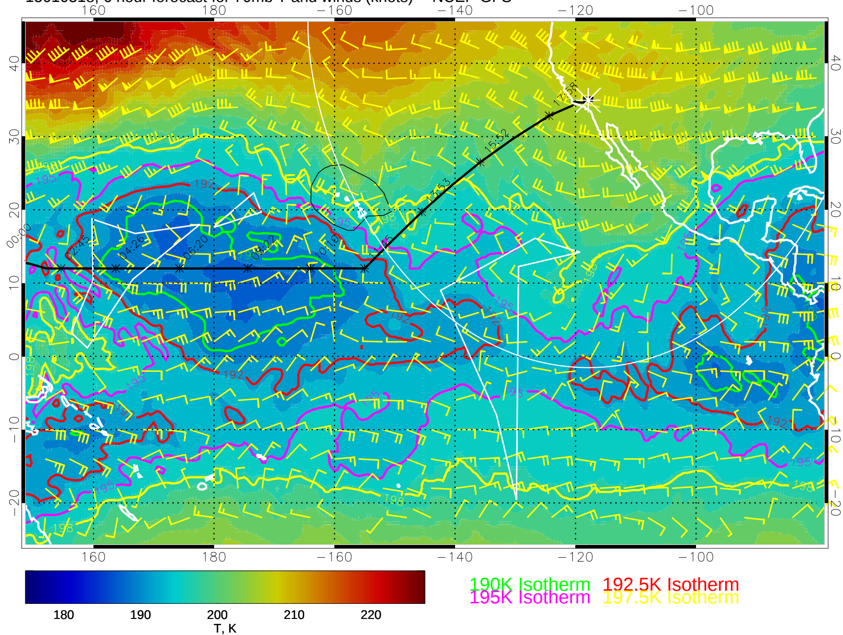
15010318, 6 hour forecast for 70mb T and winds (knots) -- NCEP GFS
