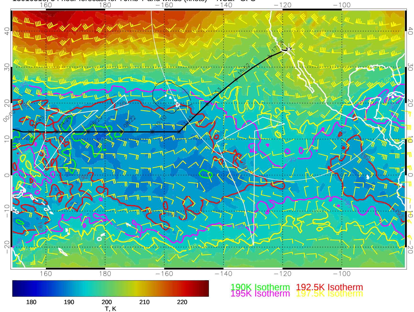
15010518, 54 hour forecast for 70mb T and winds (knots) -- NCEP GFS
