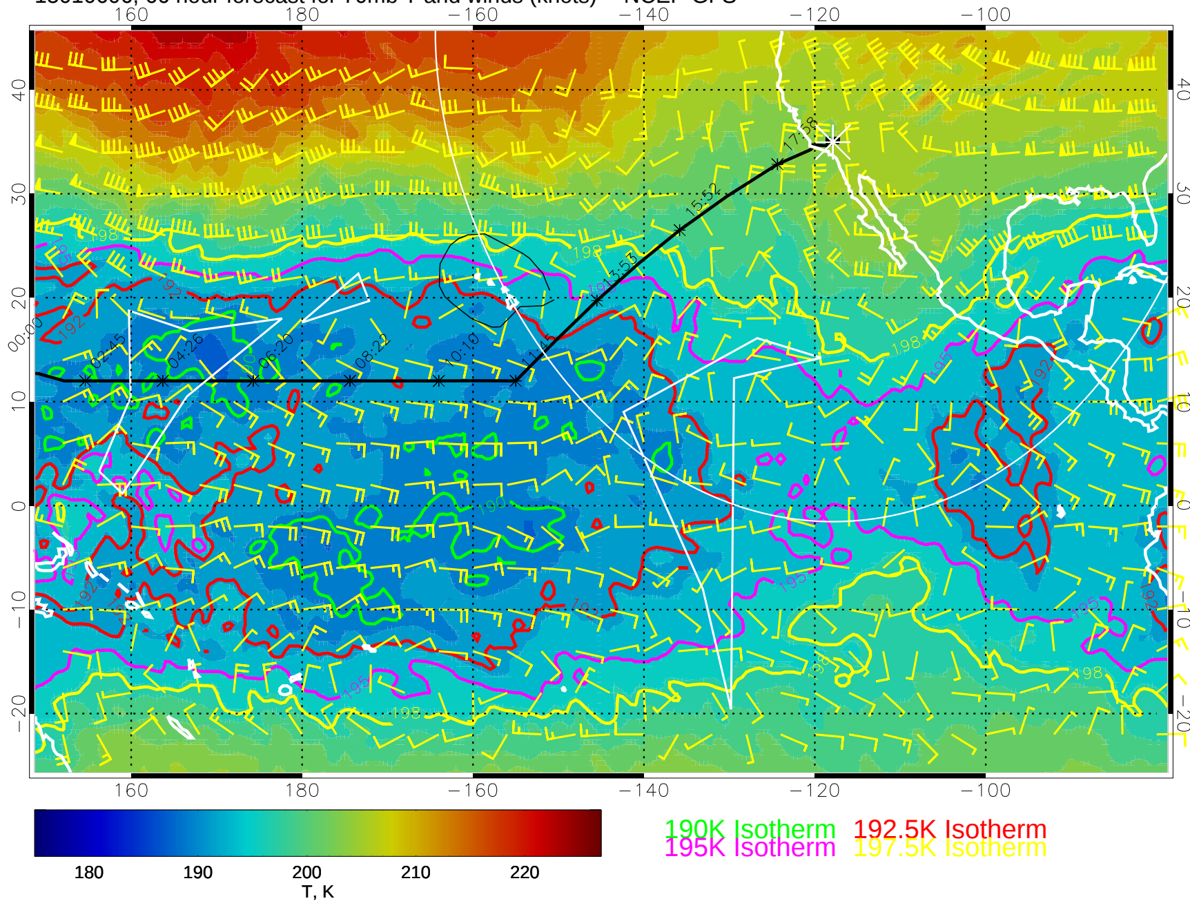
15010606, 66 hour forecast for 70mb T and winds (knots) -- NCEP GFS
