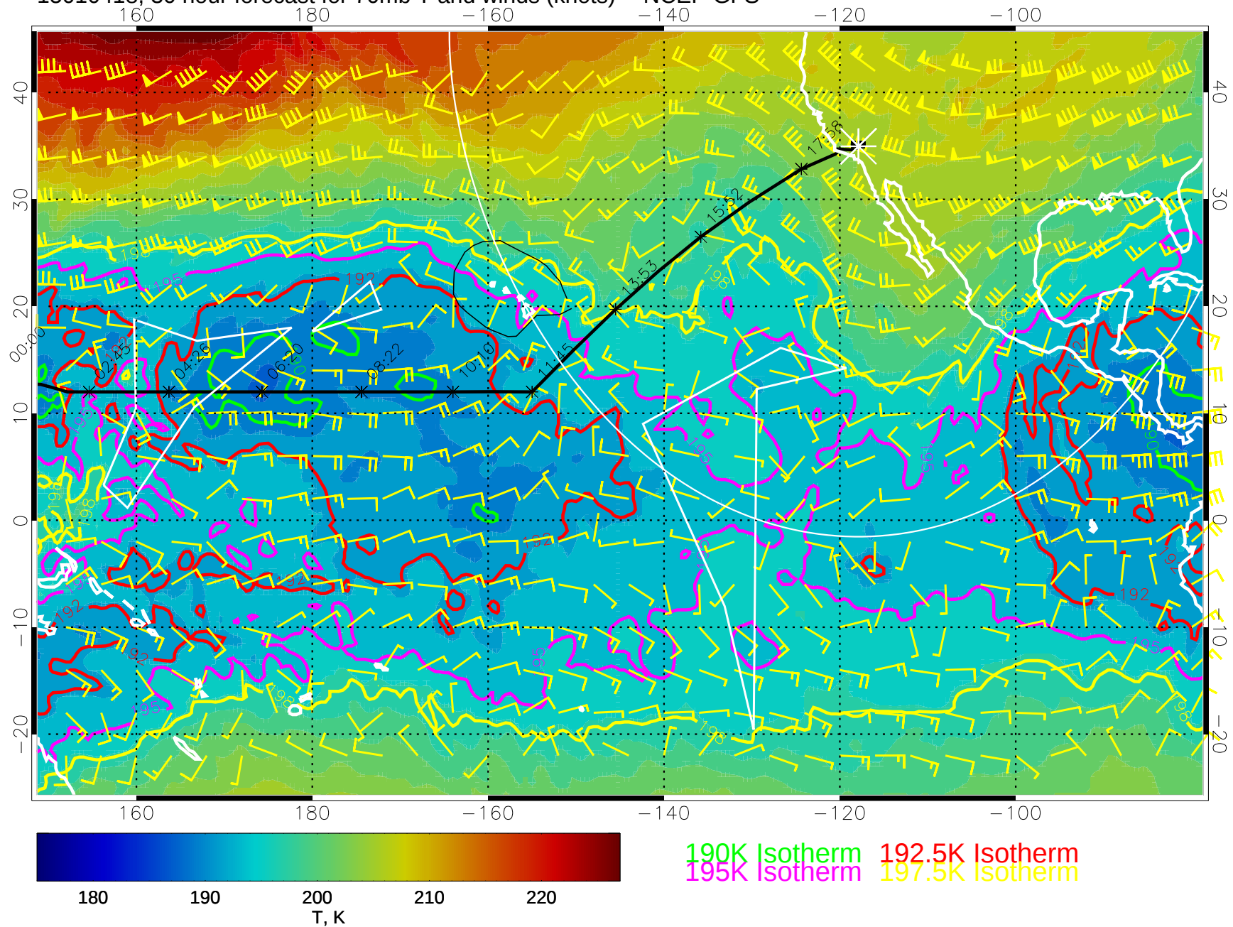
15010418, 30 hour forecast for 70mb T and winds (knots) -- NCEP GFS
