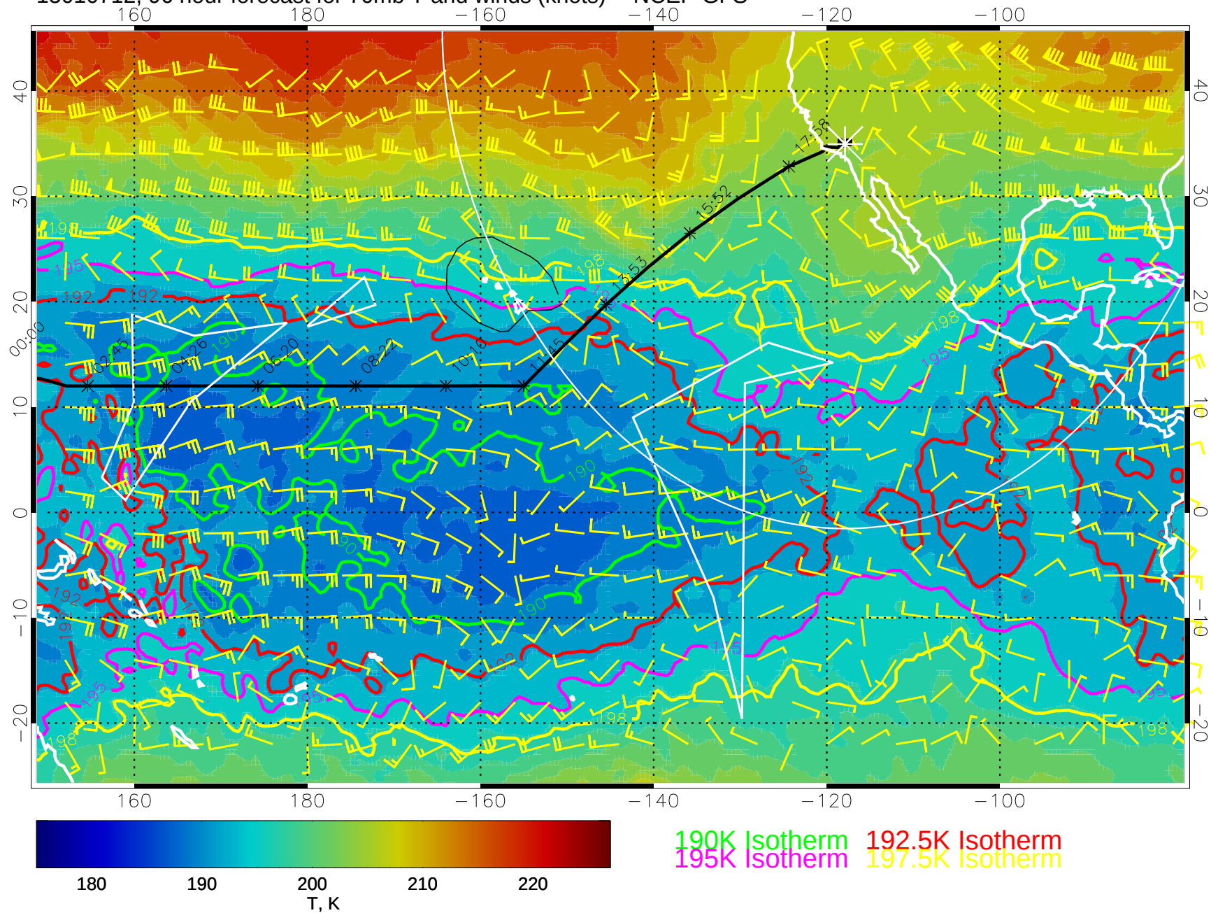
15010712, 96 hour forecast for 70mb T and winds (knots) -- NCEP GFS
