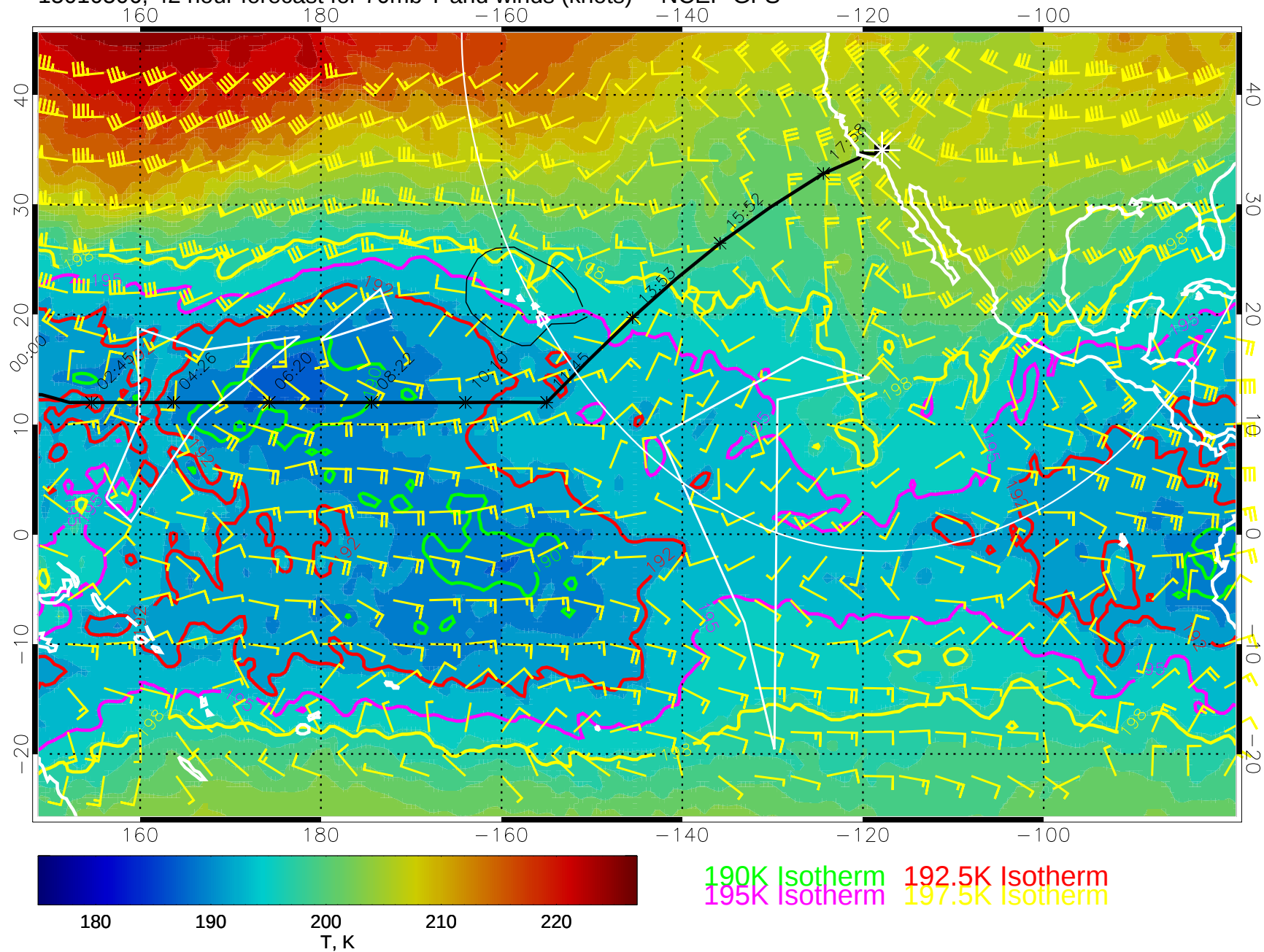
15010506, 42 hour forecast for 70mb T and winds (knots) -- NCEP GFS
