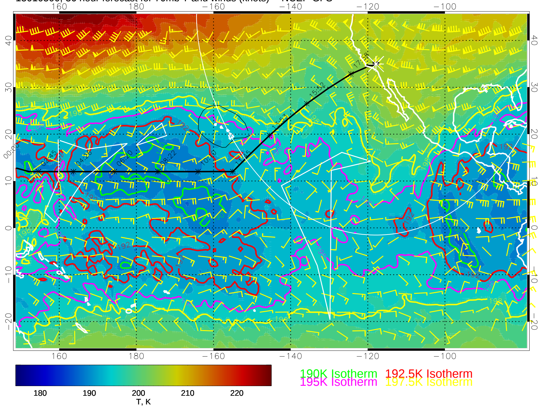
15010500, 36 hour forecast for 70mb T and winds (knots) -- NCEP GFS
