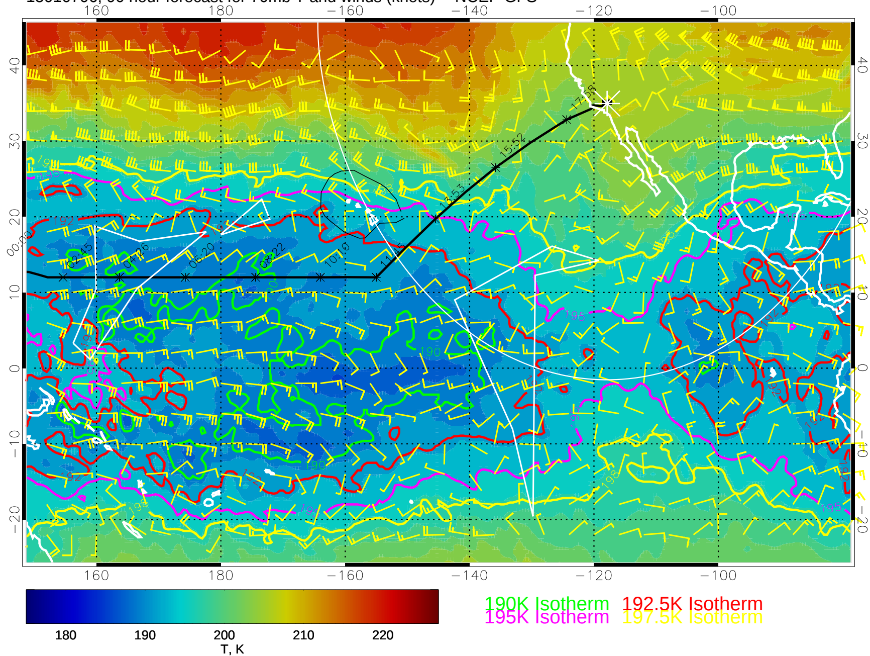
15010706, 90 hour forecast for 70mb T and winds (knots) -- NCEP GFS
