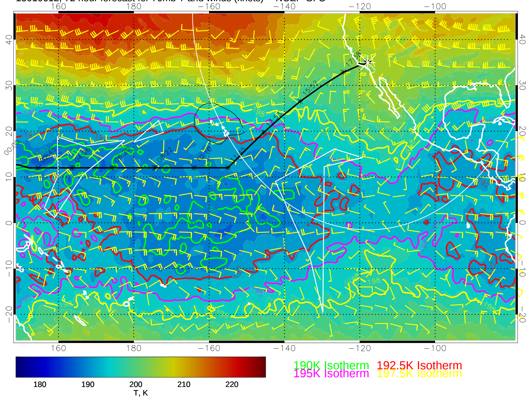
15010612, 72 hour forecast for 70mb T and winds (knots) -- NCEP GFS
