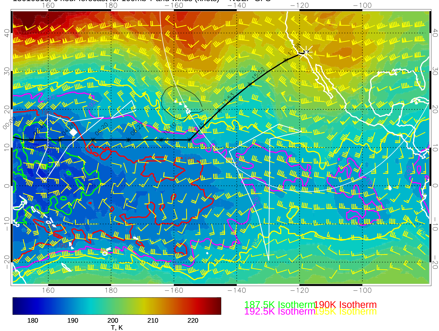
15010318, 6 hour forecast for 100mb T and winds (knots) -- NCEP GFS
