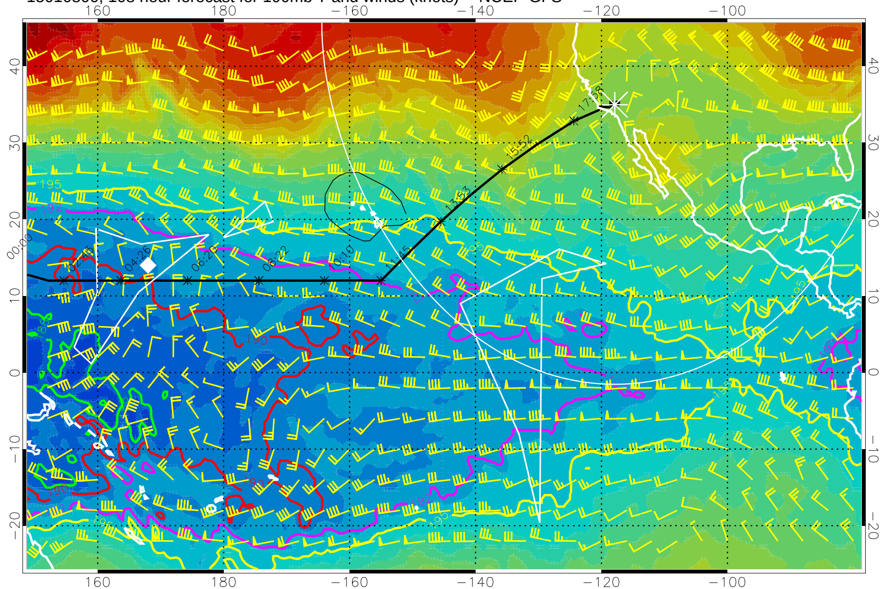
15010800, 108 hour forecast for 100mb T and winds (knots) -- NCEP GFS
