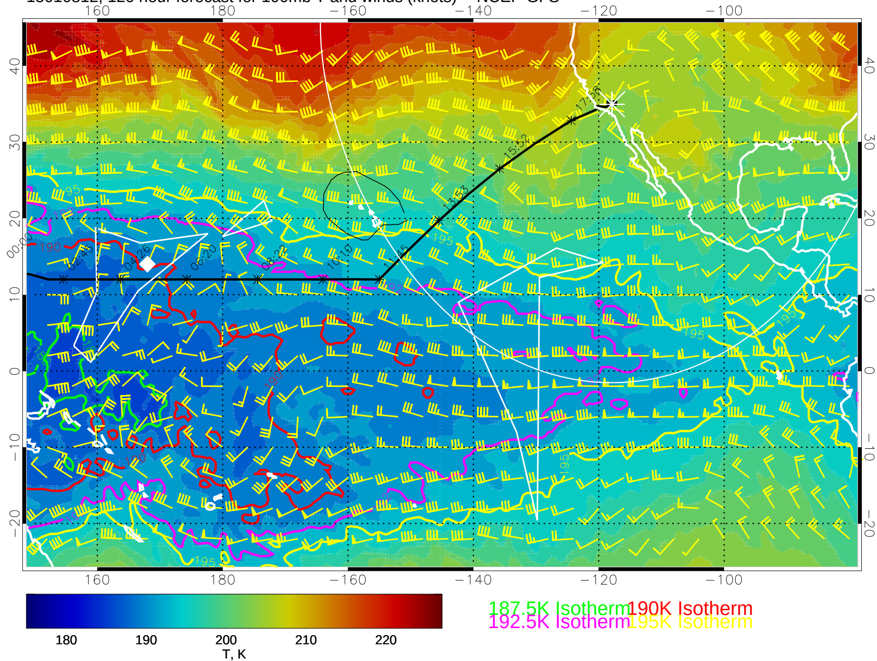
15010812, 120 hour forecast for 100mb T and winds (knots) -- NCEP GFS
