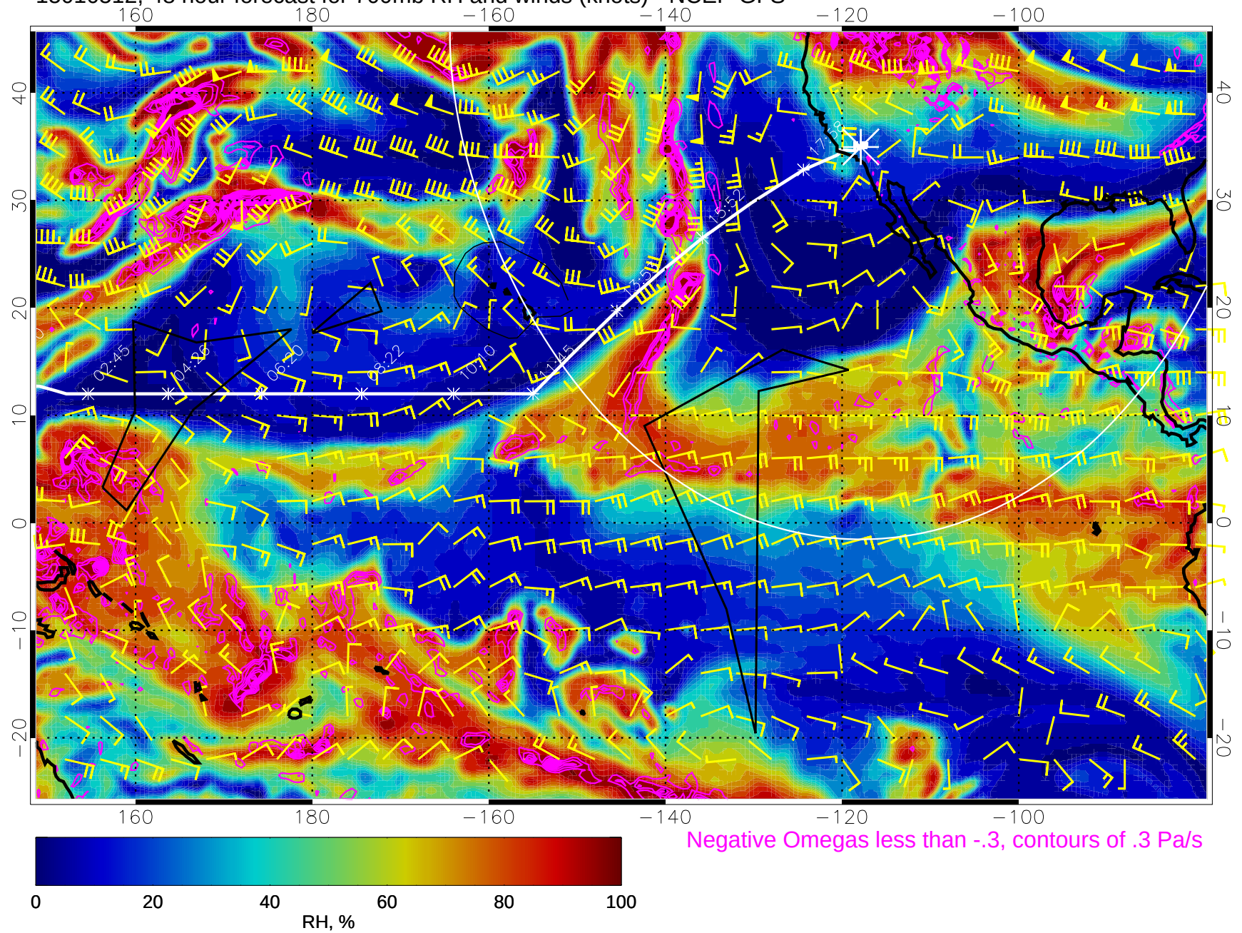
15010512, 48 hour forecast for 700mb RH and winds (knots) - NCEP GFS
