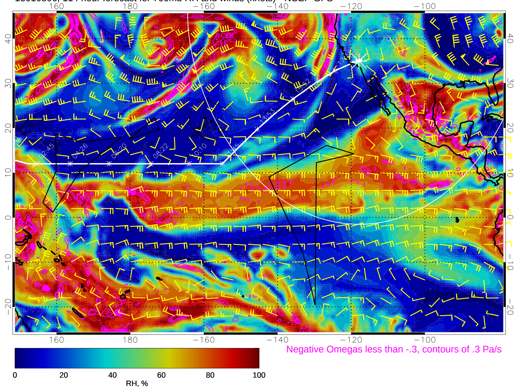
15010806, 114 hour forecast for 700mb RH and winds (knots) - NCEP GFS
