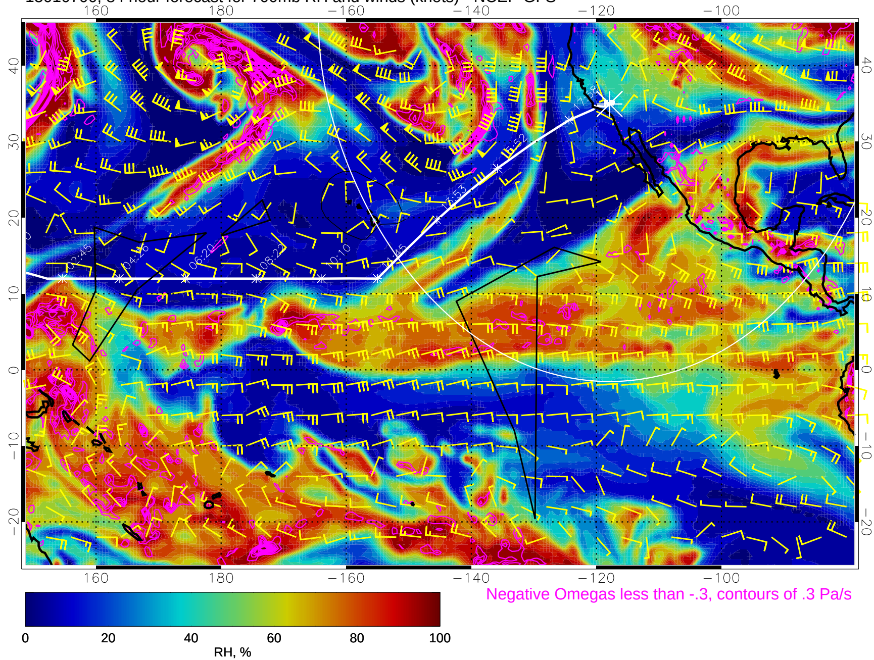
15010700, 84 hour forecast for 700mb RH and winds (knots) - NCEP GFS
