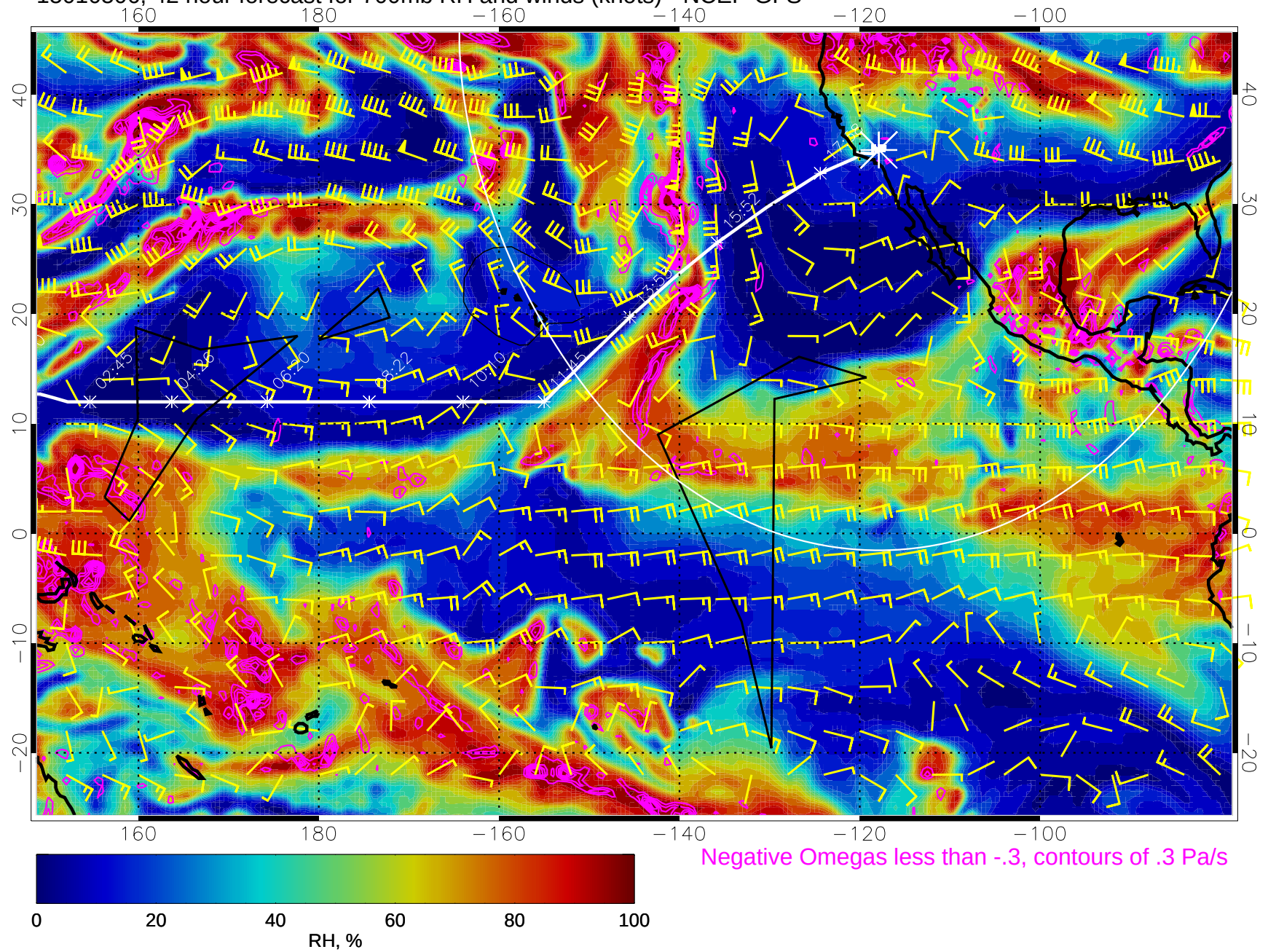
15010506, 42 hour forecast for 700mb RH and winds (knots) - NCEP GFS
