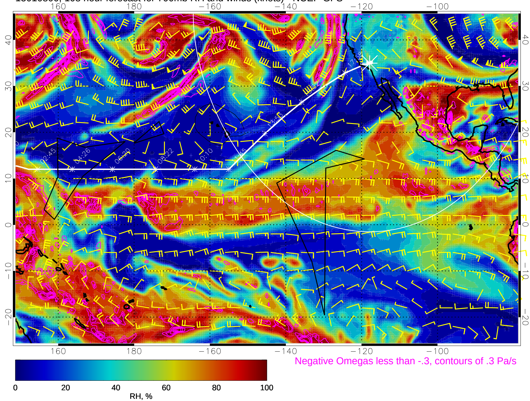
15010800, 108 hour forecast for 700mb RH and winds (knots) - NCEP GFS
