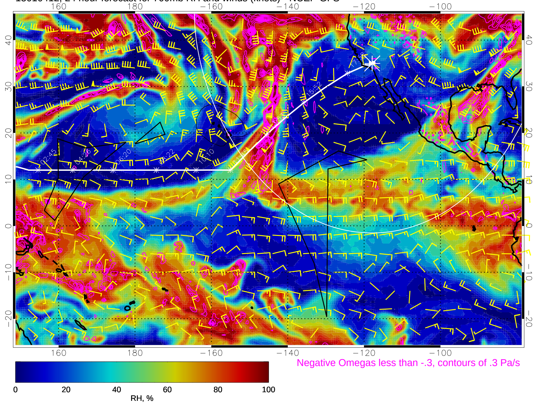
15010412, 24 hour forecast for 700mb RH and winds (knots) - NCEP GFS
