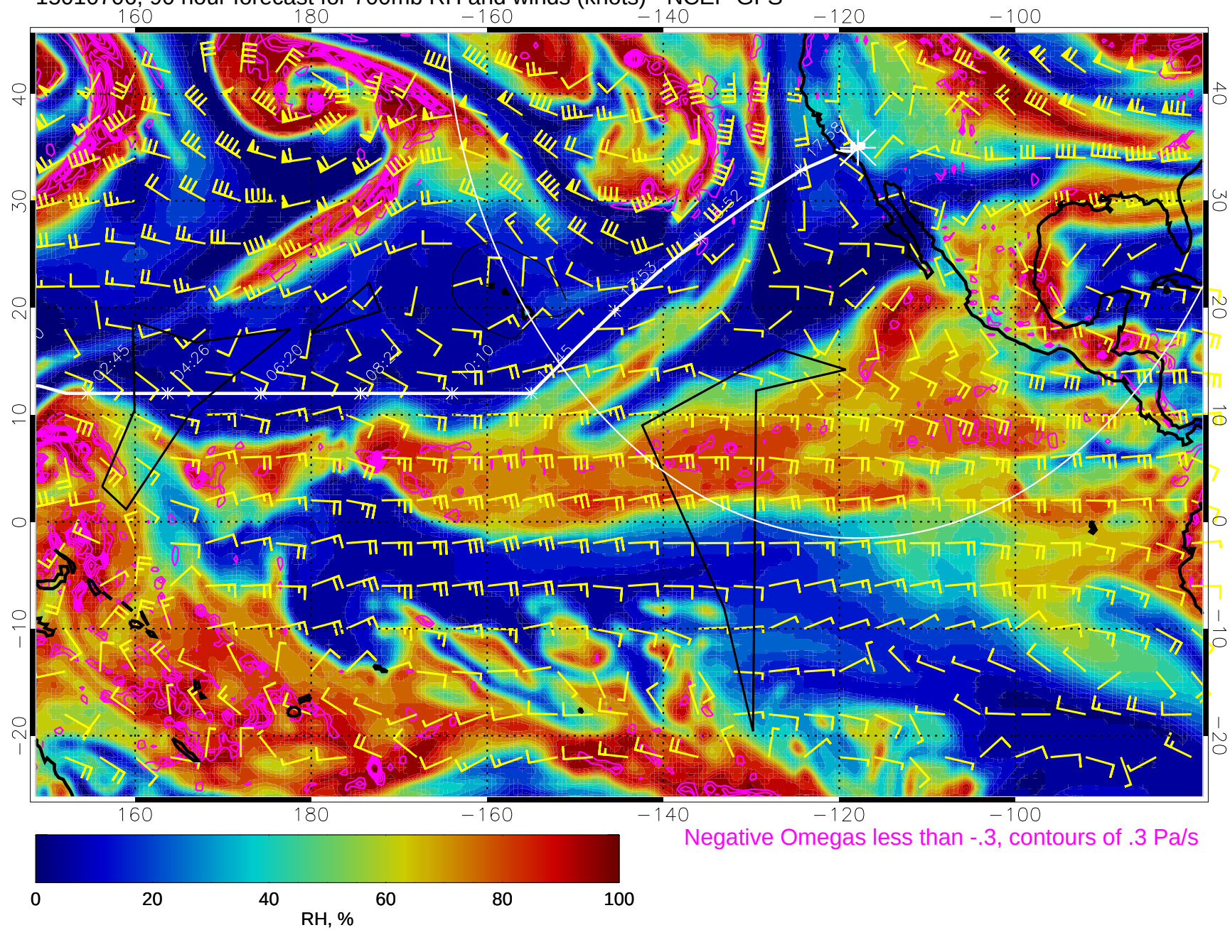
15010706, 90 hour forecast for 700mb RH and winds (knots) - NCEP GFS
