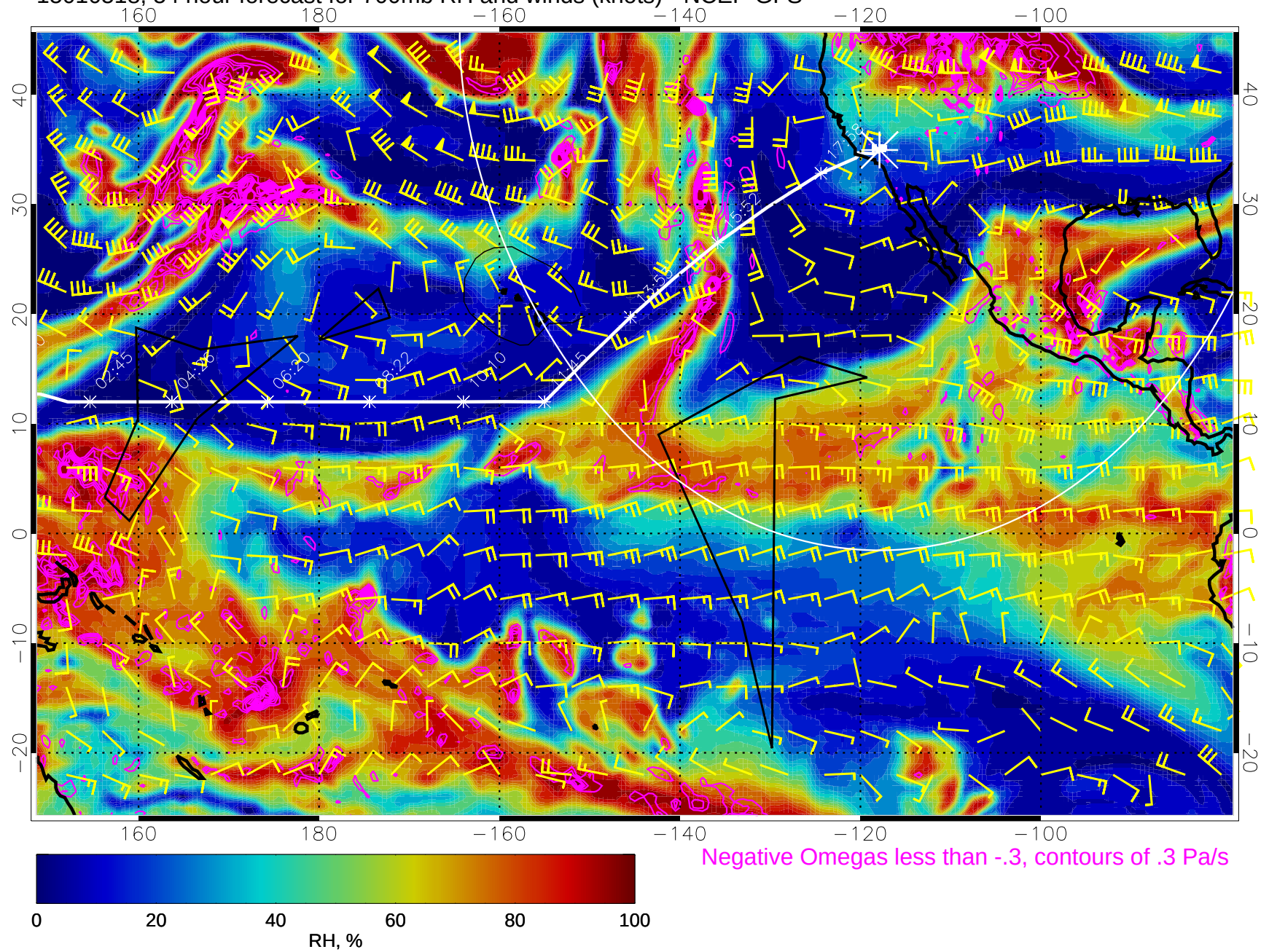
15010518, 54 hour forecast for 700mb RH and winds (knots) - NCEP GFS
