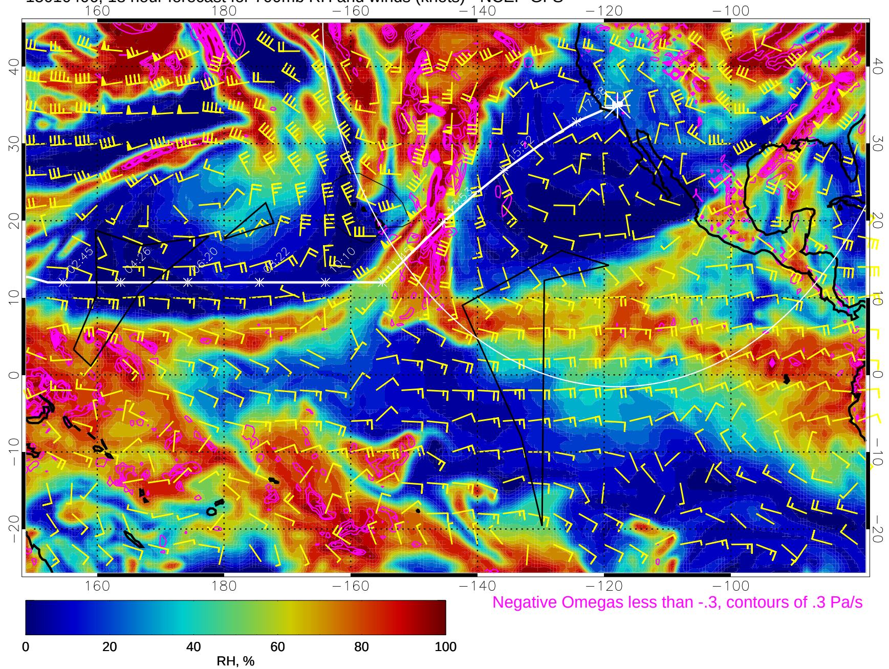
15010406, 18 hour forecast for 700mb RH and winds (knots) - NCEP GFS
