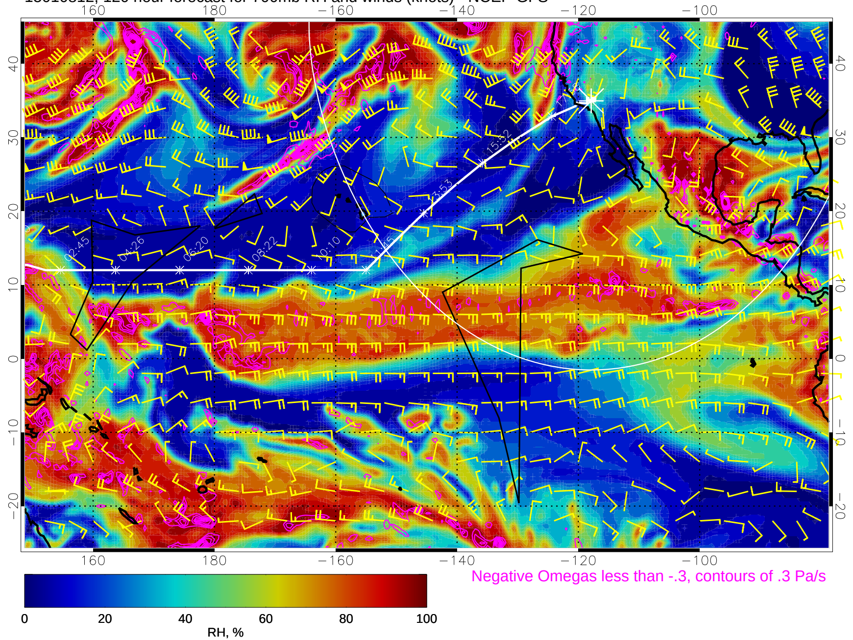
15010812, 120 hour forecast for 700mb RH and winds (knots) - NCEP GFS
