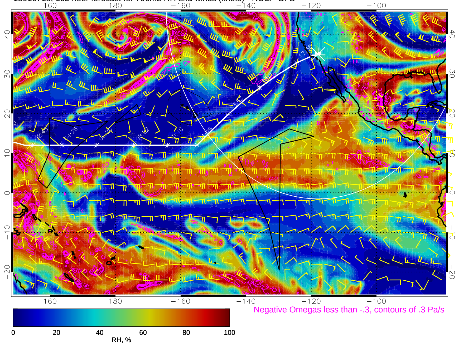
15010718, 102 hour forecast for 700mb RH and winds (knots) - NCEP GFS
