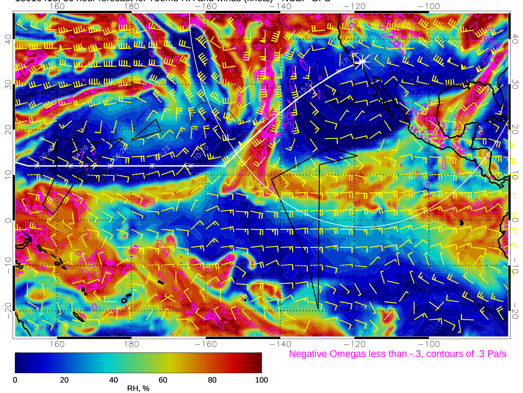
15010418, 30 hour forecast for 700mb RH and winds (knots) - NCEP GFS
