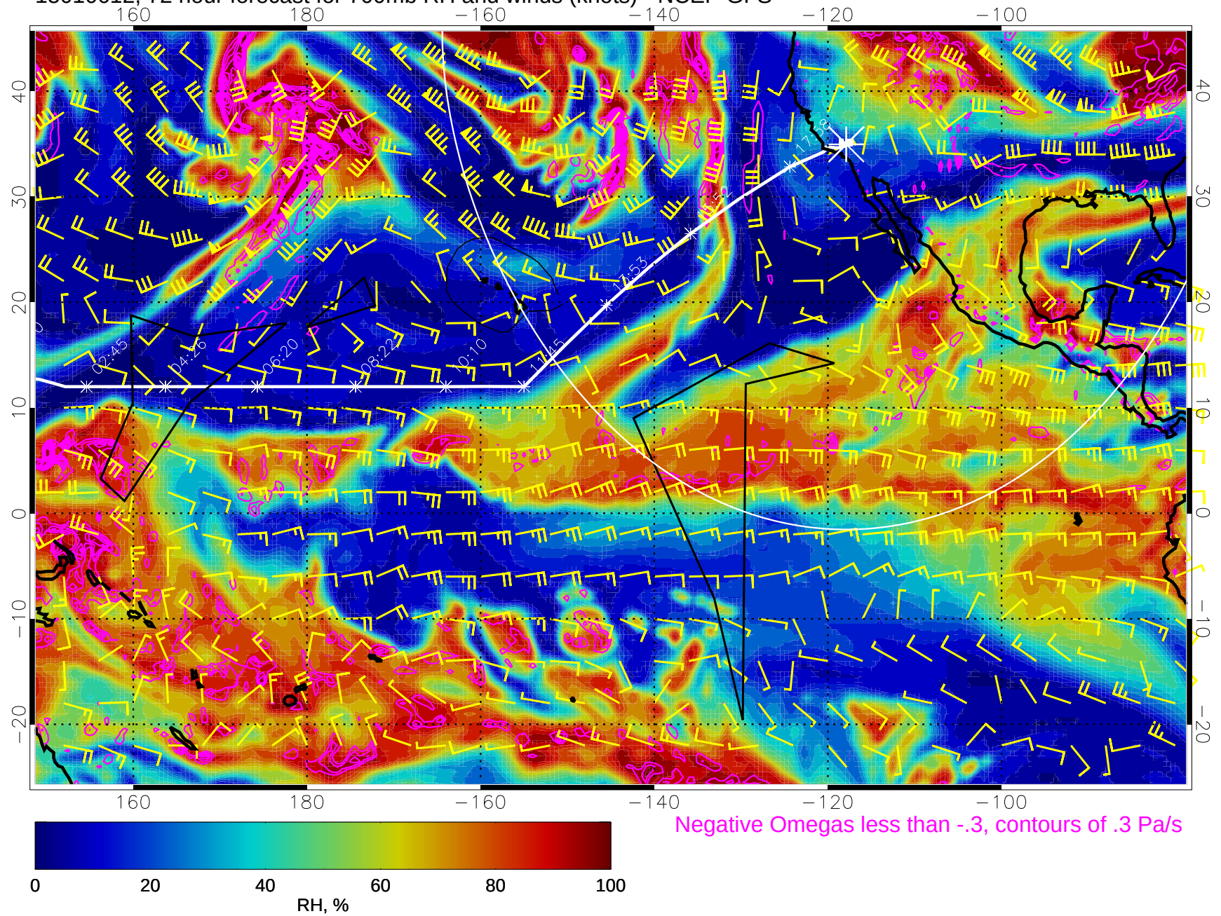
15010612, 72 hour forecast for 700mb RH and winds (knots) - NCEP GFS
