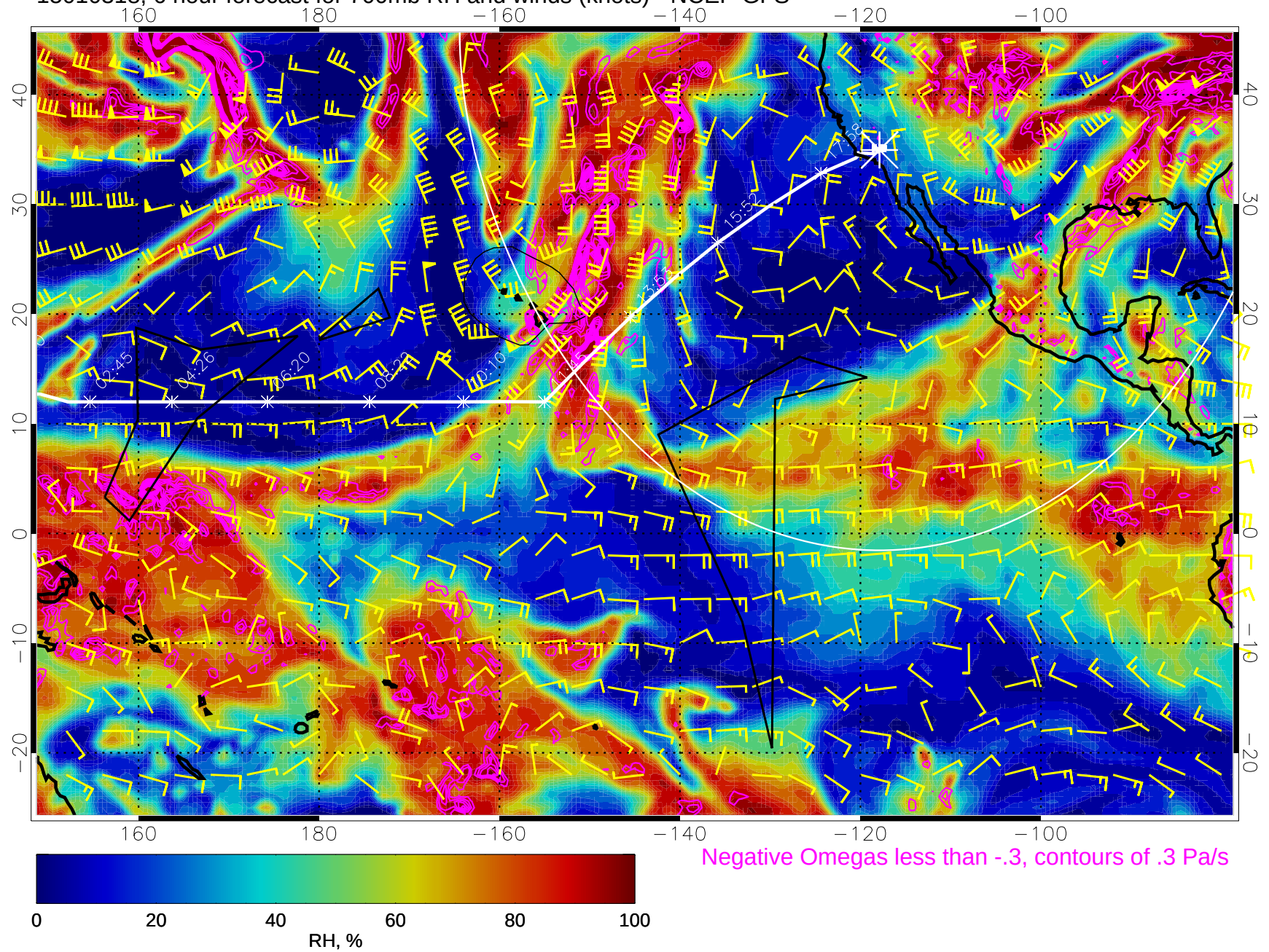
15010318, 6 hour forecast for 700mb RH and winds (knots) - NCEP GFS
