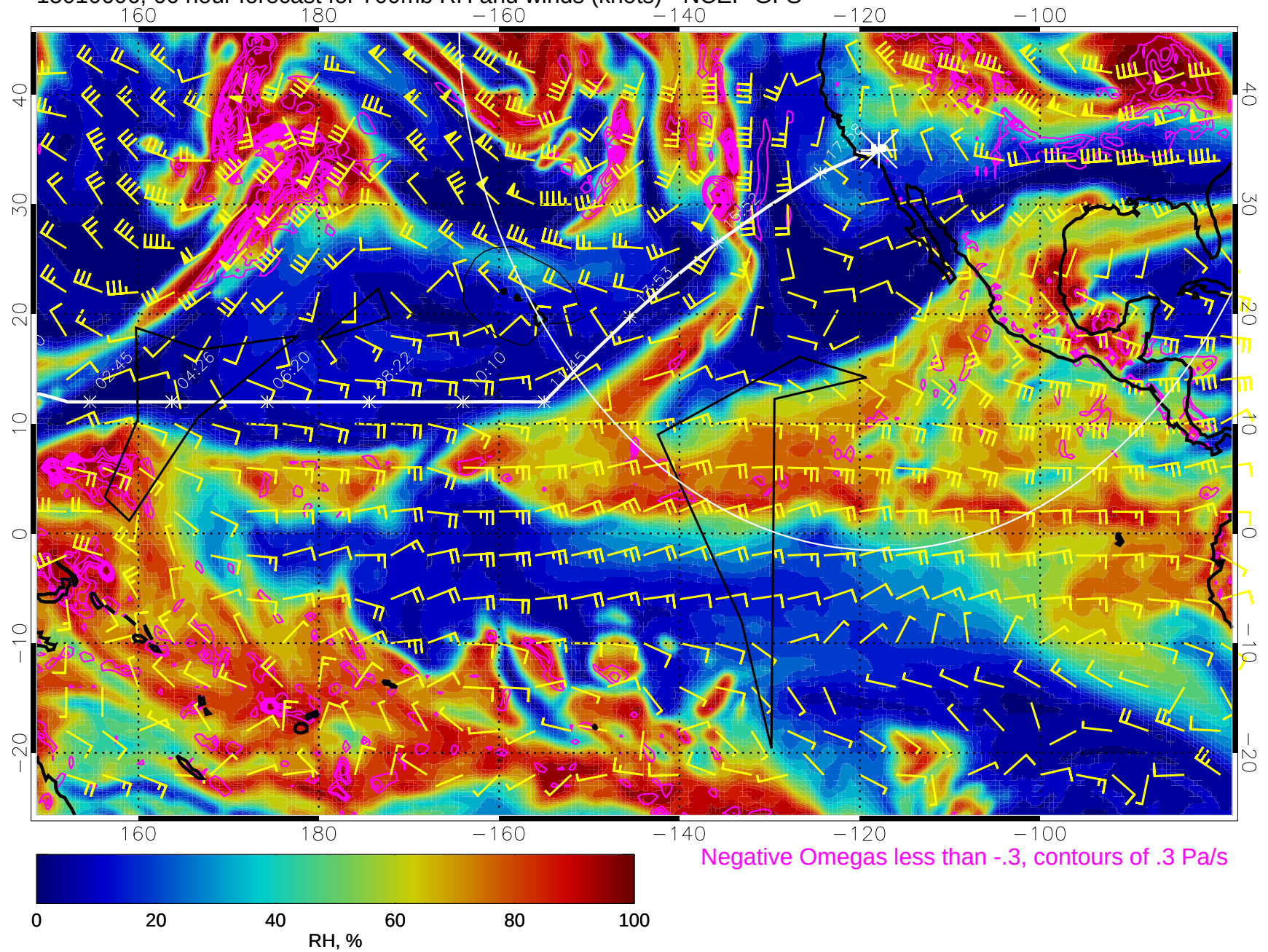
15010606, 66 hour forecast for 700mb RH and winds (knots) - NCEP GFS
