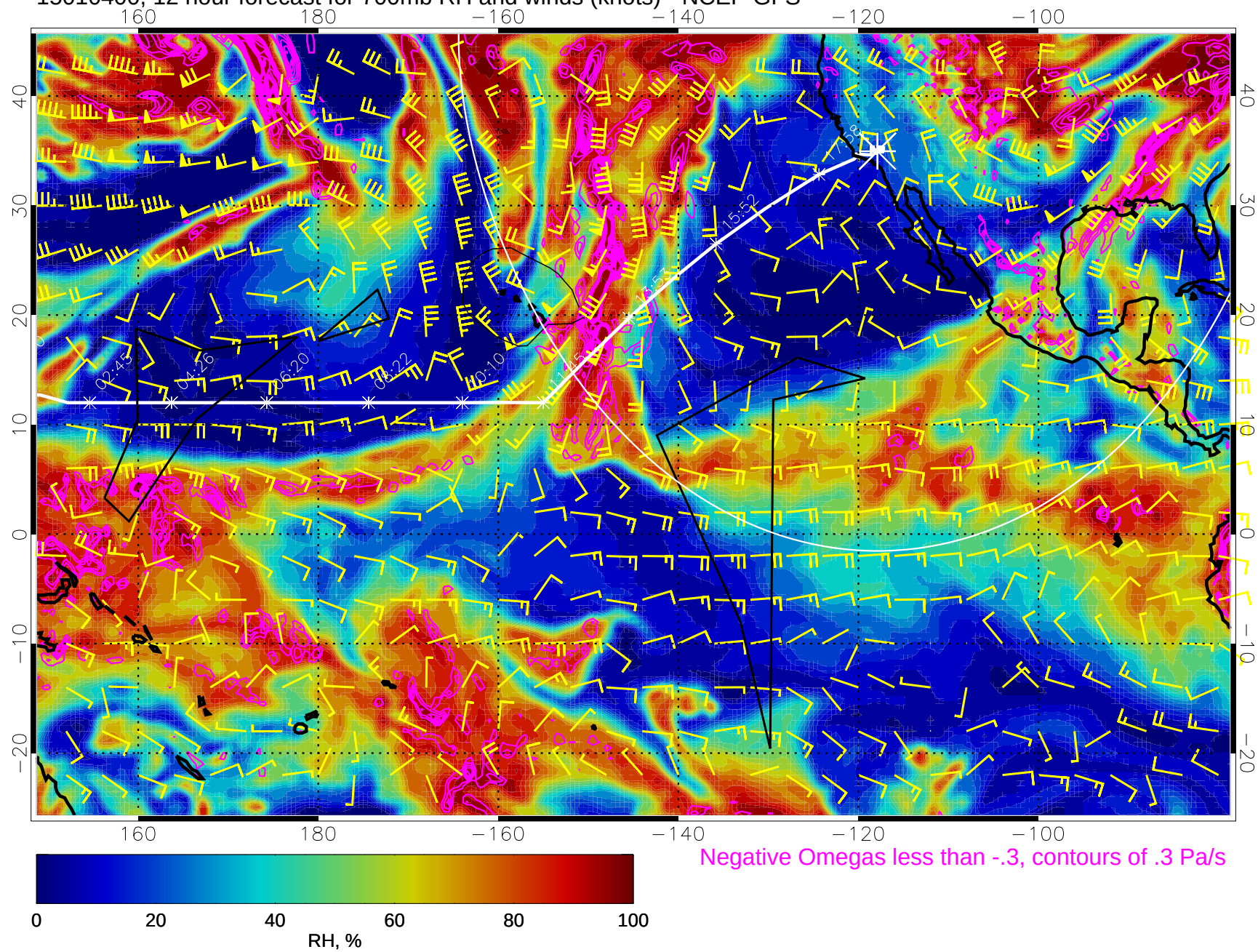
15010400, 12 hour forecast for 700mb RH and winds (knots) - NCEP GFS
