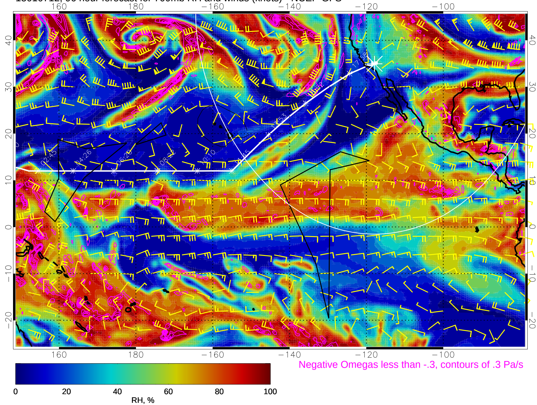
15010712, 96 hour forecast for 700mb RH and winds (knots) - NCEP GFS
