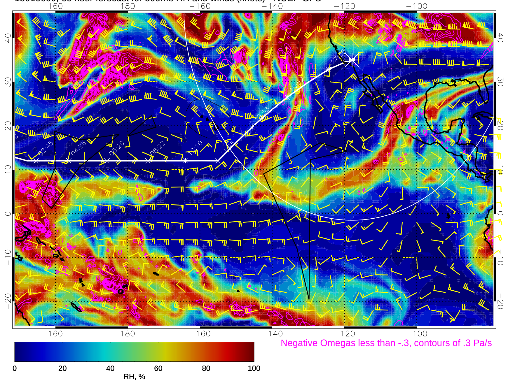
15010600, 60 hour forecast for 500mb RH and winds (knots) - NCEP GFS
