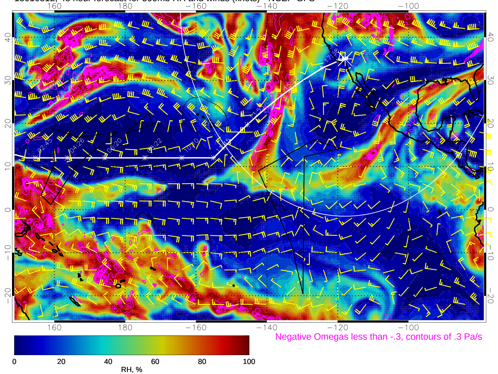
15010512, 48 hour forecast for 500mb RH and winds (knots) - NCEP GFS
