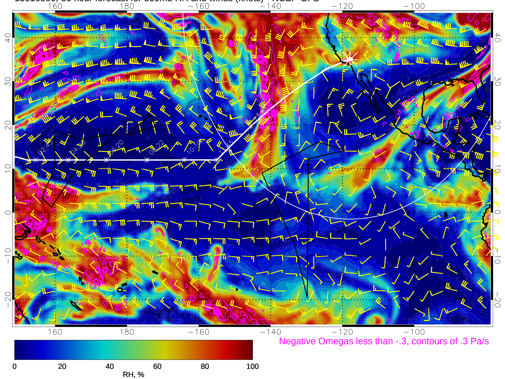
15010500, 36 hour forecast for 500mb RH and winds (knots) - NCEP GFS
