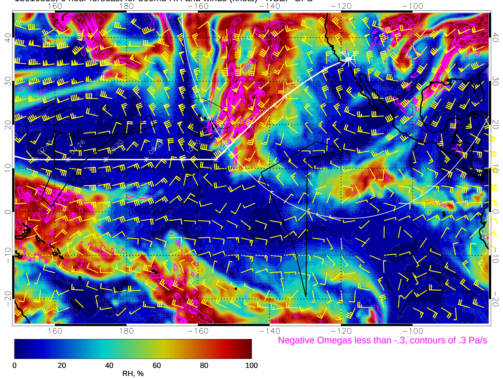
15010318, 6 hour forecast for 500mb RH and winds (knots) - NCEP GFS
