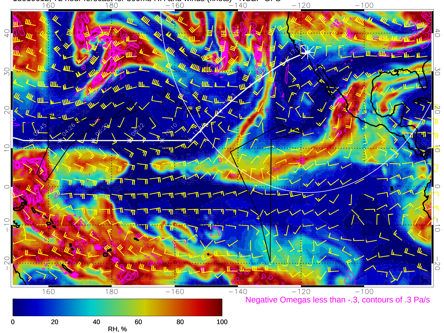
15010612, 72 hour forecast for 500mb RH and winds (knots) - NCEP GFS
