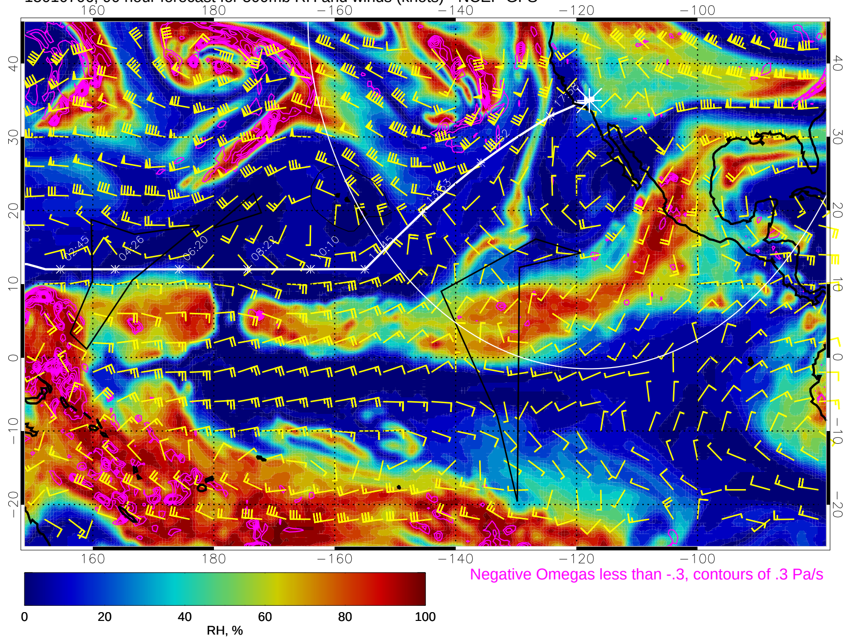
15010706, 90 hour forecast for 500mb RH and winds (knots) - NCEP GFS
