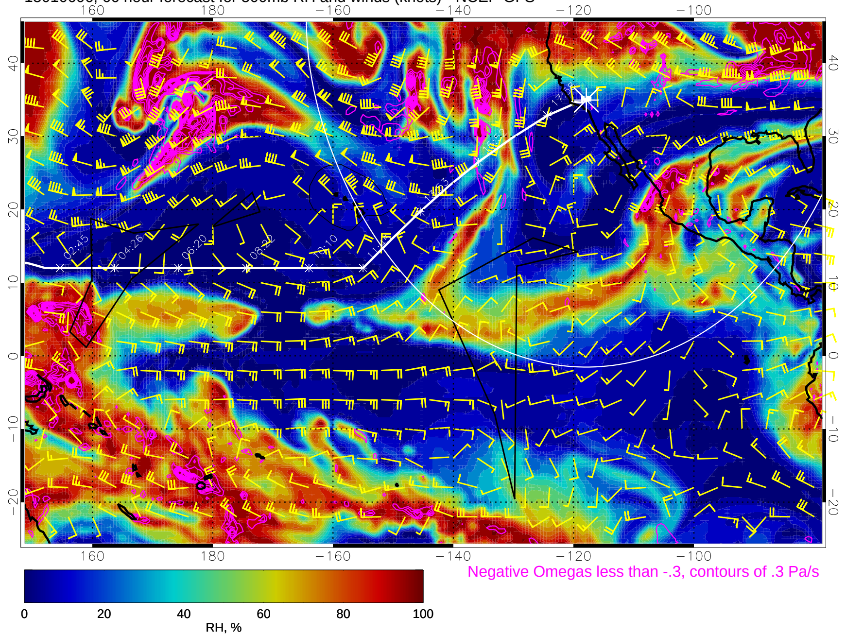
15010606, 66 hour forecast for 500mb RH and winds (knots) - NCEP GFS
