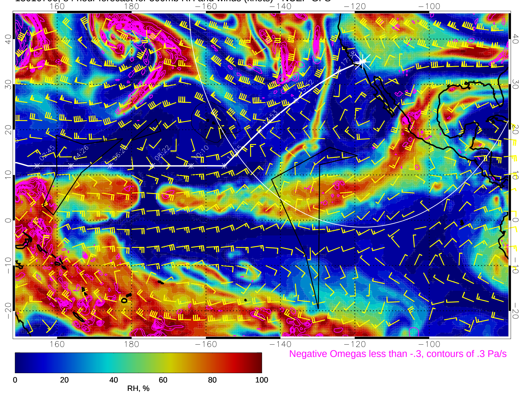
15010700, 84 hour forecast for 500mb RH and winds (knots) - NCEP GFS
