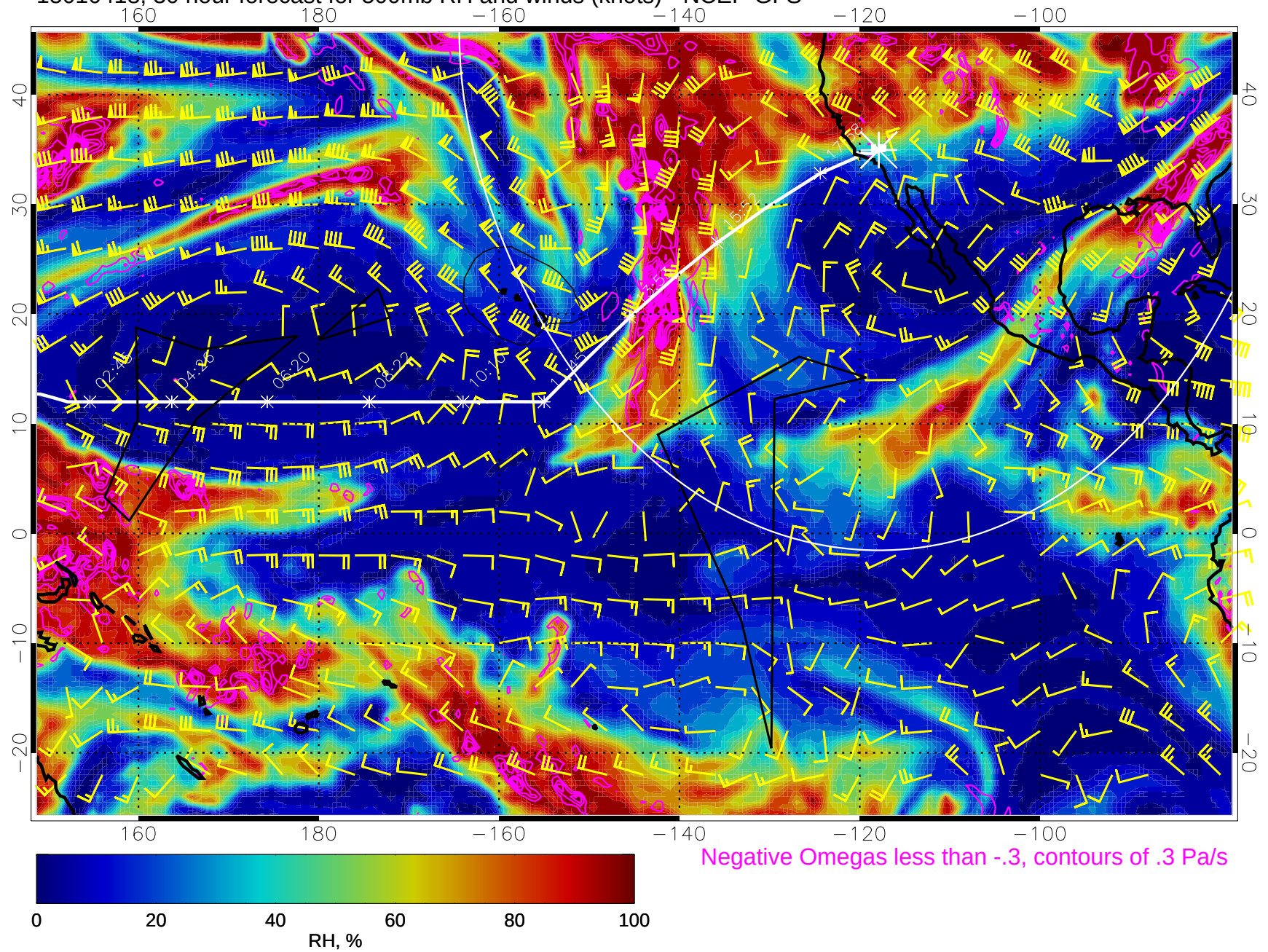
15010418, 30 hour forecast for 500mb RH and winds (knots) - NCEP GFS
