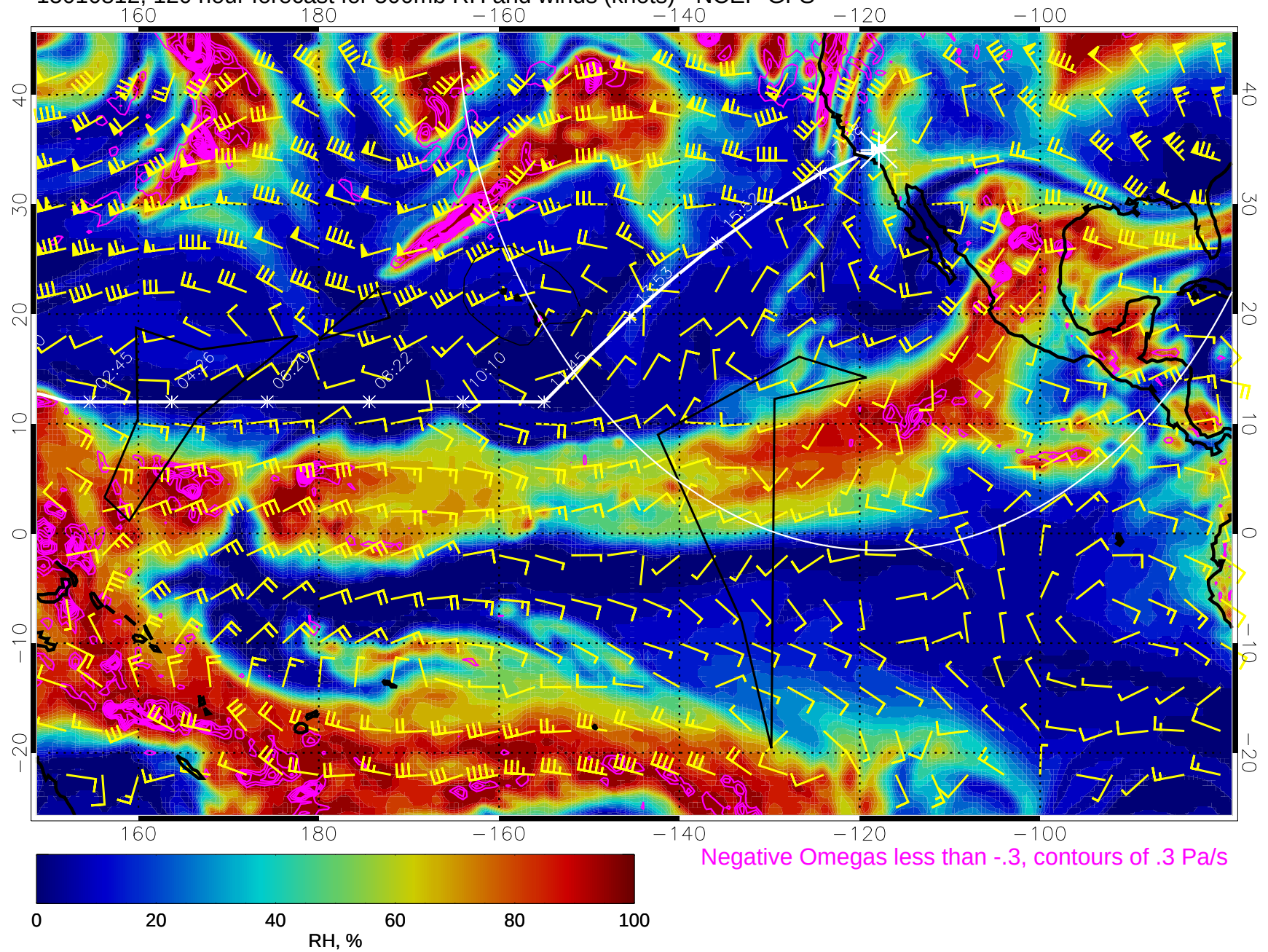
15010812, 120 hour forecast for 500mb RH and winds (knots) - NCEP GFS
