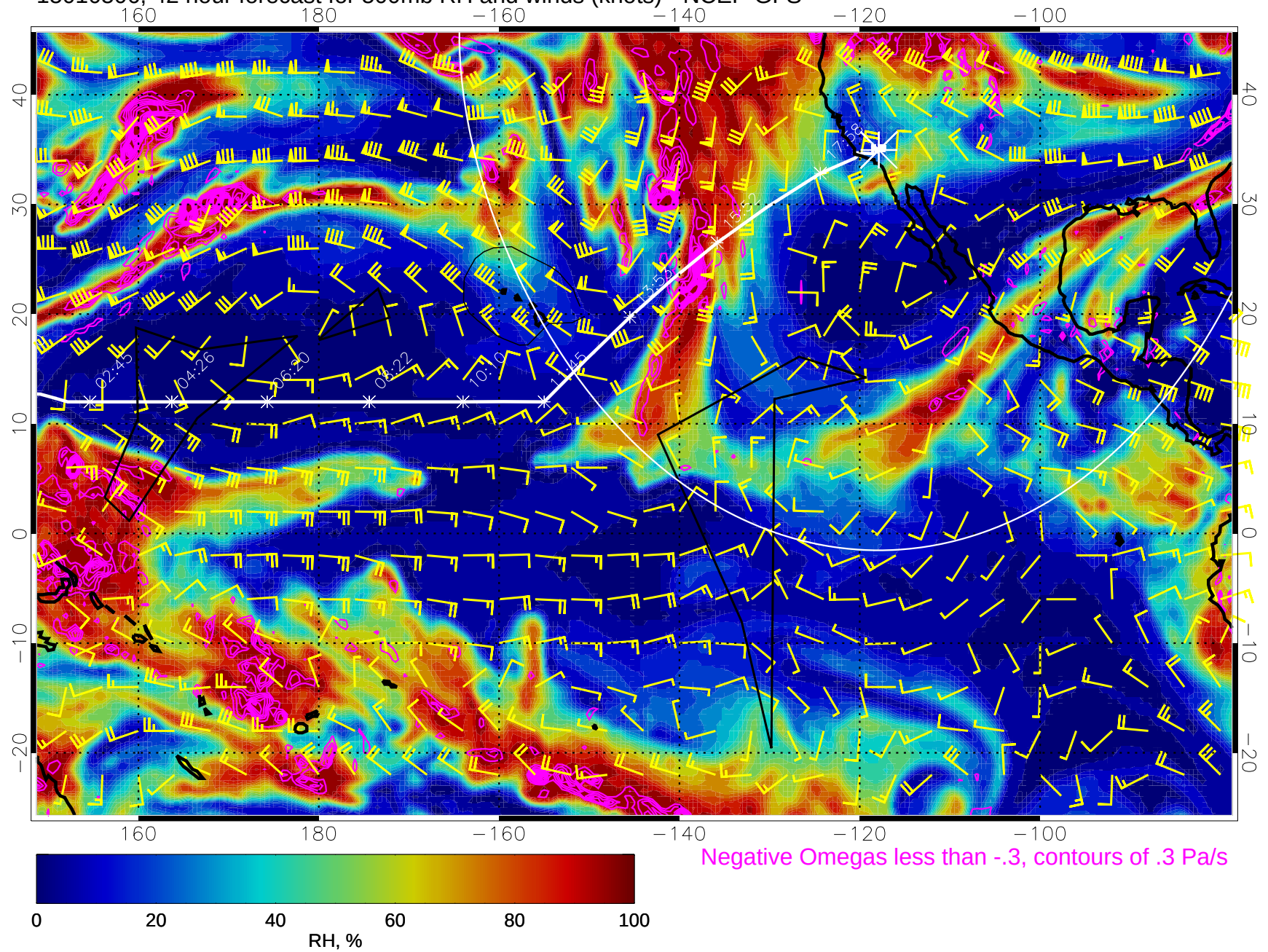
15010506, 42 hour forecast for 500mb RH and winds (knots) - NCEP GFS
