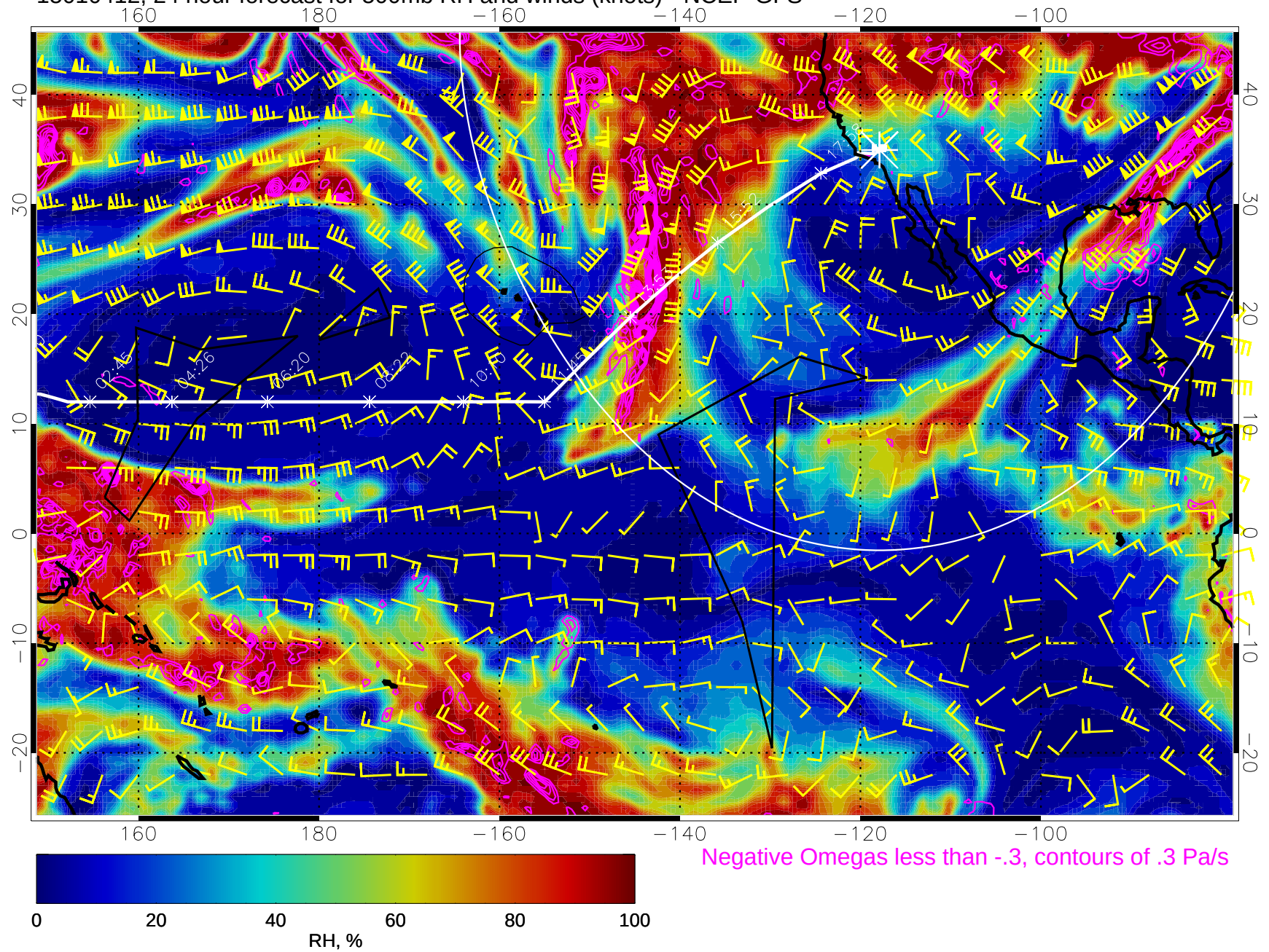
15010412, 24 hour forecast for 500mb RH and winds (knots) - NCEP GFS
