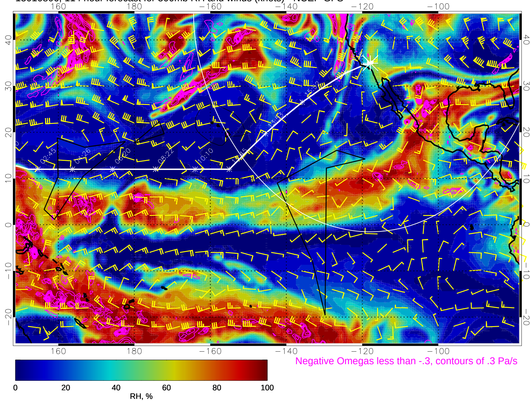
15010806, 114 hour forecast for 500mb RH and winds (knots) - NCEP GFS
