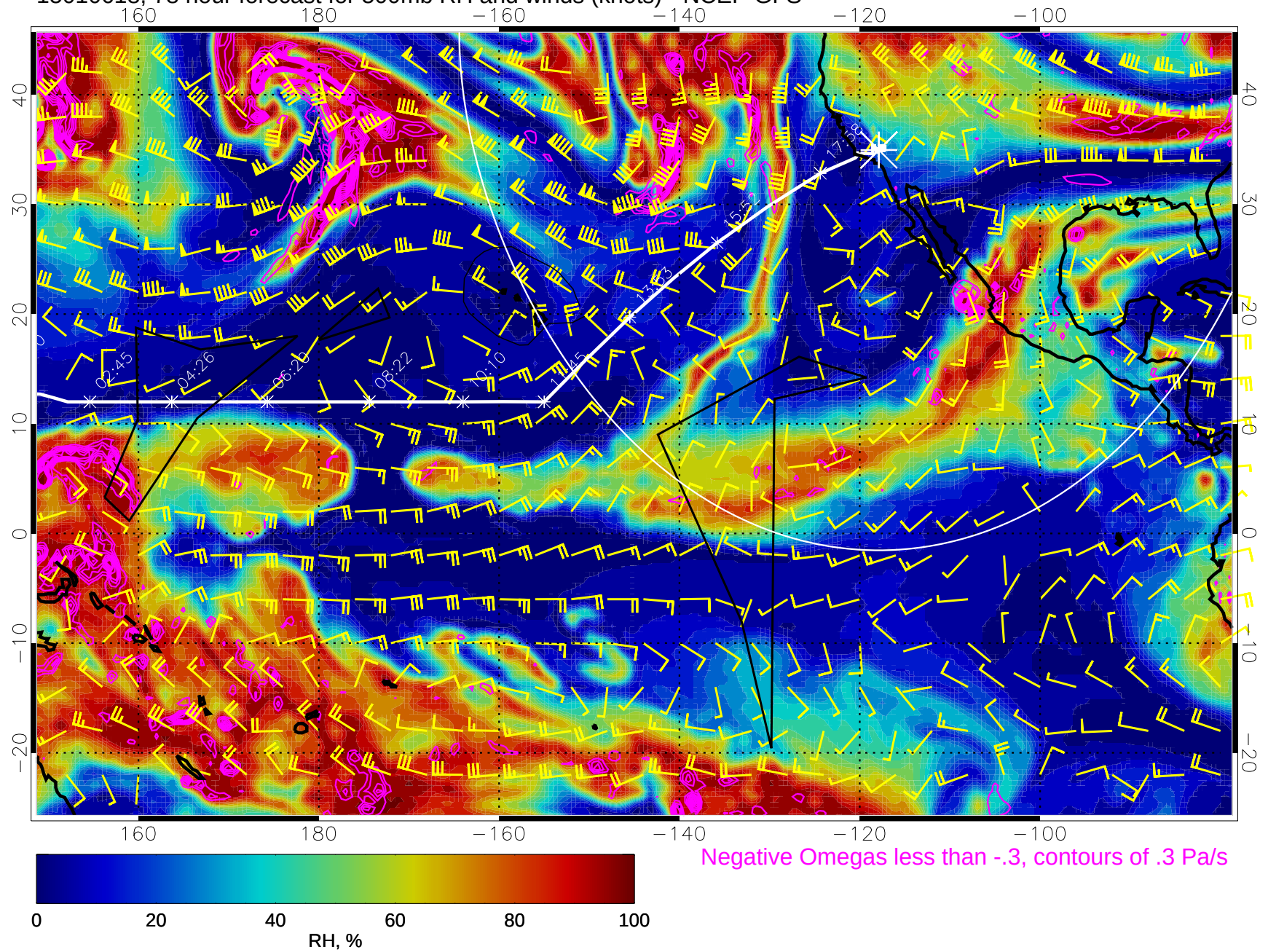
15010618, 78 hour forecast for 500mb RH and winds (knots) - NCEP GFS
