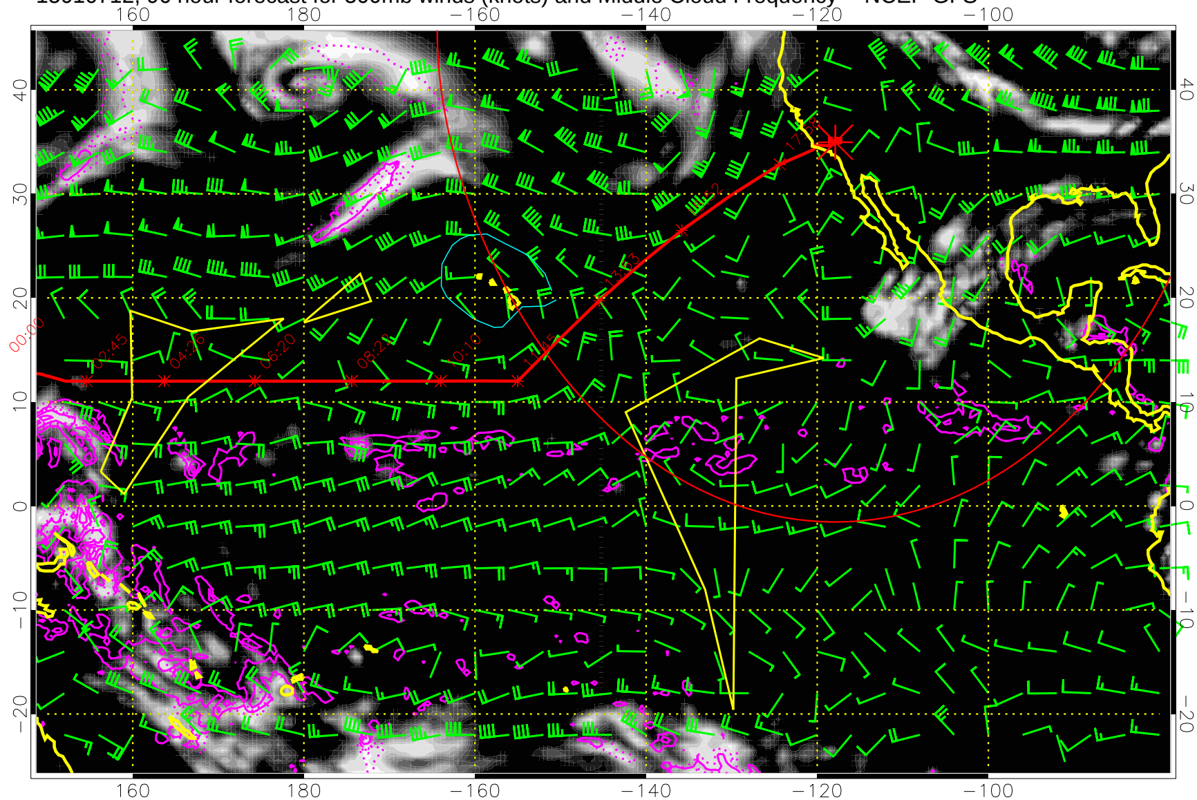
15010712, 96 hour forecast for 500mb winds (knots) and Middle Cloud Frequency -- NCEP GFS
