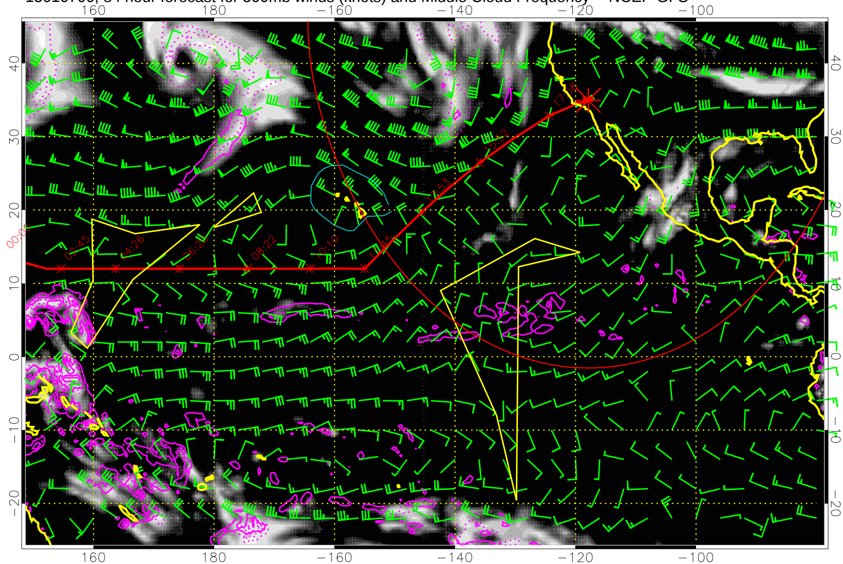
15010700, 84 hour forecast for 500mb winds (knots) and Middle Cloud Frequency -- NCEP GFS
