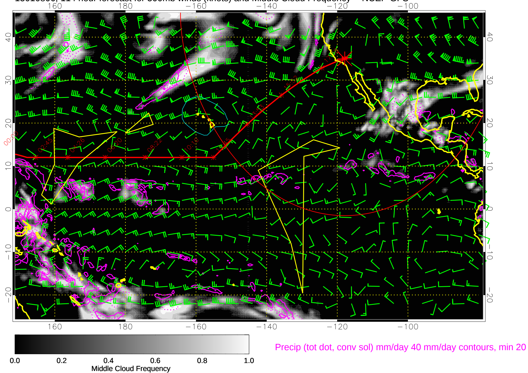
15010806, 114 hour forecast for 500mb winds (knots) and Middle Cloud Frequency -- NCEP GFS
