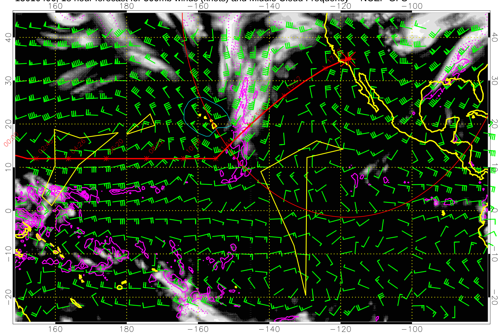
15010406, 18 hour forecast for 500mb winds (knots) and Middle Cloud Frequency -- NCEP GFS
