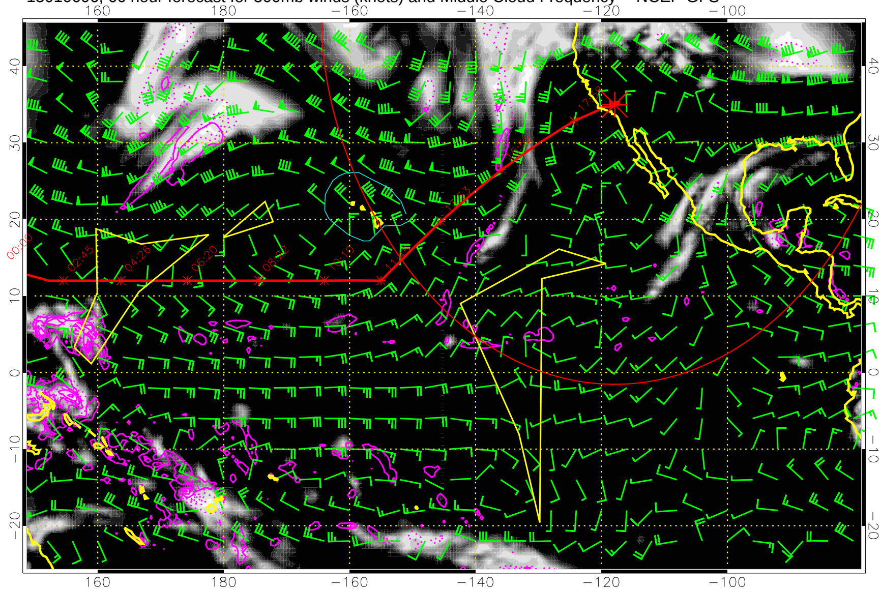
15010606, 66 hour forecast for 500mb winds (knots) and Middle Cloud Frequency -- NCEP GFS
