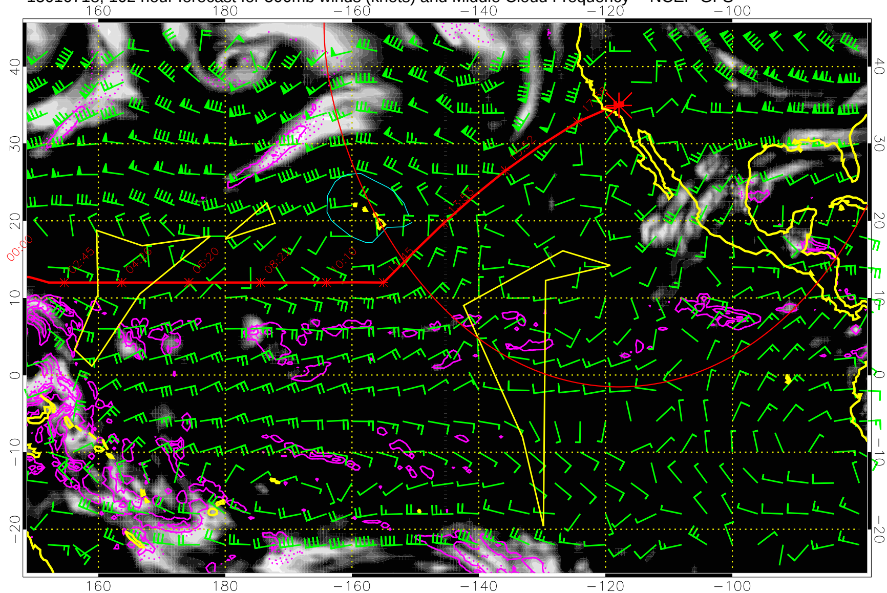
15010718, 102 hour forecast for 500mb winds (knots) and Middle Cloud Frequency -- NCEP GFS
