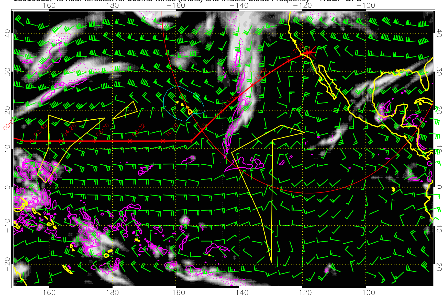
15010512, 48 hour forecast for 500mb winds (knots) and Middle Cloud Frequency -- NCEP GFS
