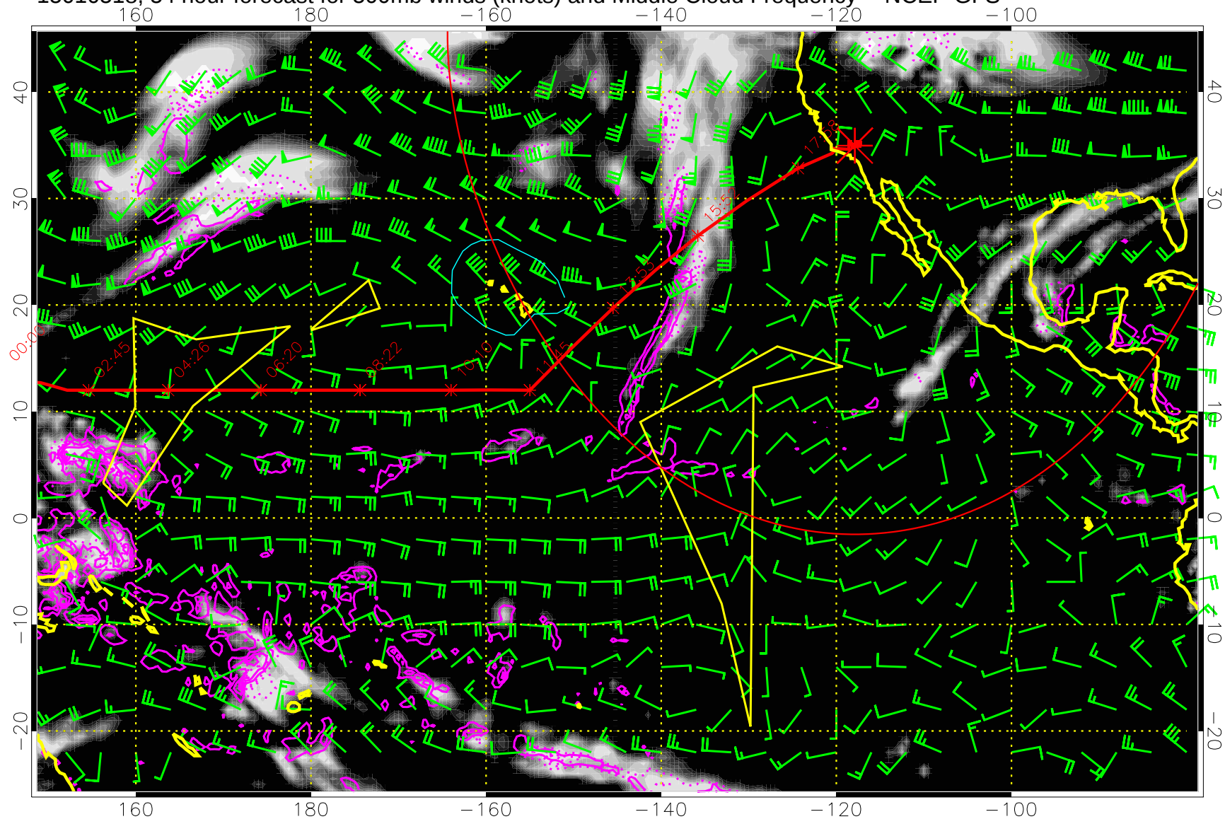
15010518, 54 hour forecast for 500mb winds (knots) and Middle Cloud Frequency -- NCEP GFS
