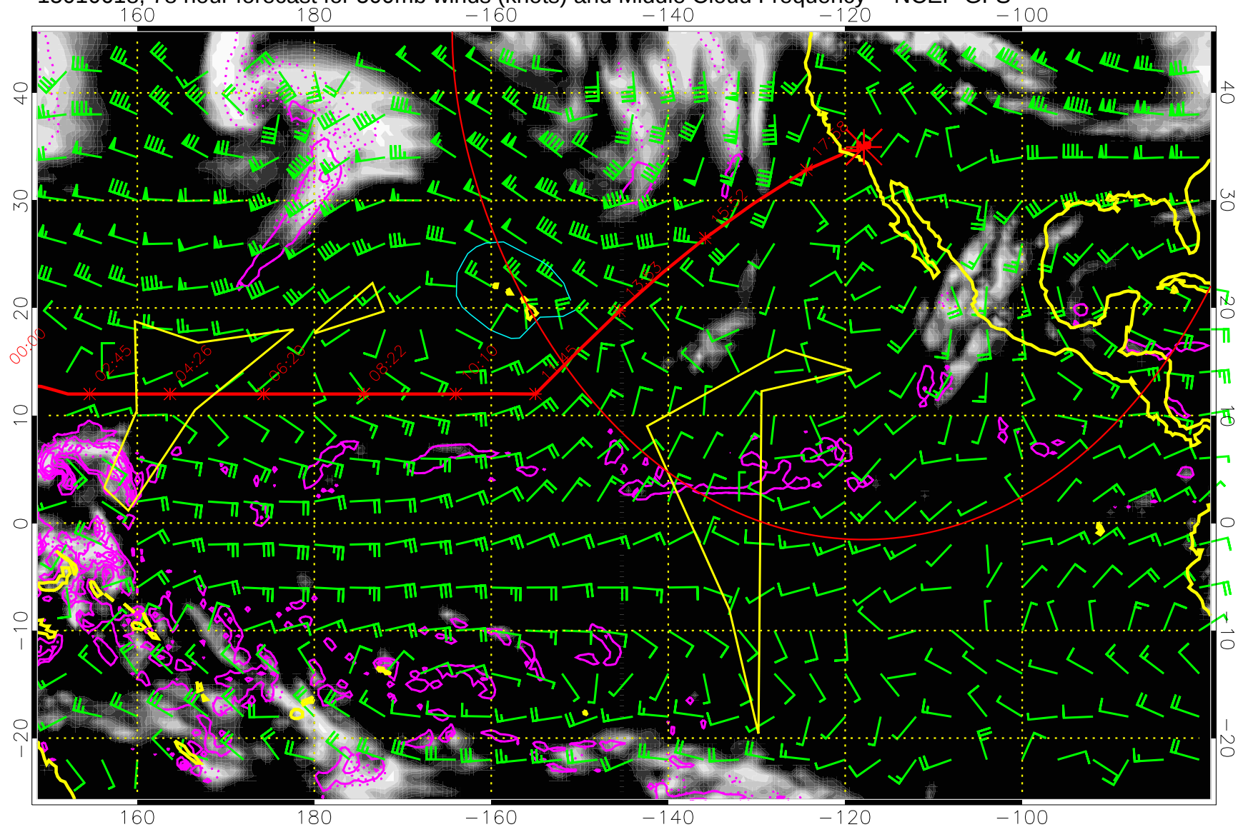
15010618, 78 hour forecast for 500mb winds (knots) and Middle Cloud Frequency -- NCEP GFS
