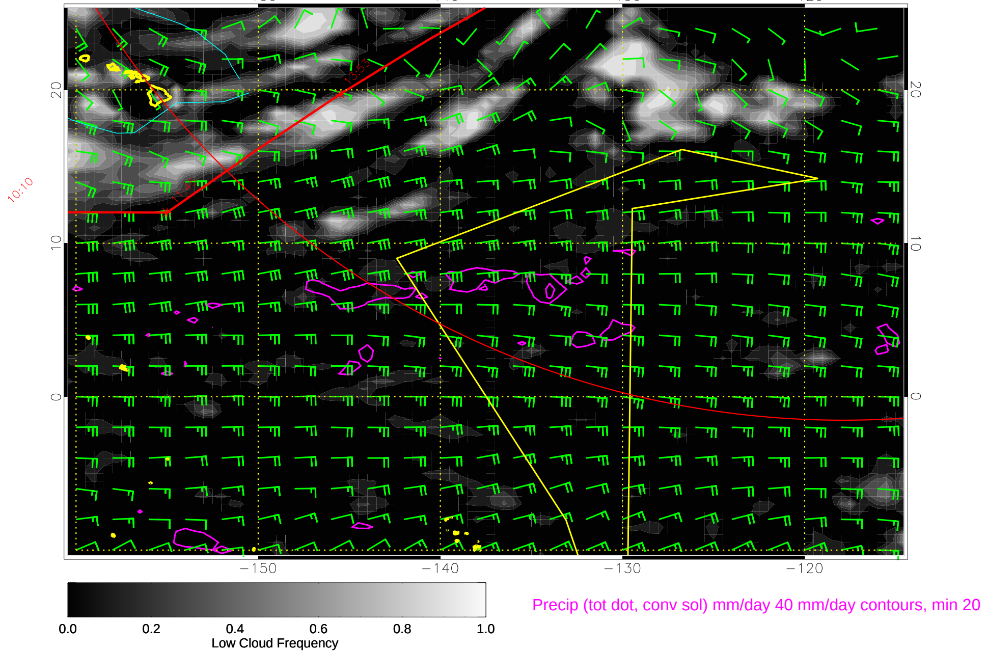
15010800, 108 hour forecast for 850mb winds (knots) and Low Cloud Frequency -- NCEP GFS
