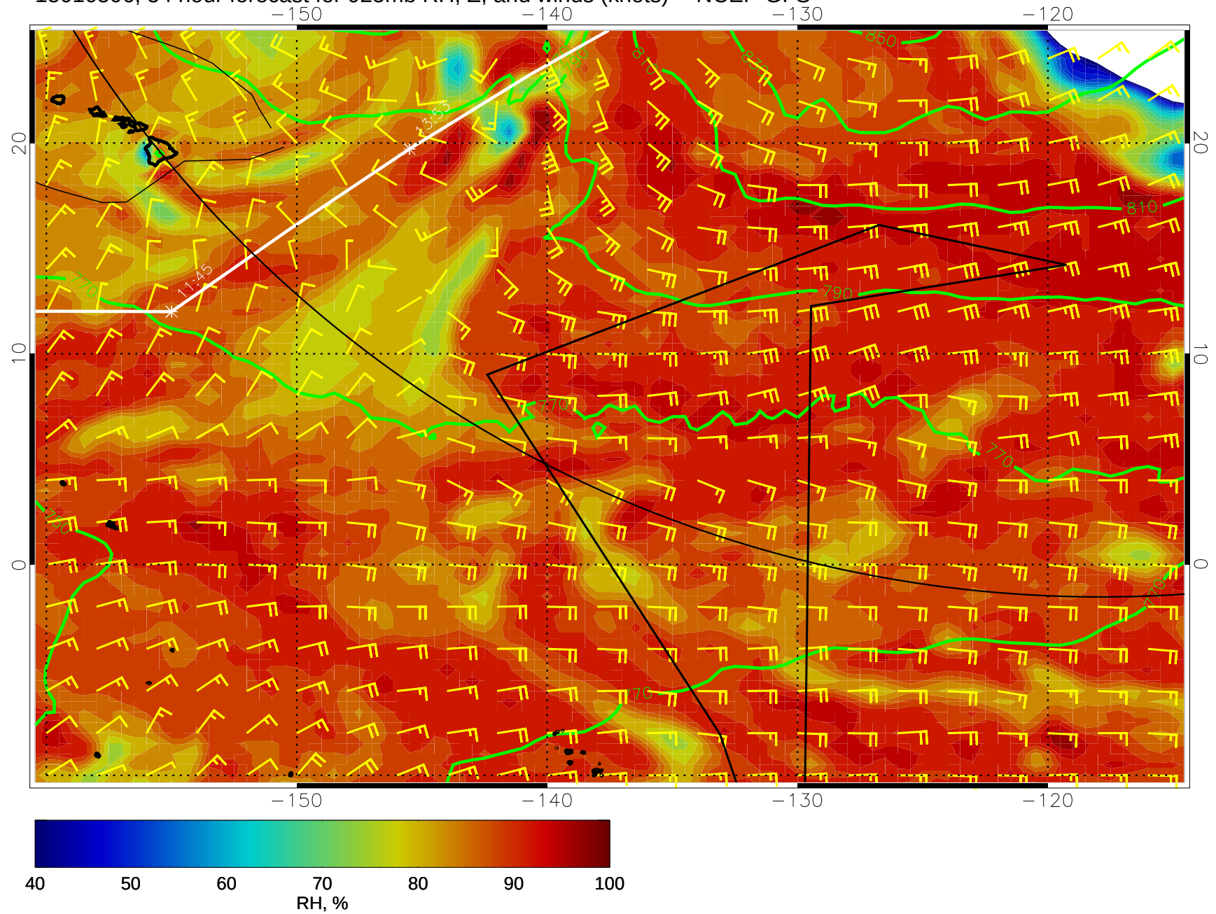
15010506, 54 hour forecast for 925mb RH, Z, and winds (knots) -- NCEP GFS
