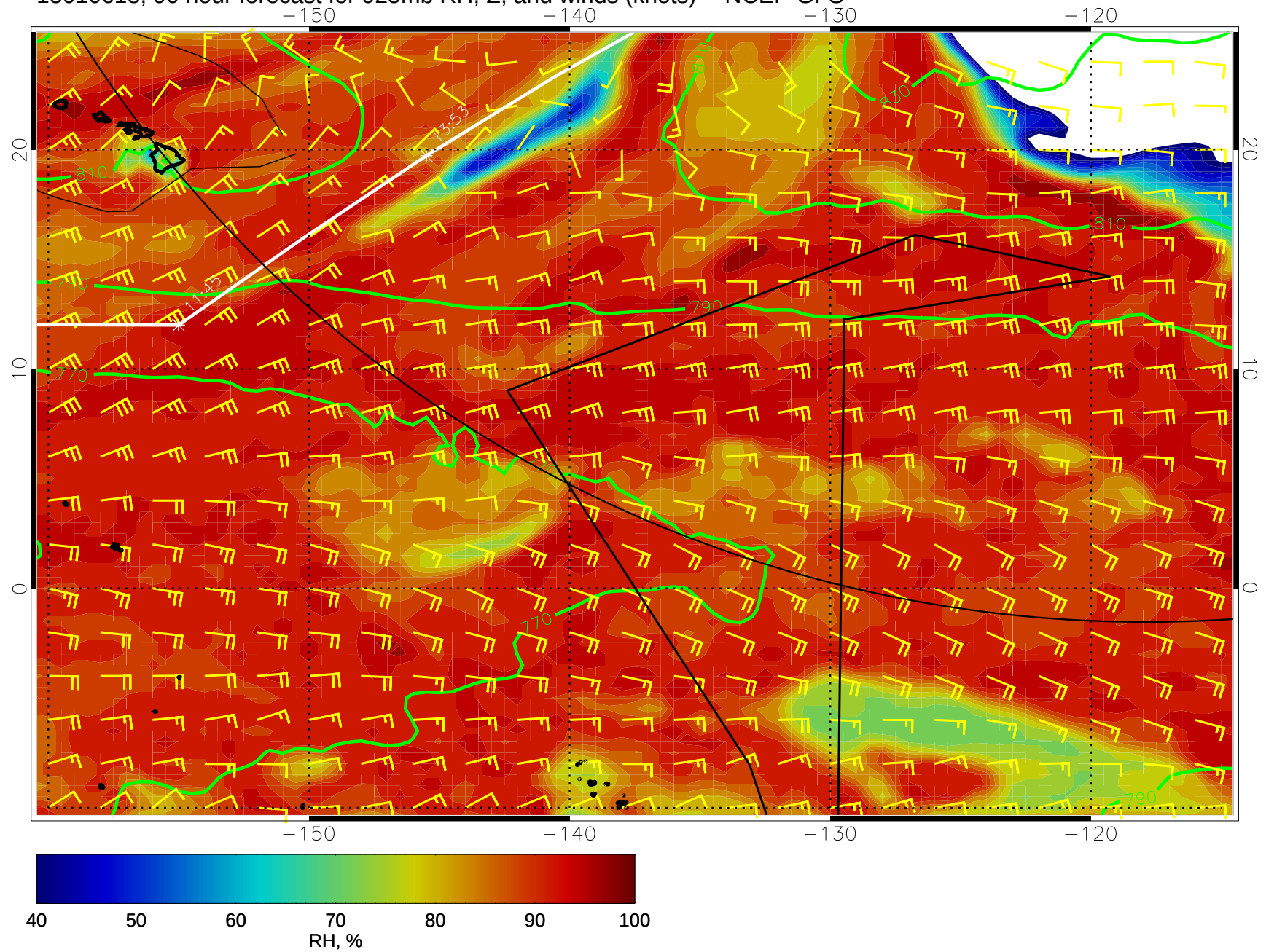
15010618, 90 hour forecast for 925mb RH, Z, and winds (knots) -- NCEP GFS
