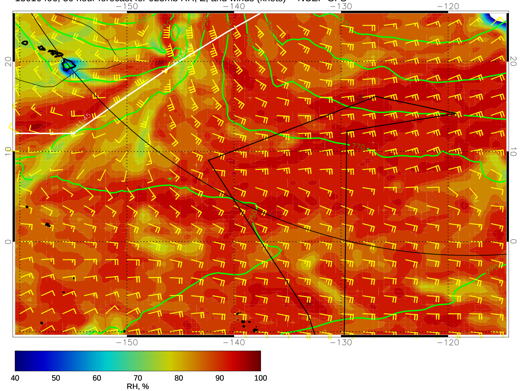
15010406, 30 hour forecast for 925mb RH, Z, and winds (knots) -- NCEP GFS
