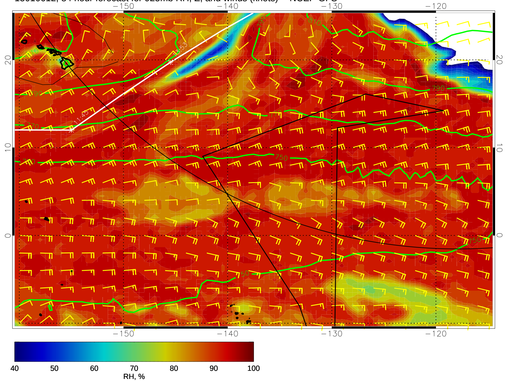
15010612, 84 hour forecast for 925mb RH, Z, and winds (knots) -- NCEP GFS
