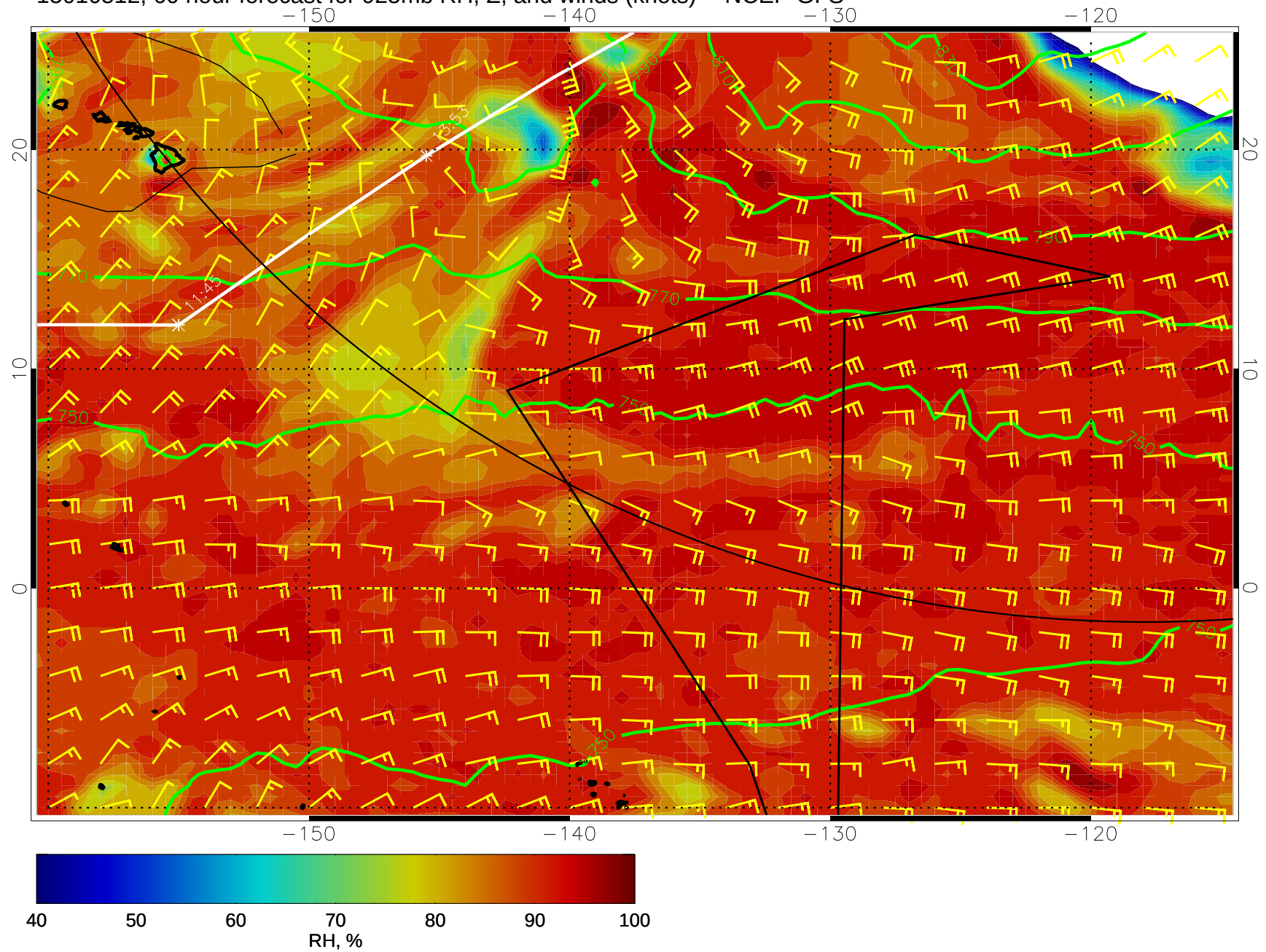
15010512, 60 hour forecast for 925mb RH, Z, and winds (knots) -- NCEP GFS
