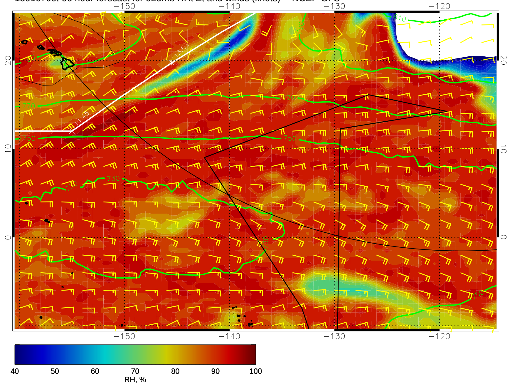
15010700, 96 hour forecast for 925mb RH, Z, and winds (knots) -- NCEP GFS
