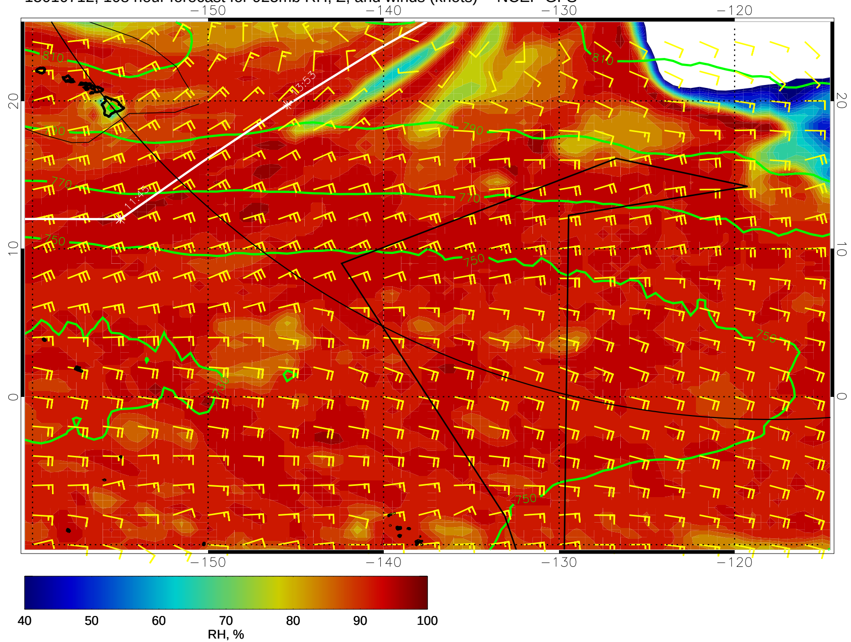
15010712, 108 hour forecast for 925mb RH, Z, and winds (knots) -- NCEP GFS
