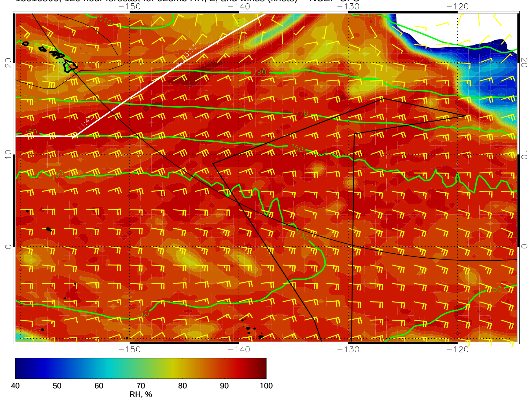
15010800, 120 hour forecast for 925mb RH, Z, and winds (knots) -- NCEP GFS
