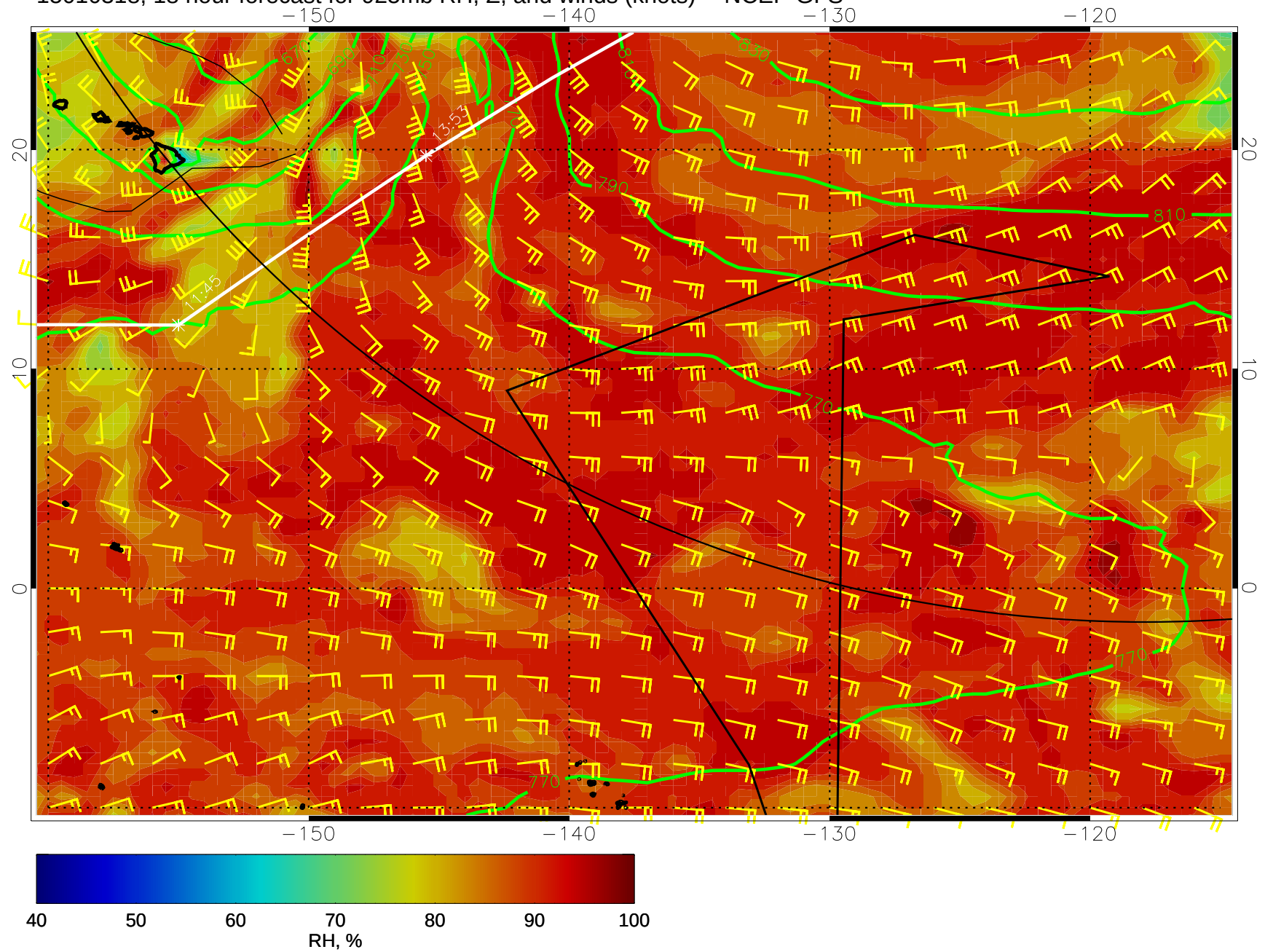
15010318, 18 hour forecast for 925mb RH, Z, and winds (knots) -- NCEP GFS
