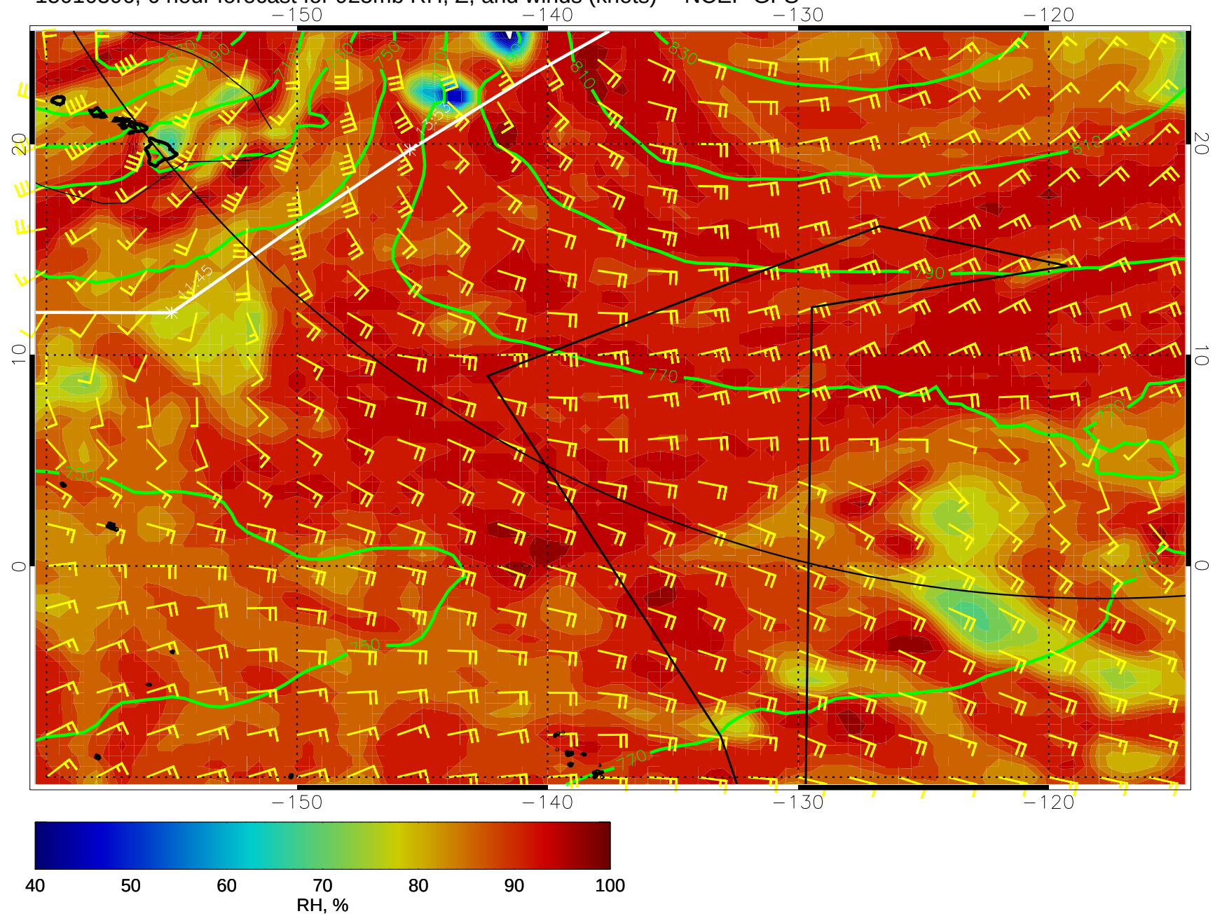
15010306, 6 hour forecast for 925mb RH, Z, and winds (knots) -- NCEP GFS
