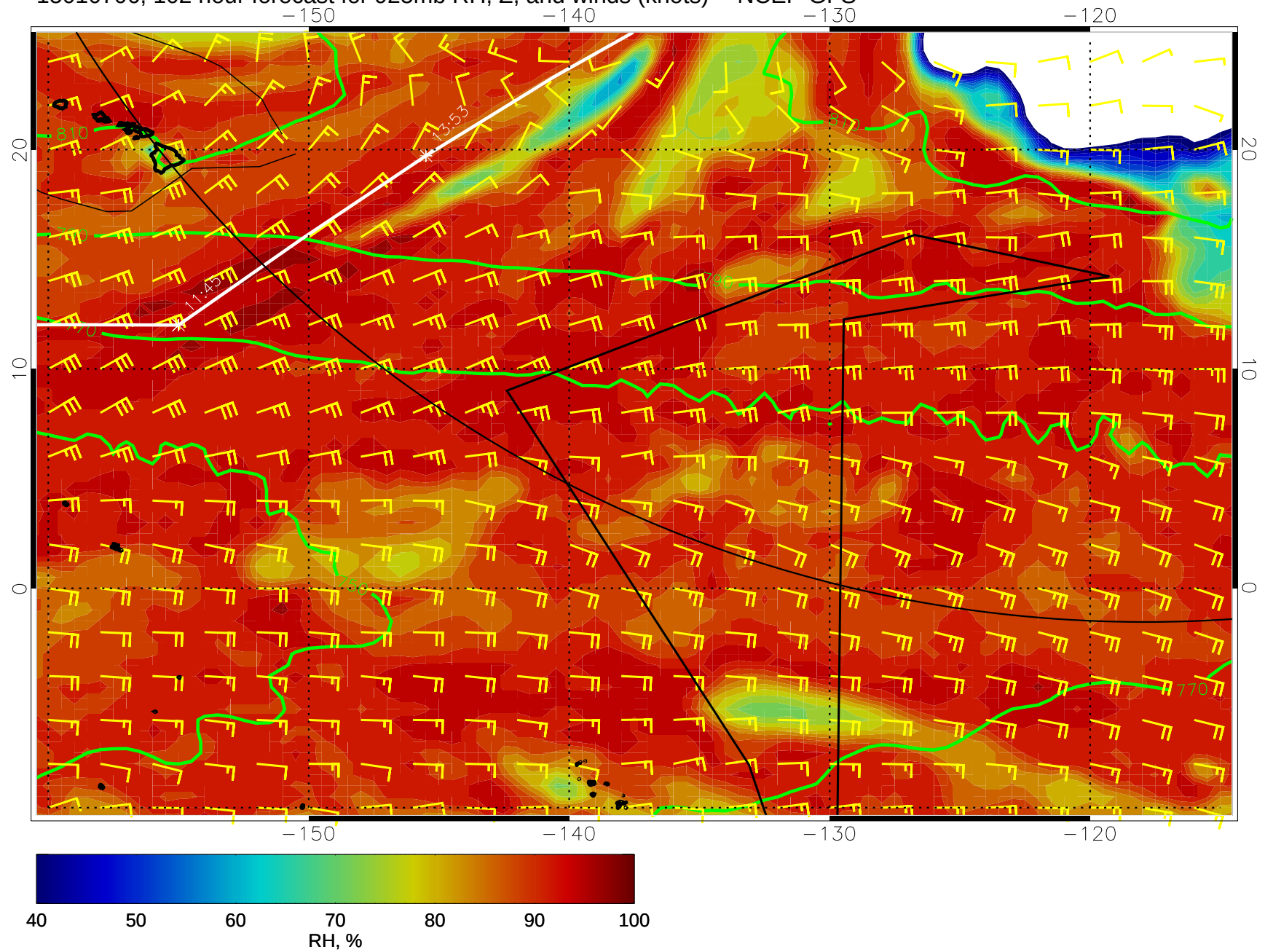
15010706, 102 hour forecast for 925mb RH, Z, and winds (knots) -- NCEP GFS
