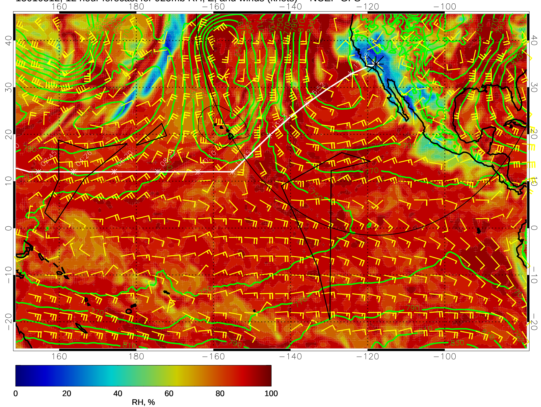
15010312, 12 hour forecast for 925mb RH, Z, and winds (knots) -- NCEP GFS
