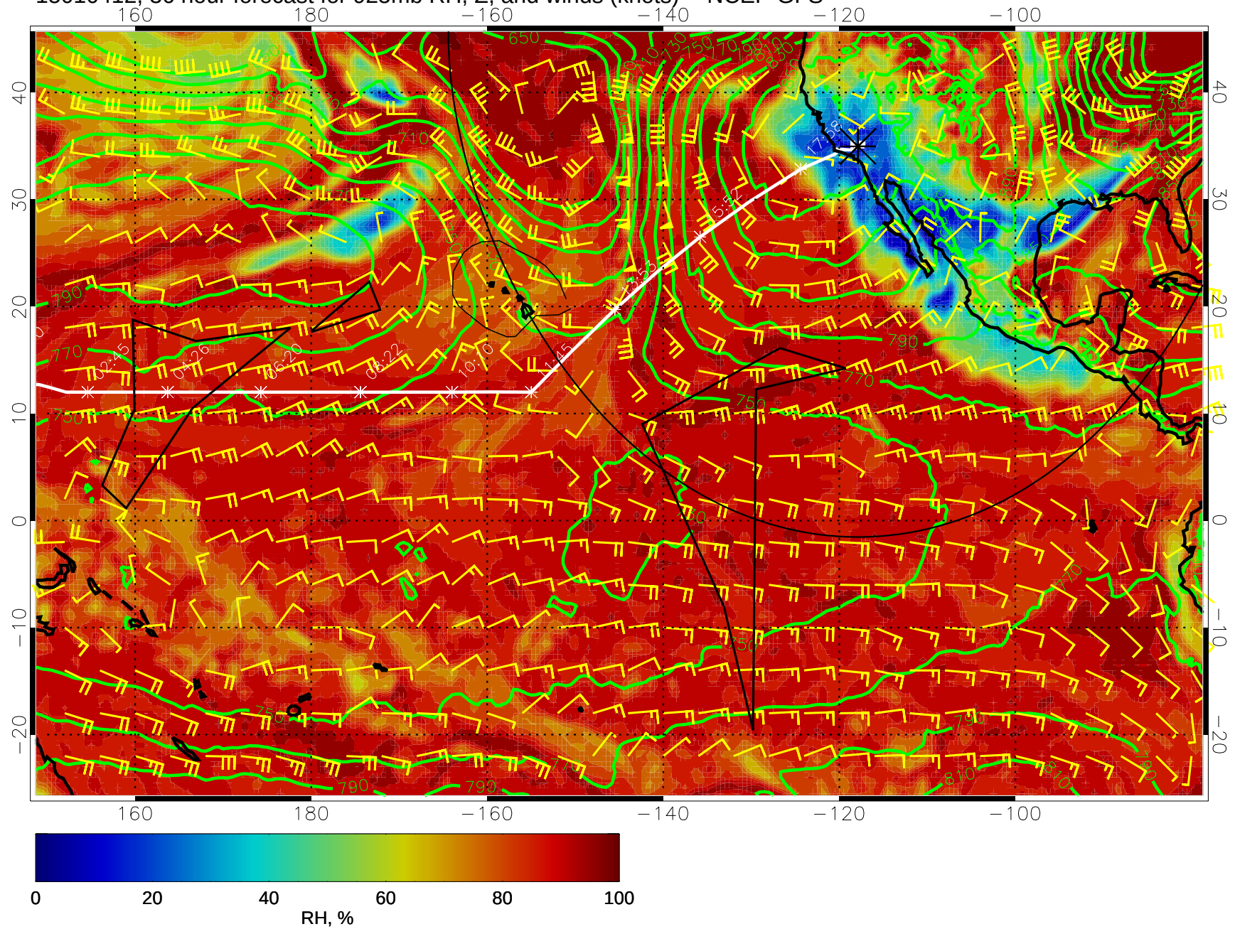
15010412, 36 hour forecast for 925mb RH, Z, and winds (knots) -- NCEP GFS
