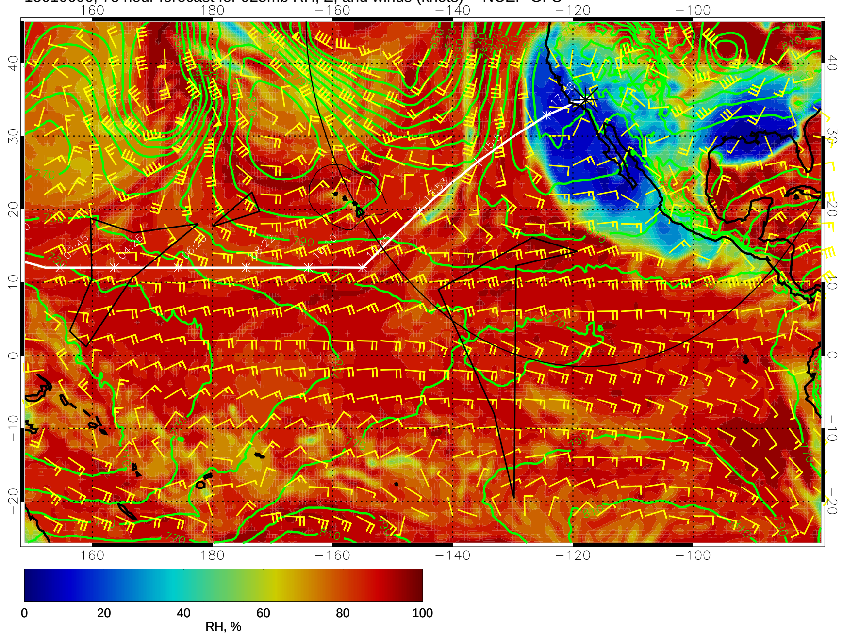
15010606, 78 hour forecast for 925mb RH, Z, and winds (knots) -- NCEP GFS
