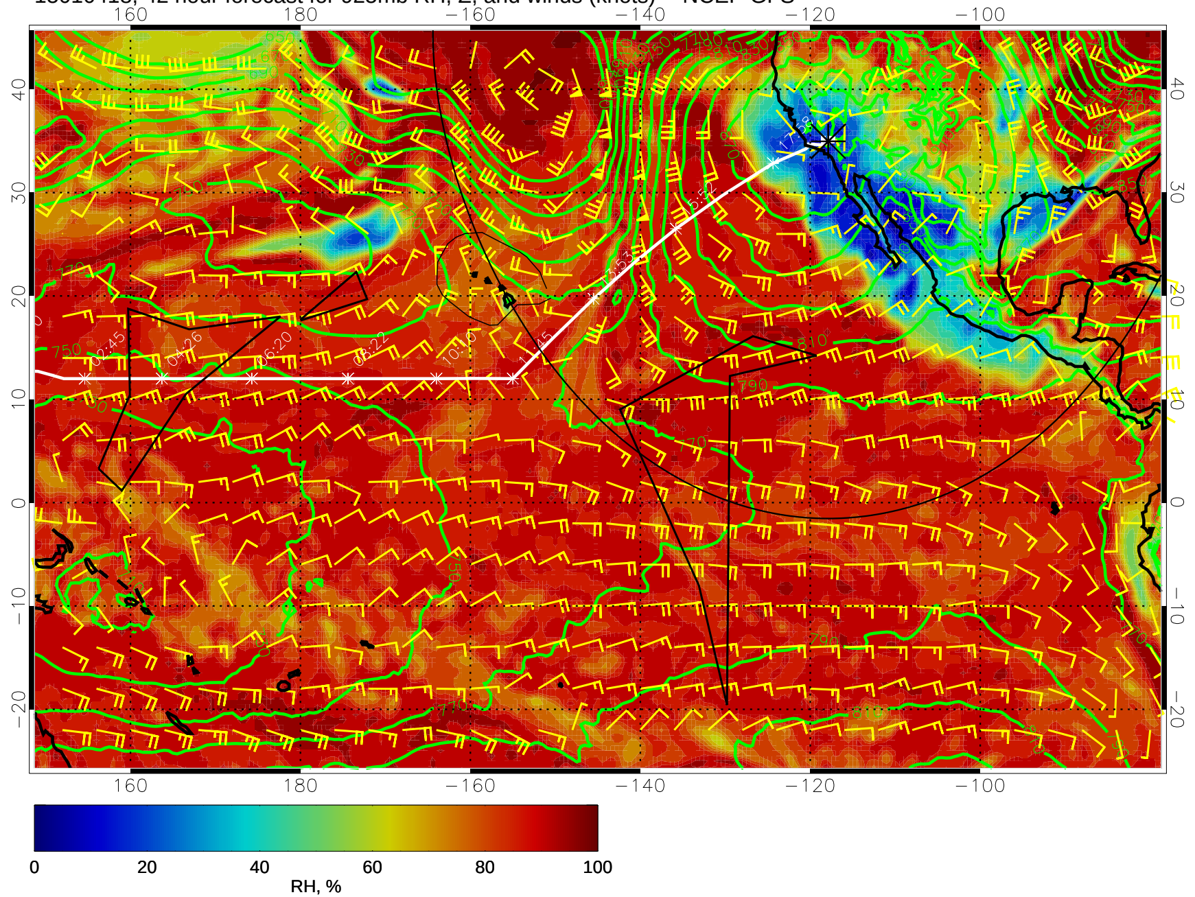
15010418, 42 hour forecast for 925mb RH, Z, and winds (knots) -- NCEP GFS
