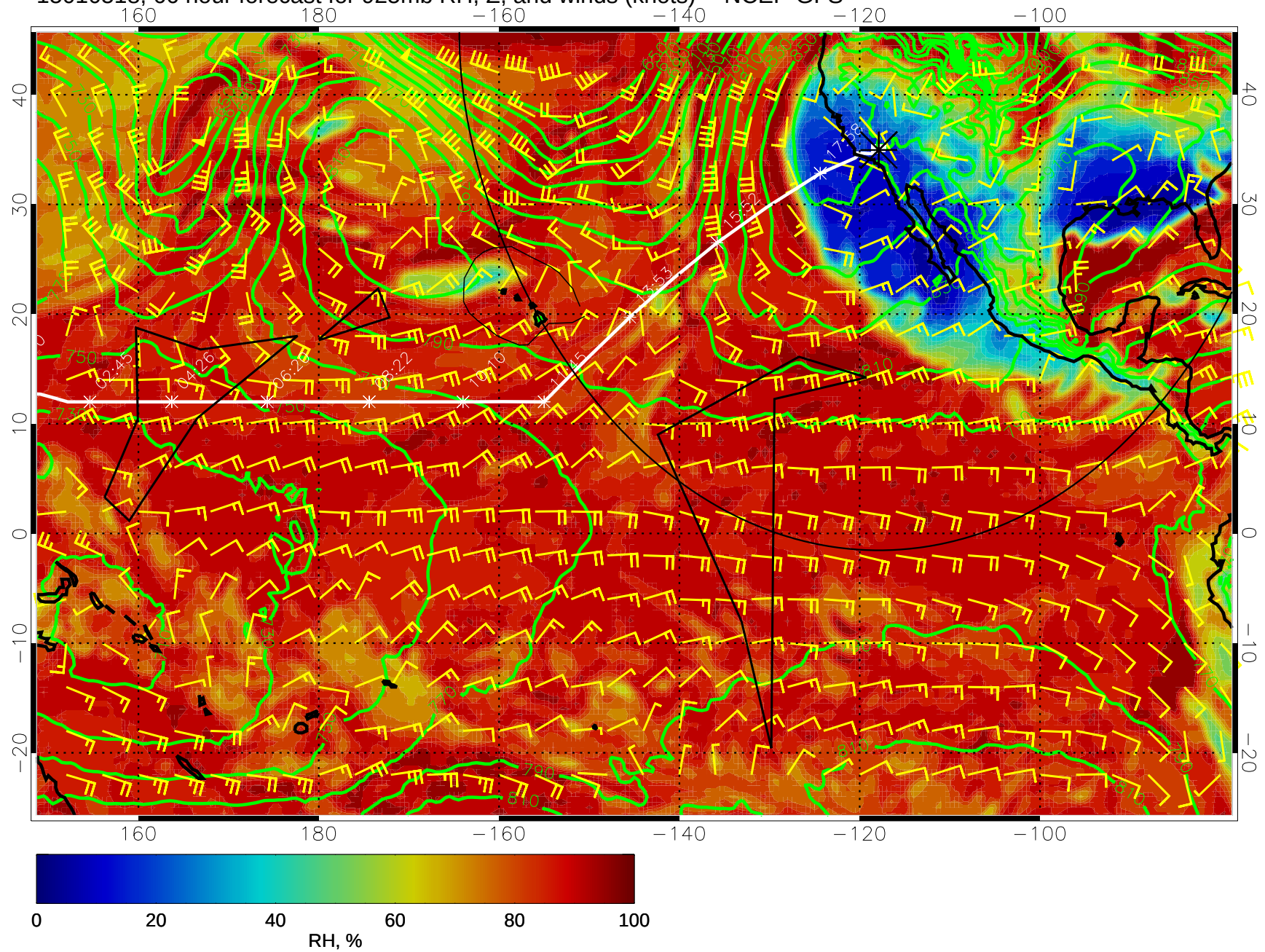
15010518, 66 hour forecast for 925mb RH, Z, and winds (knots) -- NCEP GFS
