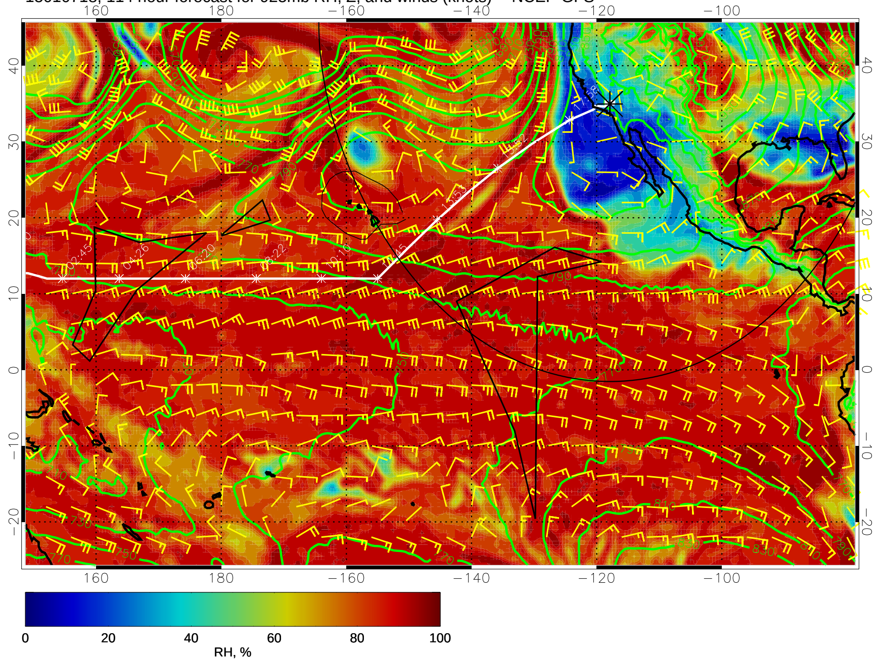
15010718, 114 hour forecast for 925mb RH, Z, and winds (knots) -- NCEP GFS
