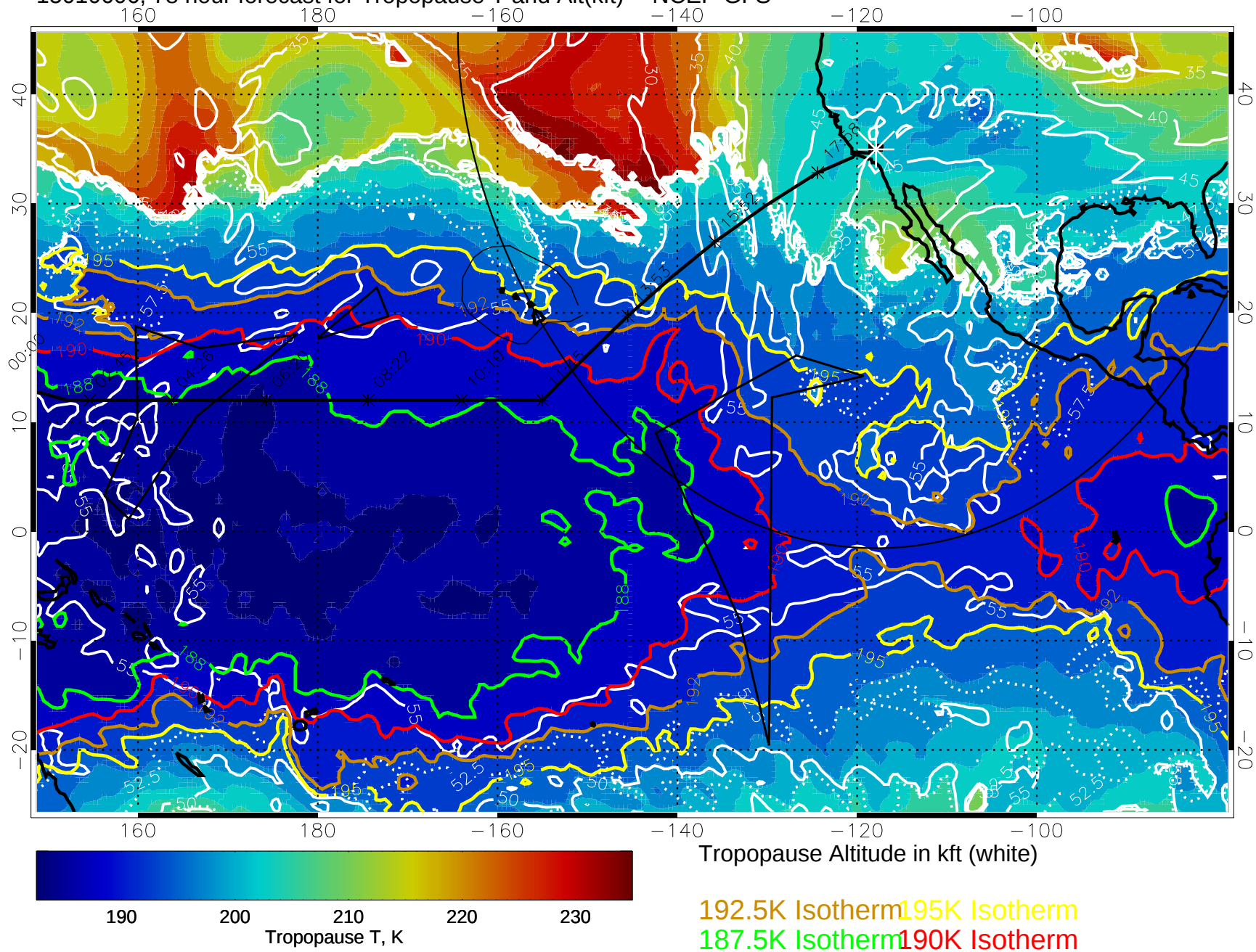
15010606, 78 hour forecast for Tropopause T and Alt(kft) -- NCEP GFS
