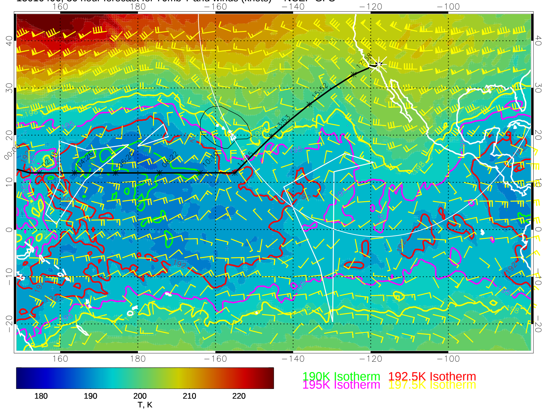
15010406, 30 hour forecast for 70mb T and winds (knots) -- NCEP GFS
