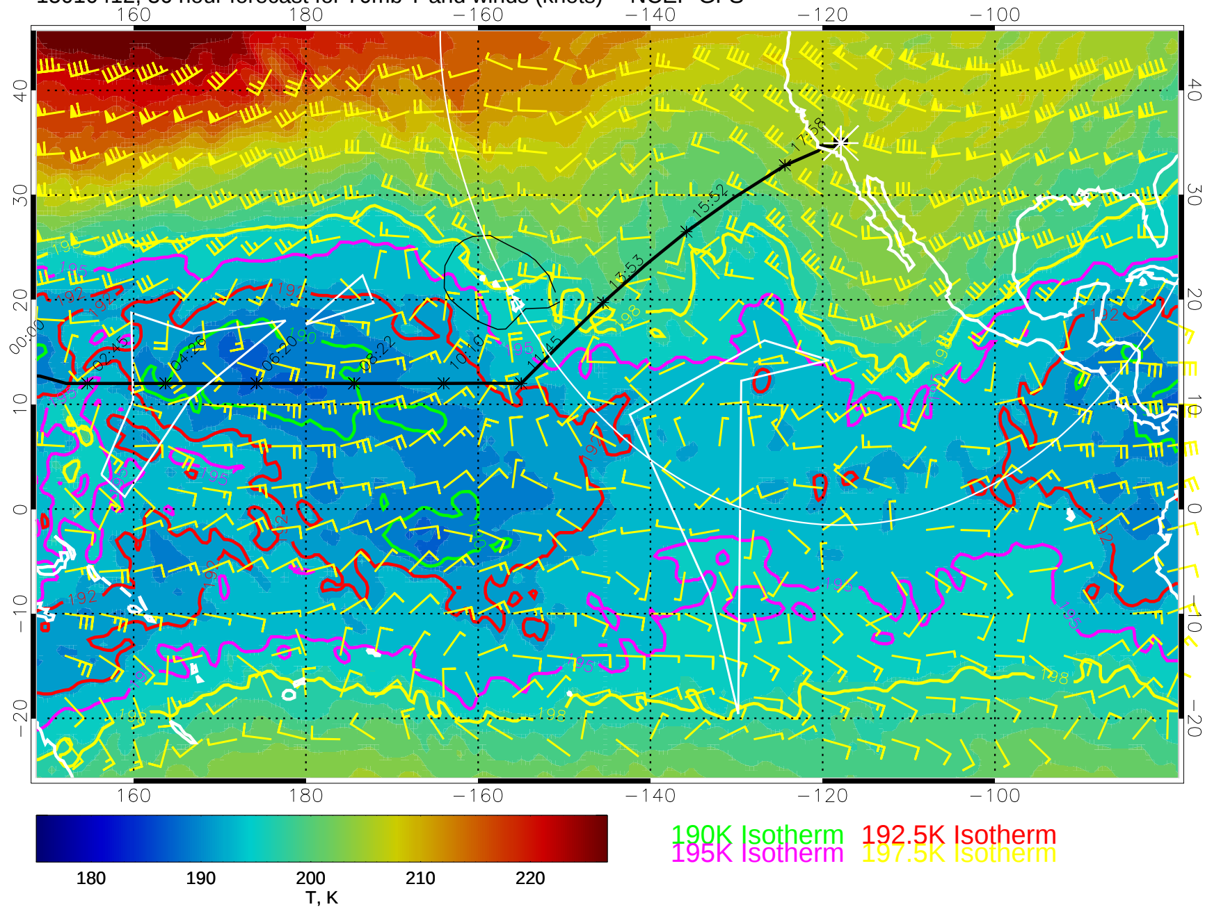
15010412, 36 hour forecast for 70mb T and winds (knots) -- NCEP GFS
