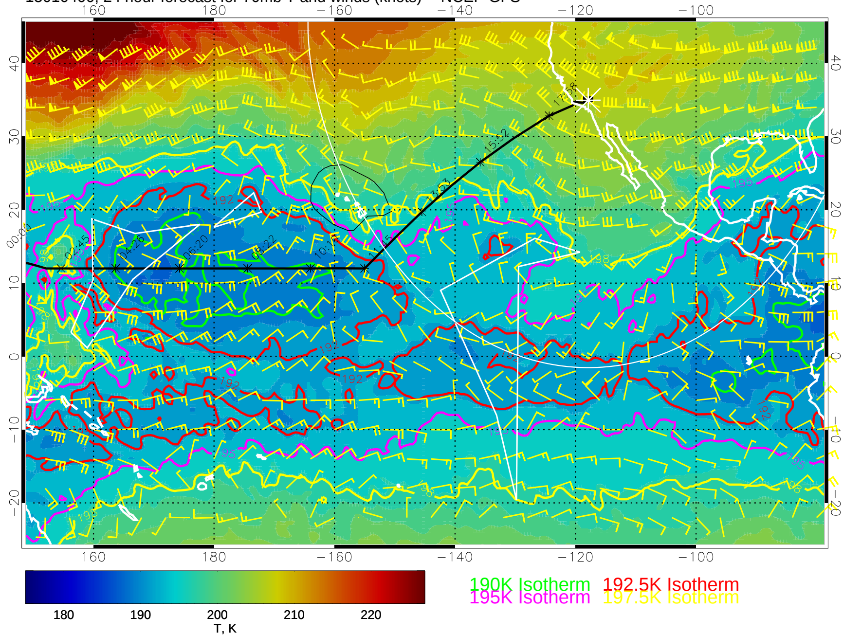
15010400, 24 hour forecast for 70mb T and winds (knots) -- NCEP GFS
