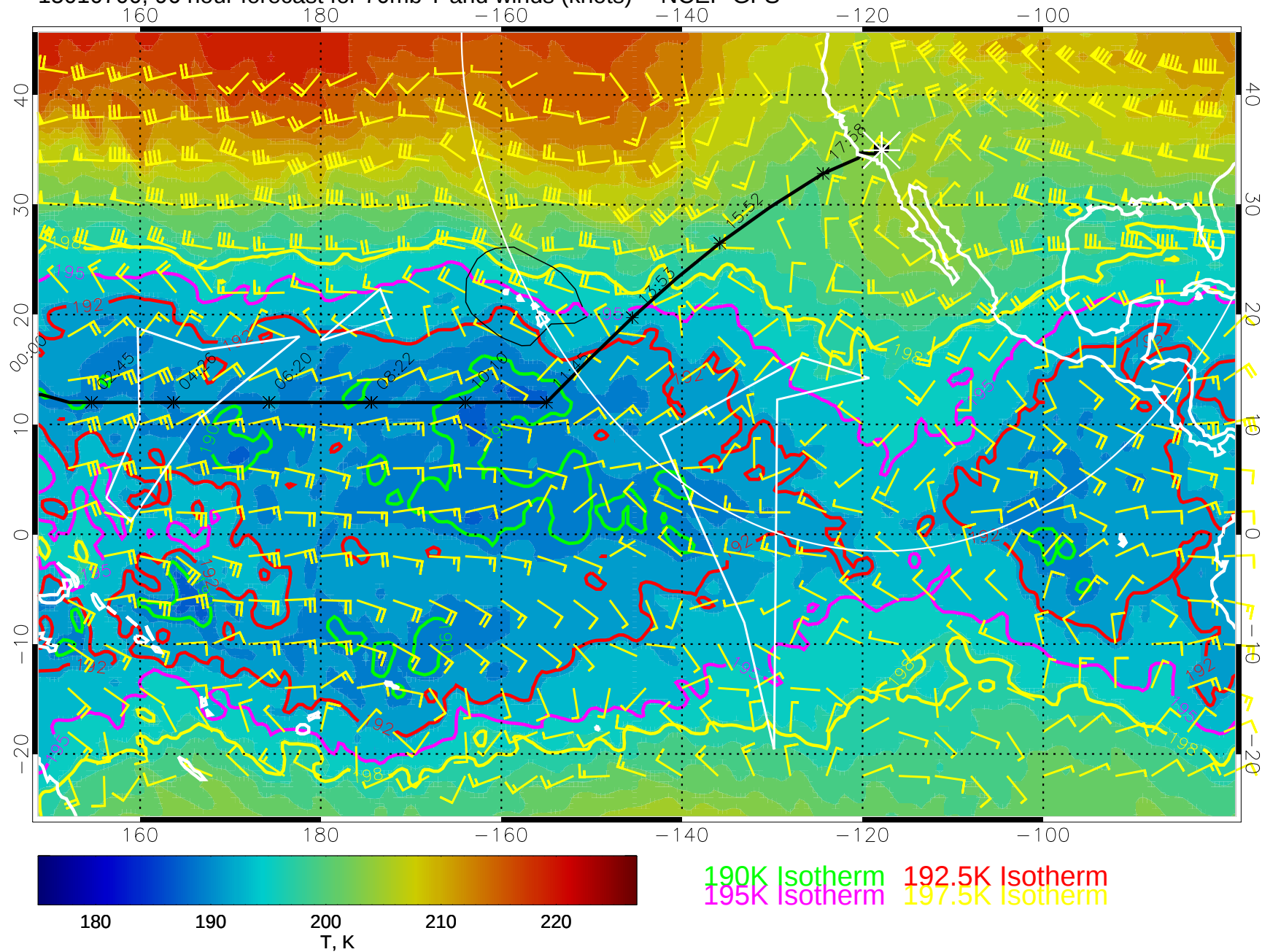
15010700, 96 hour forecast for 70mb T and winds (knots) -- NCEP GFS
