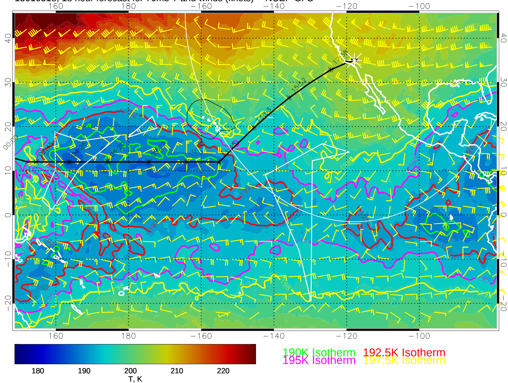
15010318, 18 hour forecast for 70mb T and winds (knots) -- NCEP GFS
