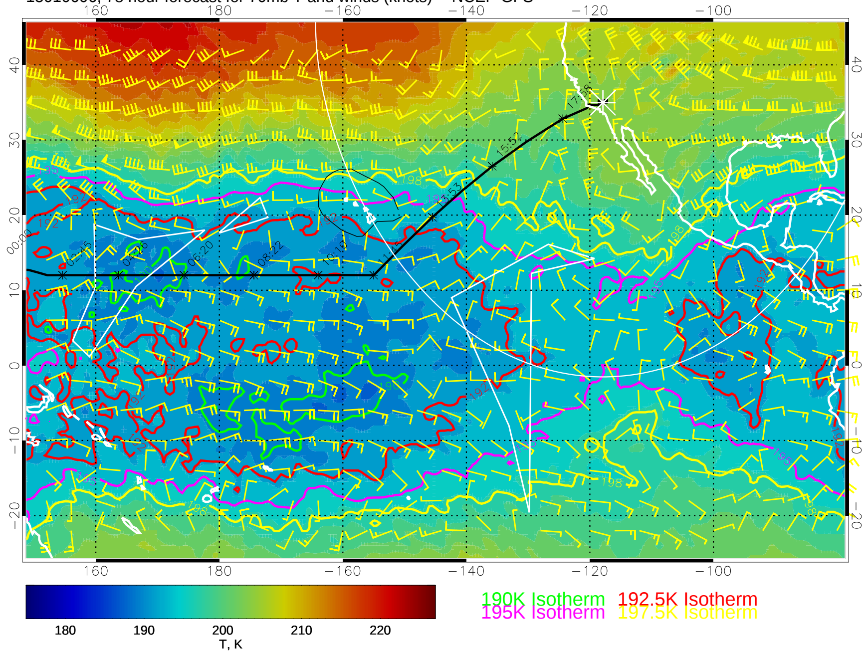
15010606, 78 hour forecast for 70mb T and winds (knots) -- NCEP GFS
