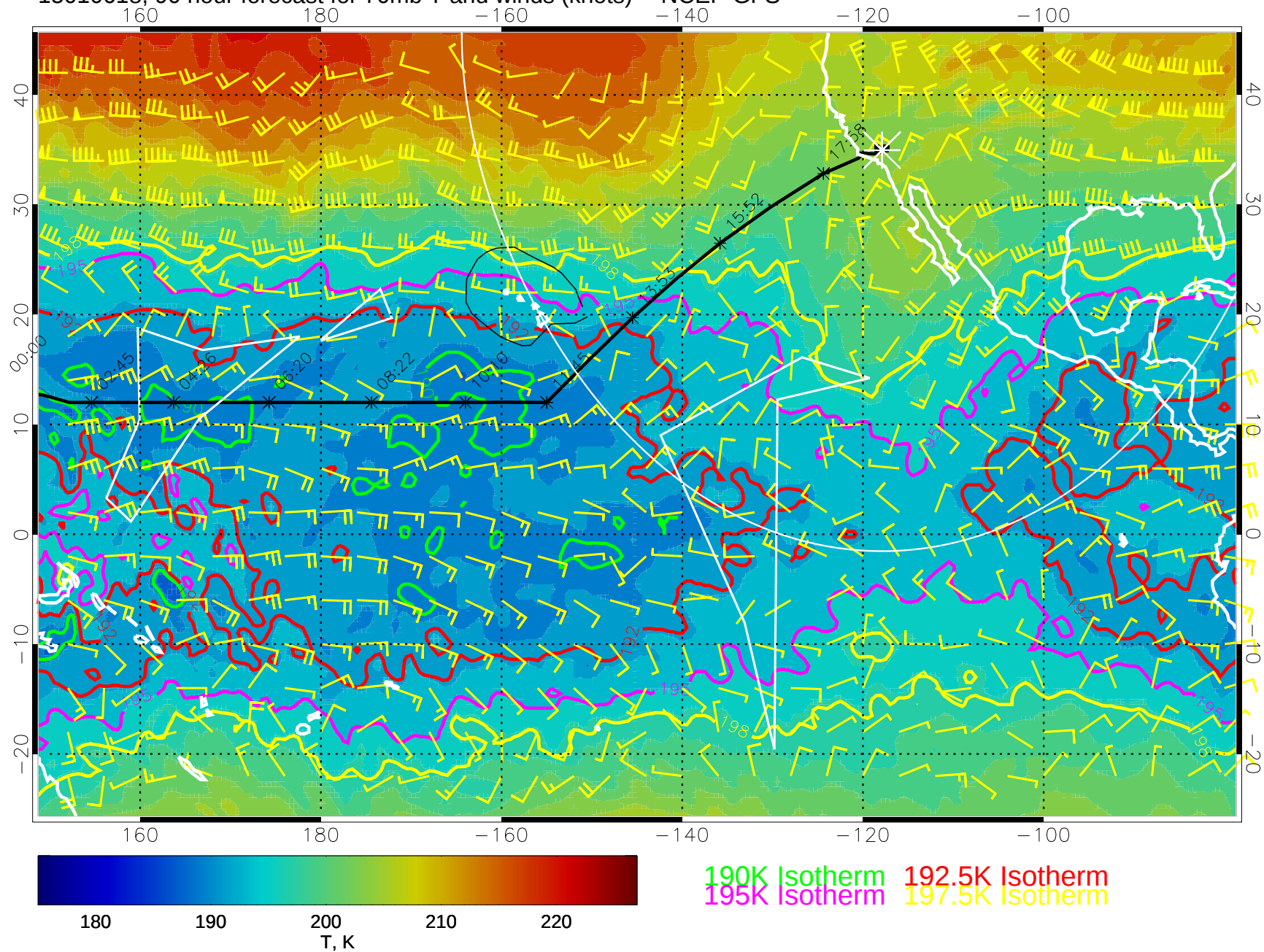
15010618, 90 hour forecast for 70mb T and winds (knots) -- NCEP GFS
