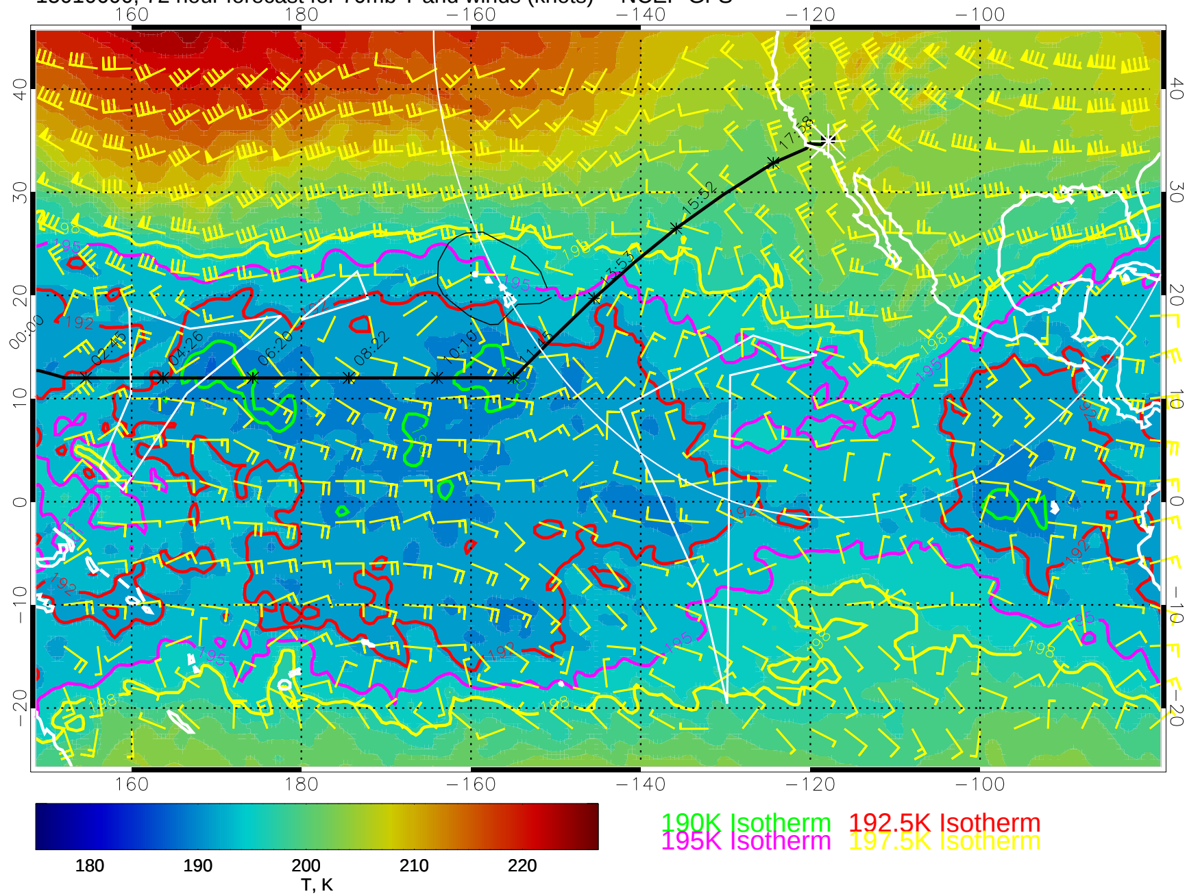
15010600, 72 hour forecast for 70mb T and winds (knots) -- NCEP GFS
