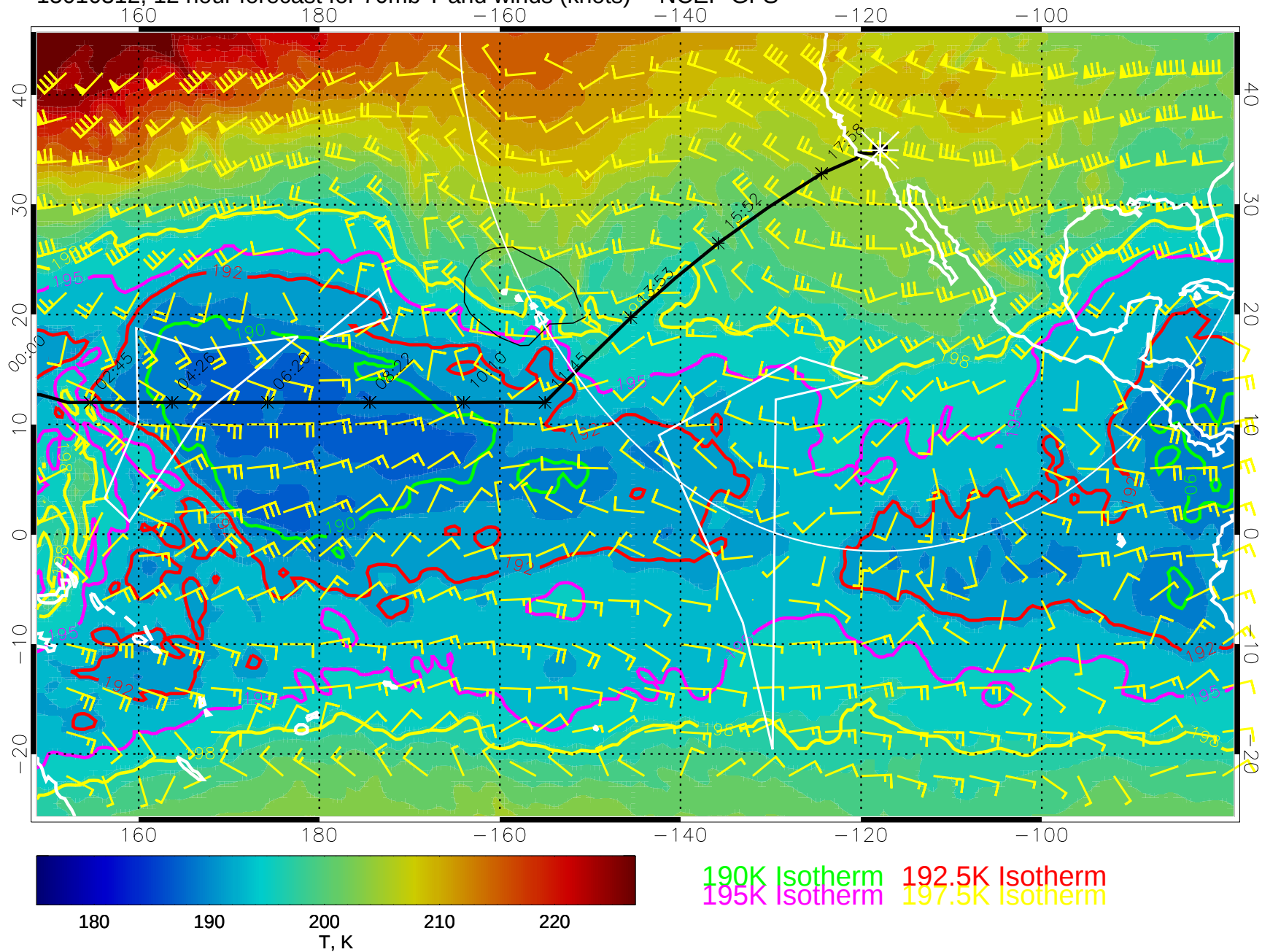
15010312, 12 hour forecast for 70mb T and winds (knots) -- NCEP GFS
