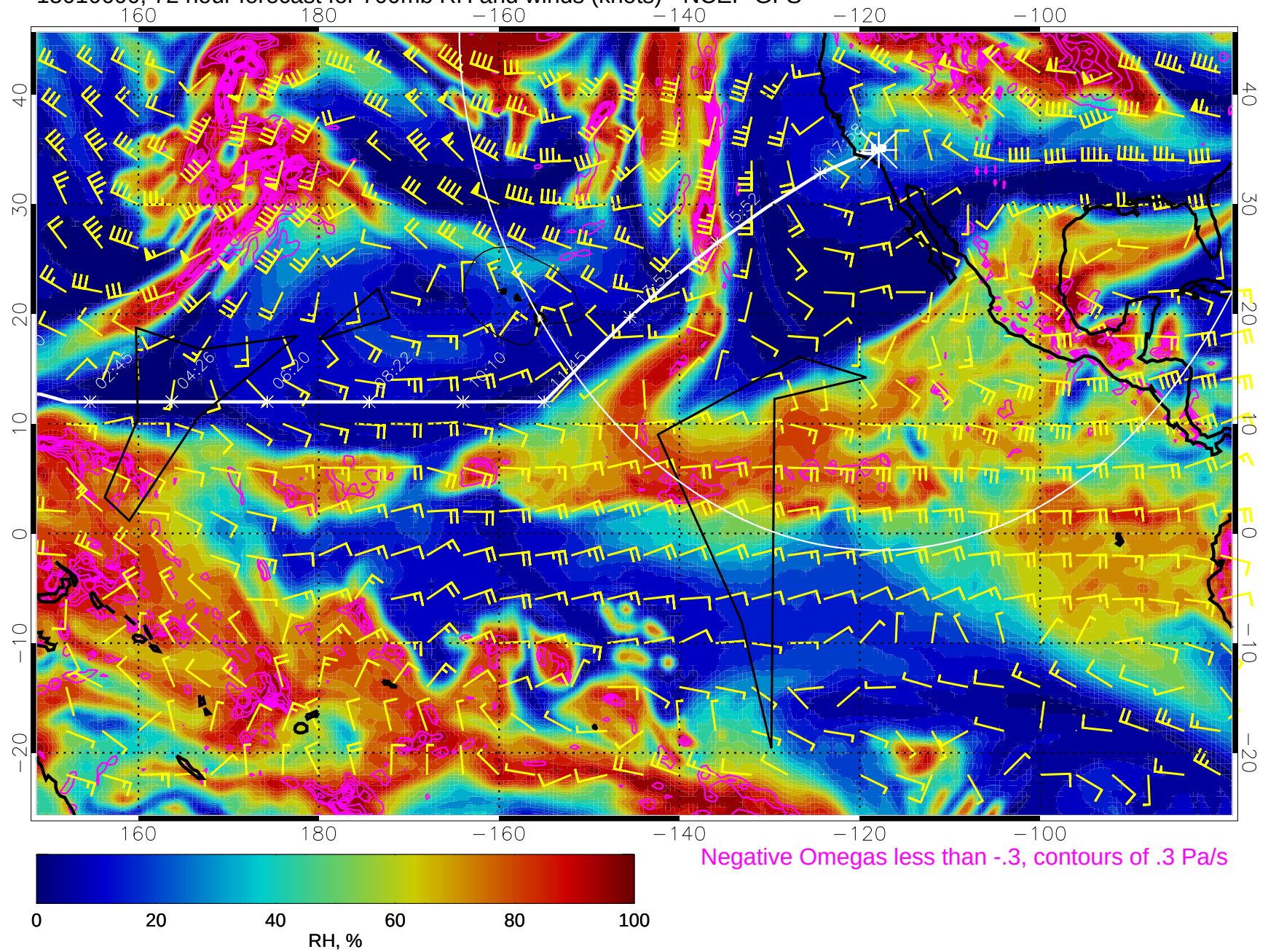
15010600, 72 hour forecast for 700mb RH and winds (knots) - NCEP GFS
