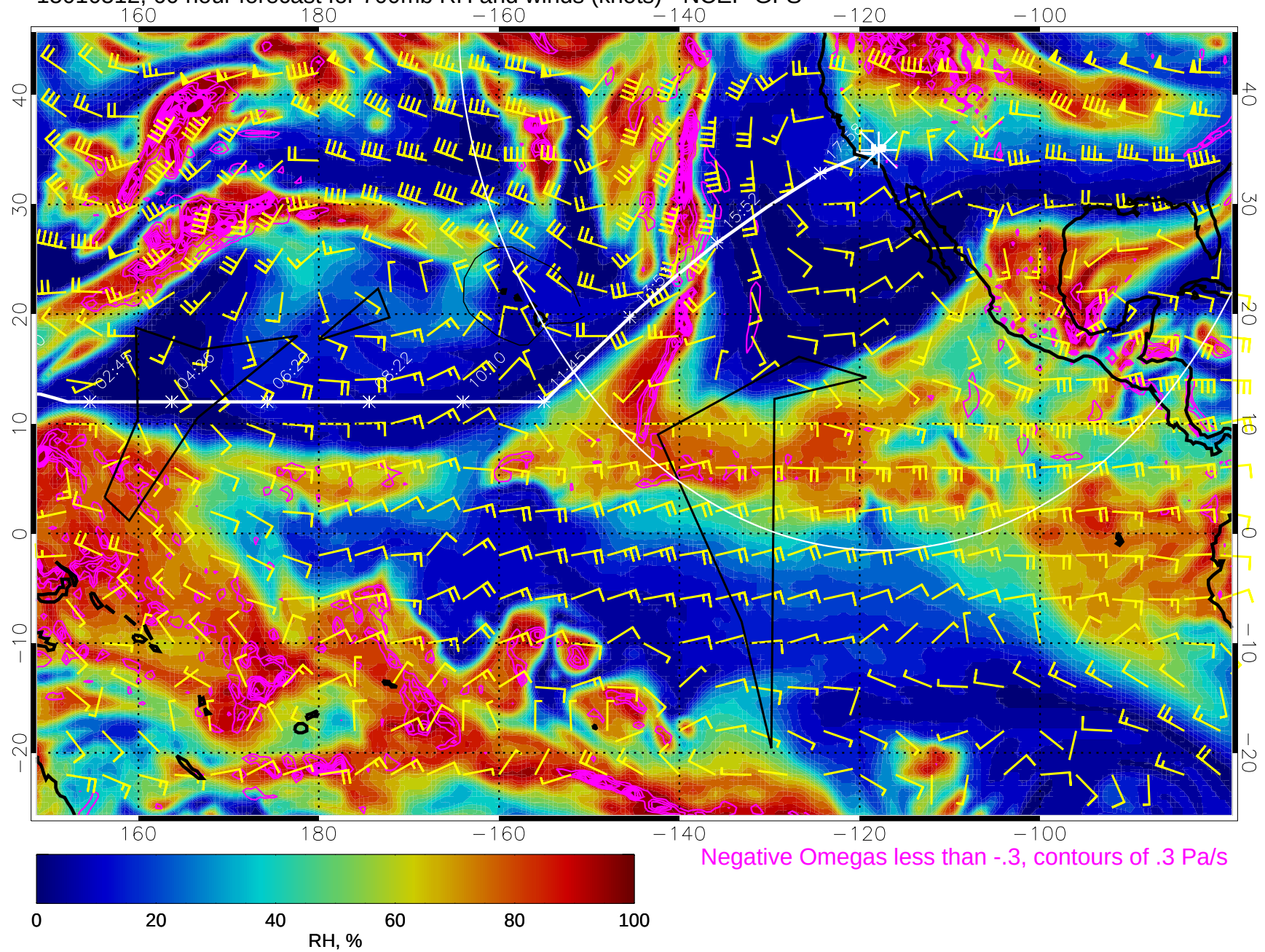
15010512, 60 hour forecast for 700mb RH and winds (knots) - NCEP GFS
