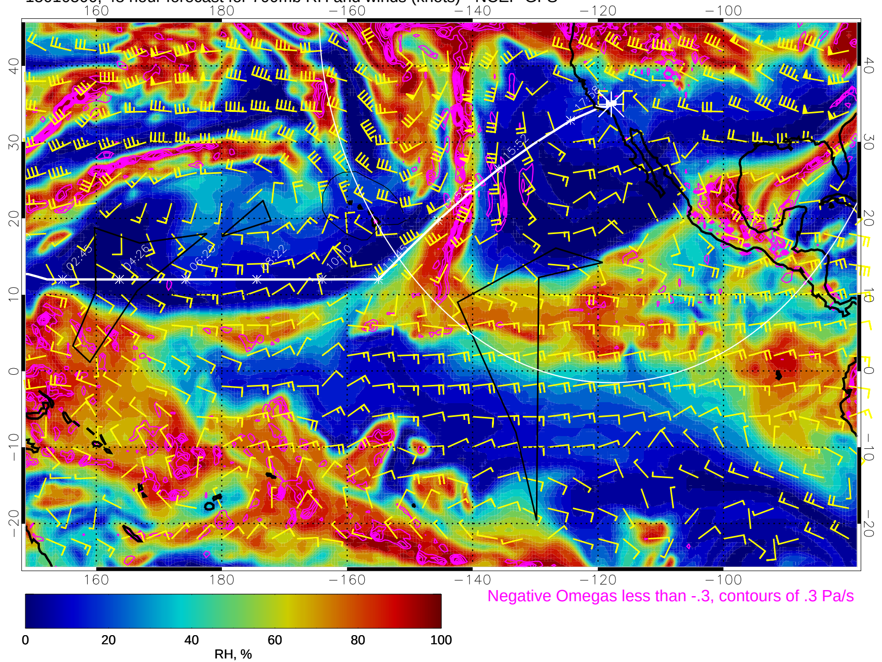
15010500, 48 hour forecast for 700mb RH and winds (knots) - NCEP GFS
