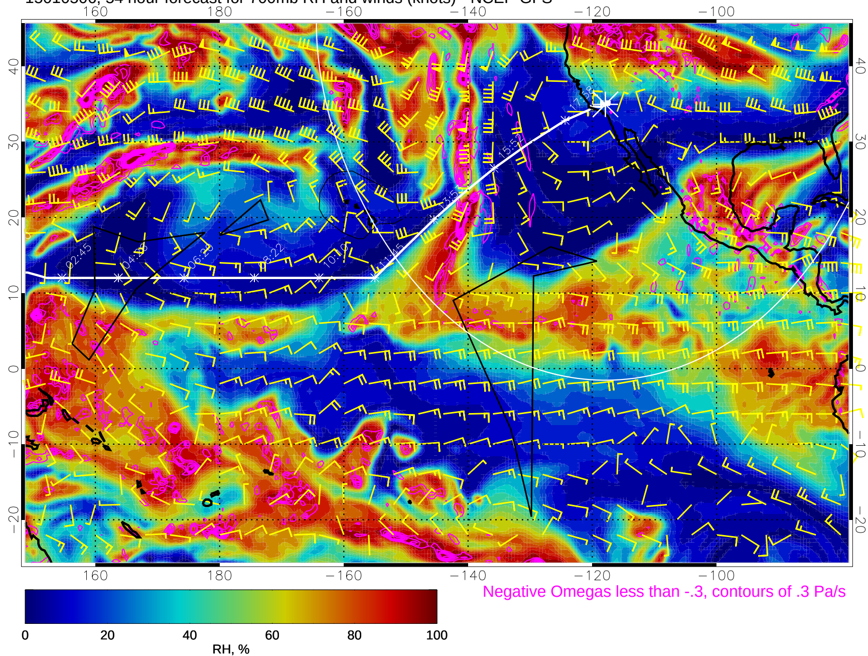
15010506, 54 hour forecast for 700mb RH and winds (knots) - NCEP GFS
