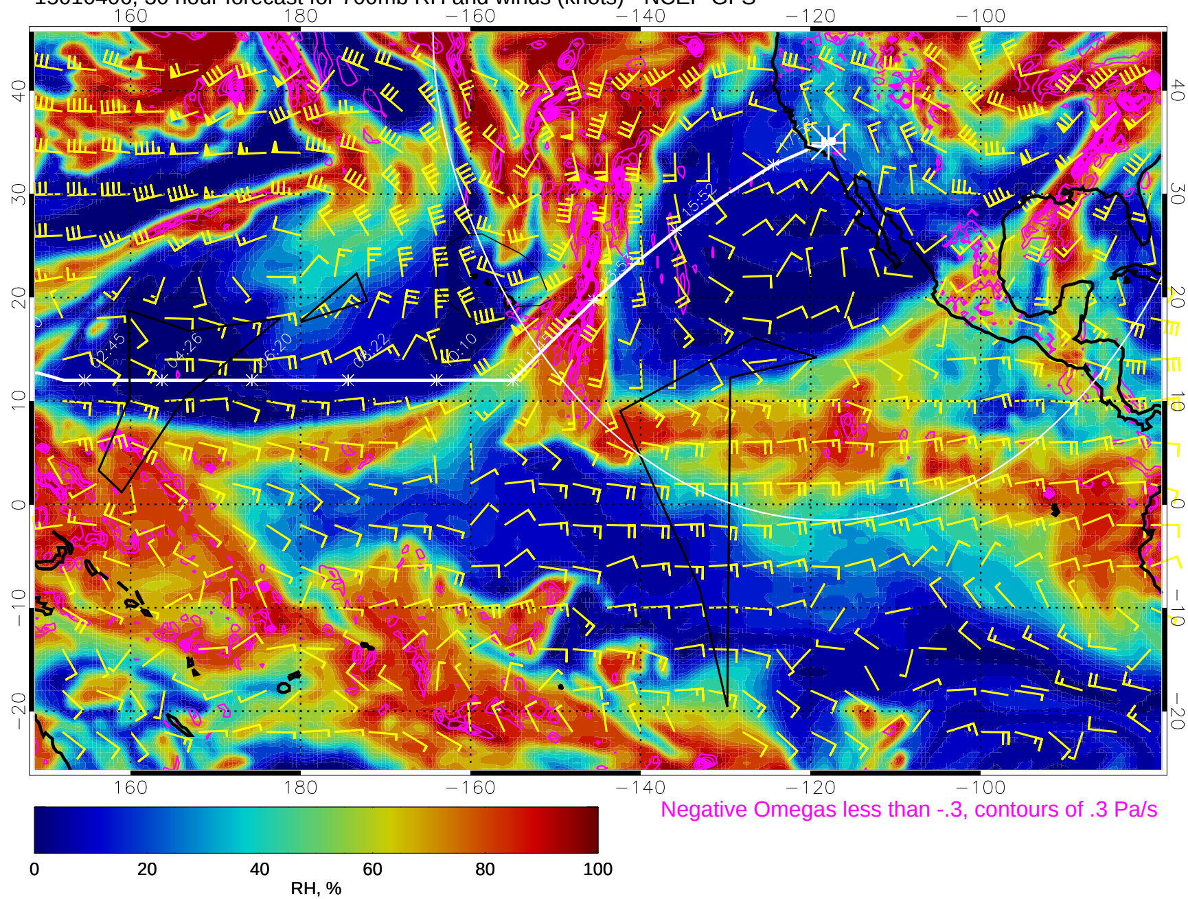
15010406, 30 hour forecast for 700mb RH and winds (knots) - NCEP GFS
