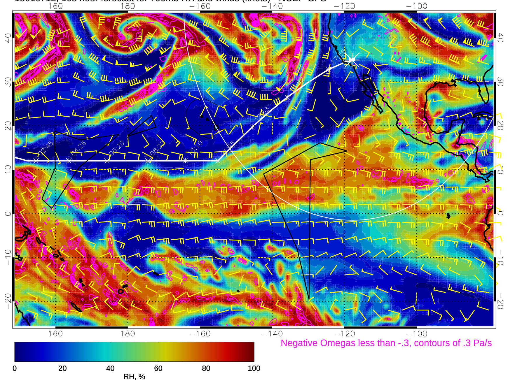
15010712, 108 hour forecast for 700mb RH and winds (knots) - NCEP GFS
