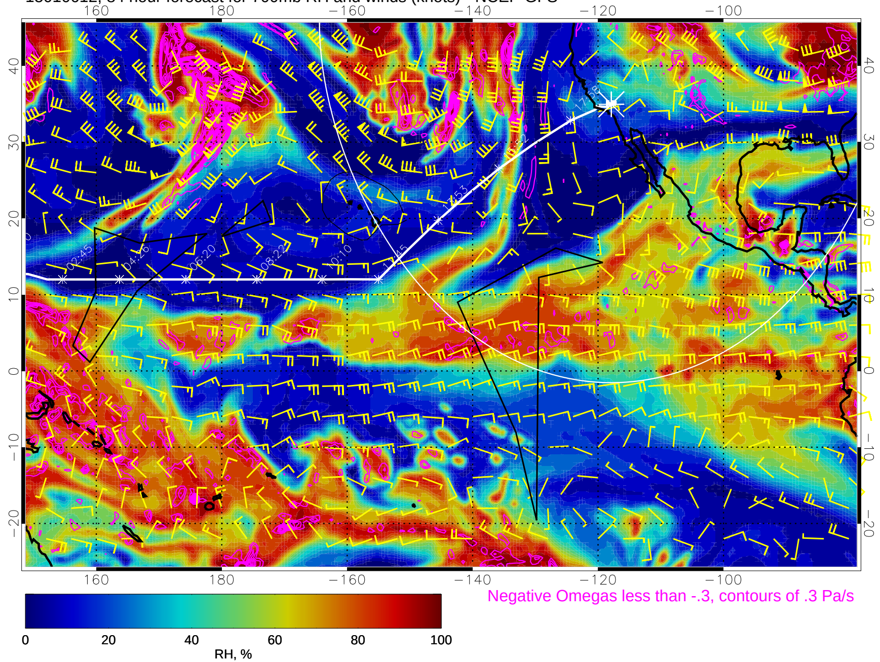
15010612, 84 hour forecast for 700mb RH and winds (knots) - NCEP GFS
