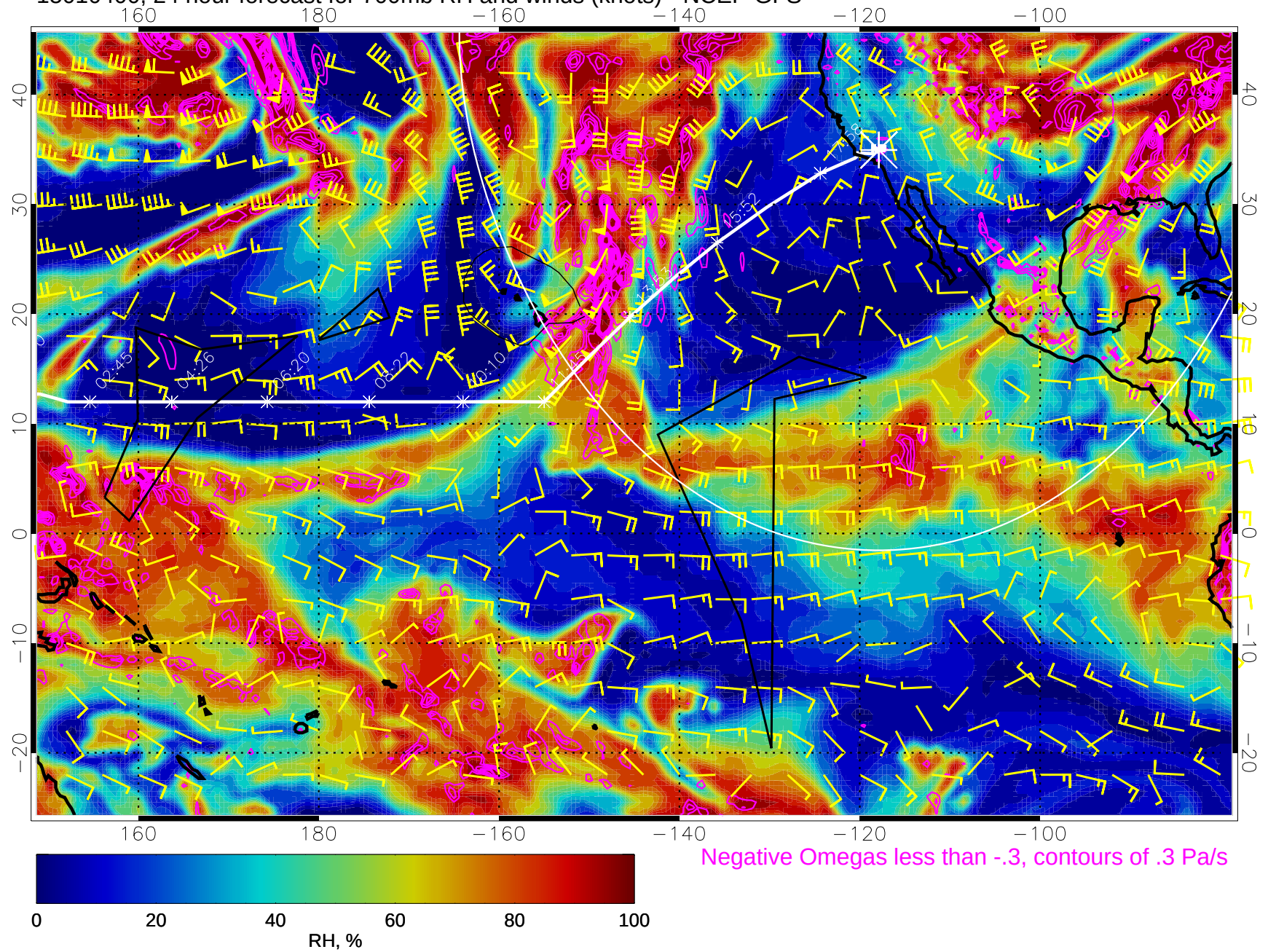
15010400, 24 hour forecast for 700mb RH and winds (knots) - NCEP GFS
