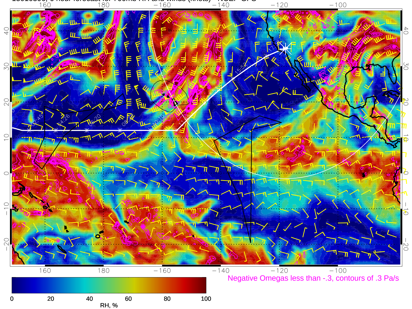
15010306, 6 hour forecast for 700mb RH and winds (knots) - NCEP GFS
