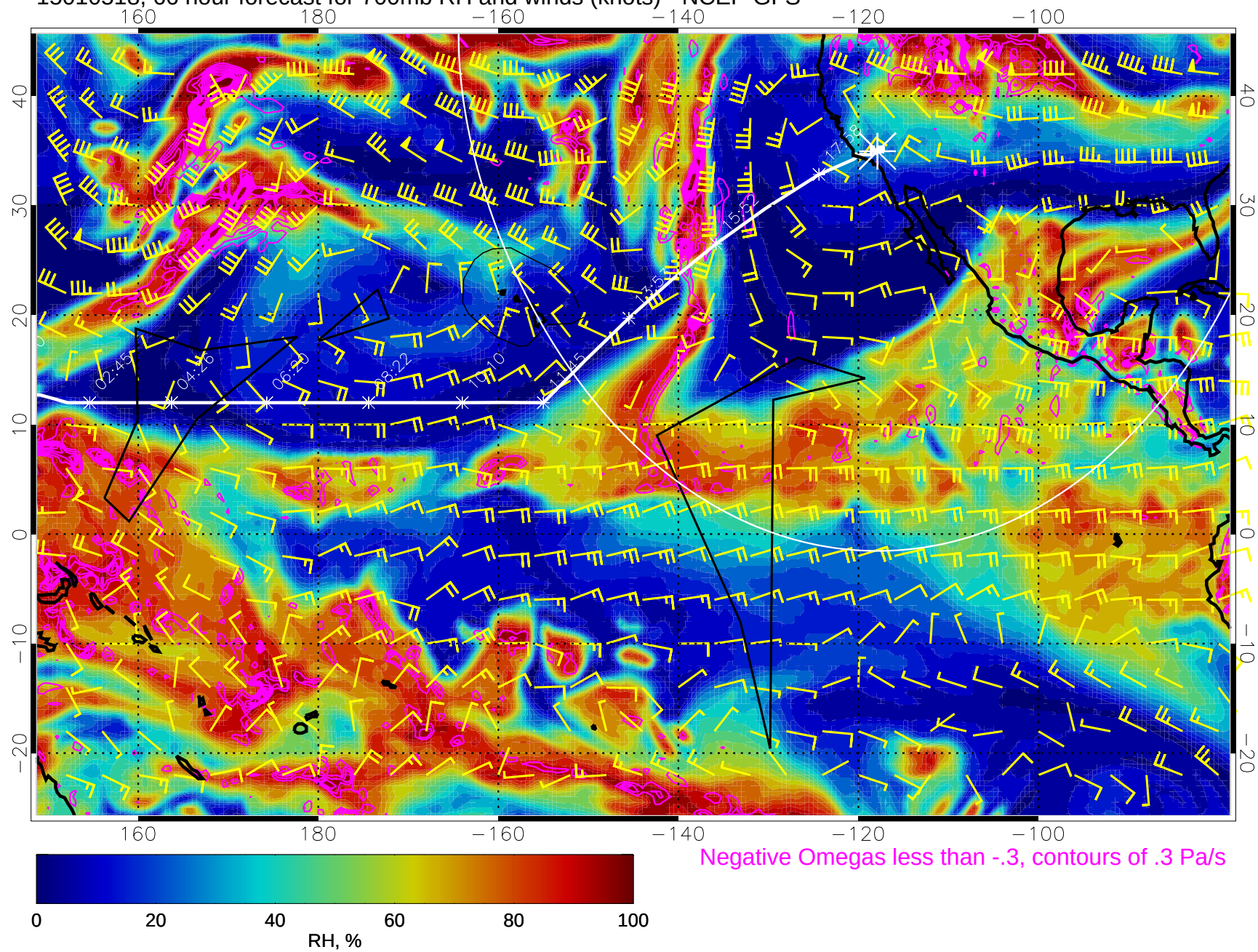
15010518, 66 hour forecast for 700mb RH and winds (knots) - NCEP GFS
