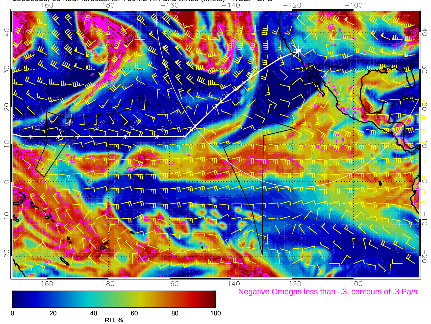
15010618, 90 hour forecast for 700mb RH and winds (knots) - NCEP GFS
