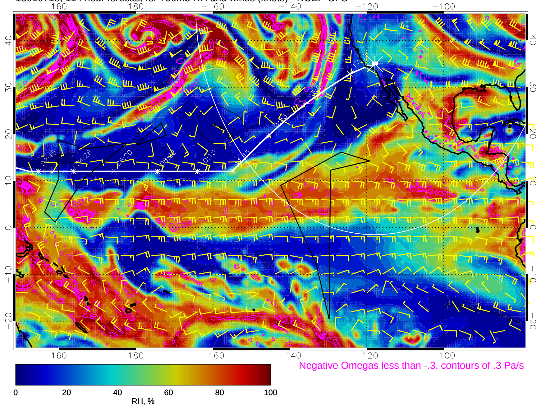
15010718, 114 hour forecast for 700mb RH and winds (knots) - NCEP GFS
