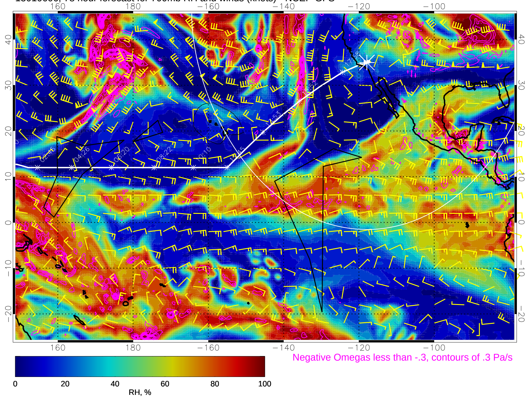
15010606, 78 hour forecast for 700mb RH and winds (knots) - NCEP GFS
