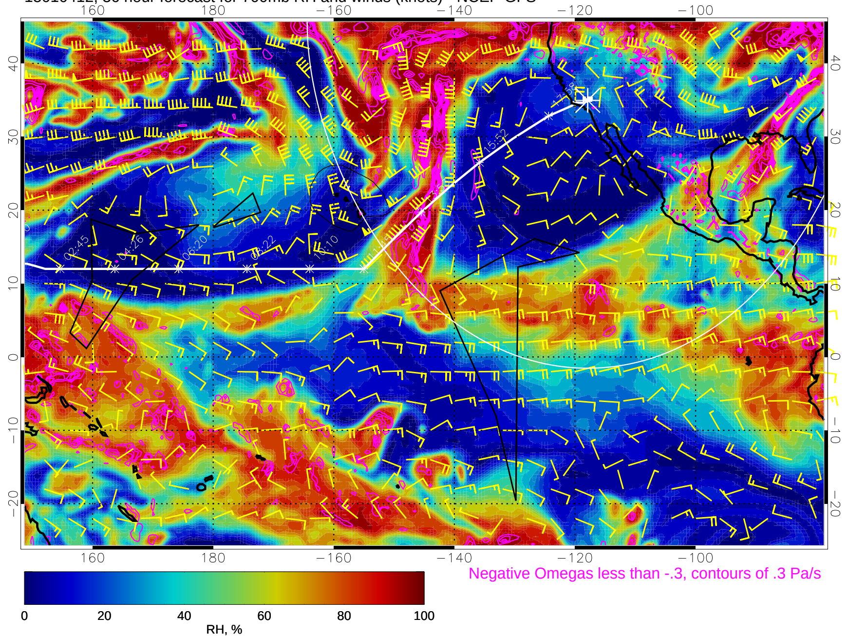
15010412, 36 hour forecast for 700mb RH and winds (knots) - NCEP GFS
