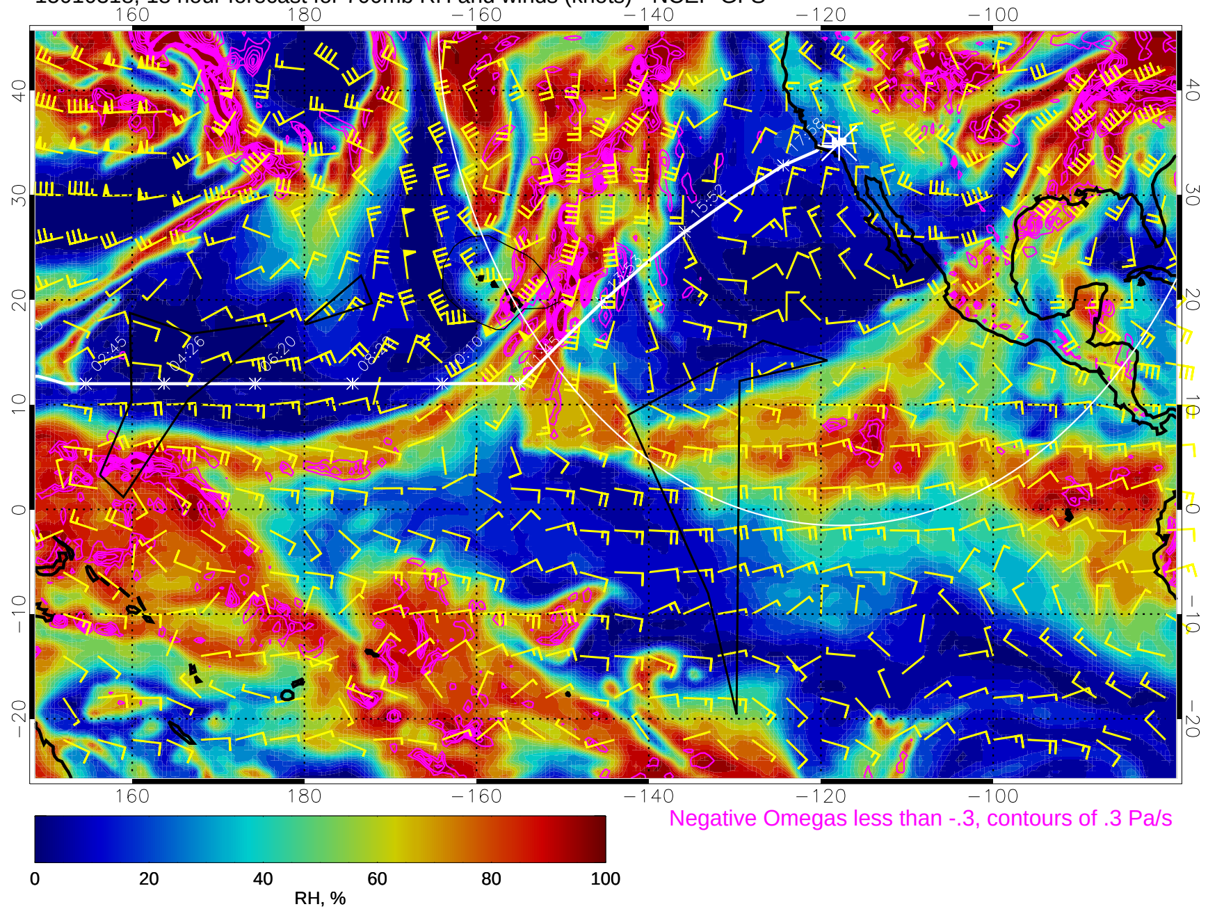
15010318, 18 hour forecast for 700mb RH and winds (knots) - NCEP GFS
