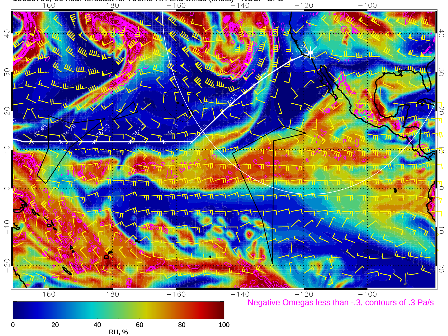
15010700, 96 hour forecast for 700mb RH and winds (knots) - NCEP GFS
