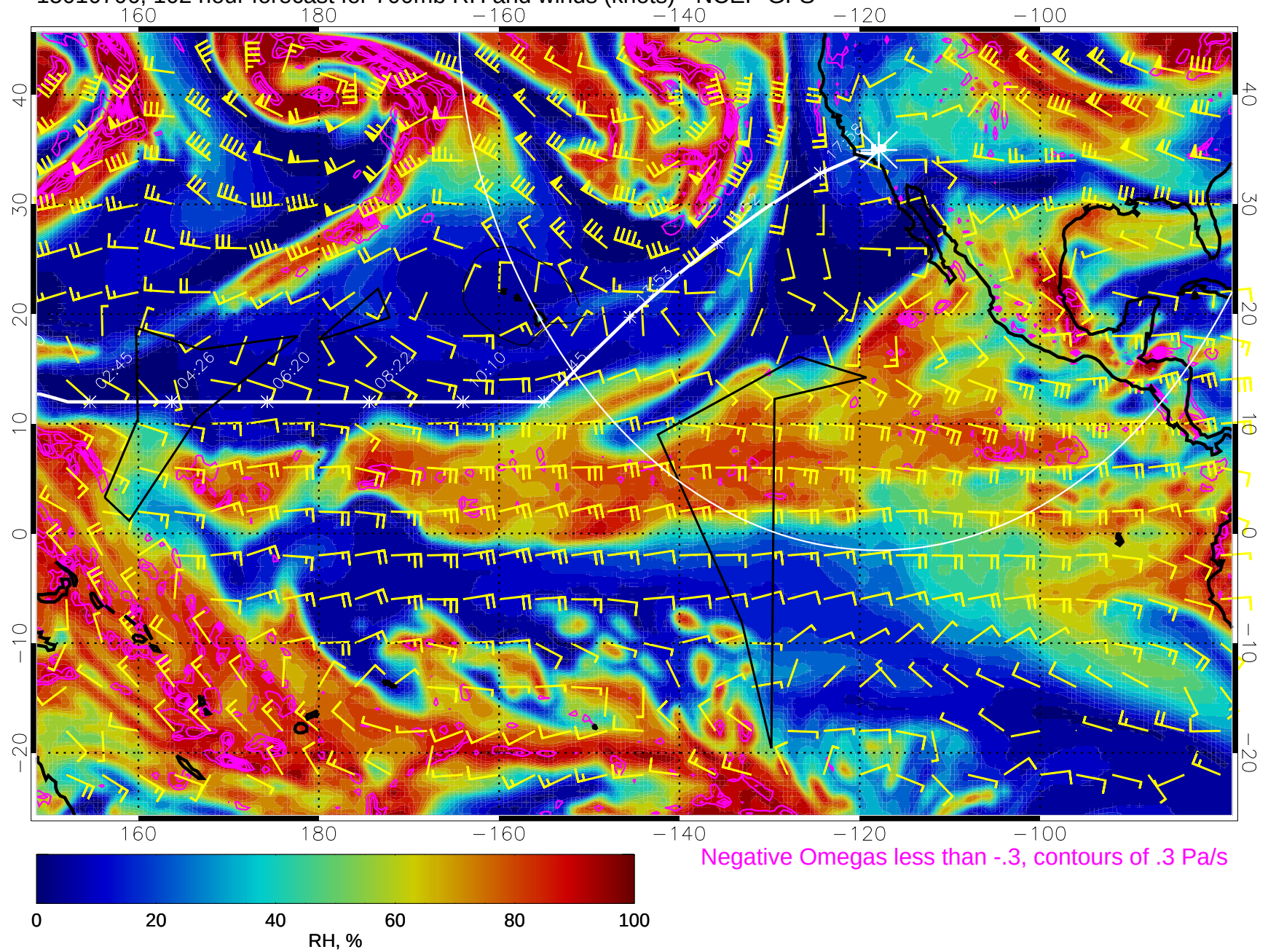
15010706, 102 hour forecast for 700mb RH and winds (knots) - NCEP GFS
