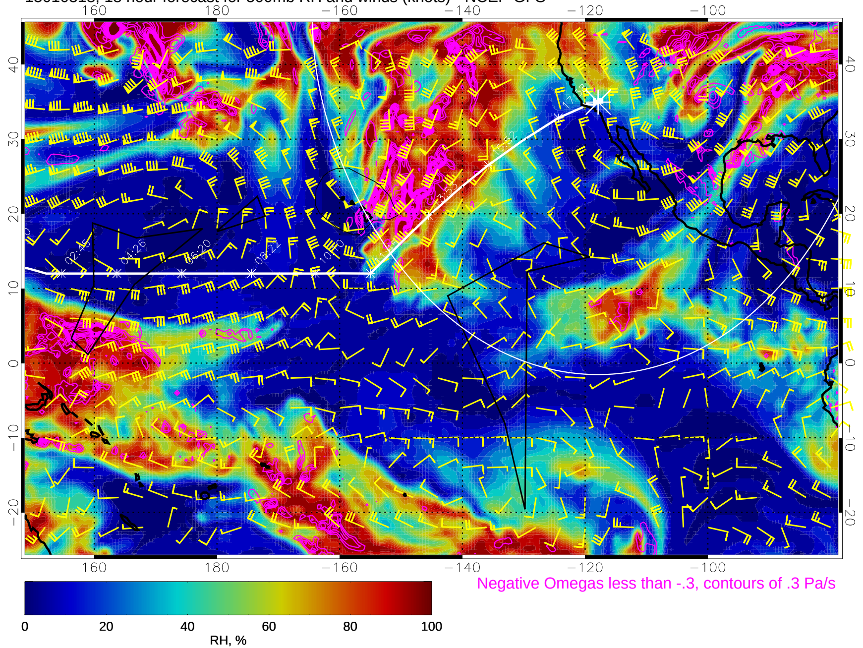
15010318, 18 hour forecast for 500mb RH and winds (knots) - NCEP GFS
