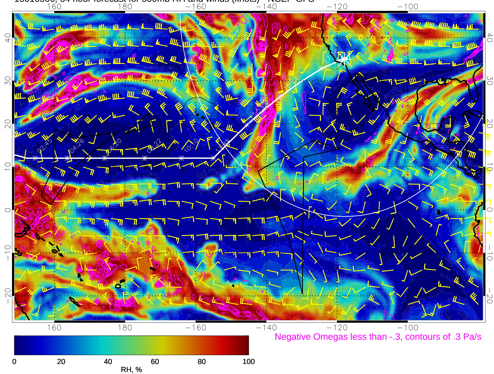
15010506, 54 hour forecast for 500mb RH and winds (knots) - NCEP GFS
