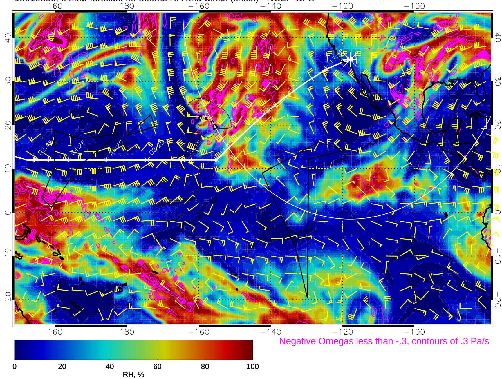
15010306, 6 hour forecast for 500mb RH and winds (knots) - NCEP GFS
