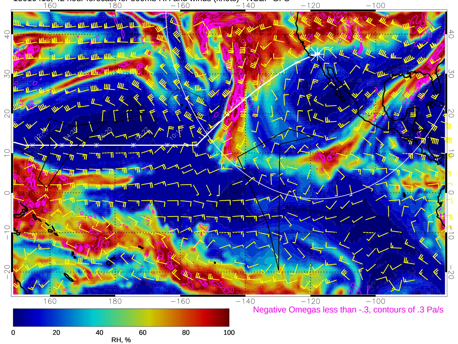
15010418, 42 hour forecast for 500mb RH and winds (knots) - NCEP GFS
