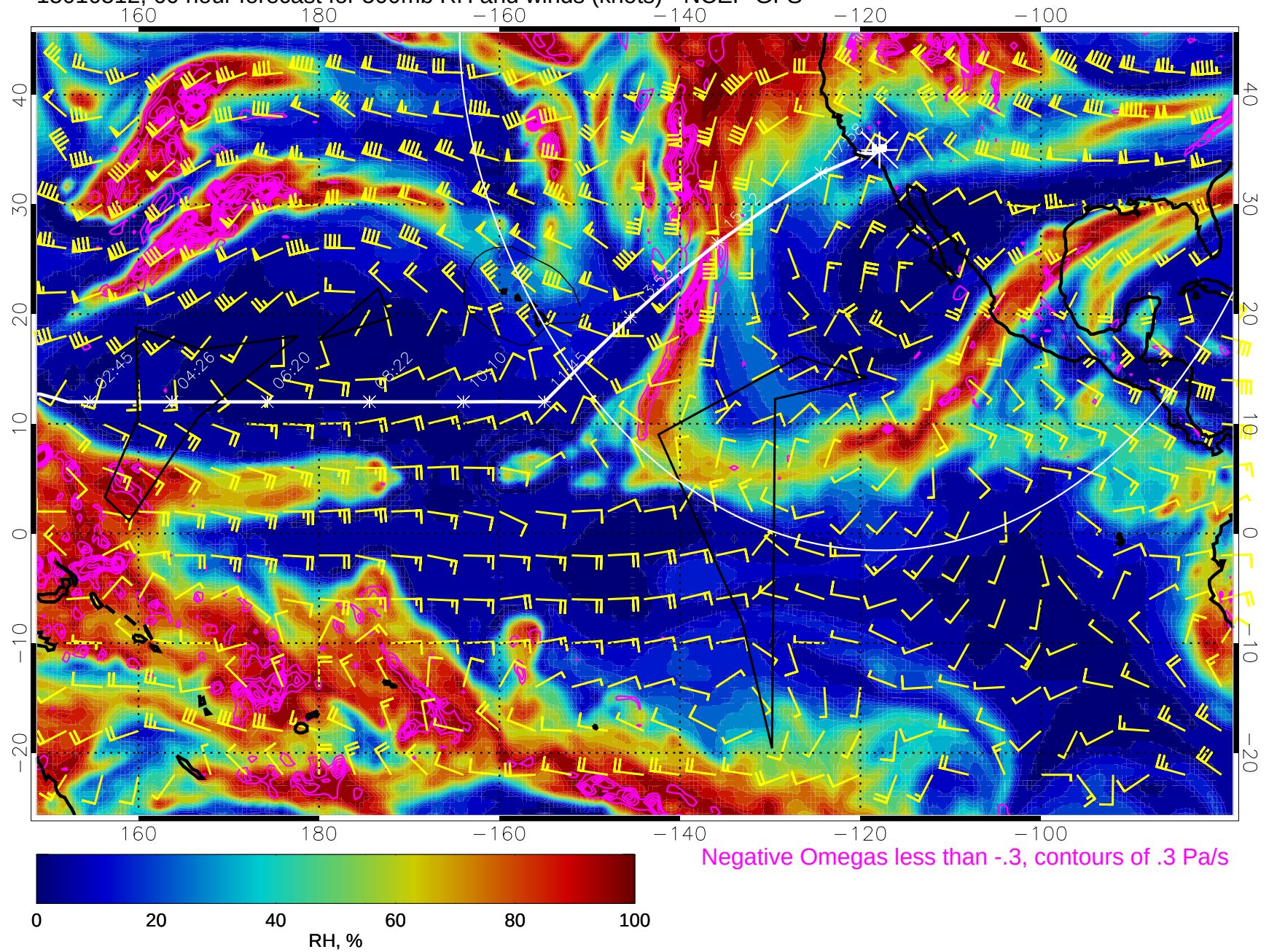
15010512, 60 hour forecast for 500mb RH and winds (knots) - NCEP GFS
