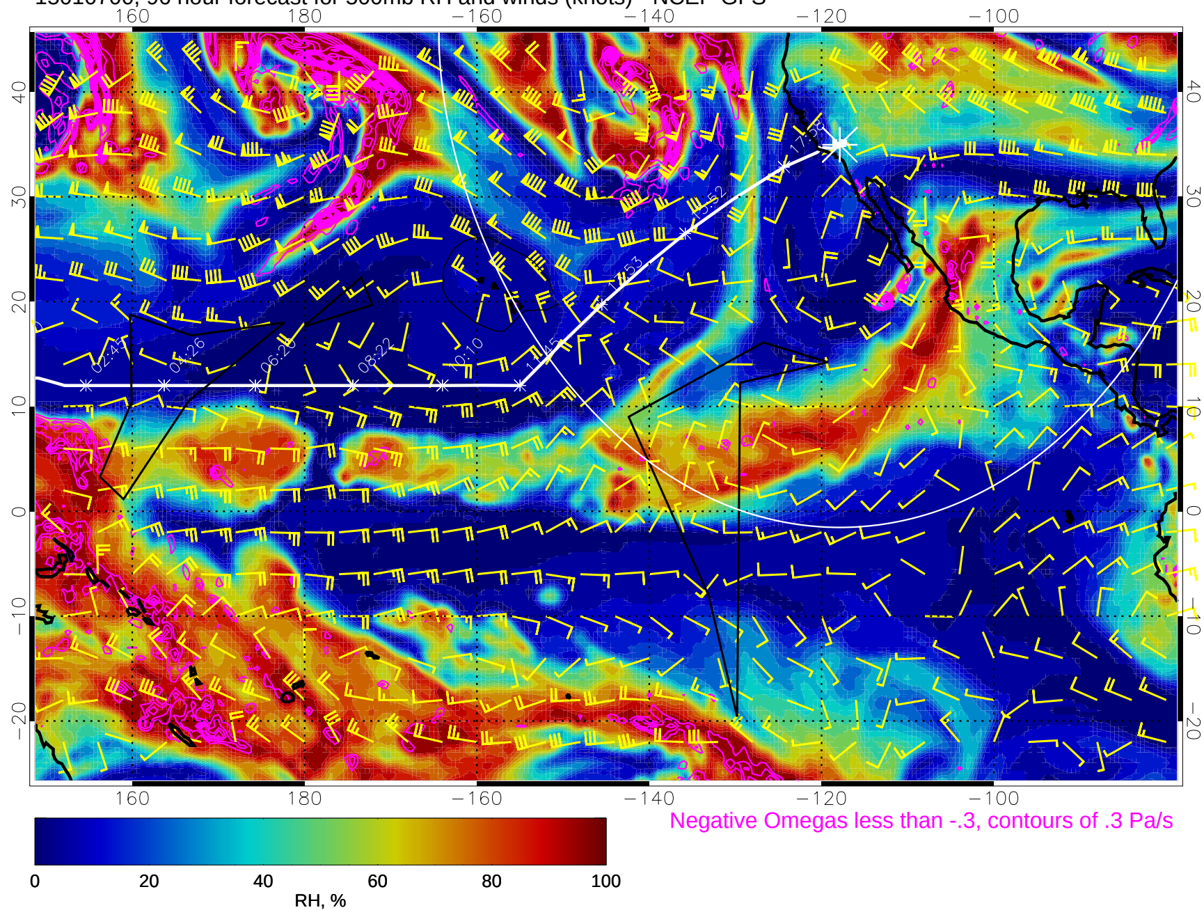
15010700, 96 hour forecast for 500mb RH and winds (knots) - NCEP GFS
