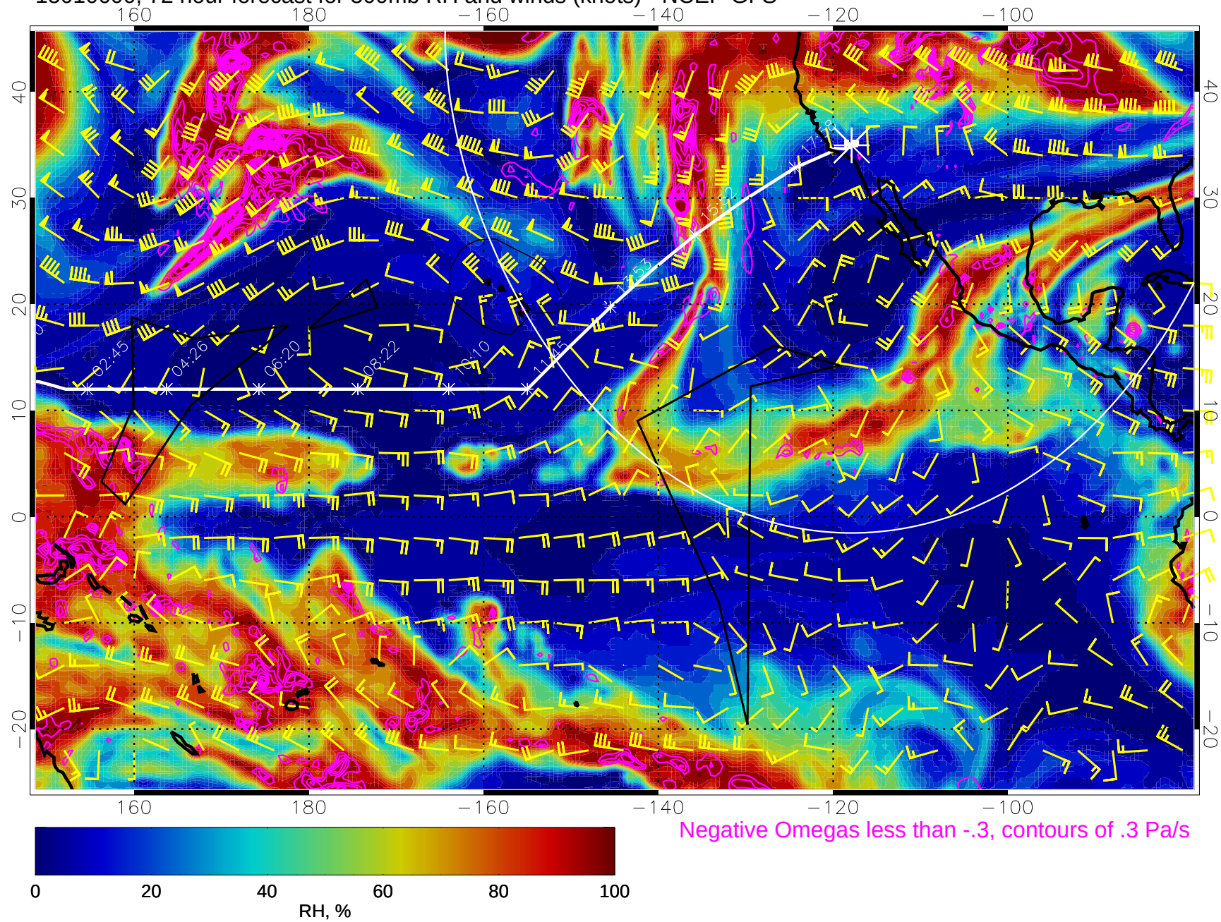
15010600, 72 hour forecast for 500mb RH and winds (knots) - NCEP GFS
