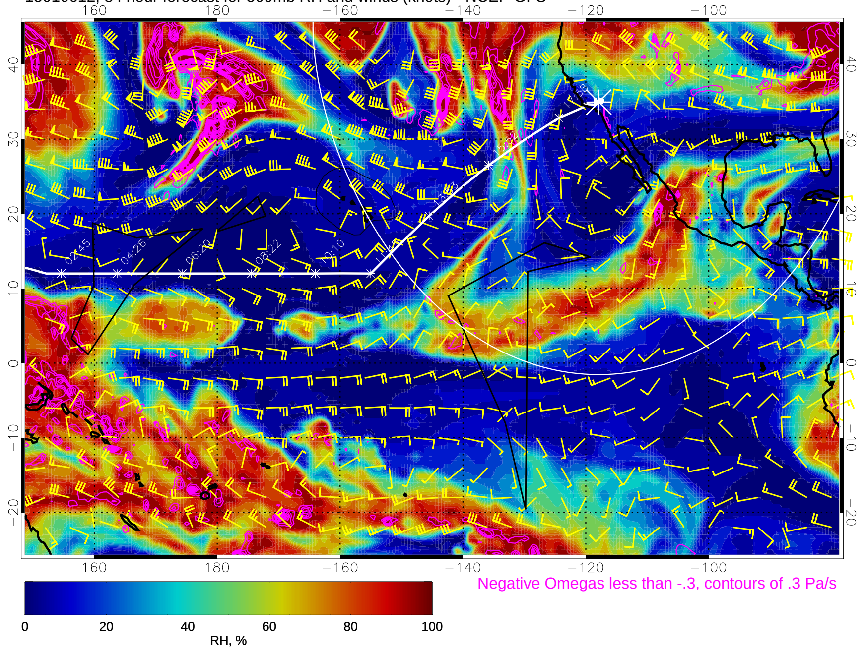
15010612, 84 hour forecast for 500mb RH and winds (knots) - NCEP GFS
