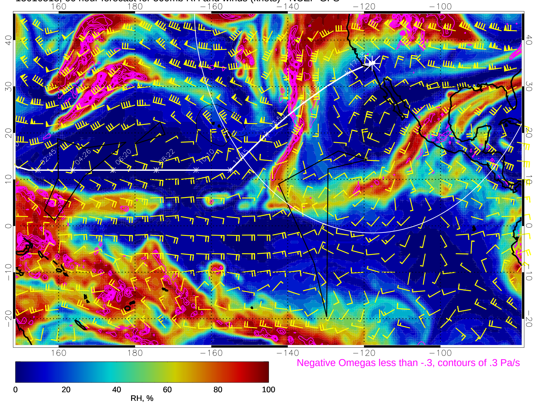
15010518, 66 hour forecast for 500mb RH and winds (knots) - NCEP GFS
