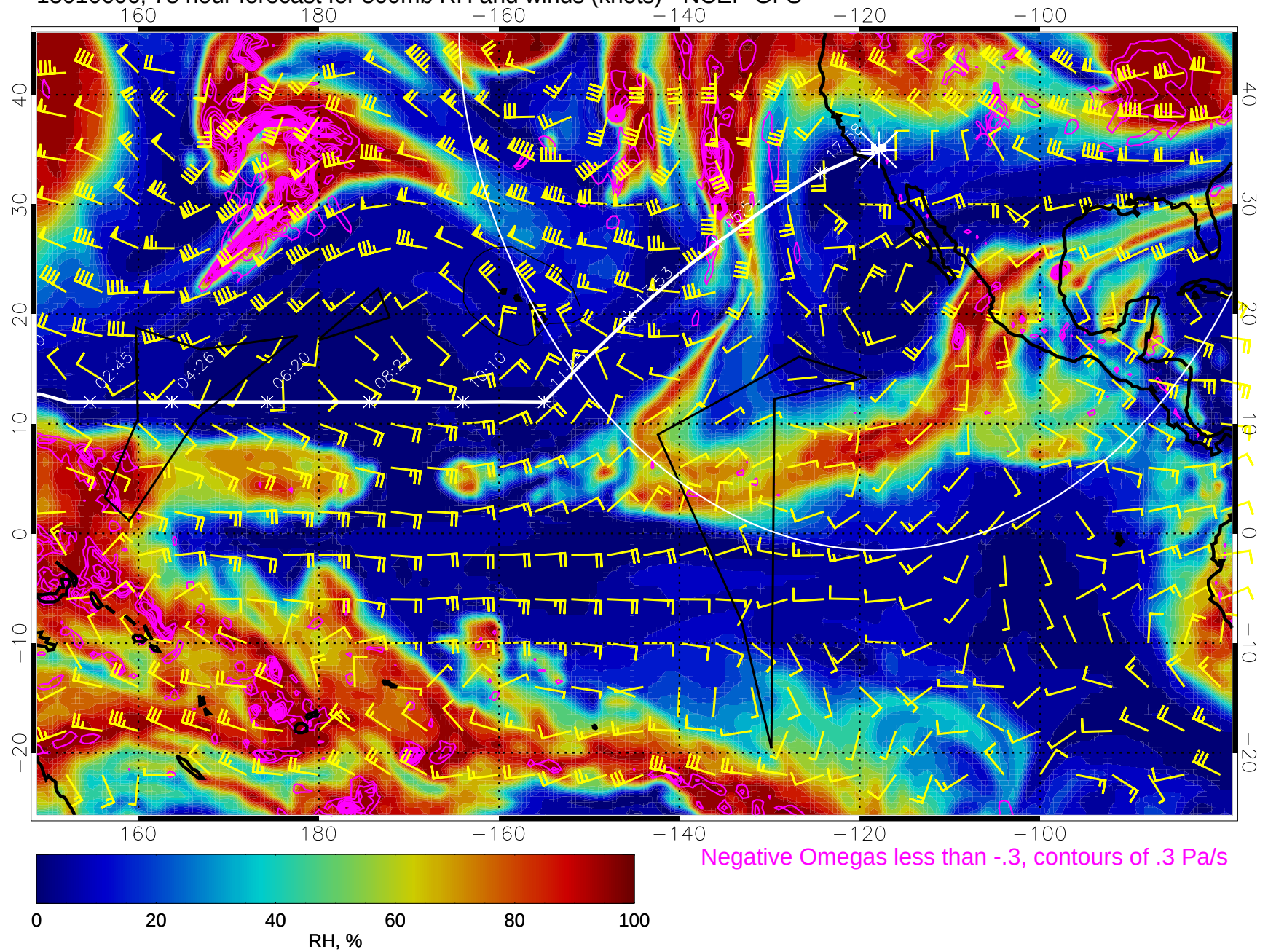
15010606, 78 hour forecast for 500mb RH and winds (knots) - NCEP GFS
