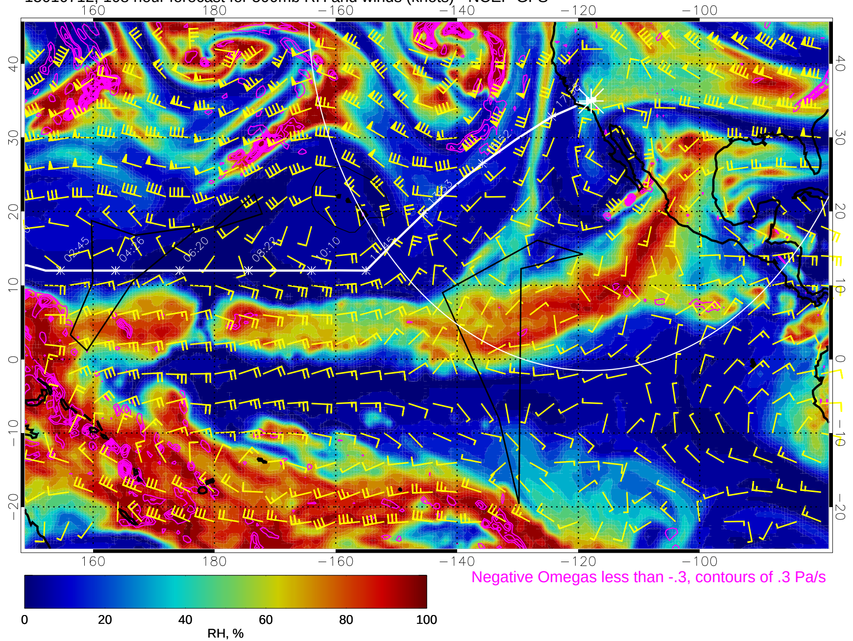
15010712, 108 hour forecast for 500mb RH and winds (knots) - NCEP GFS
