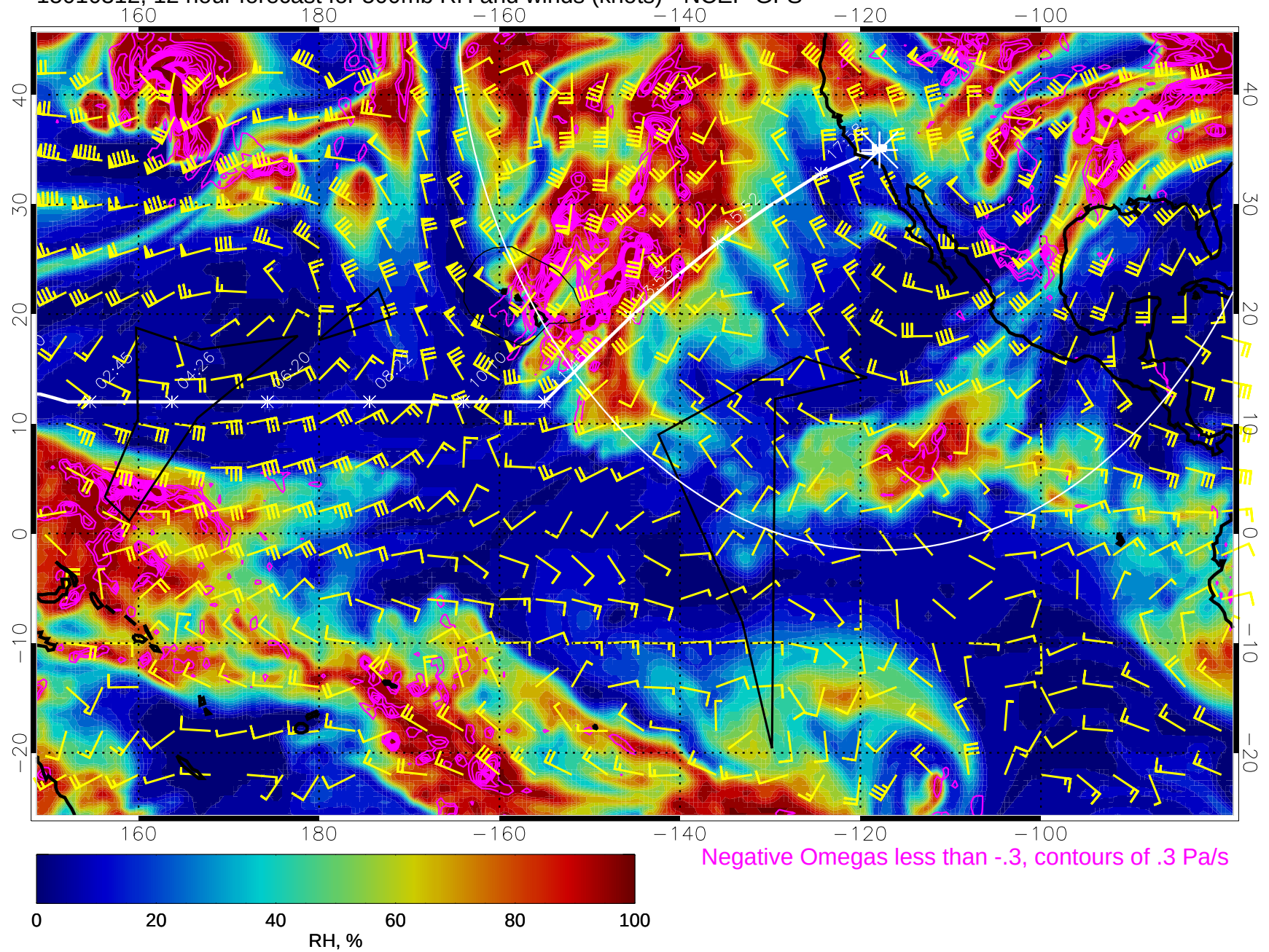
15010312, 12 hour forecast for 500mb RH and winds (knots) - NCEP GFS
