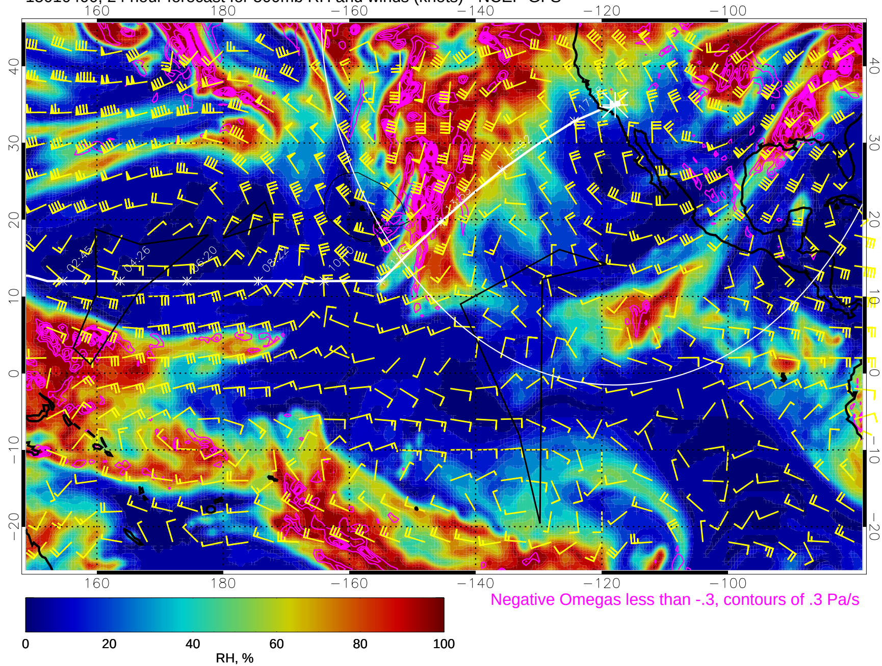
15010400, 24 hour forecast for 500mb RH and winds (knots) - NCEP GFS
