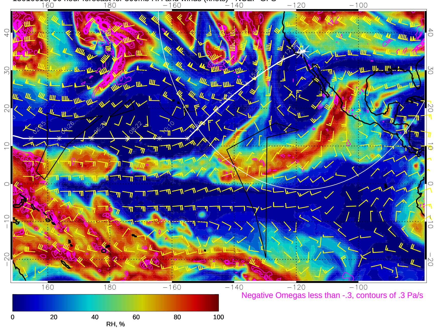
15010618, 90 hour forecast for 500mb RH and winds (knots) - NCEP GFS
