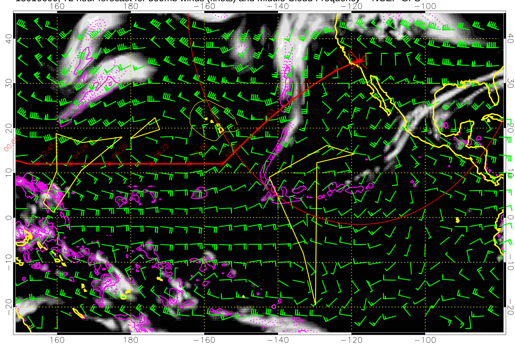
15010600, 72 hour forecast for 500mb winds (knots) and Middle Cloud Frequency -- NCEP GFS
