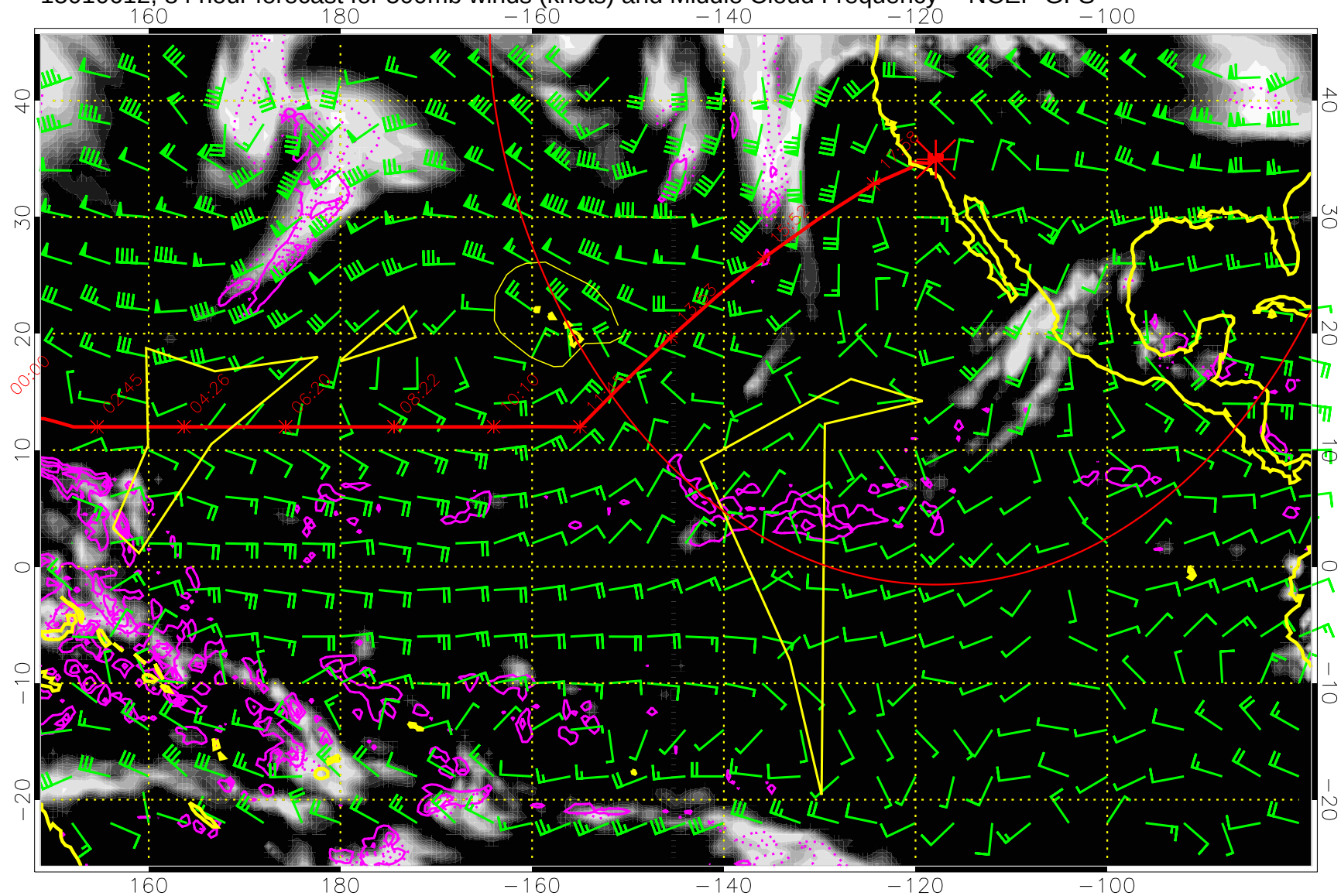
15010612, 84 hour forecast for 500mb winds (knots) and Middle Cloud Frequency -- NCEP GFS
