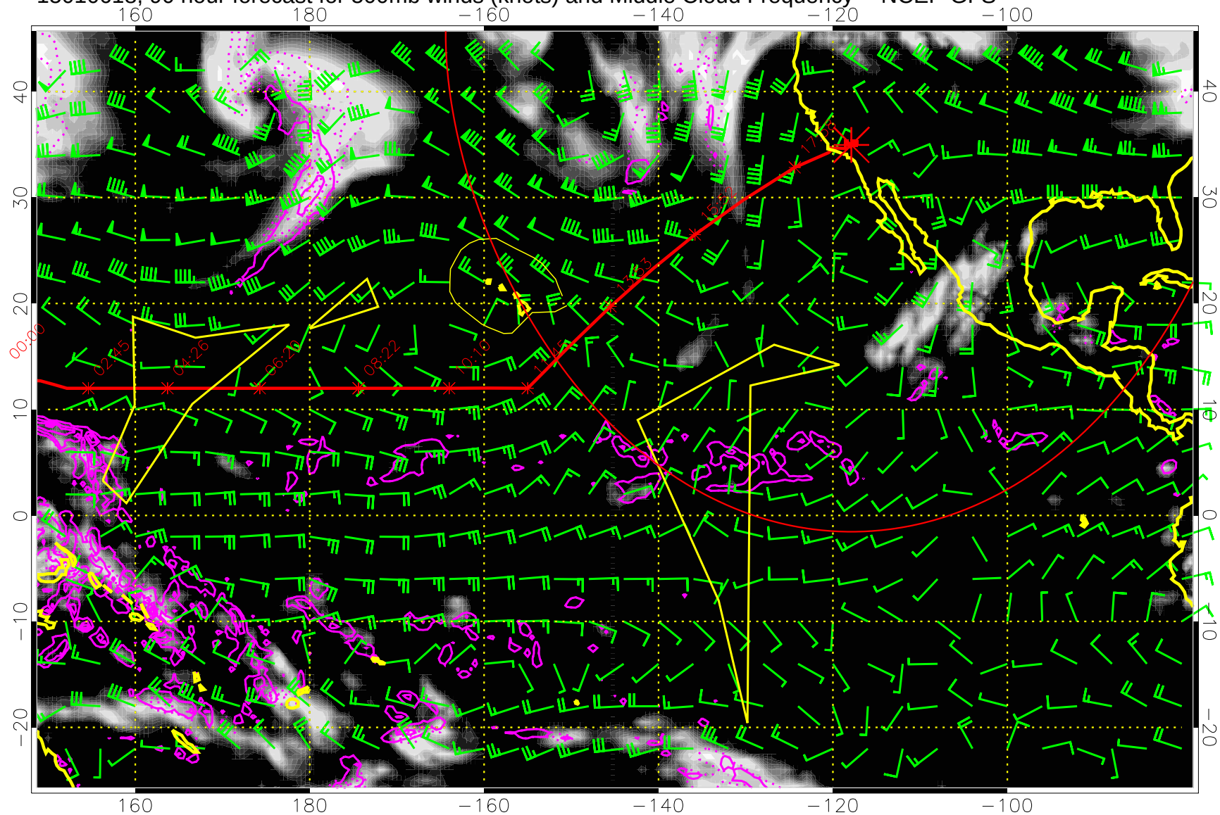
15010618, 90 hour forecast for 500mb winds (knots) and Middle Cloud Frequency -- NCEP GFS
