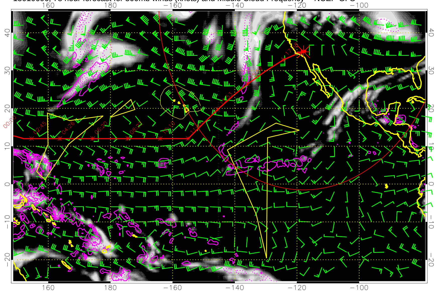
15010606, 78 hour forecast for 500mb winds (knots) and Middle Cloud Frequency -- NCEP GFS
