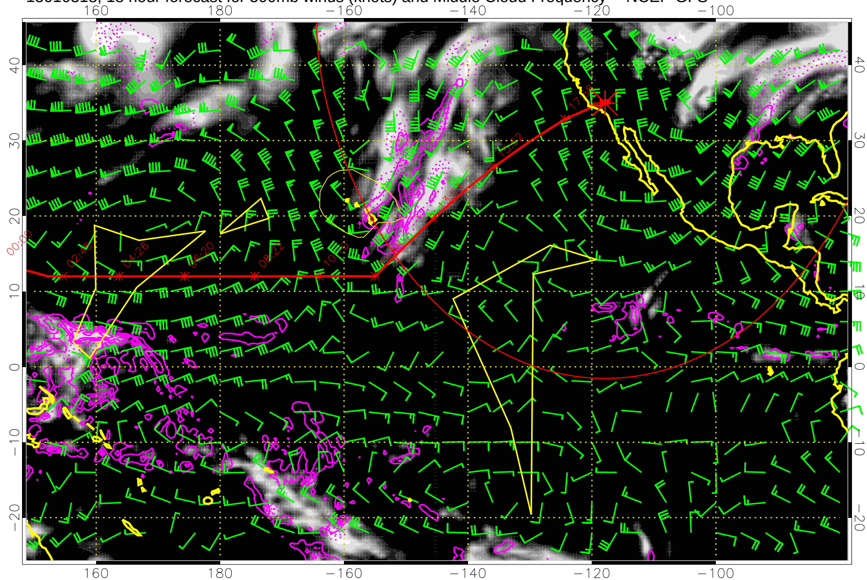
15010318, 18 hour forecast for 500mb winds (knots) and Middle Cloud Frequency -- NCEP GFS
