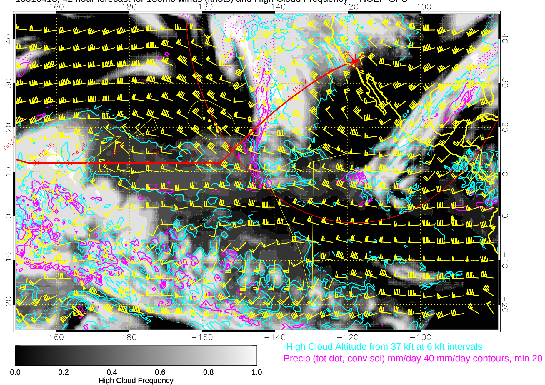
15010418, 42 hour forecast for 150mb winds (knots) and High Cloud Frequency -- NCEP GFS
