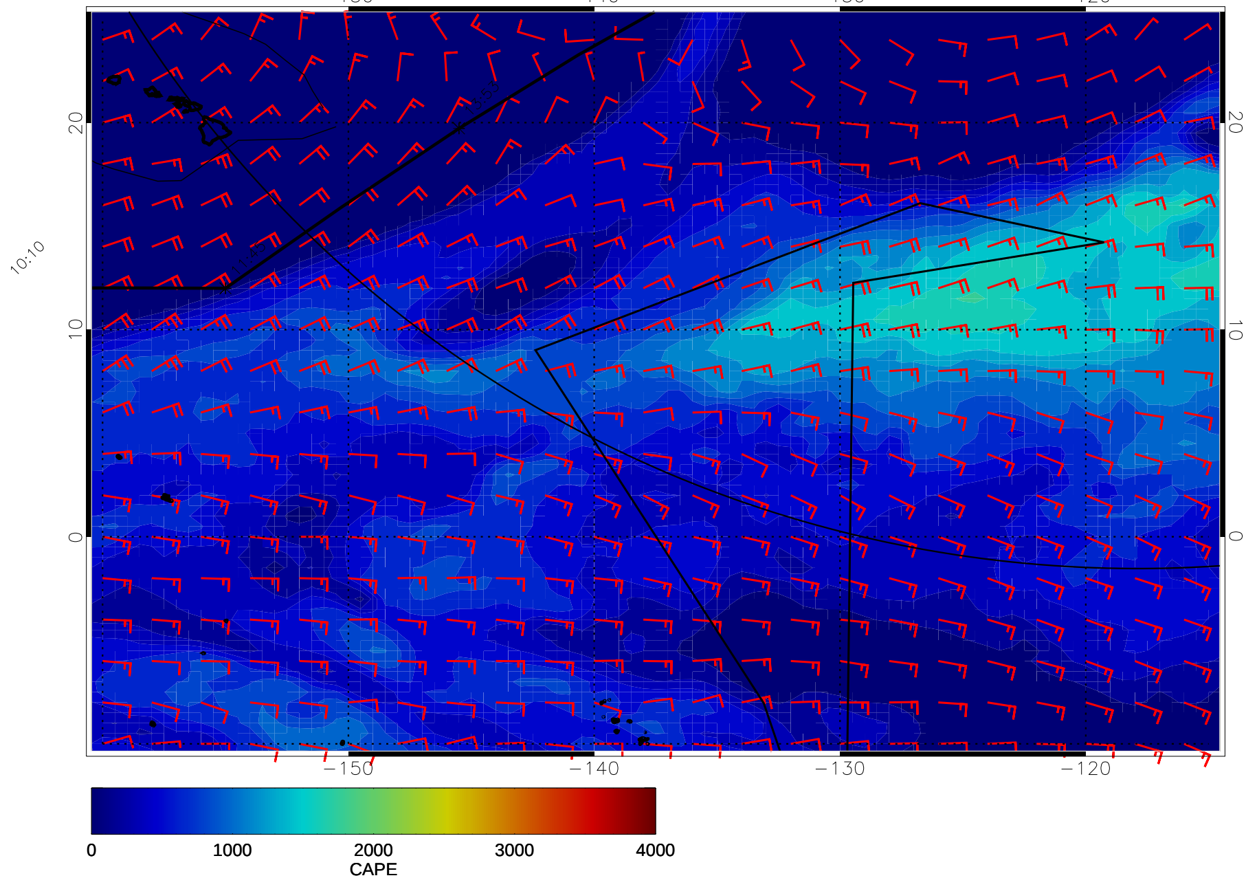
15010706, 102 hour forecast for CAPE and surface winds (knots) -- NCEP GFS
